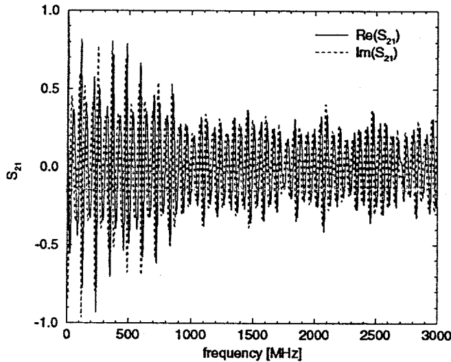
Figure 3. Uncalibrated S_{21} Parameter of the Kicker Half Module
