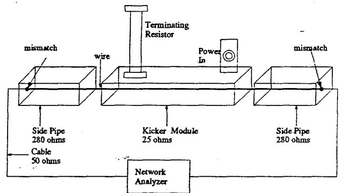
Figure 2. Bench Setup for Wire Measurement
