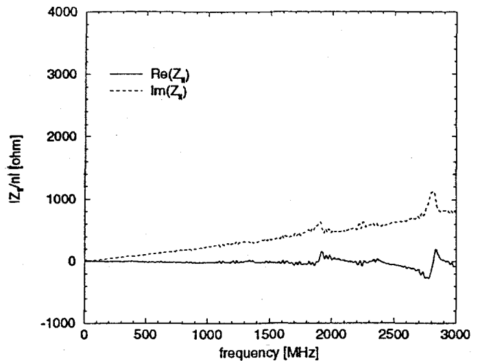
Figure 7. Kicker Impedance with Copper Strips
