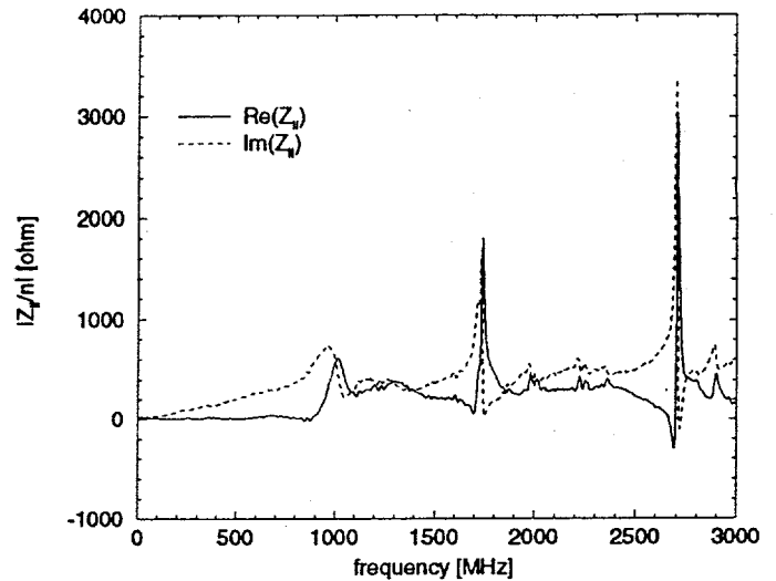
Figure 5. Injection Kicker Half Module Impedance
