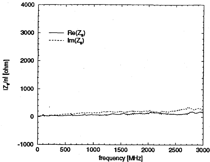
Figure 6. Kicker Impedance with Conductively Coated Ceramic Pipe
