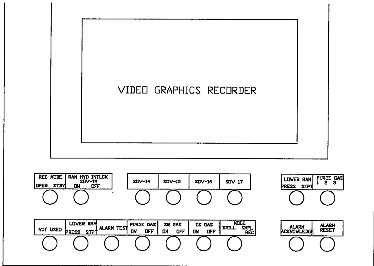
Figure 11 Video Graphic Recorder and HBD Instrumentation Controls
