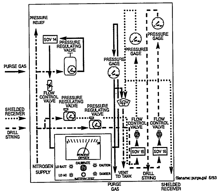
Figure 18) Purge Gas Controls.
