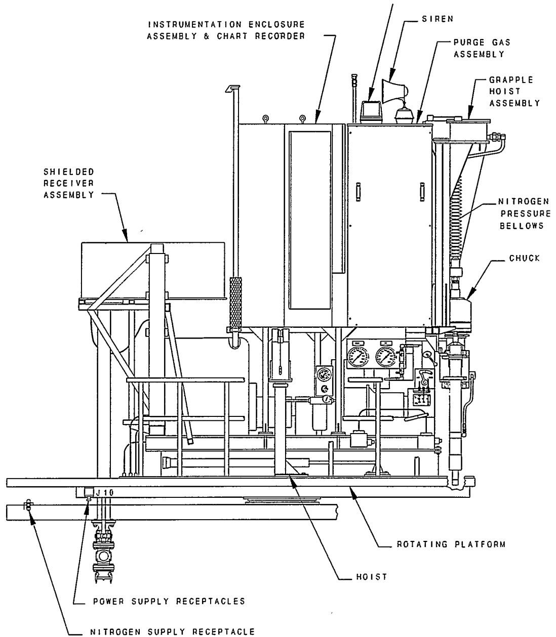
Figure 2) System Controls and Alarms (Driver Side). Note: Drawing is of system 2, an accurate drawing for systems 3&4 is not available and Minor difference from systems 3 and 4 exist.
