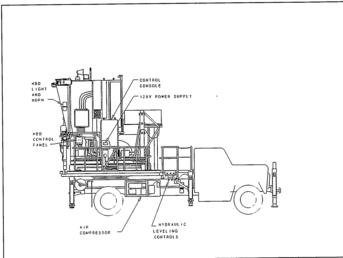
Figure 1) System Controls and Alarms (Passenger Side).
