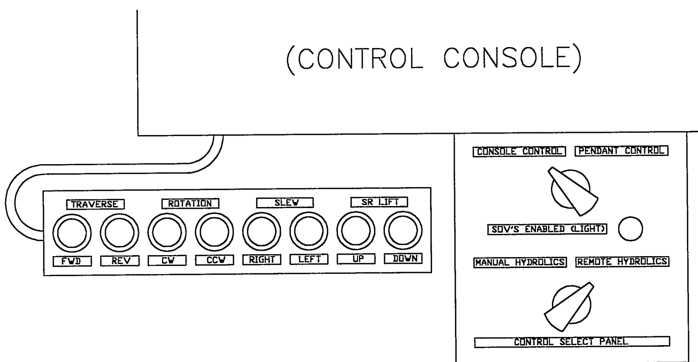
Figure 8) Pendant Controls and Control Select Panel
