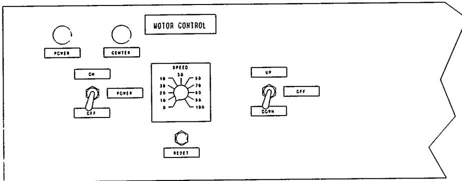
Figure 13) Shielded Receiver Hoist Motor Panel.
