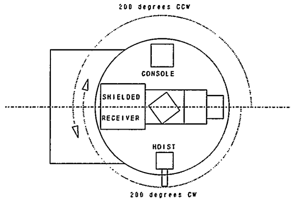
Figure 9) Platform Rotation from Home Position.
