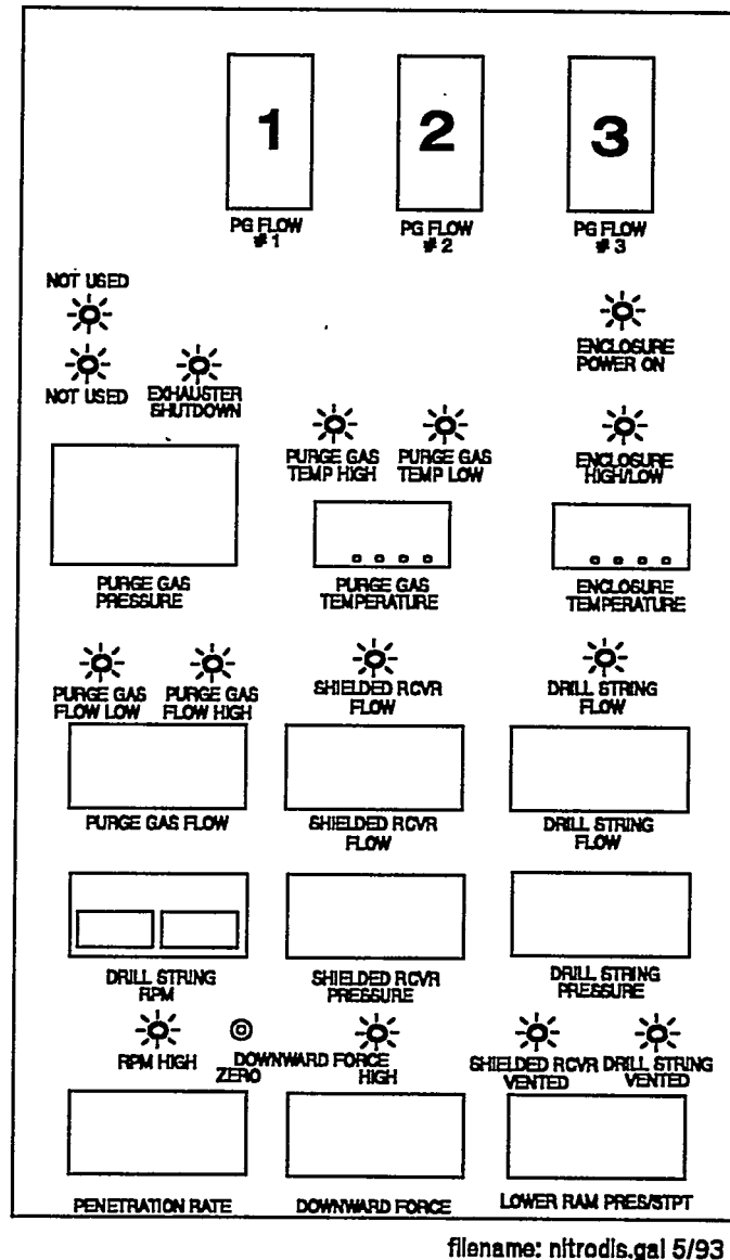
Figure 16) Instrumentation Display Panel.
