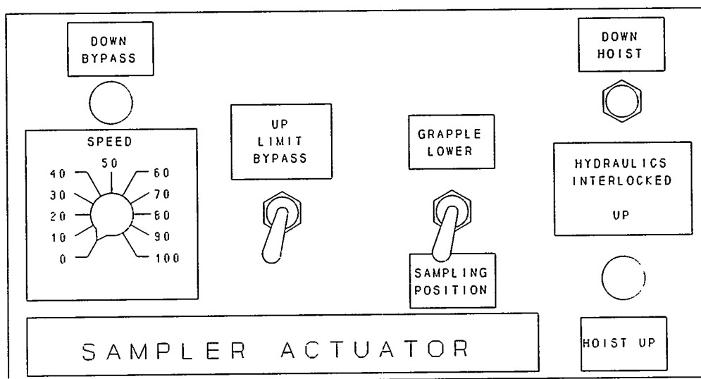
Figure 10) Drill Rig Actuator Controls
