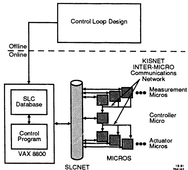
Figure 2: Feedback System Architecture.
