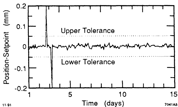
Figure 5: History Plot of Feedback Control.
