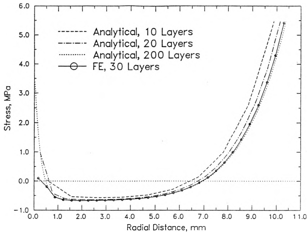
Figure 4. Circumferential Stresses in Capacitor Winding
