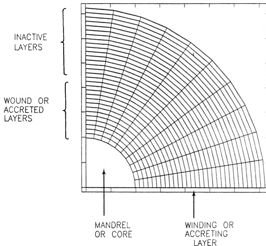
Figure 2. Finite Element Approach to Tape Winding
