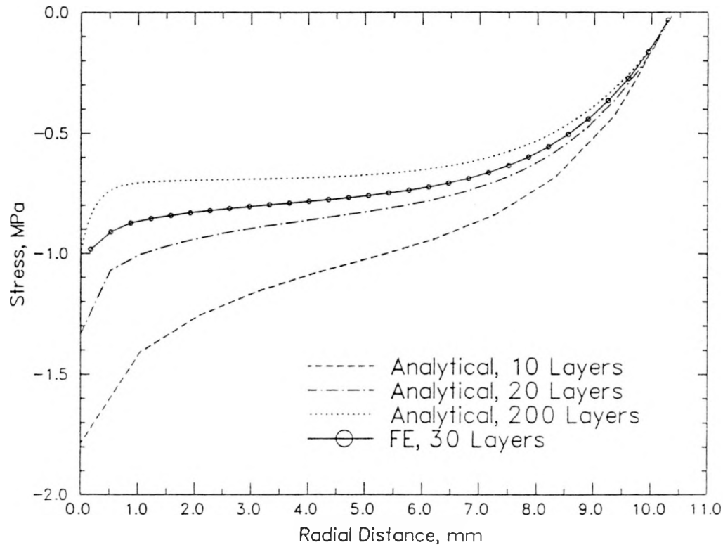
Figure 3. Radial Stresses in Capacitor Winding
