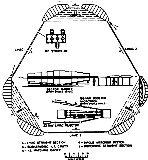
Fig. 1. Schematic of the Argonne National Laboratory 4 GeV Electron Microtron-GEM
