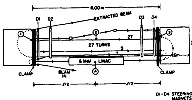
Fig. 2. Racetrack Microtron (RTM) Layout
