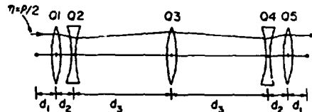
Fig. 7. Three focussing systems used in the hexatron for orbit containment.
