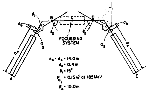
Fig. 6. Layout of hexatron for one superperiod showing location of focussing system.
