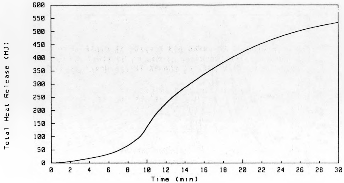
Figure 3.13: Time Integral of the Heat Release Rate (Total Cumulative Heat Release) for the Unaged Rockbestos FIREWALL III Cable Fire Test
