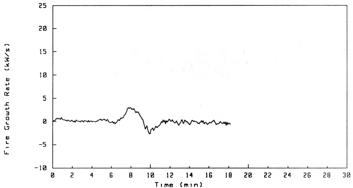
Figure 3.4: Time Rate of Change in the Heat Release Rate (Rate of Fire Intensity Growth or Decline) During the Burning of the Aged BIW Bostrad 7E Cable Product
