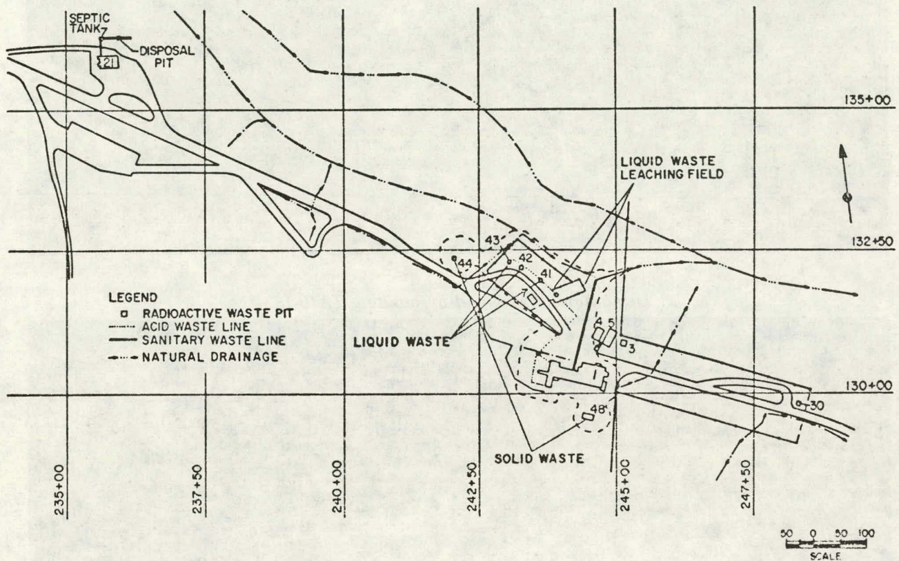
Fig. 8. Waste handling facilities at Bayo Canyon.
