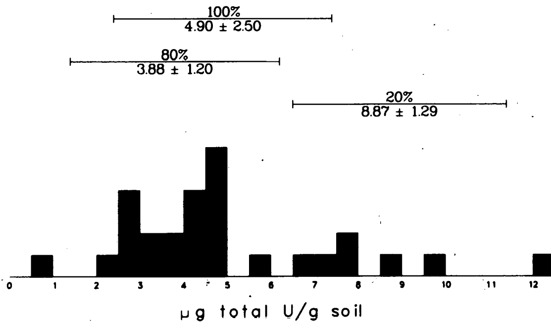
Fig. E-2. Frequency Distribution—Total U in 0-5 cm.
