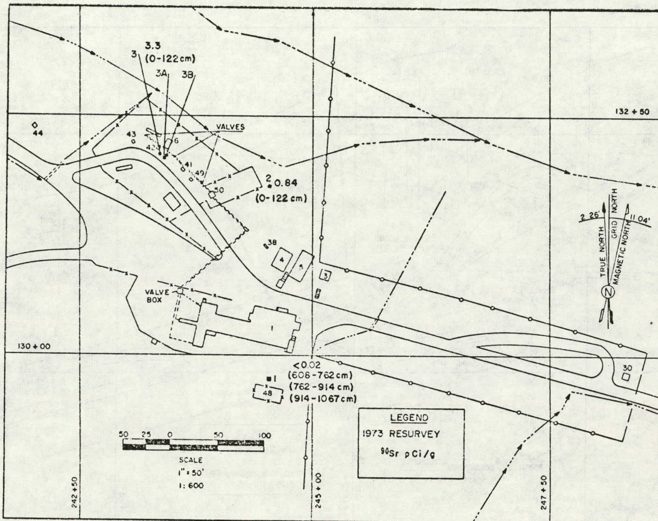
Fig. 16. 90Sr in auger samples; 1973 resurvey effort.
