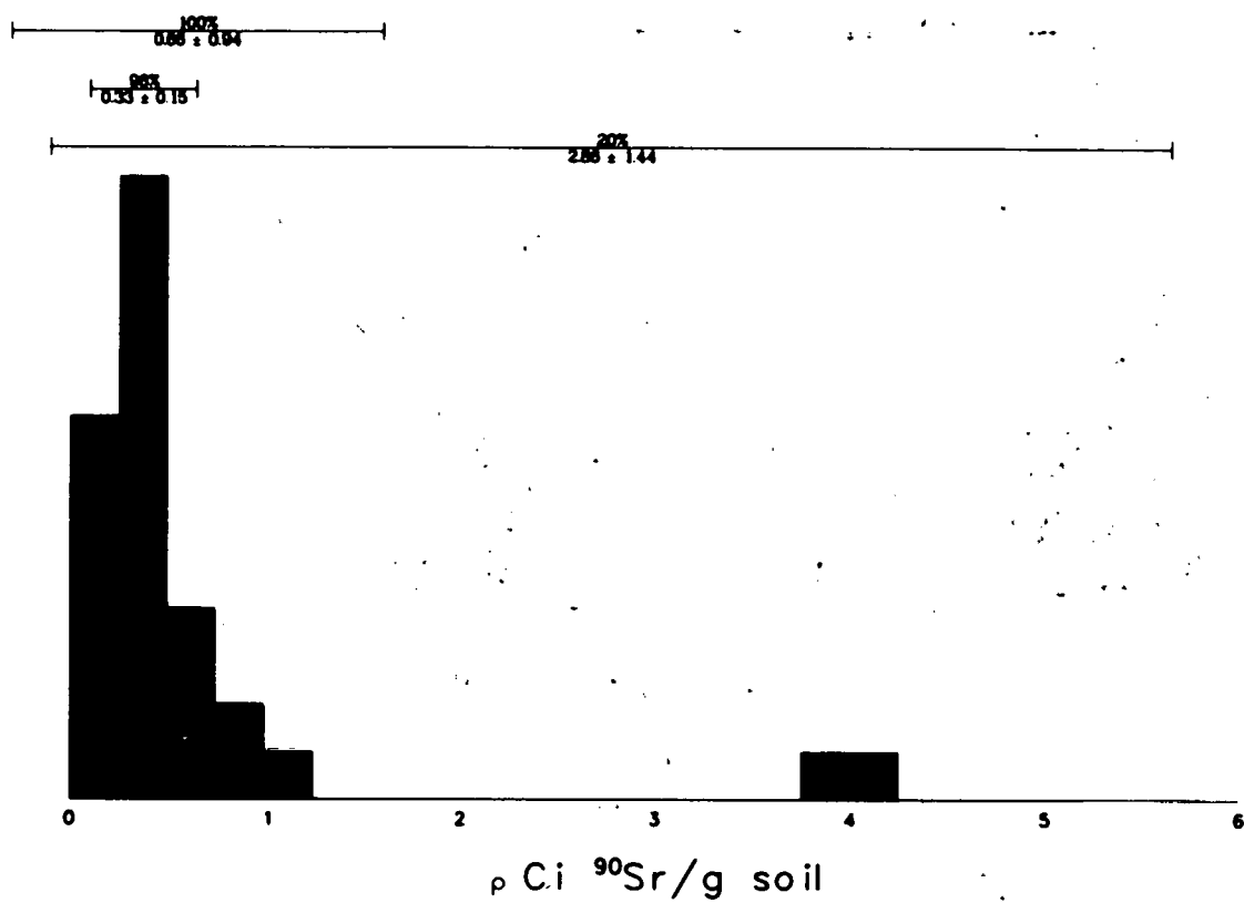
Fig. E-3. Frequency Distribution— 90 Sr in 0-30 cm.
