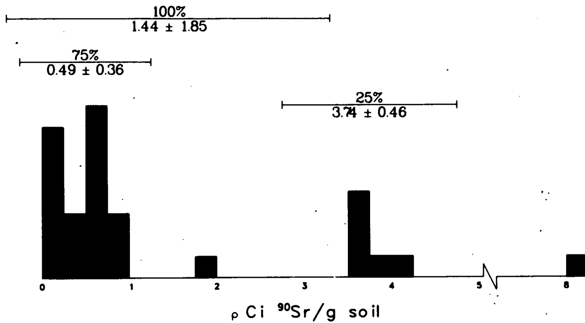
Fig. E-1. Frequency Distribution— ^{90}\text{Sr} in 0-5 cm.
