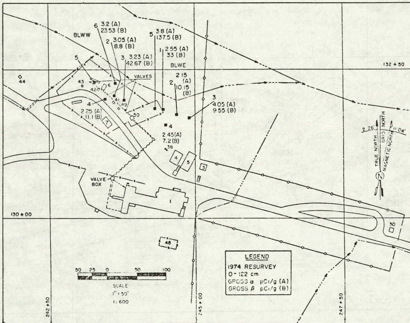
Fig. 17. Gross \alpha - \beta activity in auger samples; 0-122 cm depth; 1974 resurvey effort.
