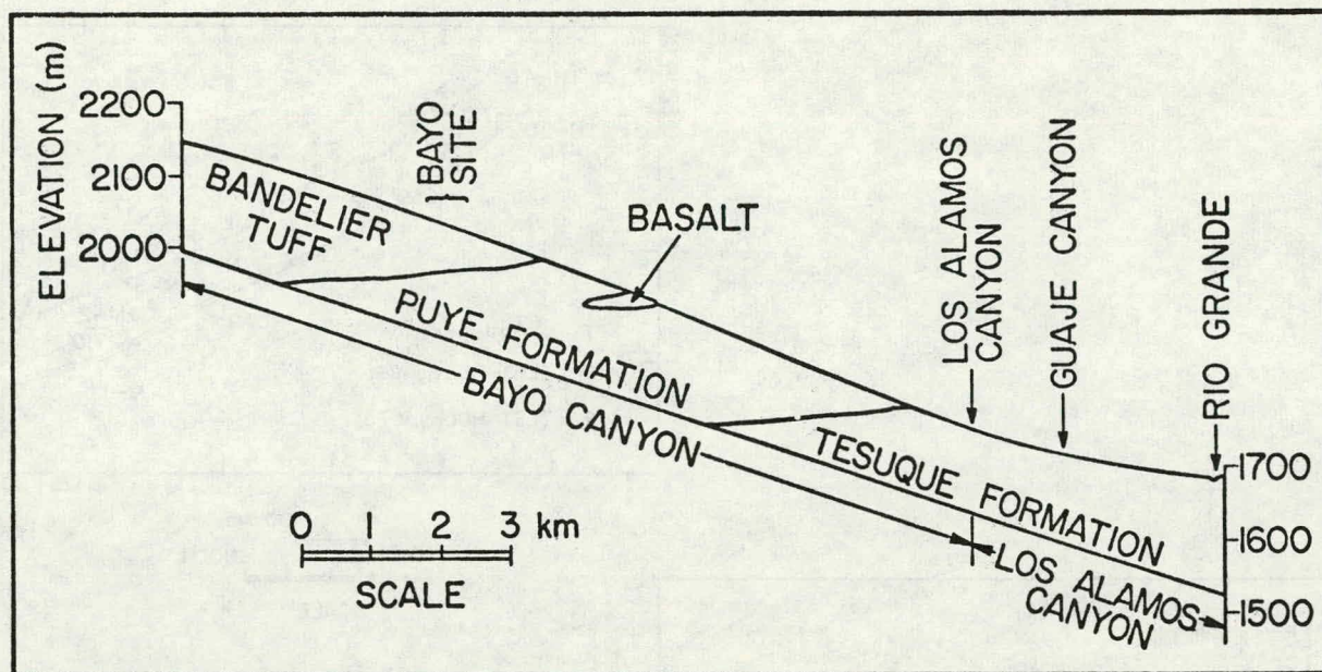
Fig. A-3. Geology underlying alluvium in Bayo and lower Los Alamos Canyons.
