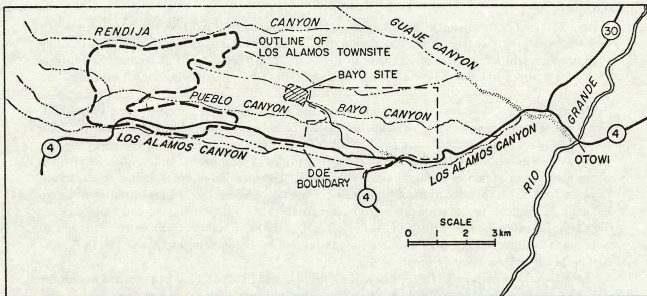
Fig. A-1. Location of Bayo Site relative to Los Alamos townsite.
