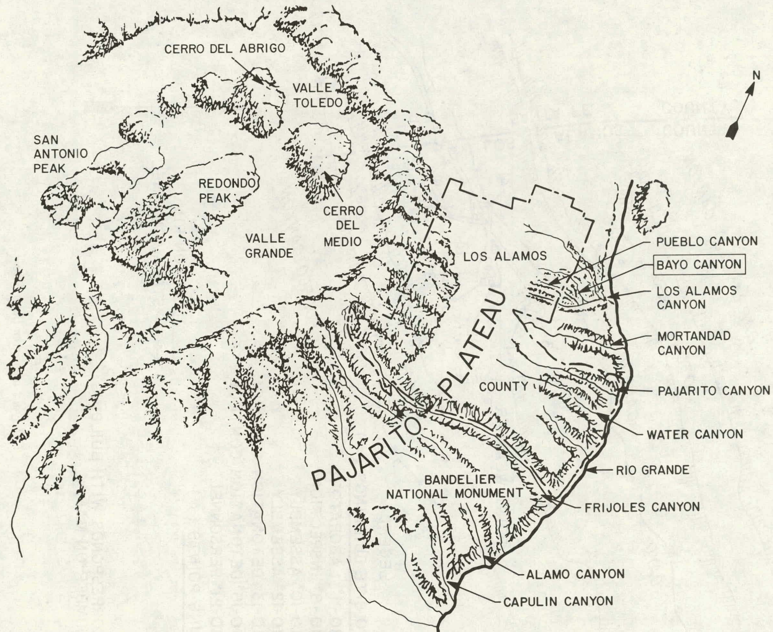
Fig. 2. Physiographic setting of Bayo Canyon.
