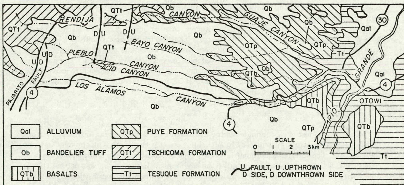
Fig. A-2. Geologic map of the Pajarito Plateau adjacent to Bayo Site.
