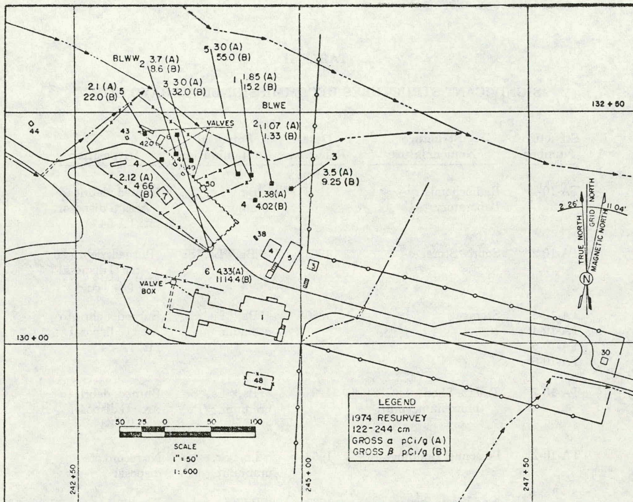
Fig. 18. Gross \alpha - \beta activity in auger samples; 122-124 cm depth; 1974 resurvey effort.
