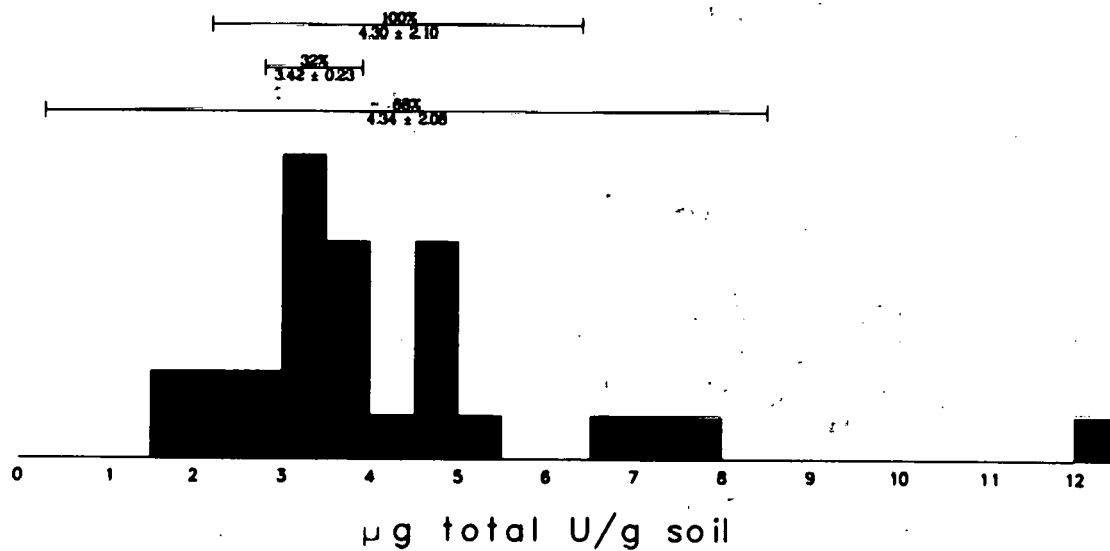
Fig. E-4. Frequency Distribution—Total U in 0-30 cm.
