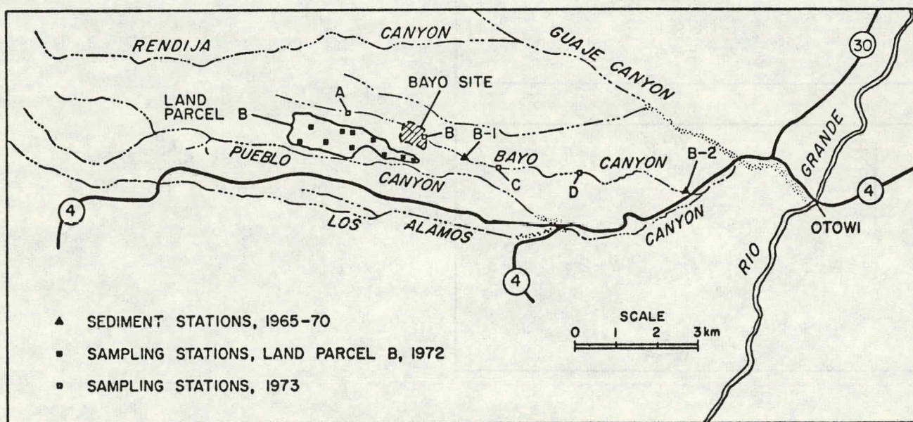
Fig. A-4. Location of sampling station and Land Parcel B in and adjacent to Bayo Canyon.
