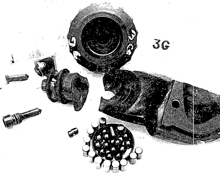
FIGURE 3 MK-II BIT "G", LUG #3 COMPONENTS, INCLUDING BROKEN LUG
