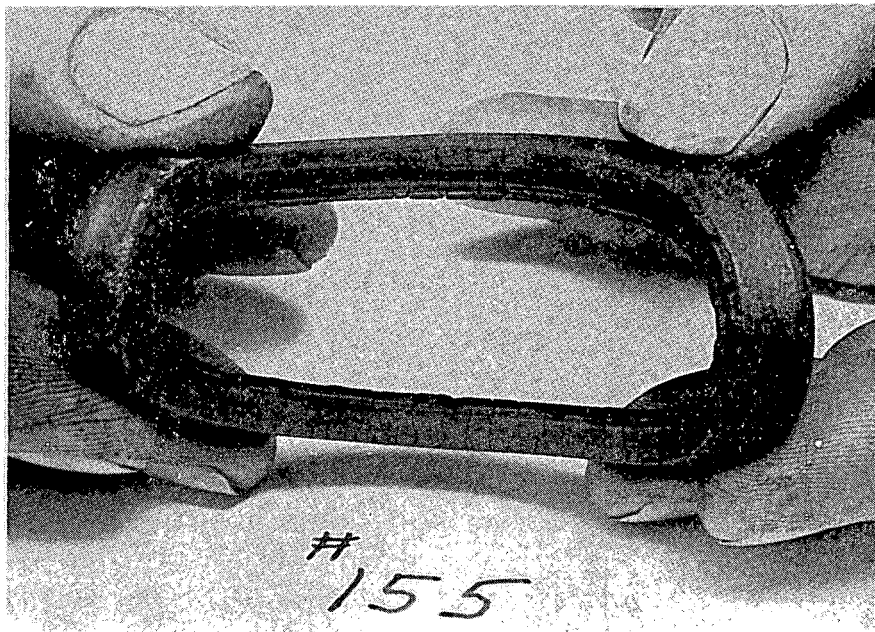
FIGURE 26 VITON SEAL RUN 93 1/2 HOURS WITH ABRASIVES AT 200°C
