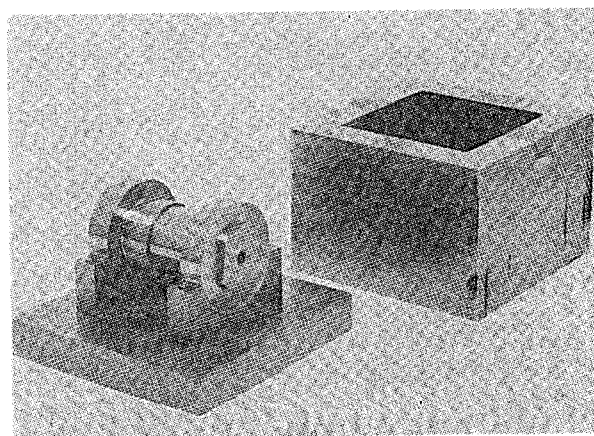
FIGURE 28 - TEST RING IN JOURNAL-BEARING RING-HOLDER, AND PARTIALLY COMPLETED PRESSURE VESSEL
