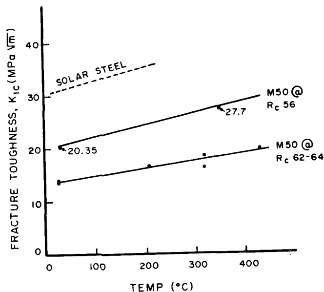
FIGURE 12 FRACTURE TOUGHNESS FOR ROLLER BEARING STEELS
