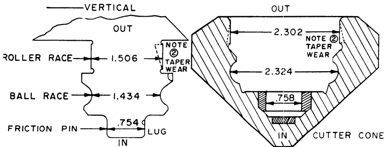
Figure 9 LOCATIONS FOR WEAR MEASUREMENTS OF TABLE 2
