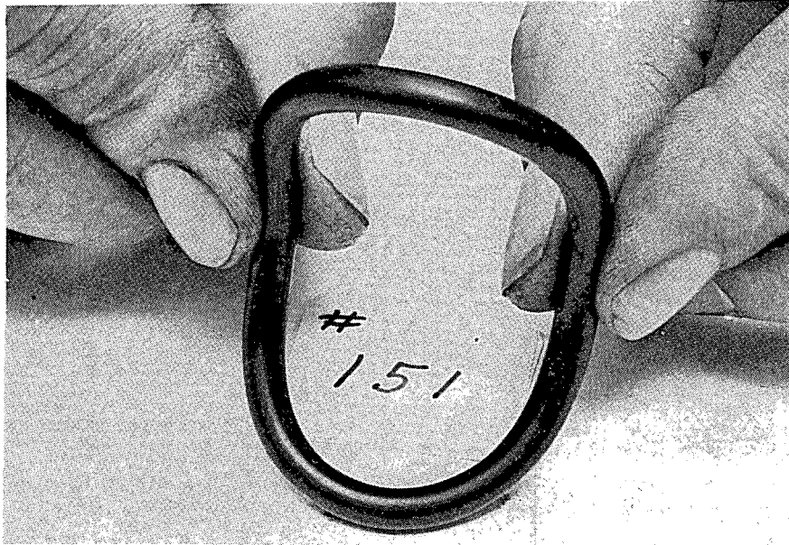
FIGURE 22 KALREZ O-RING, SHOWING COMPRESSION-SET AFTER 32 HRS AT 125°C
