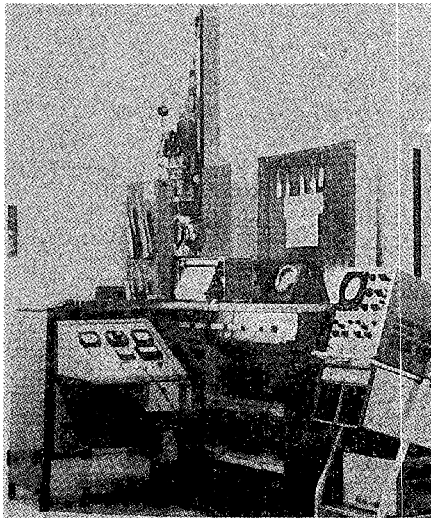
FIGURE 16 SEAL TEST FACILITY
