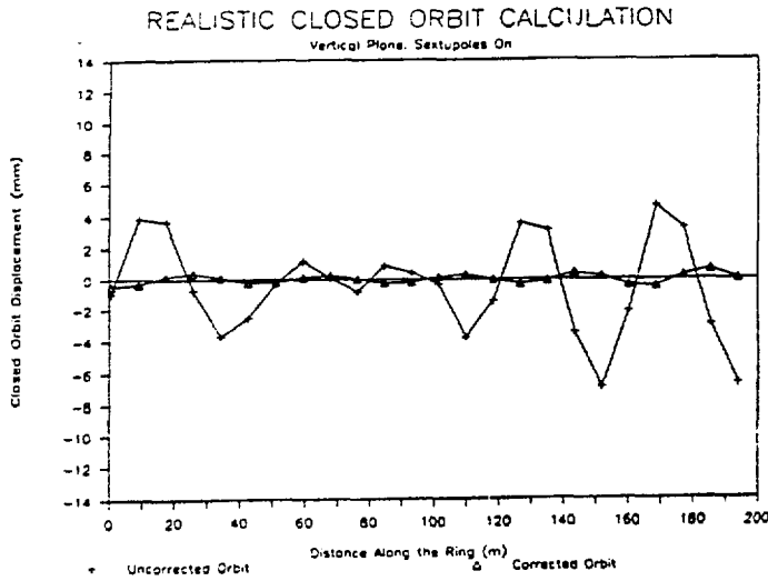
Fig. 1. Horizontal incorrected (+) and corrected ( \Delta ) closed orbits for realistic error distribution.
