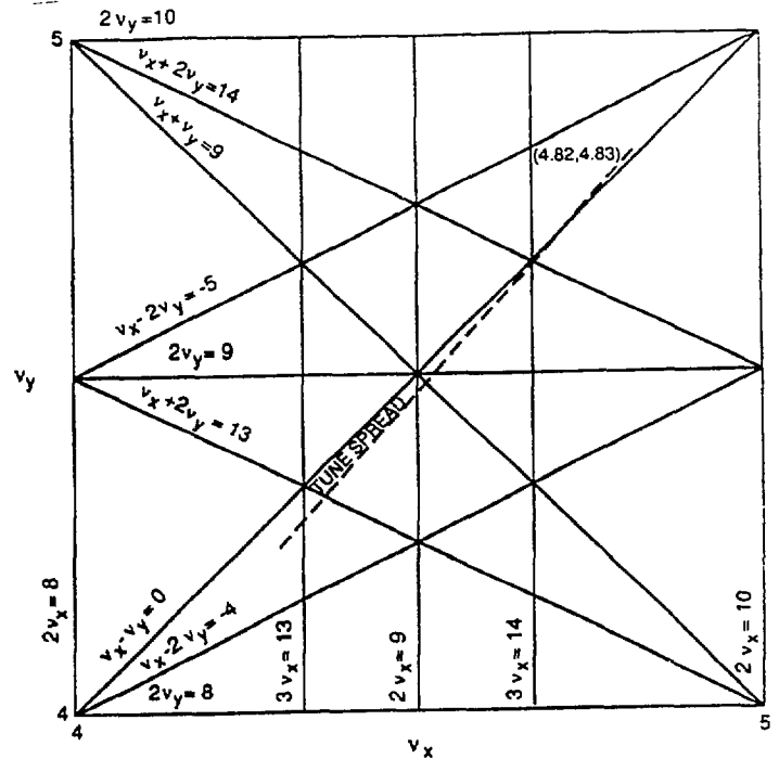
Fig. 3. The tune diagram with the expected tune spread due to space charge.
