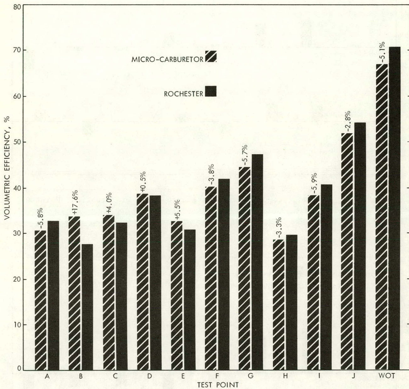
Figure 3-10. Volumetric Efficiency
