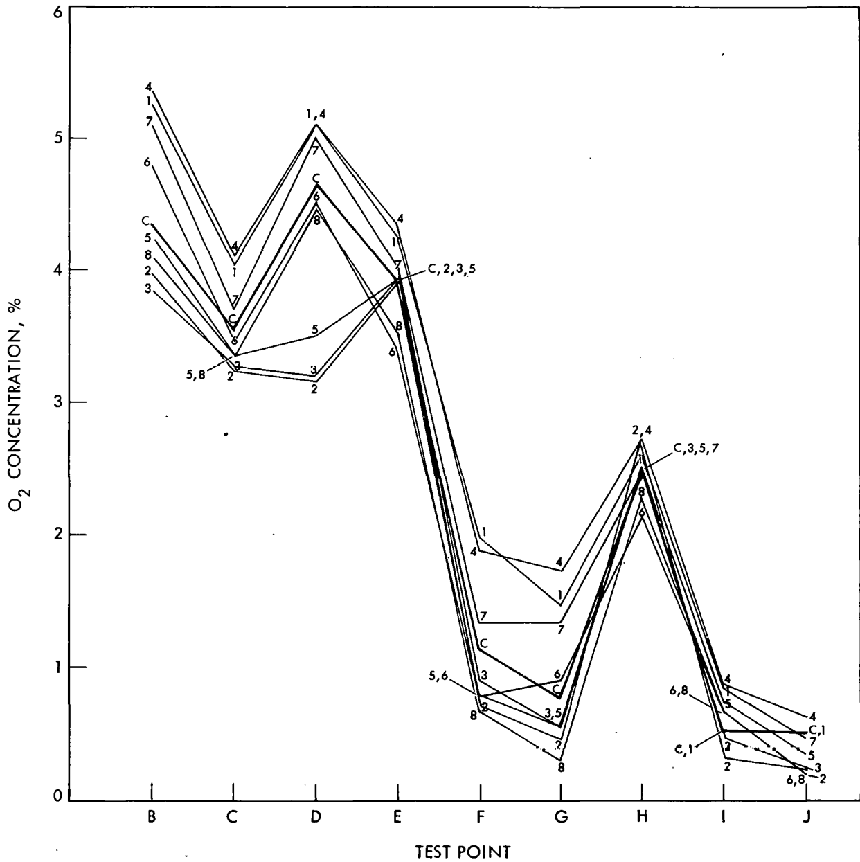
Figure B-10. Cylinder-to-Cylinder O 2 Distribution, Micro-Carburetor
