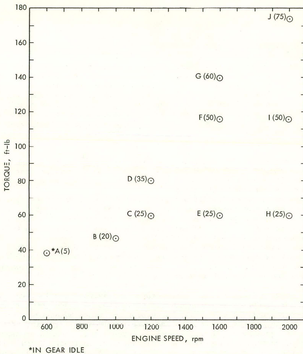
Figure 3-1. Constant Speed/Load Test Points, ft-lb. Brake Mean Effective Pressure (psi) in Parentheses
