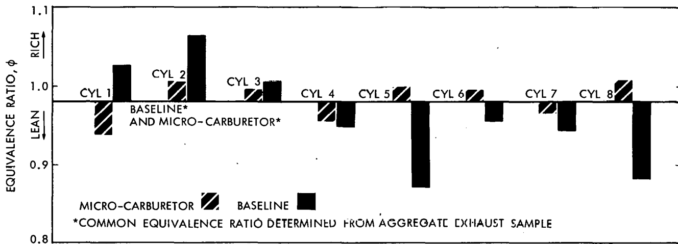
Figure 3-11e. Cylinder-to-Cylinder Equivalence Ratio Distribution, Point F
