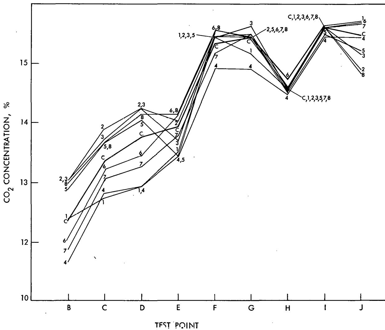
Figure B-6. Cylinder-to-Cylinder CO 2 Distribution, Micro-Carburetor
