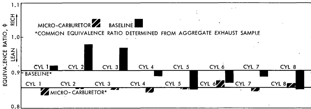
Figure 3-11d. Cylinder-to-Cylinder Equivalence Ratio Distribution, Point E
