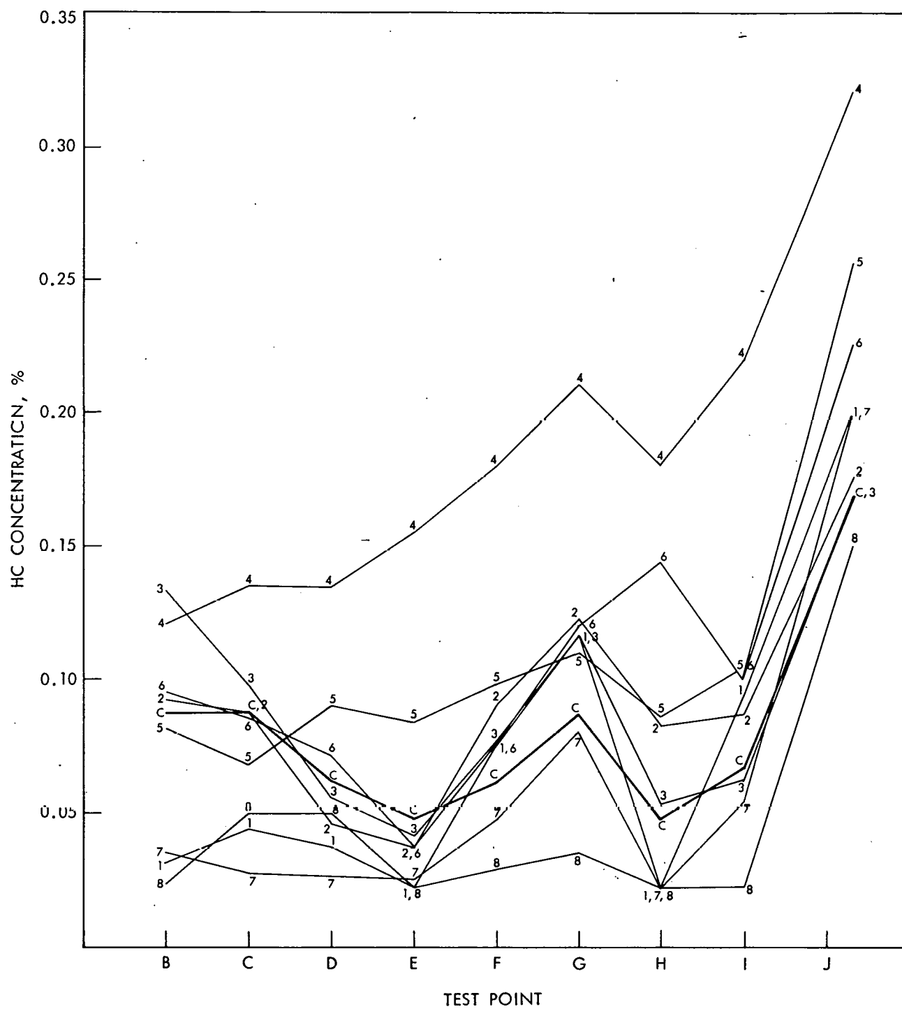
Figure B-2. Cylinder-to-Cylinder HC Distribution, Baseline
