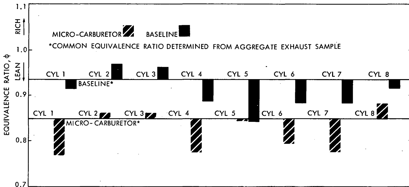
Figure 3-11c. Cylinder-to-Cylinder Equivalence Ratio Distribution, Point D
