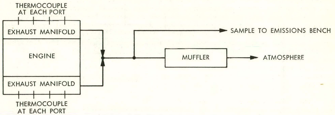
Figure 3-3. Engine Dynamometer Exhaust Plumbing - Aggregate Emissions Sampling
