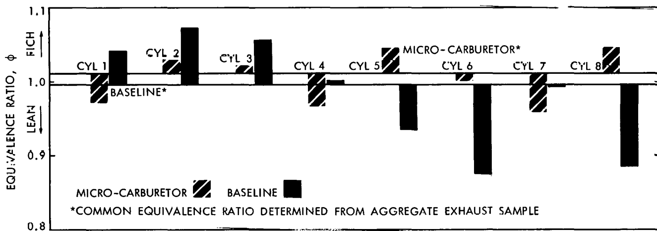
Figure 3-11f. Cylinder-to-Cylinder Equivalence Ratio Distribution, Point G
