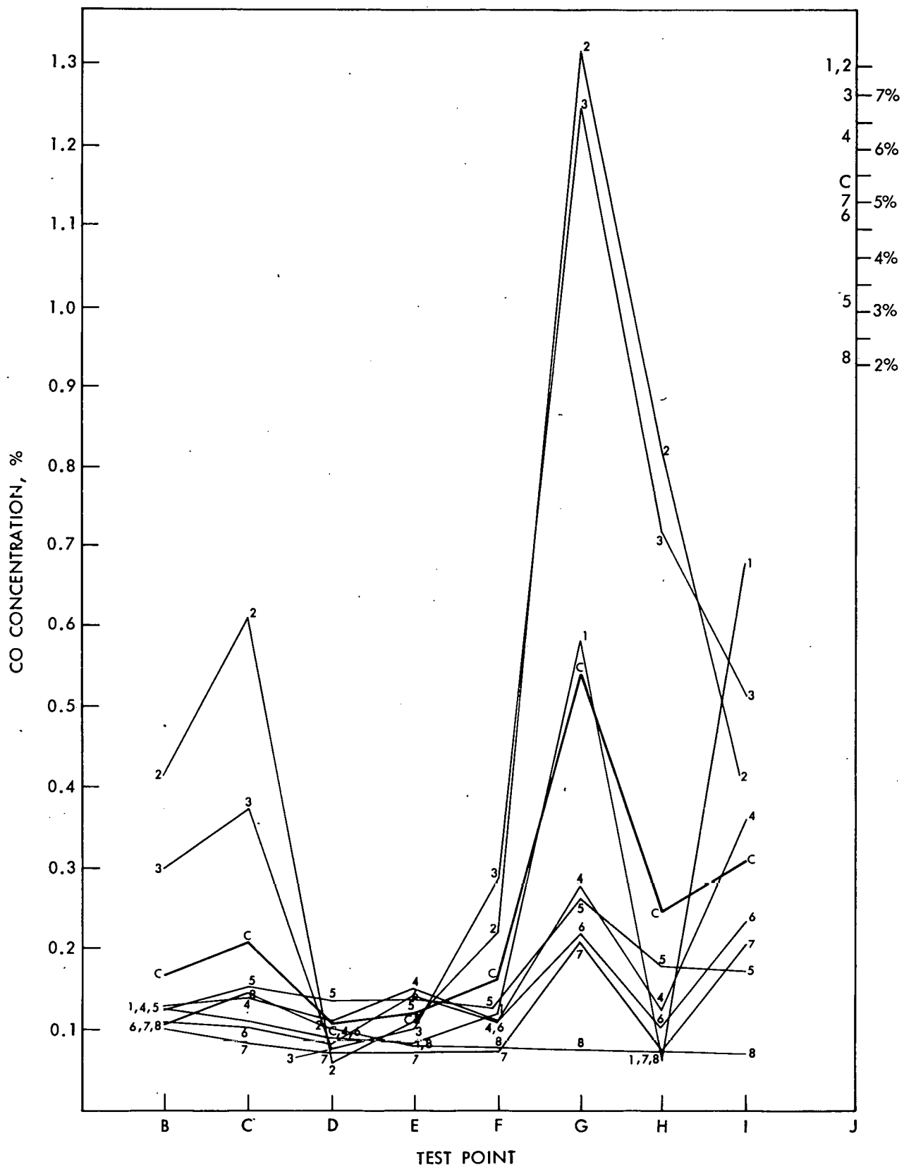
Figure B-4. Cylinder-to-Cylinder CO Distribution, Baseline
