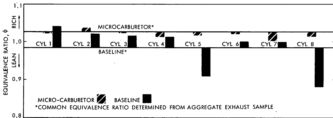
Figure 3-11h. Cylinder-to-Cylinder Equivalence Ratio Distribution, Point I
