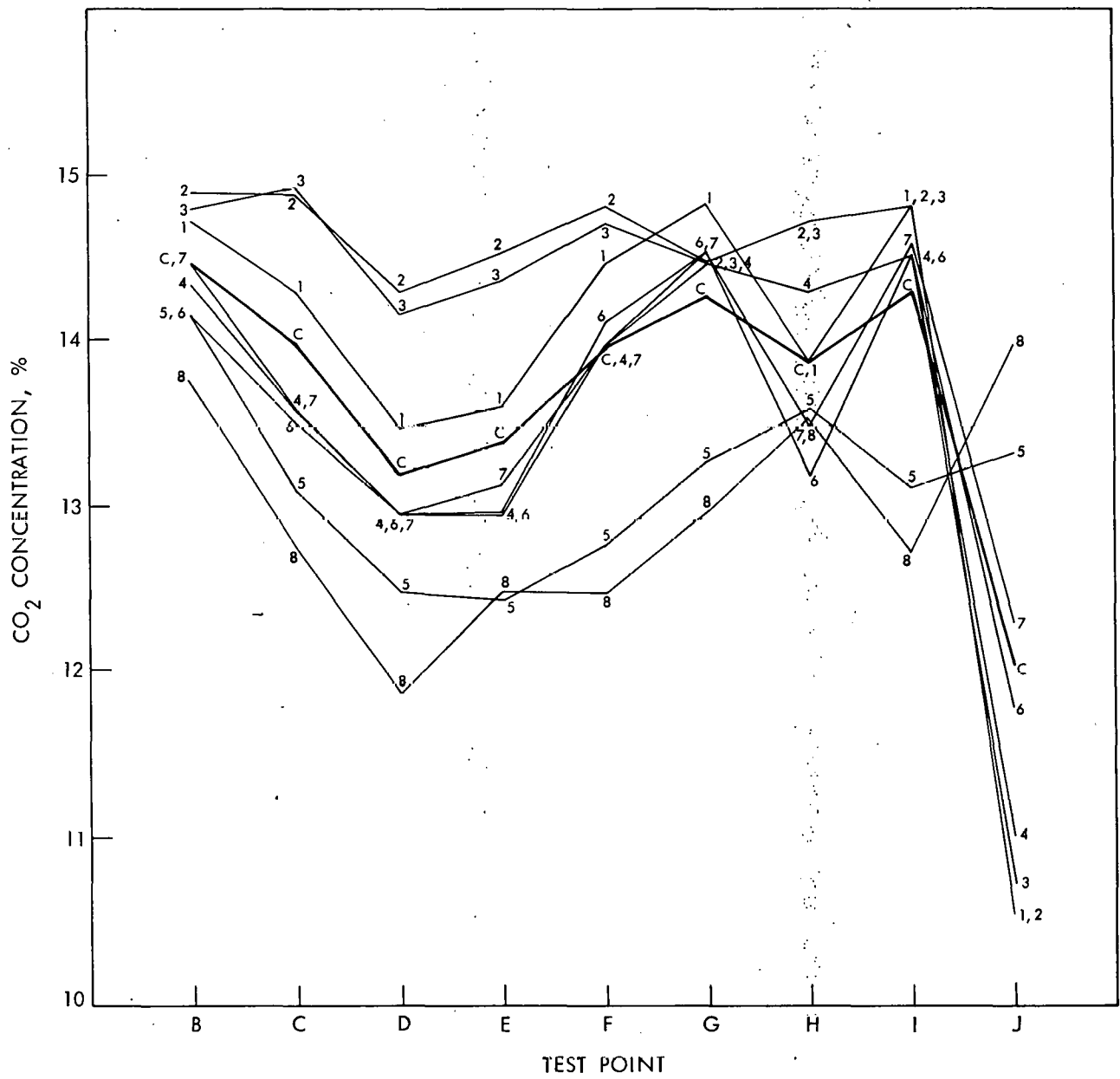
Figure B-1. Cylinder-to-Cylinder CO 2 Distribution, Baseline
