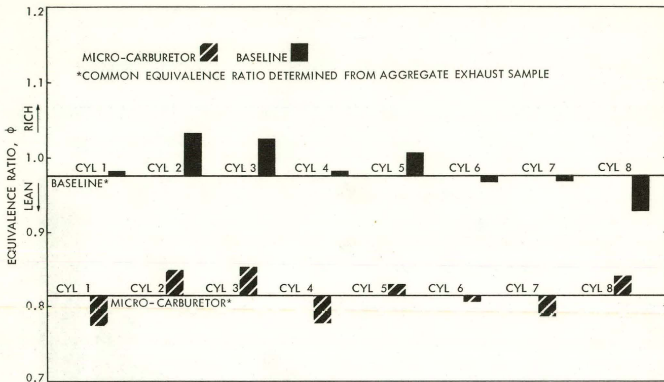
Figure 3-11a. Cylinder-to-Cylinder Equivalence Ratio Distribution, Point B
