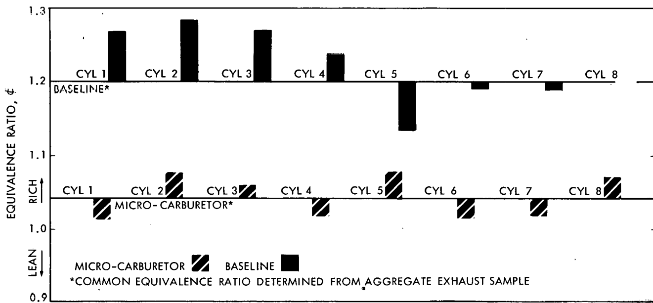
Figure 3-11i. Cylinder-to-Cylinder Equivalence Ratio Distribution, Point J
