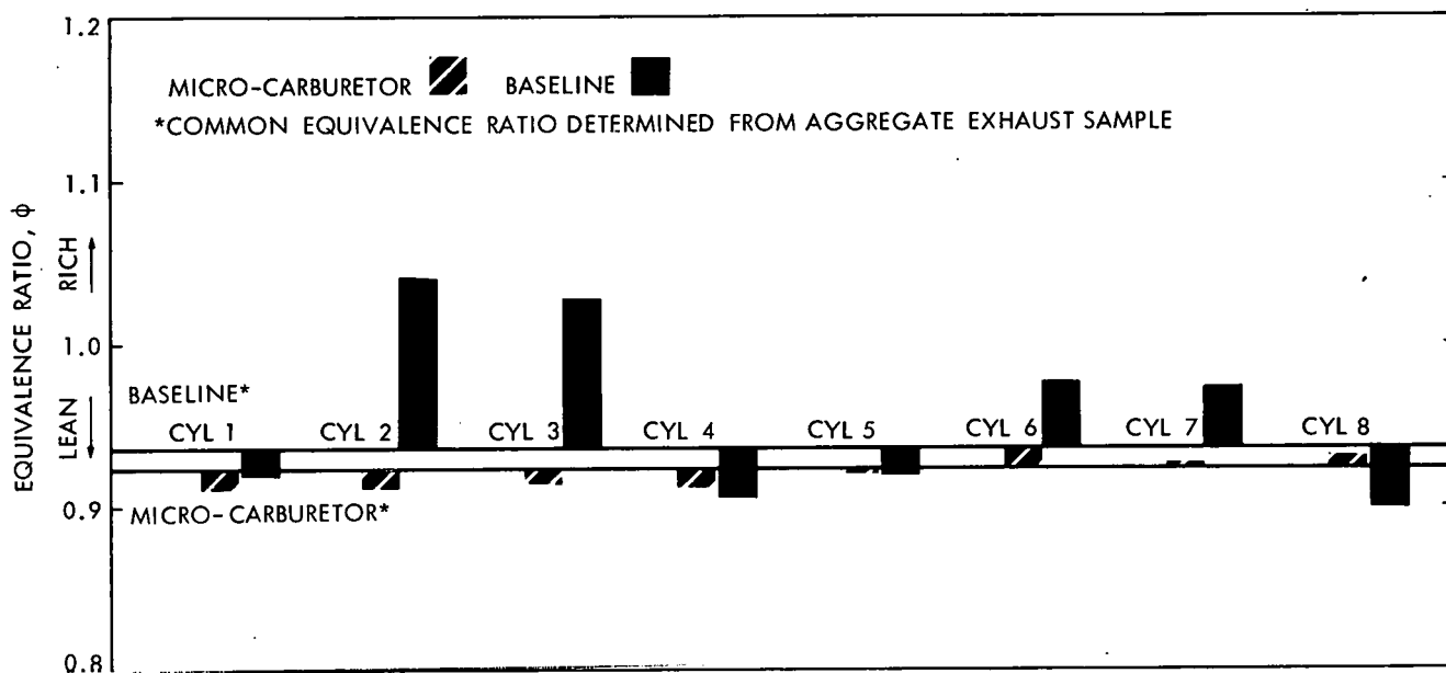
Figure 3-11g. Cylinder-to-Cylinder Equivalence Ratio Distribution, Point H
