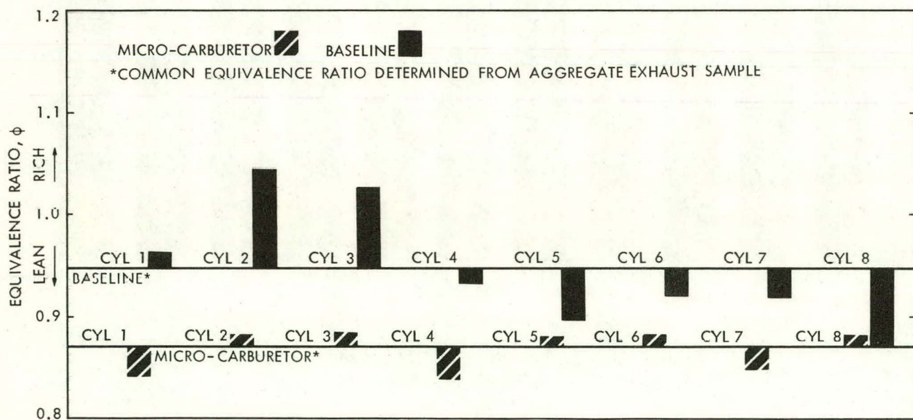
Figure 3-11b. Cylinder-to-Cylinder Equivalence Ratio Distribution, Point C
