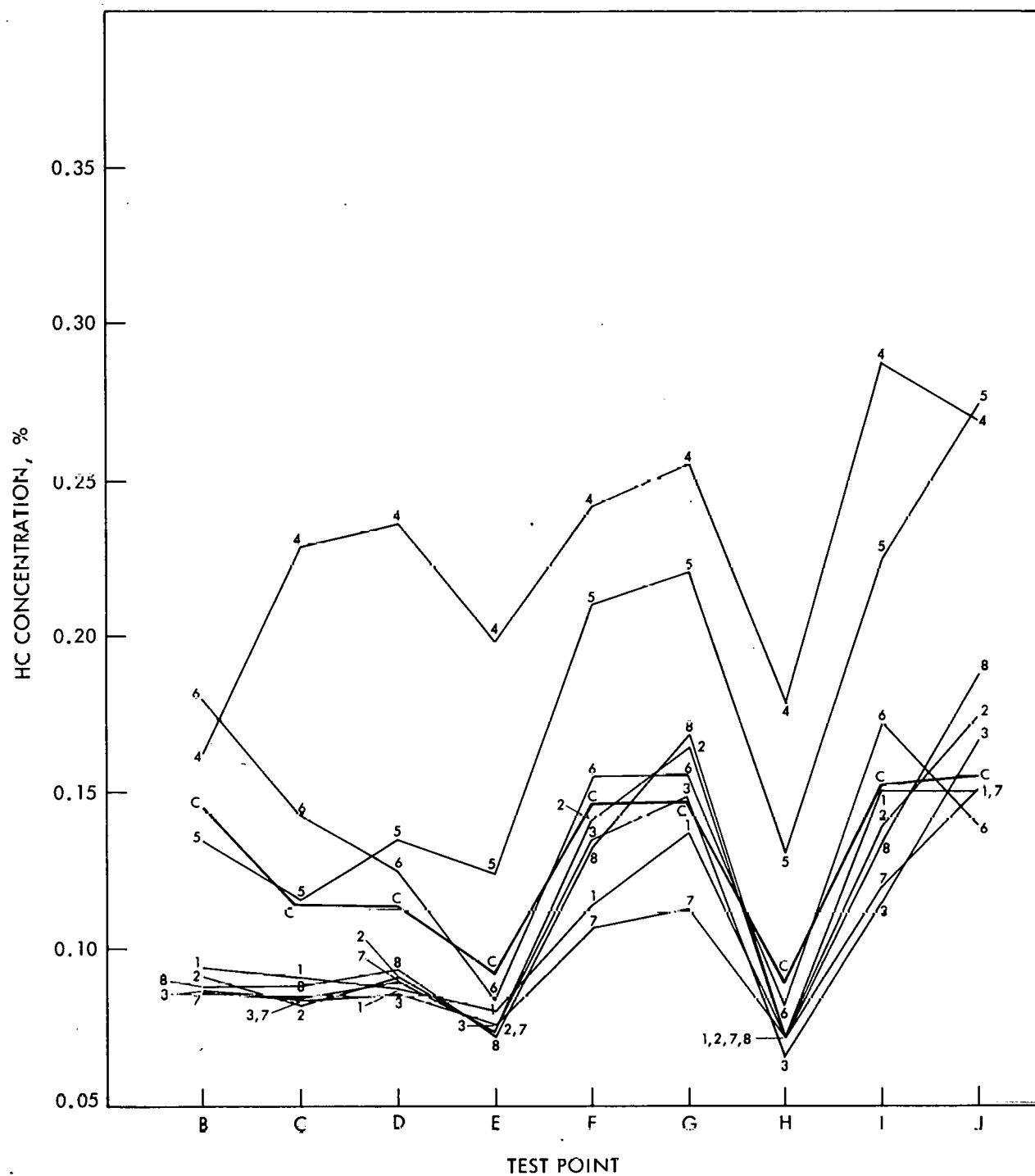
Figure B-7. Cylinder-to-Cylinder HC Distribution, Micro-Carburetor
