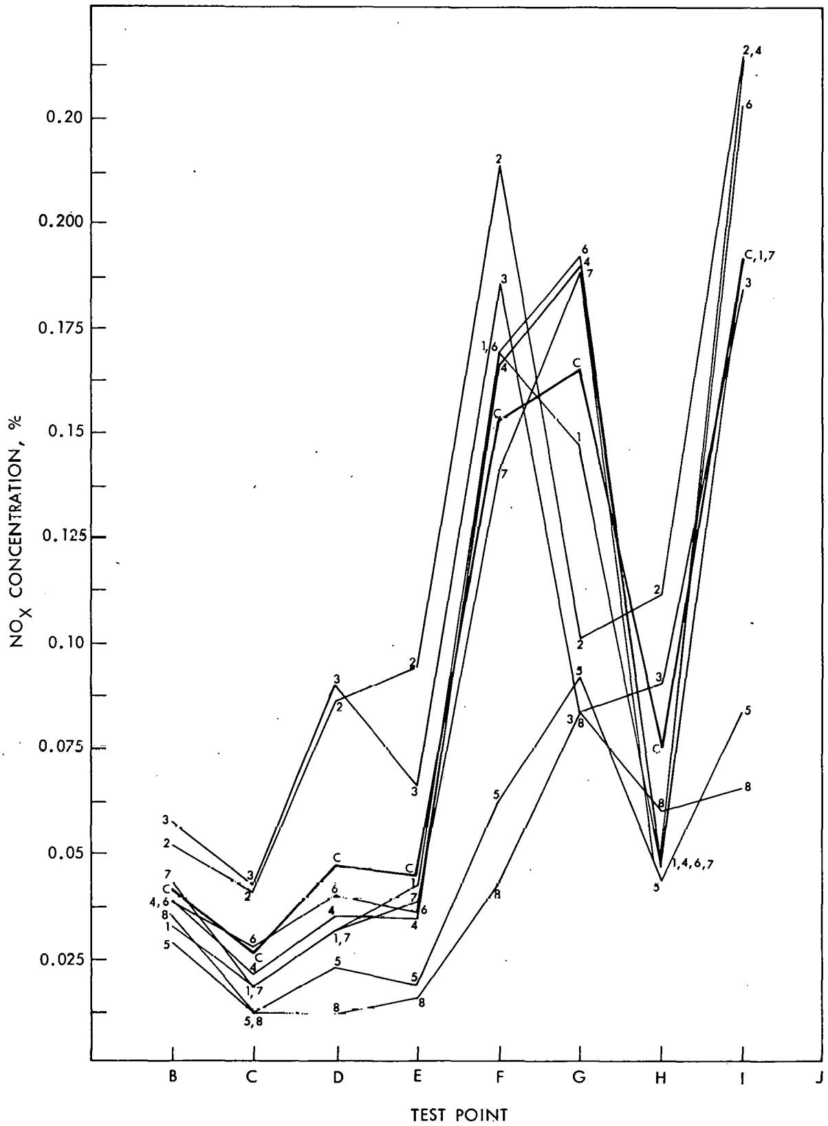
Figure B-3. Cylinder-to-Cylinder NO x Distribution, Baseline
