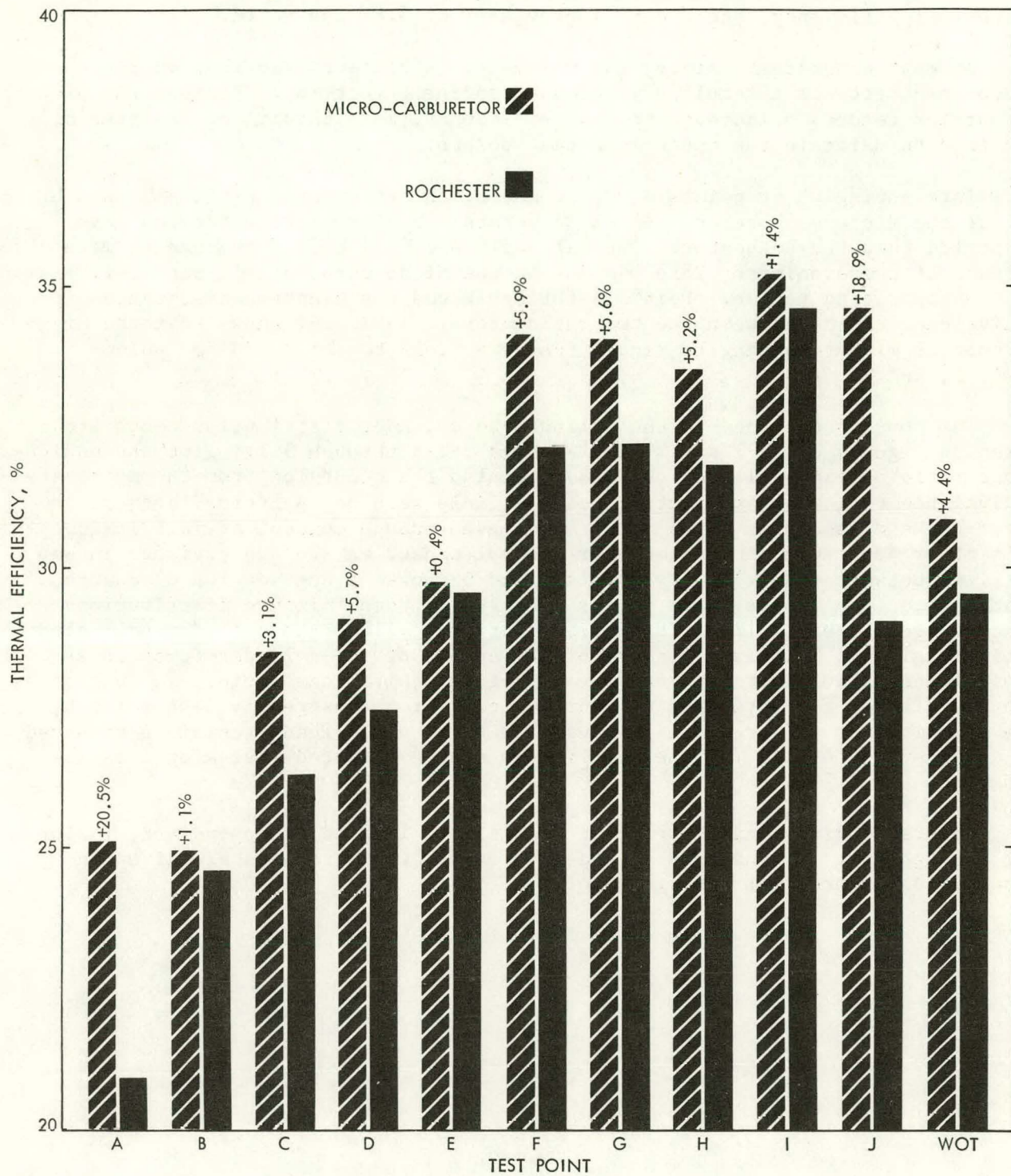
Figure 3-9. Thermal Efficiency
