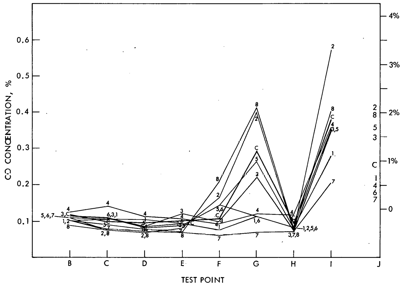
Figure B-9. Cylinder-to-Cylinder CO Distribution, Micro-Carburetor
