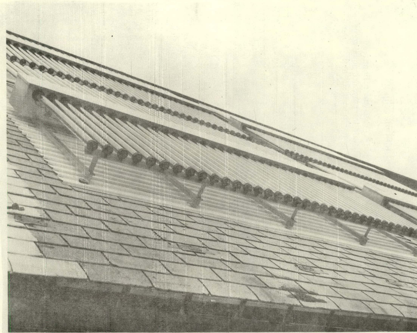
Figure 7. Collector array reflective backing. White vinyl siding used on MSFC Solar Demonstration Facility, Huntsville, Alabama.
