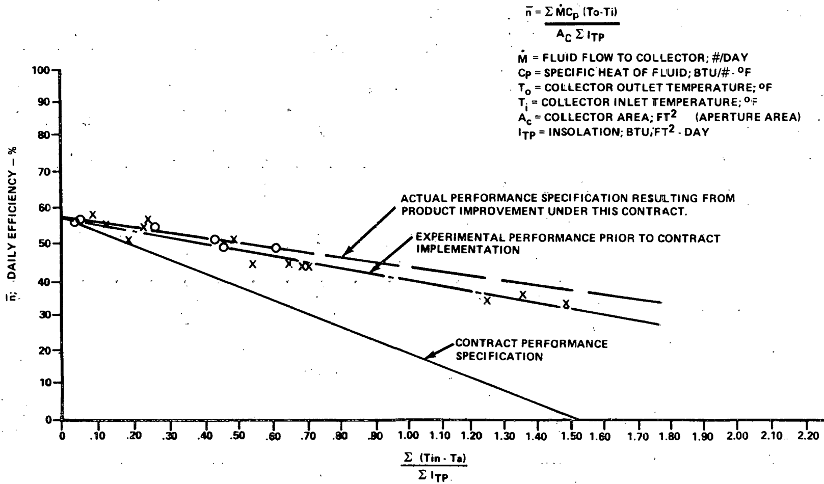
Figure 10. Model SEC-601 collector efficiency.
