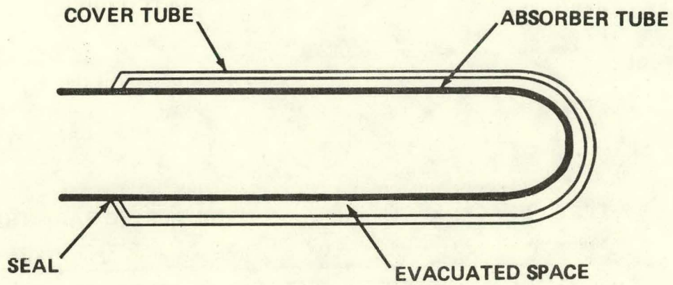
Figure 3. Evacuated tubular solar collector.
