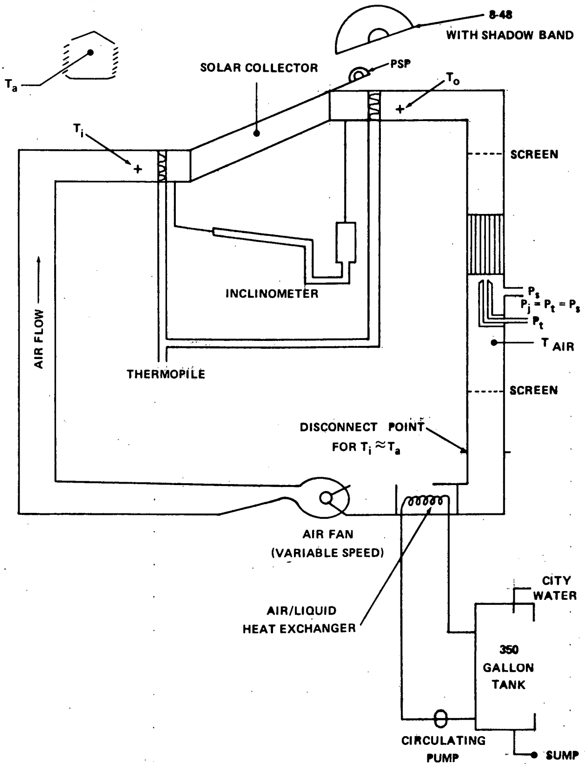
Figure 9. Test loop schematic model SEC-601 air-cooled collector.
