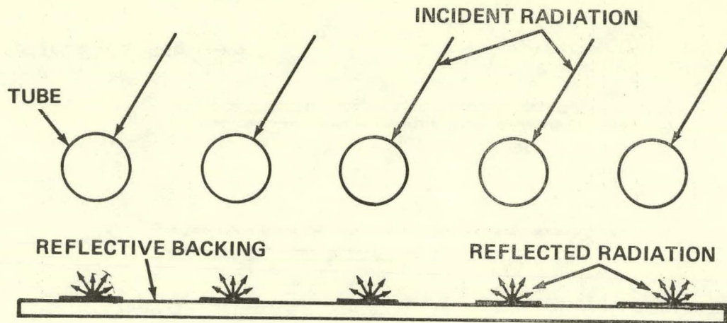
Figure 6. Collector array radiation interception.
