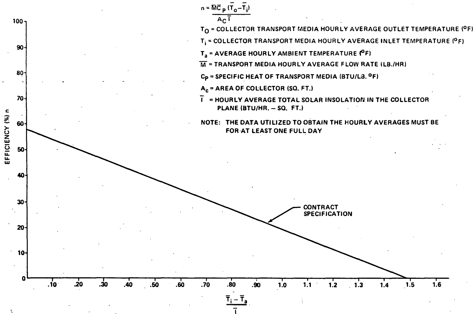
Figure 8. Efficiency as a function of operating conditions, performance must be above line.
