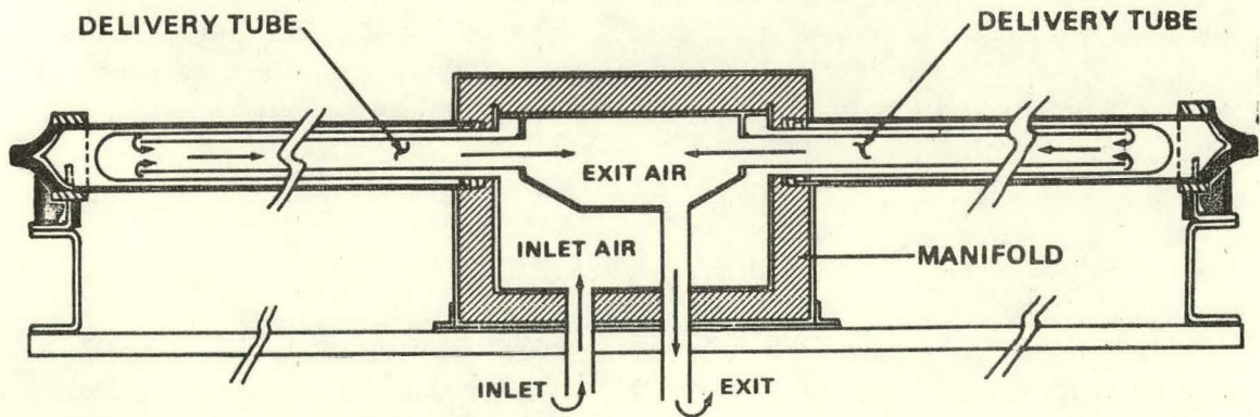
Figure 5. Collector pair and manifold.
