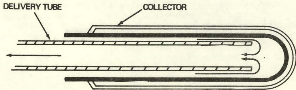
Figure 4. Delivery tube with evacuated tubular collector.
