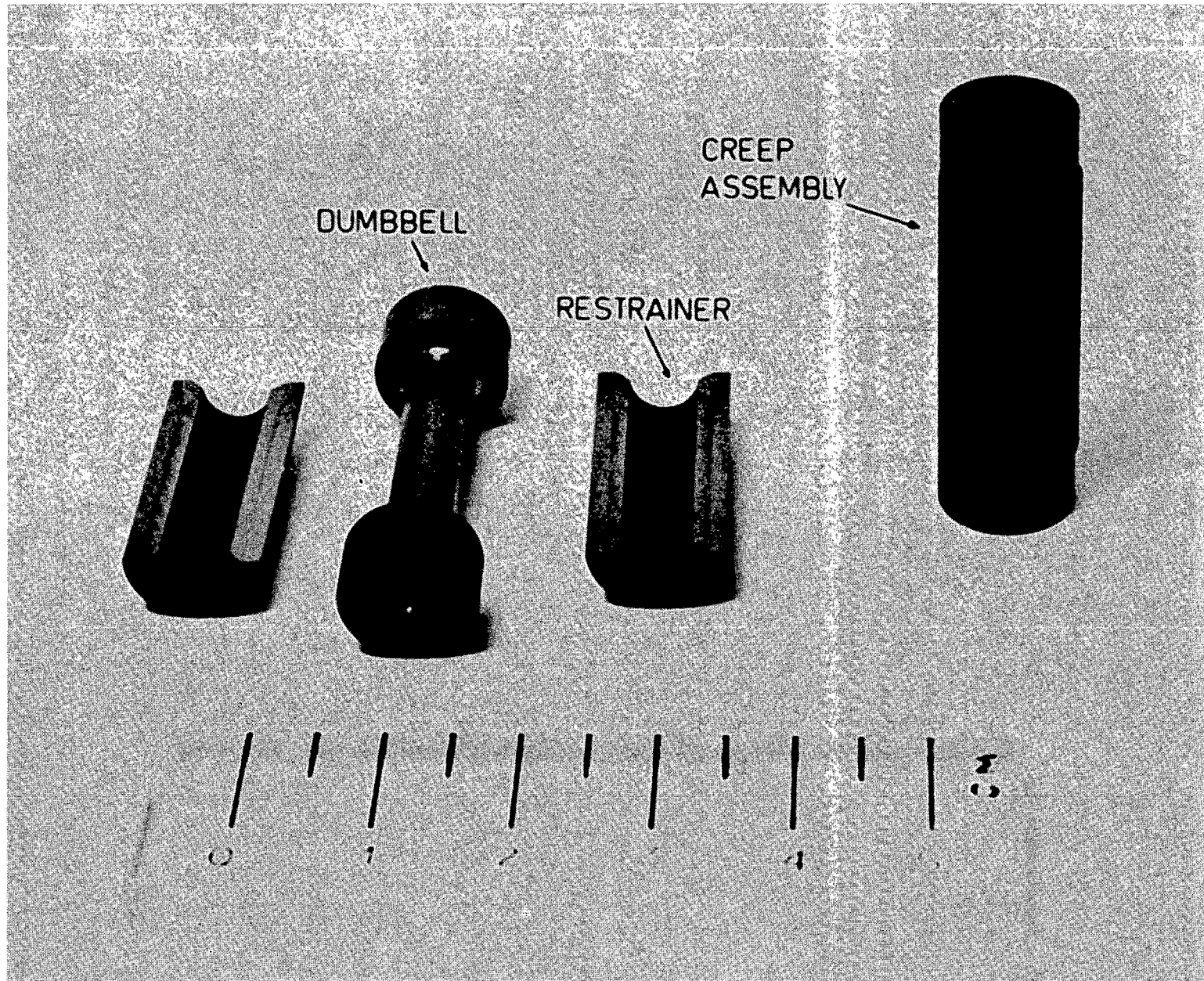
Fig. 2. Creep specimen and restraining pads for restrained shrinkage tests (from Ref. 12)
