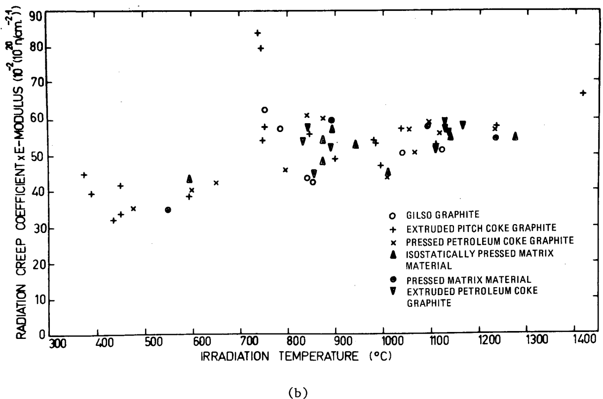
Fig. 15. Steady-state irradiation creep data from restrained shrinkage tests: (a) creep coefficient as a function of temperature; (b) creep coefficient multiplied by initial Young's modulus as a function of temperature (from Ref. 12)
