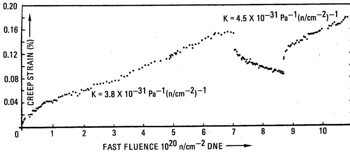
Fig. 12. Creep strain record of experiment D-166-01 at 850°C with tensile stress of 6 MPa (from Ref. 22)
