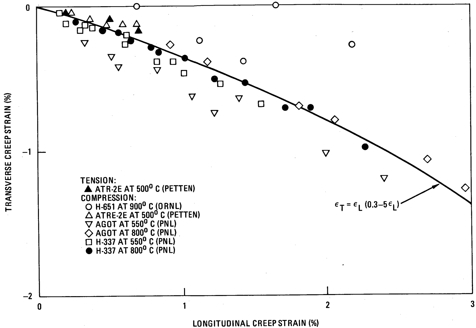
Fig. 19. Composite plot of transverse creep strain as a function of longitudinal creep strain
