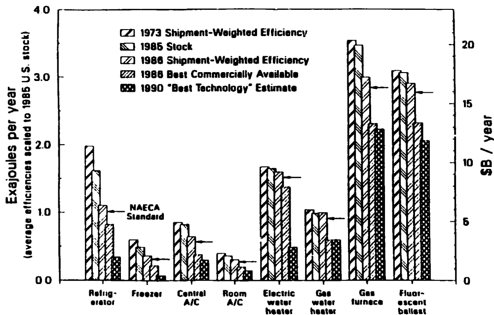
Figure 1. Trends in U.S. Appliance Efficiency
