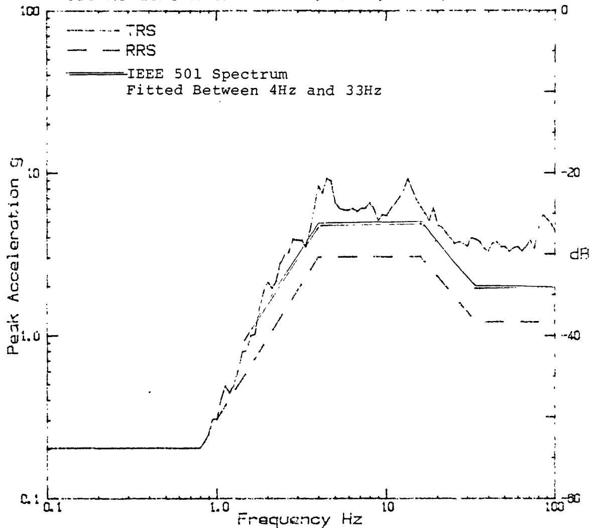
RESPONSE SPECTRUM
