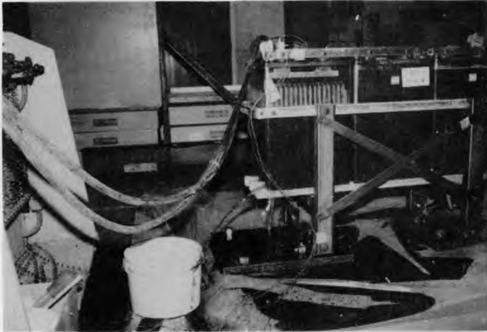
FIGURE 3 Case Failure After High-Level Shaking
