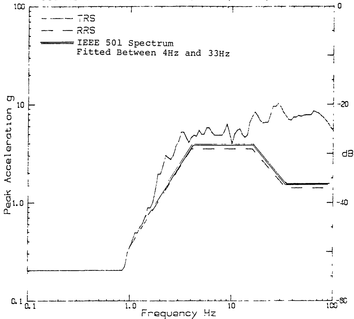
RESPONSE SPECTRUM
