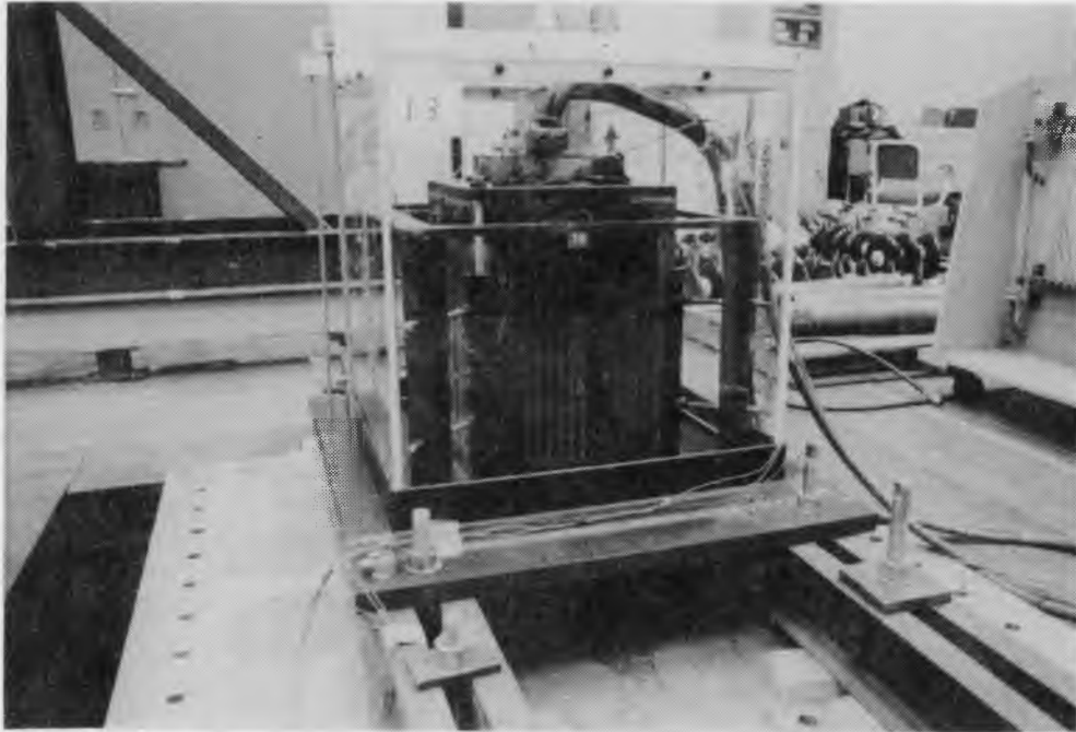
FIGURE 1 Single Cell Test Rig
