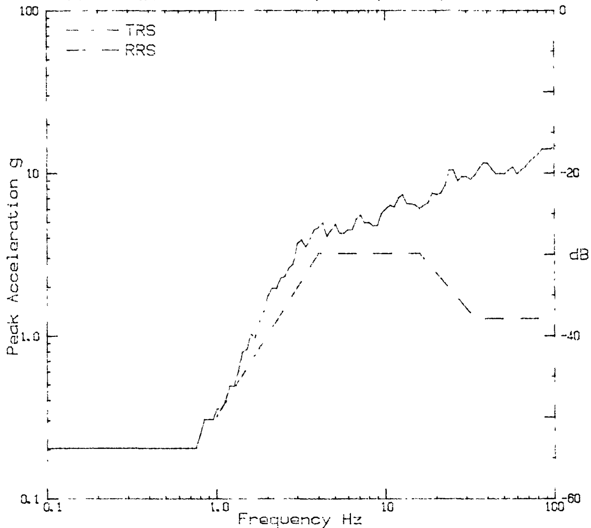
RESPONSE SPECTRUM
