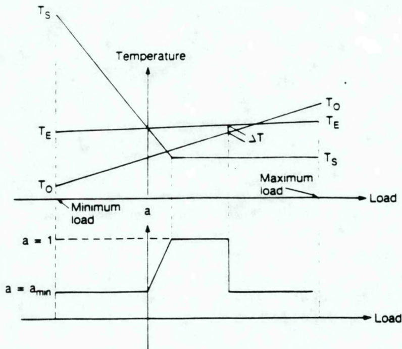
Figure 5. Control strategy of economizer cycle. Outdoor air ratio "a" ( Q_o/Q_a ) depends on the temperatures in the system and preset temperature difference \Delta T between outdoor air and exhaust air. Its minimum value a_{min} depends on minimum outdoor air flow rate. T_E = exhaust temperature, T_S = supply temperature, T_O = outdoor air temperature.
