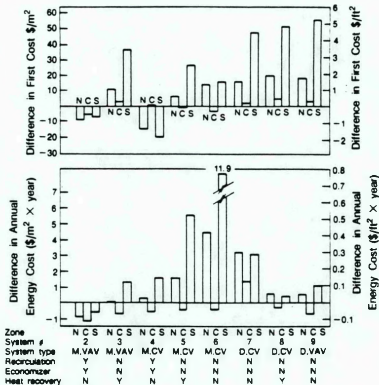
Figure 11. Comparison of first cost and annual energy cost of Systems 2 - 9 to the same costs for System 1 in the Minneapolis climate. The assumed costs of electricity and natural gas are 5.7 cents/ kWh and 1.3 cents/kWh, respectively.
