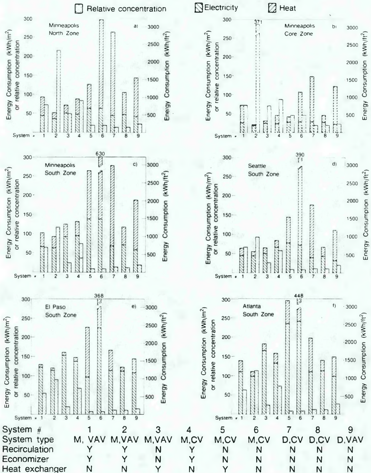
Figure 9. Energy consumption and relative pollutant concentrations for different air conditioning and air distribution systems. The design minimum outside air supply is 20 cfm (10 L/s) per occupant for all systems except No. 2, in which the outside air flow is 15% of the supply air flow. M = mixing system, D = displacement system, VAV = variable air volume, CV = constant volume.
