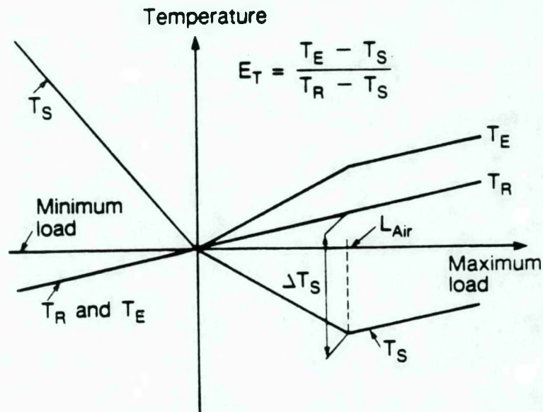
Figure 2. Control strategy of displacement ventilation with constant air flow. E_T = temperature efficiency. L_{AIR} = maximum cooling by air, \Delta T_S = maximum temperature difference between room and supply air, T_E = exhaust temperature, T_S = supply temperature, T_R = room temperature at height 2.6 ft (0.8 m)
