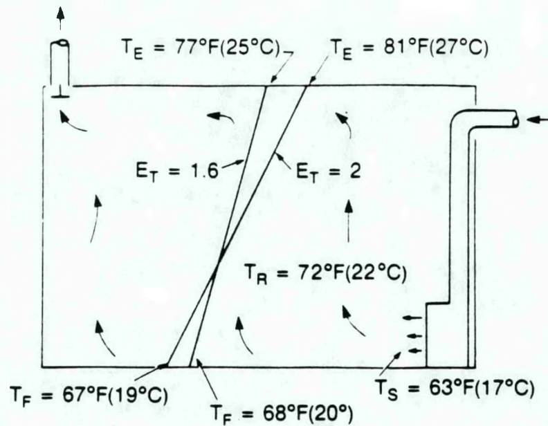
Figure 1. Illustration of layout, flow patterns, and temperature profile with displacement ventilation. T_E = exhaust air temperature, T_S = supply air temperature, T_R = room temperature, T_F = air temperature close to floor, E_T = temperature efficiency.
