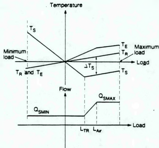
Figure 6. Control strategy of displacement ventilation system with variable air flow and terminal reheats. L_{TR} = the cooling load which still can be met with minimum supply air flow, L_{AIR} = maximum cooling by air, Q_{SMIN} = minimum supply air flow, Q_{SMAX} = maximum supply air flow \Delta T_S = maximum temperature difference between room and supply air, T_E = exhaust temperature, T_S = supply temperature, T_R = room temperature at height 2.6 ft (0.8 m).
