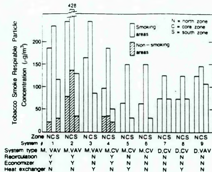
Figure 10. Predicted tobacco smoke respirable particle concentrations in smoking and nonsmoking areas in Minneapolis. Systems Number 3 and Numbers 5 - 9 do not recirculate air; therefore, the predicted concentration in the nonsmoking areas is zero. M = mixing system, D = displacement system, VAV = variable air volume, CV constant volume.
