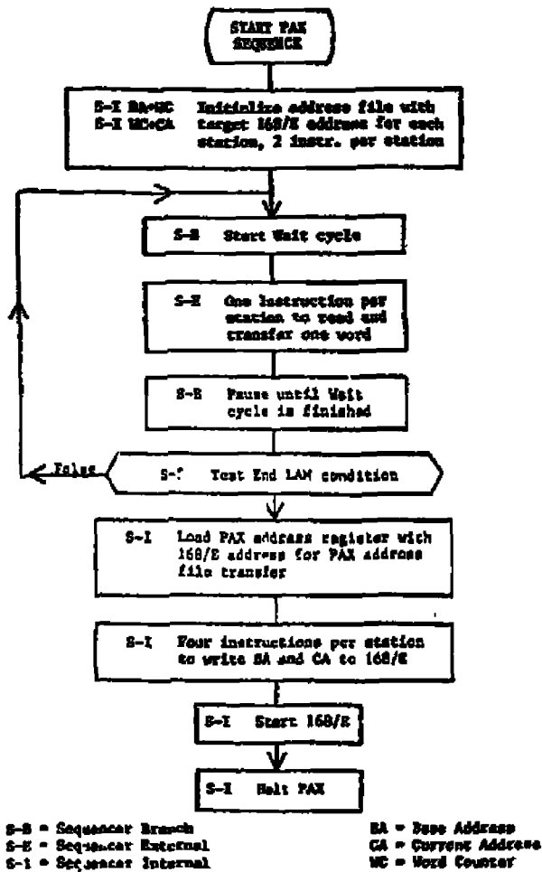
Fig. 5. Flowchart for a PAX read sequence.
