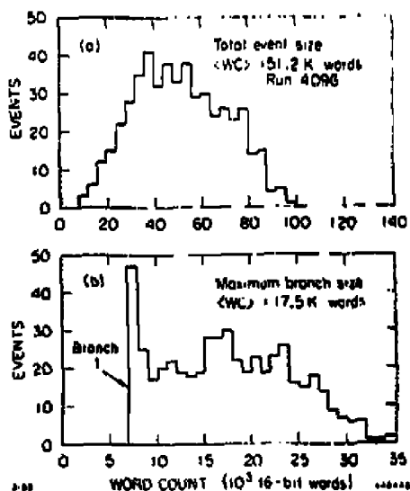
Fig. 1. UA1 event sizes.
