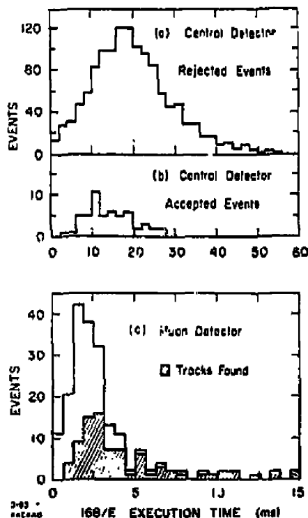
Fig. 8. 168/E algorithm execution time.
