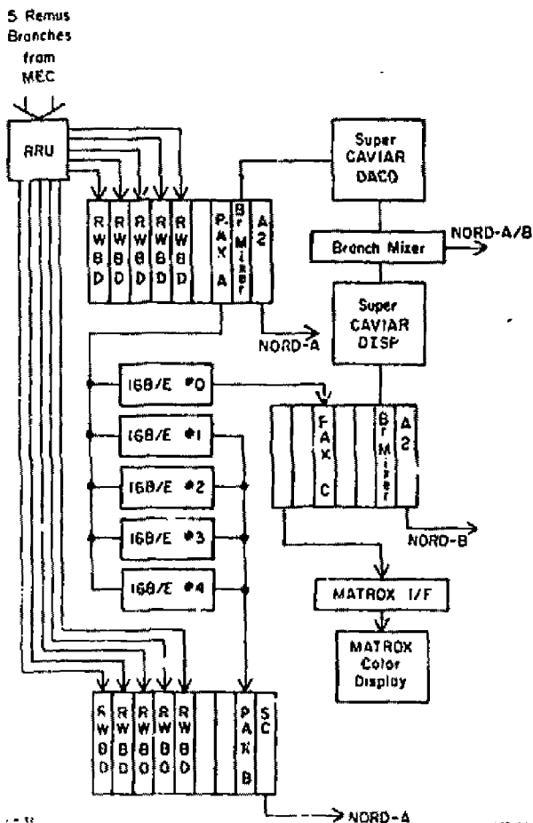
Fig. 9. PAX-168/E with Super CAVIAR.
