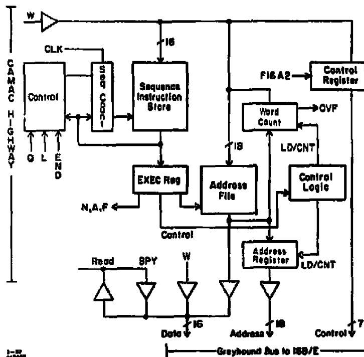
Fig. 4. PAX logic diagram.
