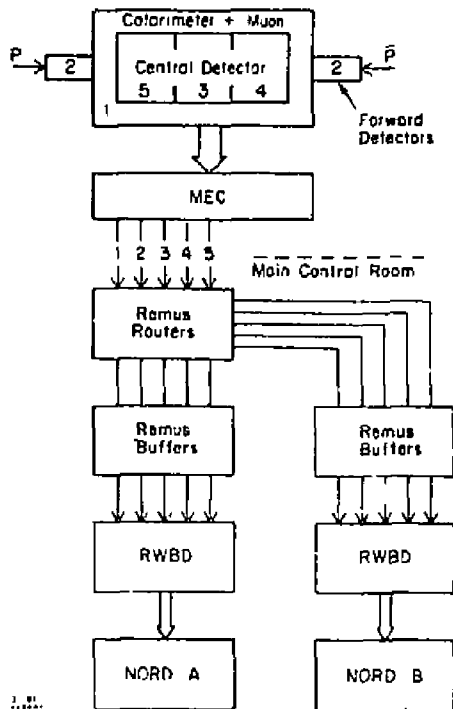
Fig. 2. NORD Remus system without 168/E.
