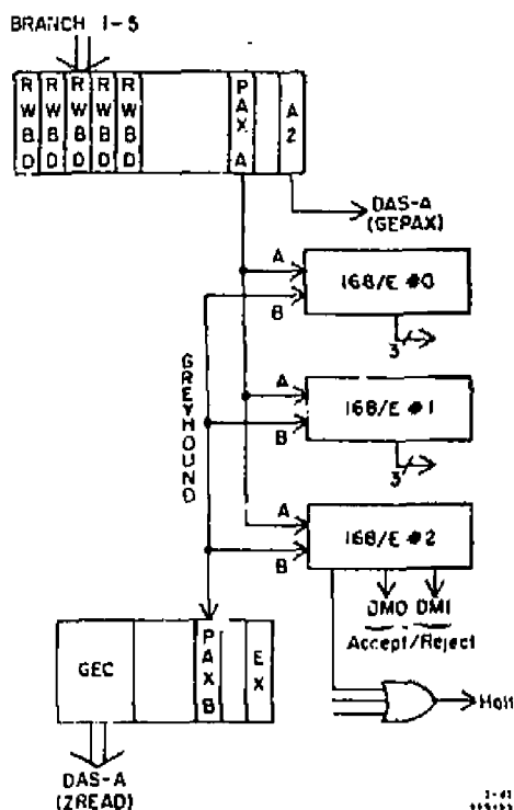
Fig. 7. NORD configuration with PAX and 168/E.
