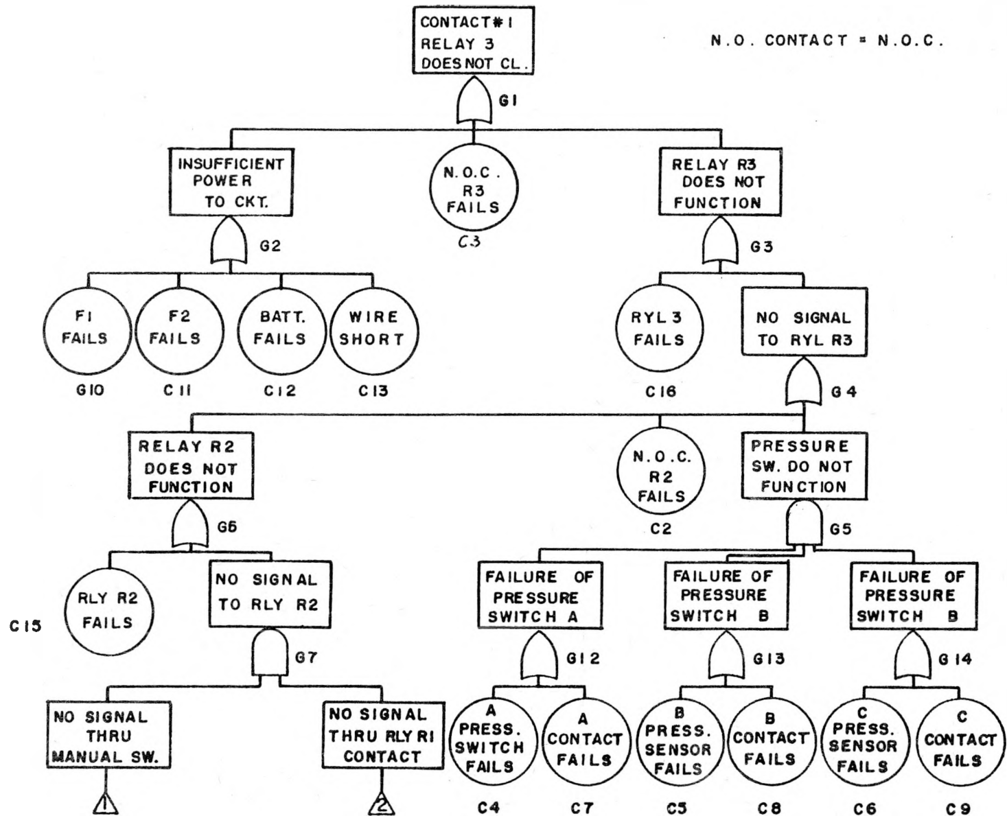
Figure 1.2 Fault Tree for Standby Protection Circuit
