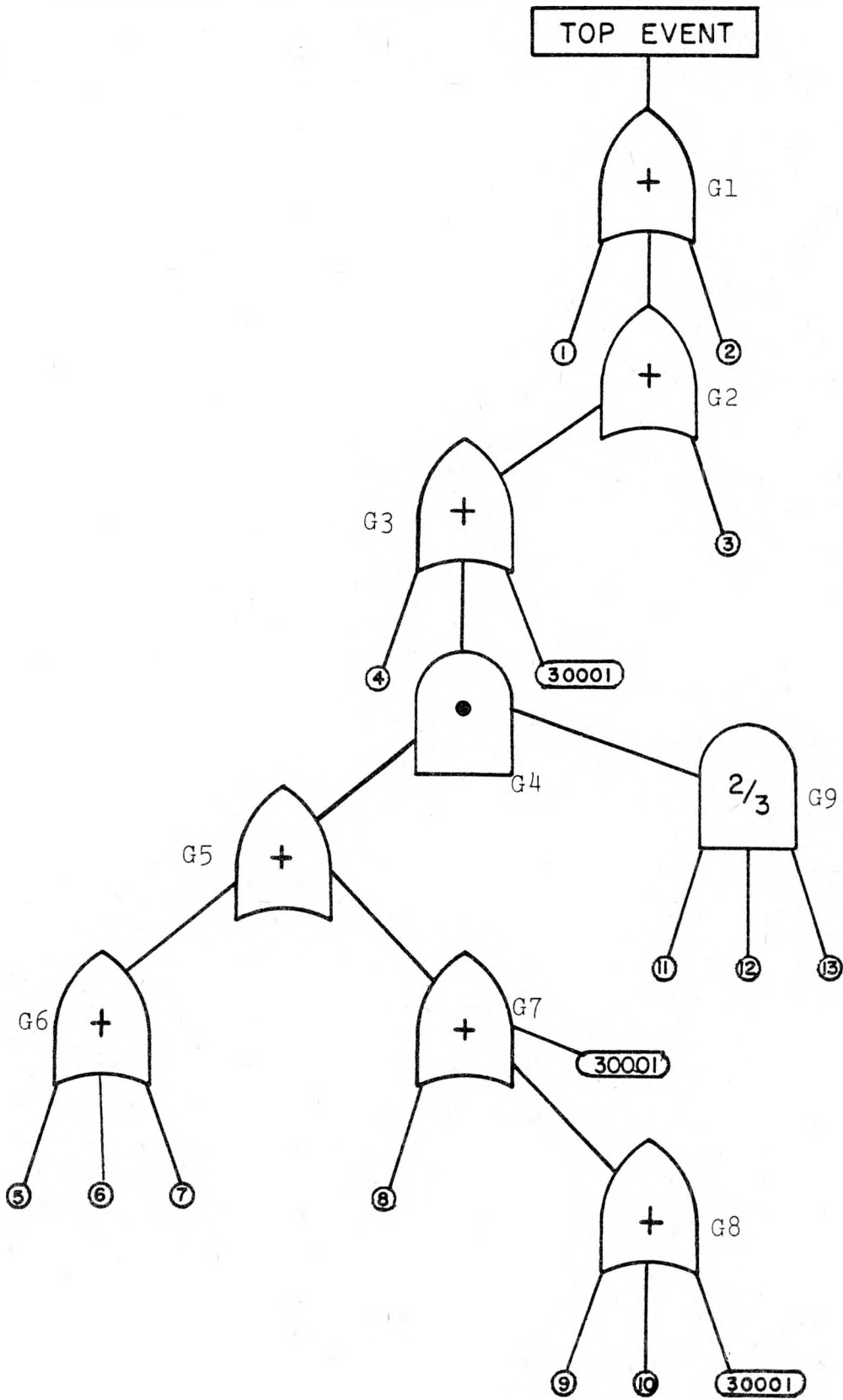
FIGURE 3.20 PRESSURE TANK RUPTURE FAULT TREE
