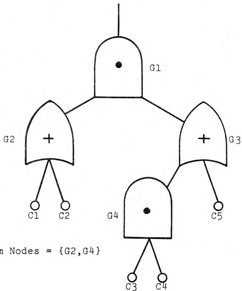
FIGURE 3.5 FAULT TREE BOTTOM BRANCH GATE NODES
