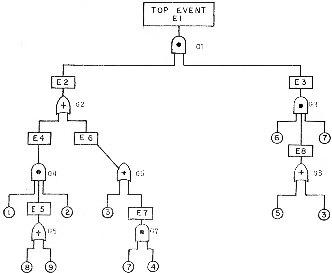
FIGURE 1.4 FAULT TREE EXAMPLE I
