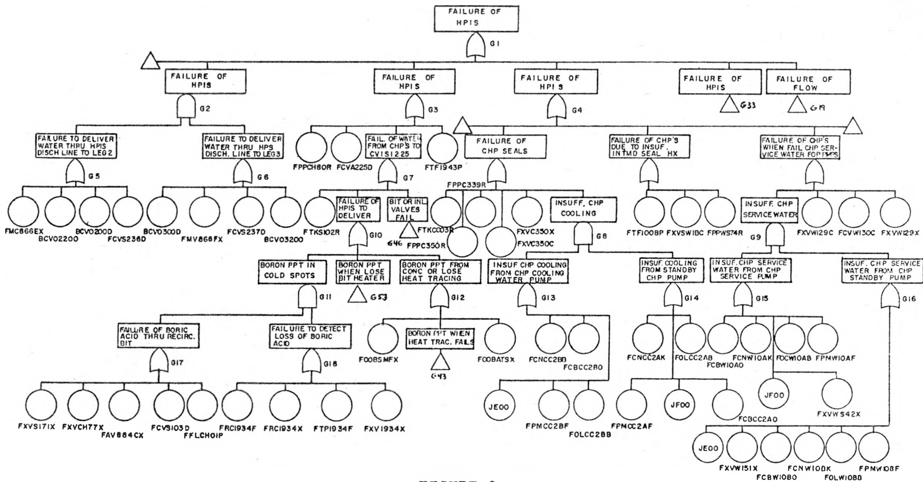
FIGURE 9 REDUCED FAULT TREE OF THE HPIS
