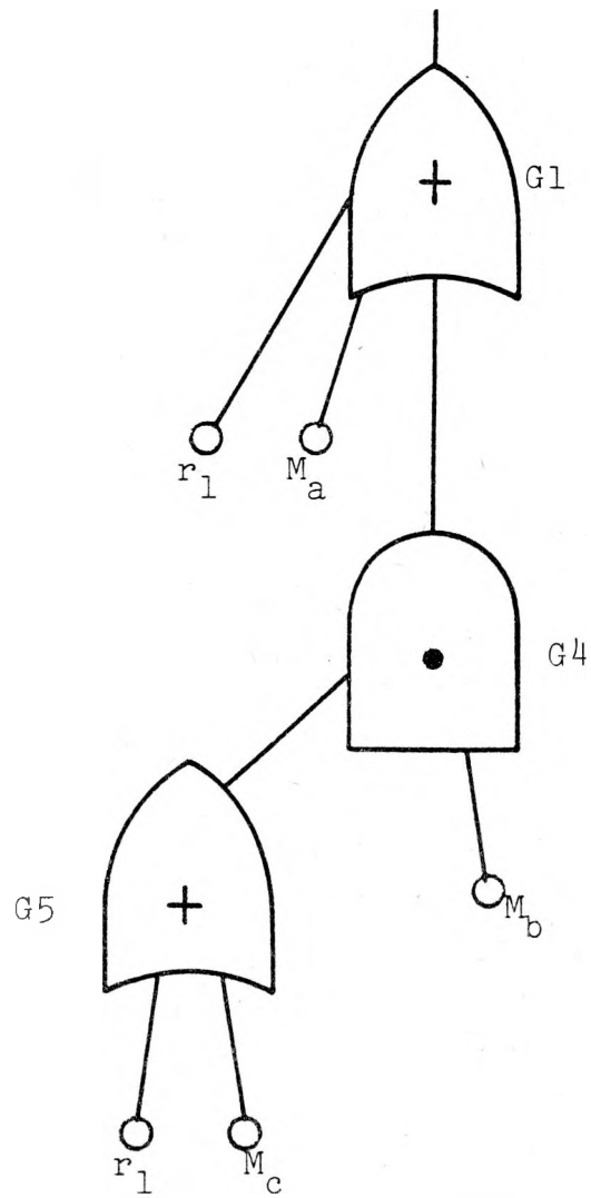
FIGURE 3.24 HIGHER ORDER MODULE
