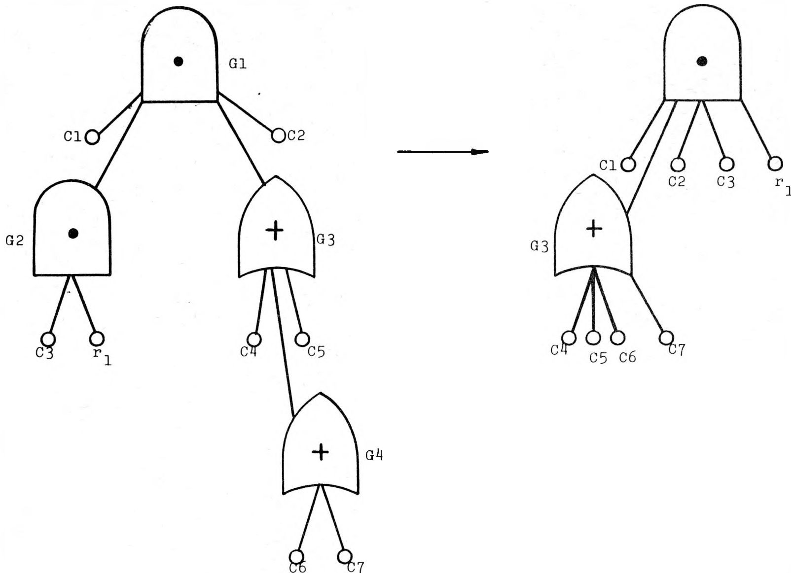
FIGURE 3.6 COALESCED GATELESS NODES
