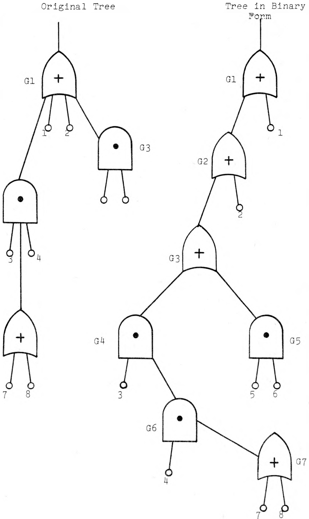
FIGURE 3.13 FAULT TREE IN BINARY GATE FORM
