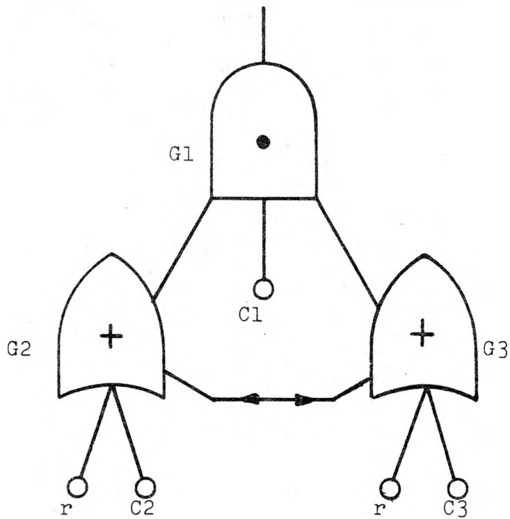
FIGURE 3.4 FAULT TREE NODE INTERCONNECTIONS
