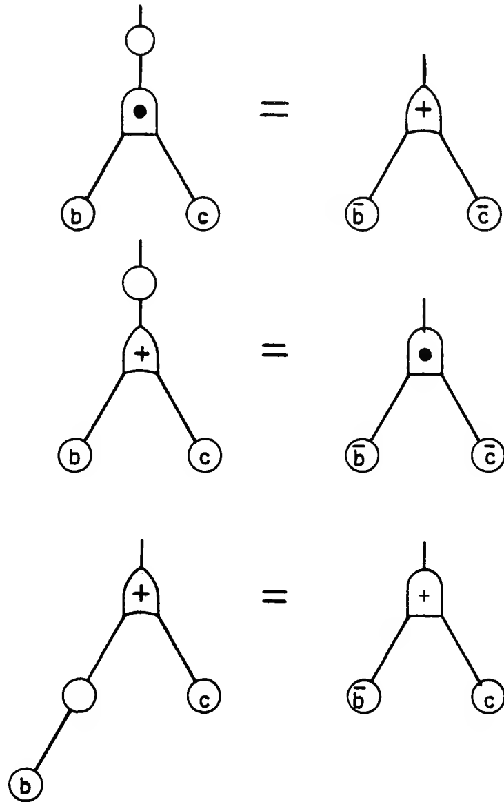
FIGURE 3.34 DUAL COMPONENT STATES
