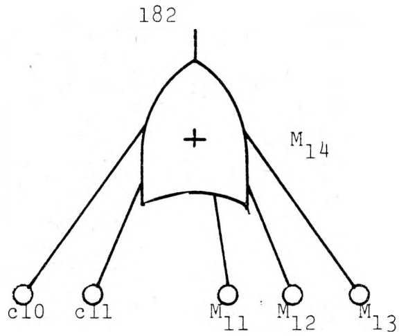
FIGURE 3.23 SIMPLE GATE MODULE
