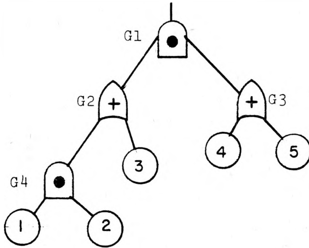
FIGURE 1.12 FAULT TREE EXAMPLE II IN BINARY GATE FORM
