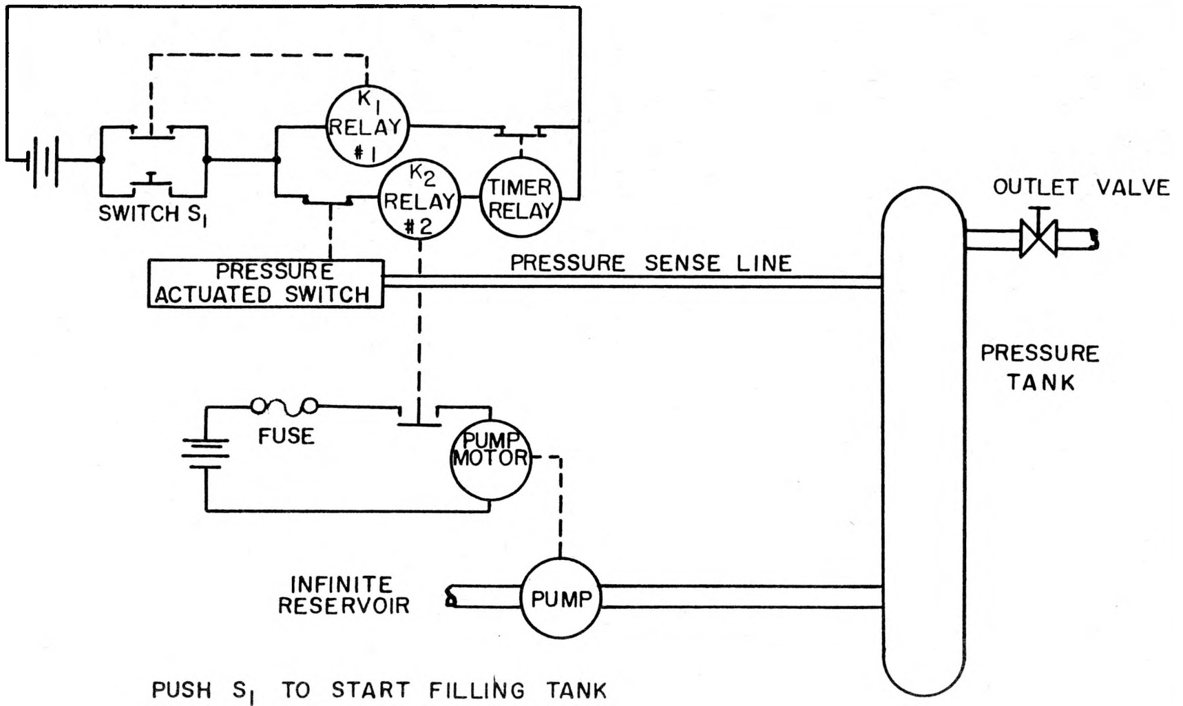
FIGURE 3.19 PRESSURE TANK EXAMPLE
