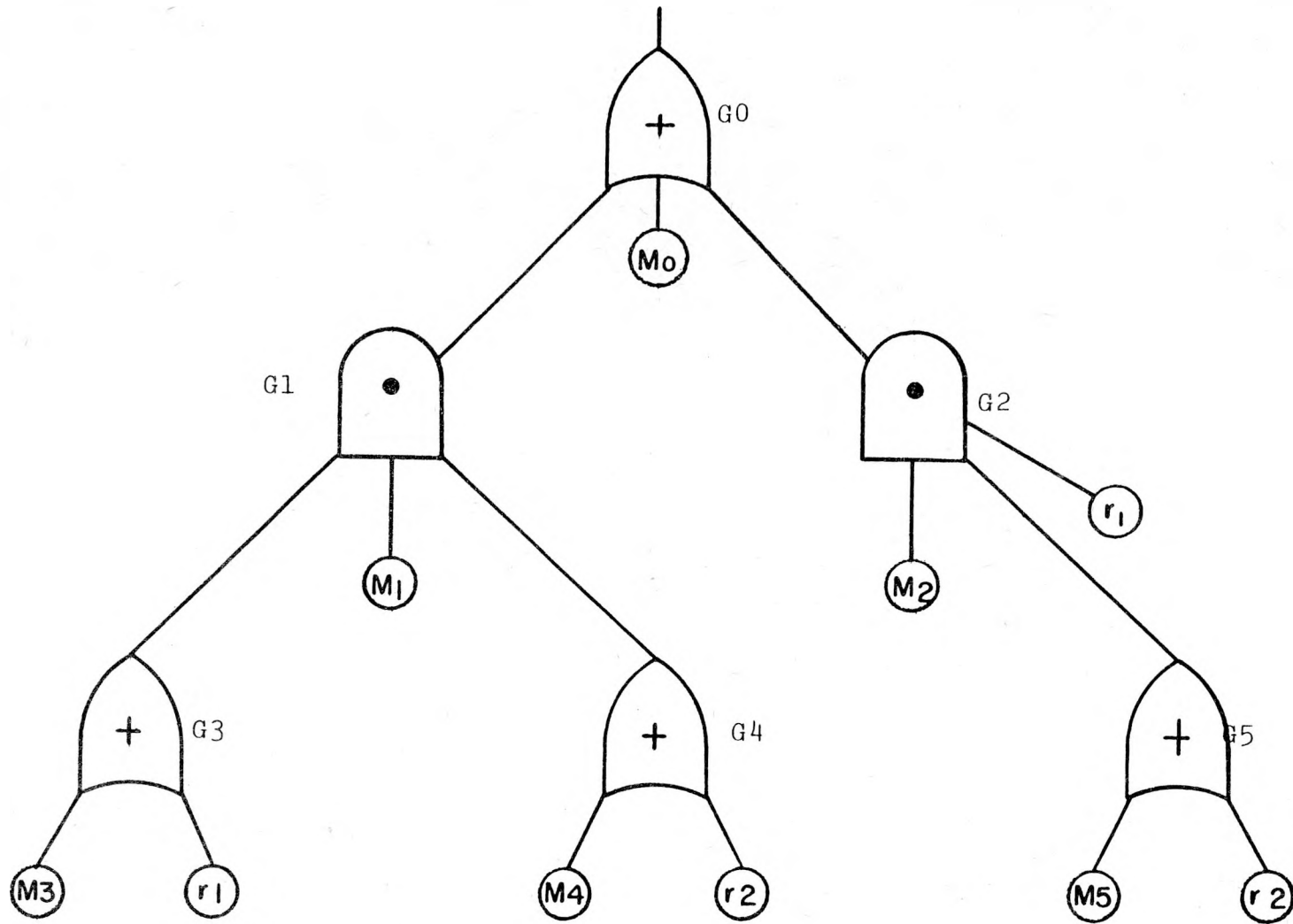
FIGURE 3.31 OR -PARENT GATE HIGHER ORDER MODULE EXAMPLE I
