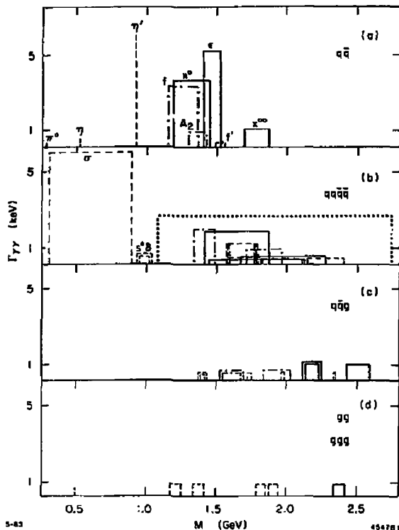
Fig. 1. Predictions for \gamma\gamma widths of: a) q\bar{q} states, b) qq\bar{q}\bar{q} states, c) q\bar{q}g states, d) gg and ggg states.
