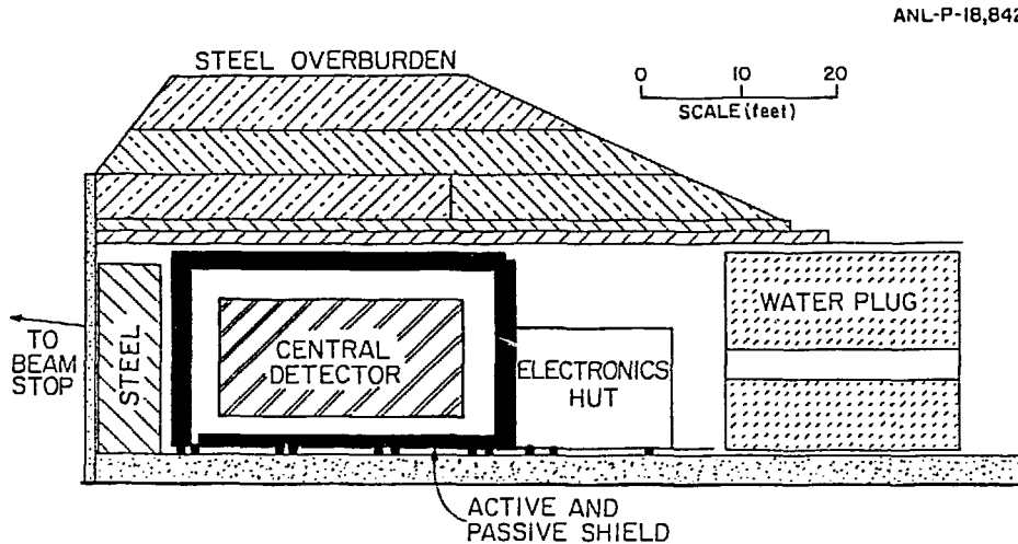
Fig. 2 The experimental arrangement. The neutrino detector and the concentric active and passive shield are housed in a tunnel under 2500 \text{ g/cm}^2 of overburden 26 m from the LAMPF beamstop. LAMPF itself is about 2200 m above sea level.
