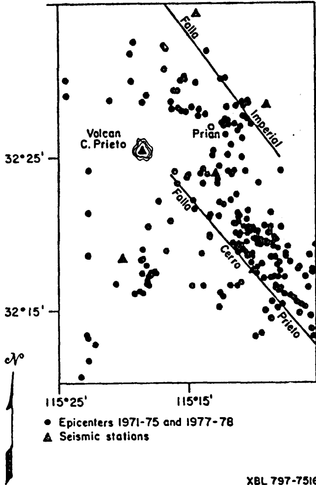
Figure 2: Microseismic studies illustrating the active movement along the northwestern terminus of the Cerro Prieto hybrid transform fault and the north to northeasterly shift to the Imperial hybrid transform fault (data from Albores and others, 1979).
