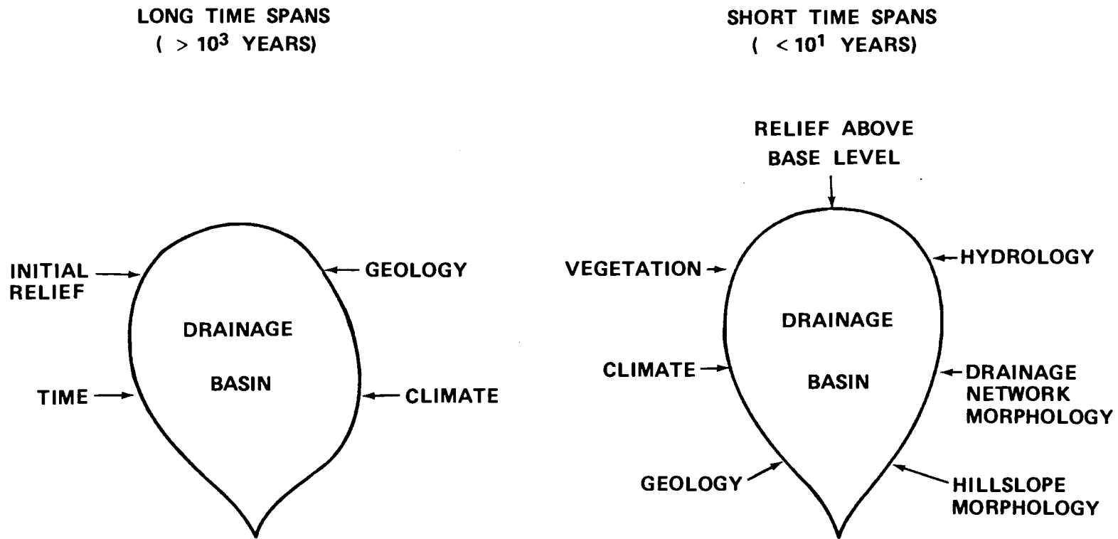
FIGURE 2. Independent Variables that Influence the Cycle of Erosion During Different Time Spans
