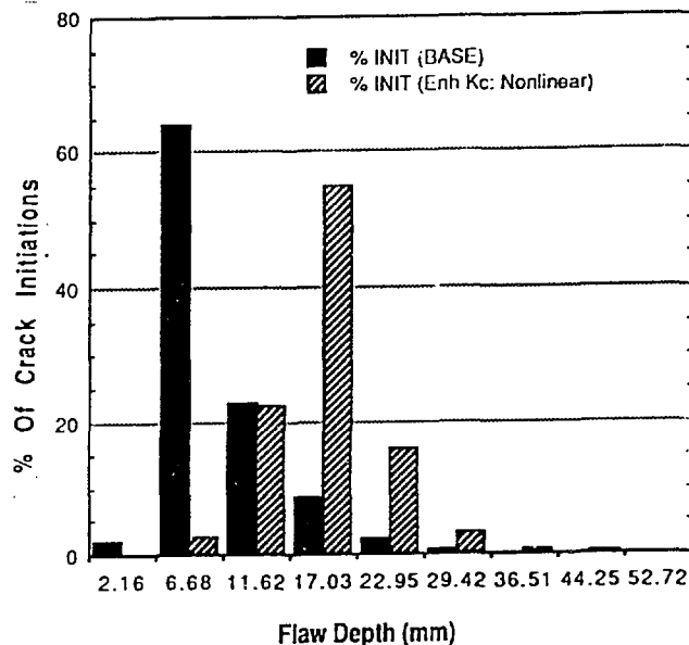
Fig. 11. Enhanced K_{Ic} data significantly reduces P(F|E) for two reasons: a) for shallow flaws, probability of crack initiation is reduced, and b) flaw density for critical size flaws is reduced.
