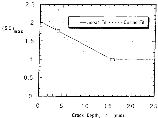
Fig. 7. (SC)_{max} vs crack depth was determined using a linear and nonlinear fit from the two data points.
