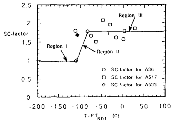
Fig. 6. The SC-factor for A533 was estimated using the A36 and A517 data for a = 3.8 mm and is divided into three regions.
