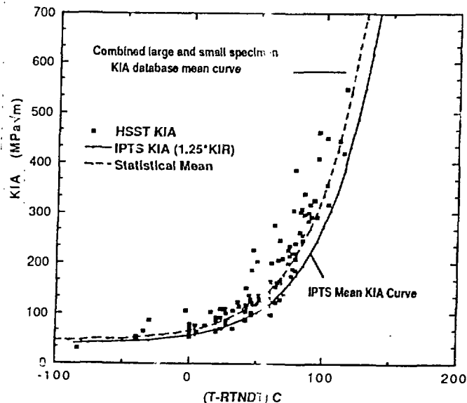
Fig. 10. The statistical mean curve for the combined HSST data base is steeper than the mean curve used in the IPTS study
