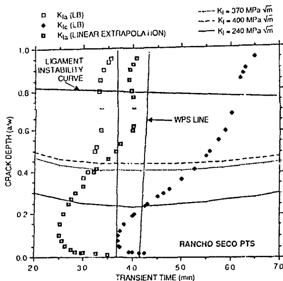
Fig. 5. Negation of enhanced crack-arrest potential by onset of unstable ductile tearing.
