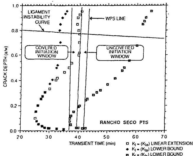
Fig. 3. K_{IA} linear extrapolation showing reduction of range of flaw depths that can result in failure.
