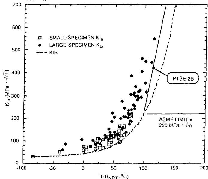
Fig. 1. Combined large- and small-specimen HSST K_{Ia} data base (two extrapolations above 220 \text{ MPa} \cdot \sqrt{\text{m}} ).
