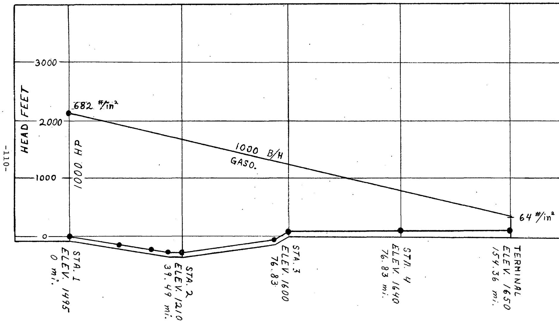
FIGURE 4.3.6.1.2-1 - HYDRAULIC GRADIENT, ONE PUMP, ALL GASOLINE
