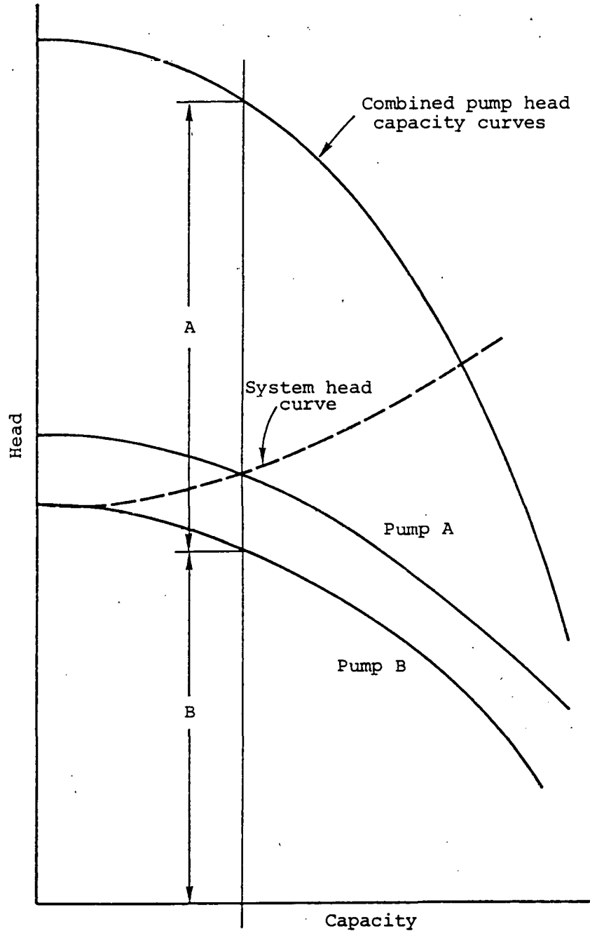
Fig. 7.1.1-5 - Head-capacity curves of pumps operating in series
