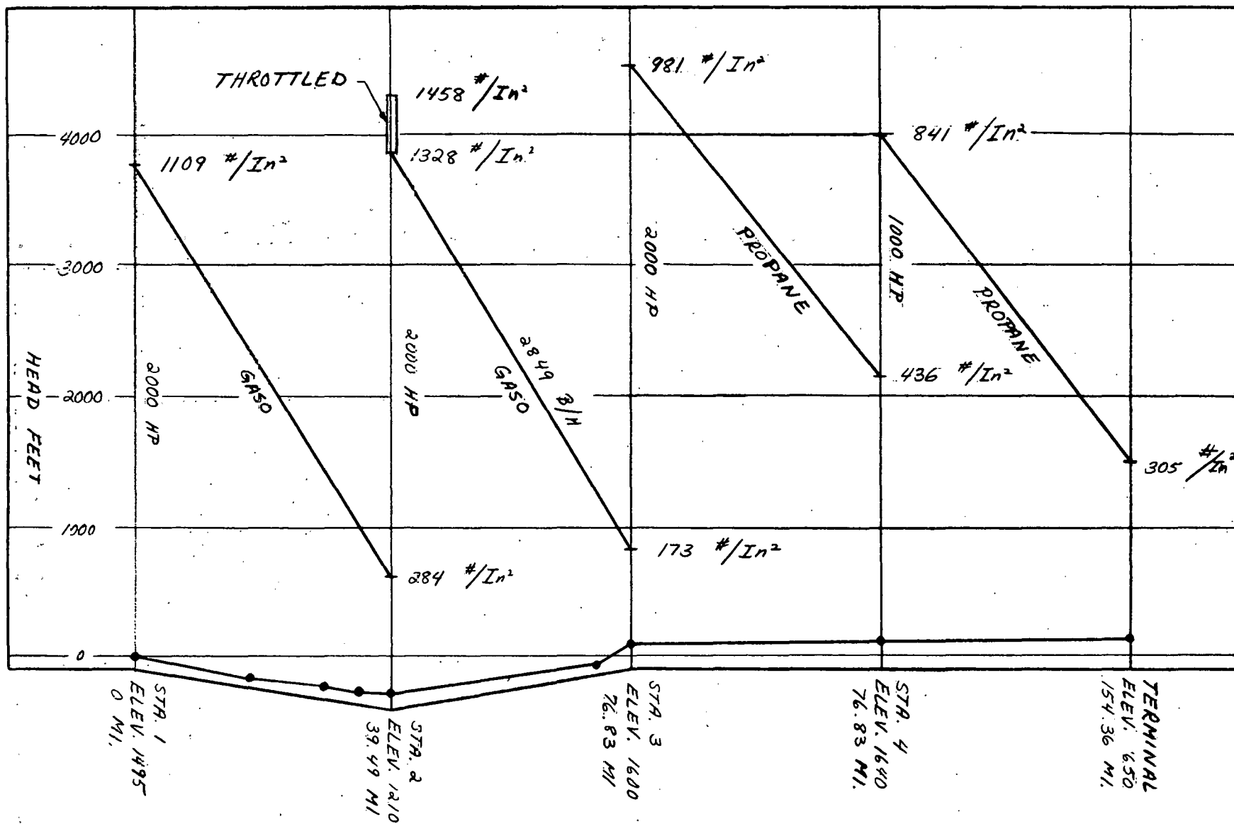
FIGURE 4.3.5.1.2-16 - HYDRAULIC GRADIENT, EIGHT/NINE PUMPS, TWO INITIAL SEGMENTS GASOLINE, TWO SEGMENTS PROPANE
