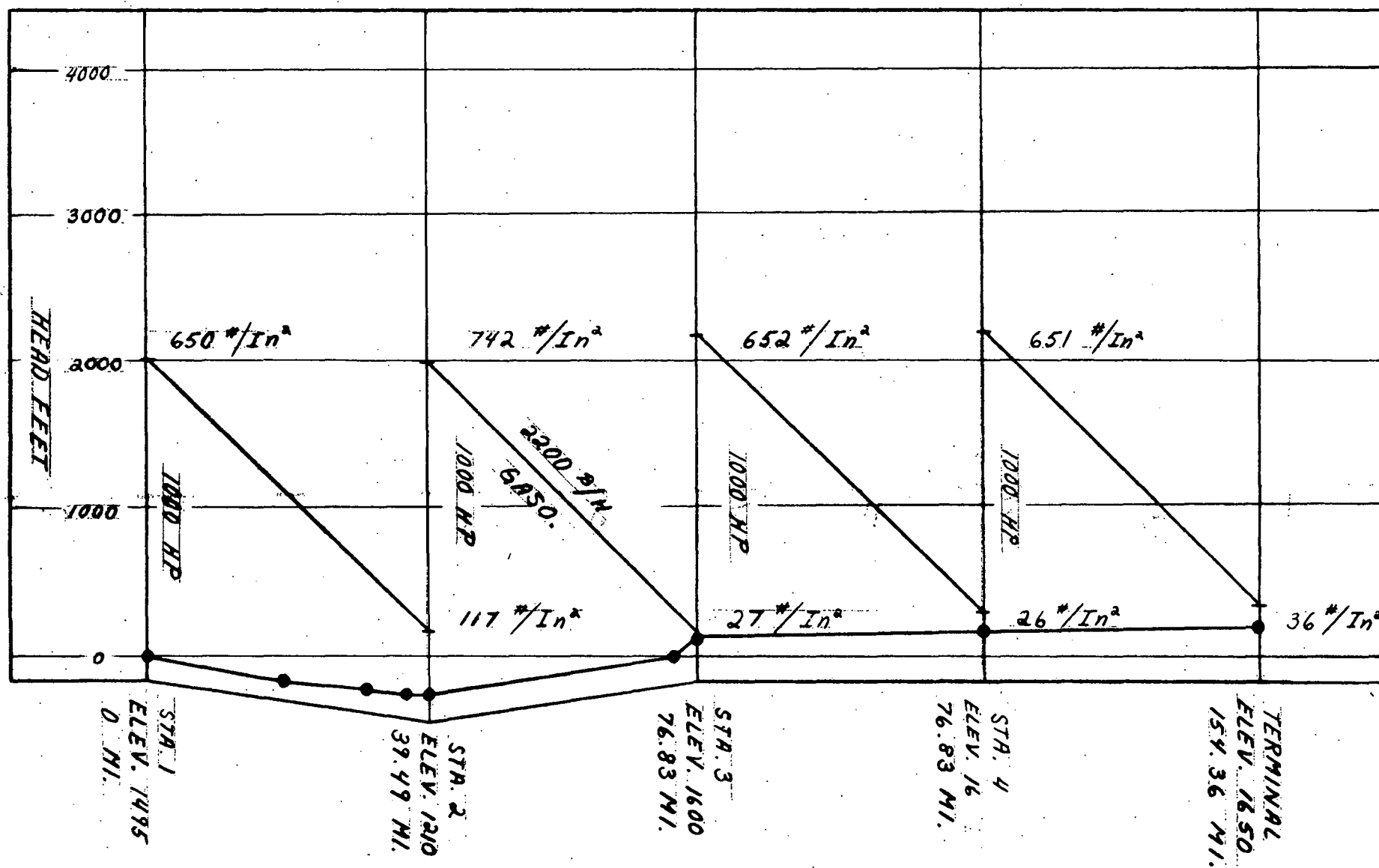
FIGURE 4.3.6.1.2-4 - HYDRAULIC GRADIENT, FOUR PUMPS, ALL GASOLINE
