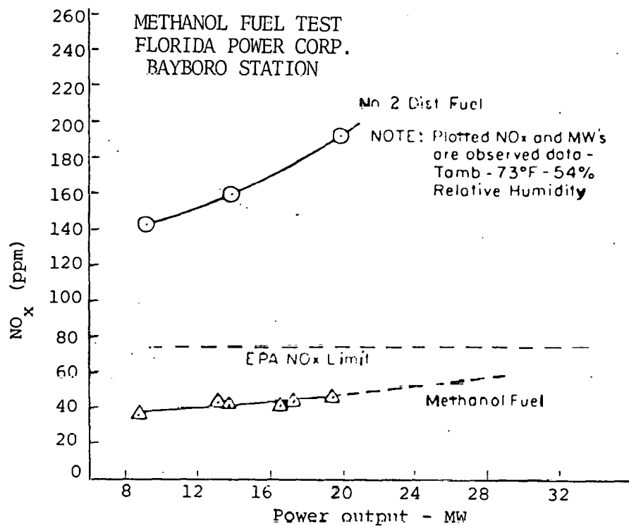
Fig. 5.3.2-1 - NO x Emissions - Gas Turbine Test with Methanol Fuel
