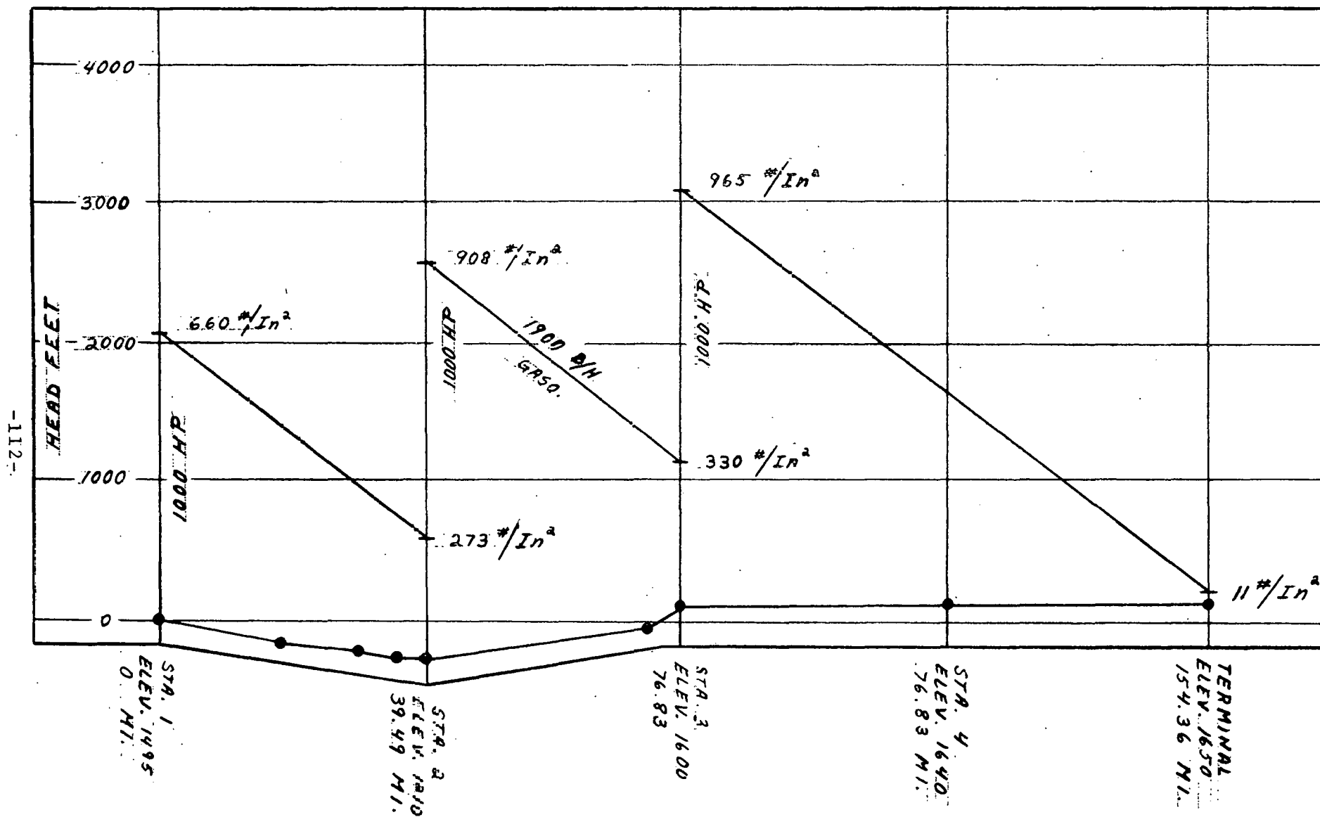
FIGURE 4.3.6.1.2-3 - HYDRAULIC GRADIENT, THREE PUMPS, ALL GASOLINE
