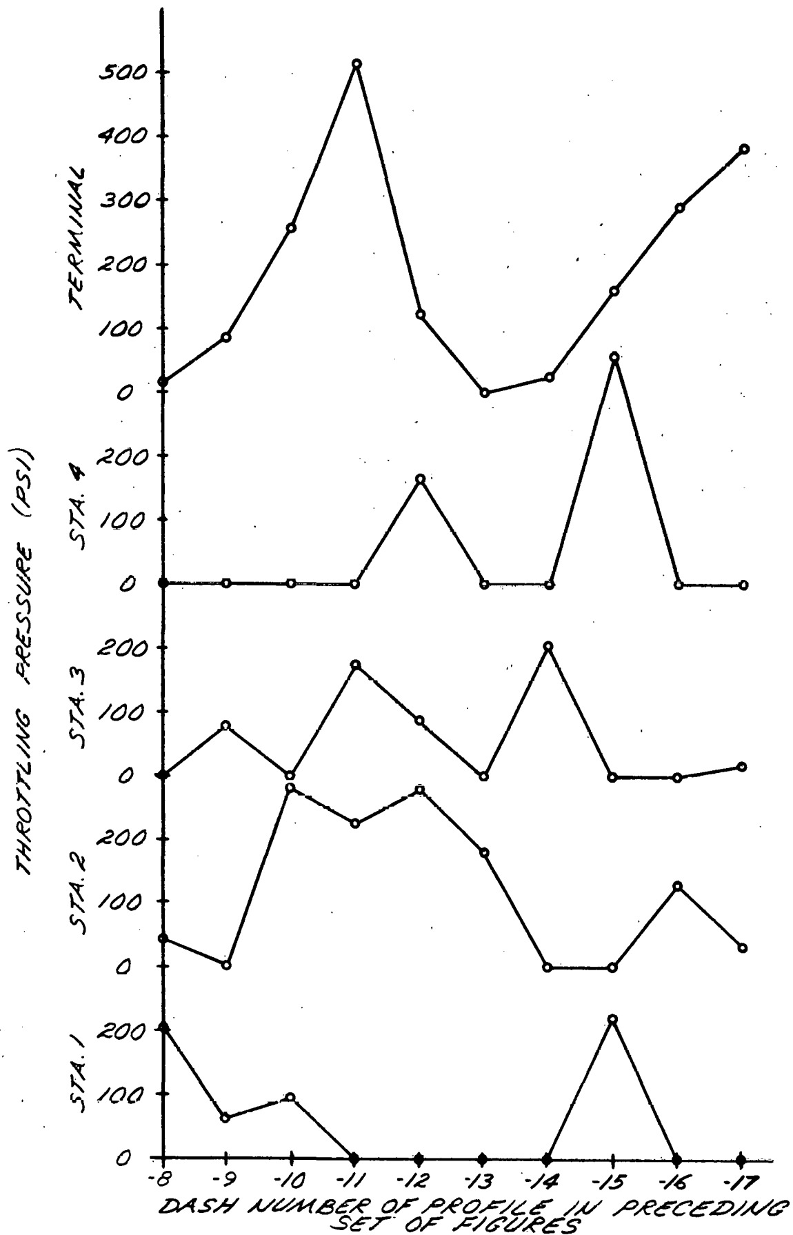
FIGURE 4.3.6.1.2-21 - THROTTLING ENERGY WASTED IN TYPICAL FULL CAPACITY PRODUCTS PIPELINE DUTY CYCLE
