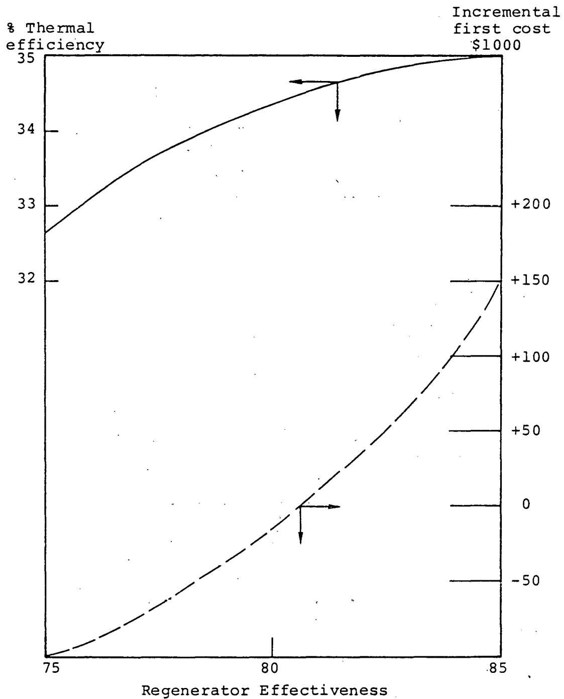
Fig. 4.1.1.1-3 Effects of regencrator effectiveness
