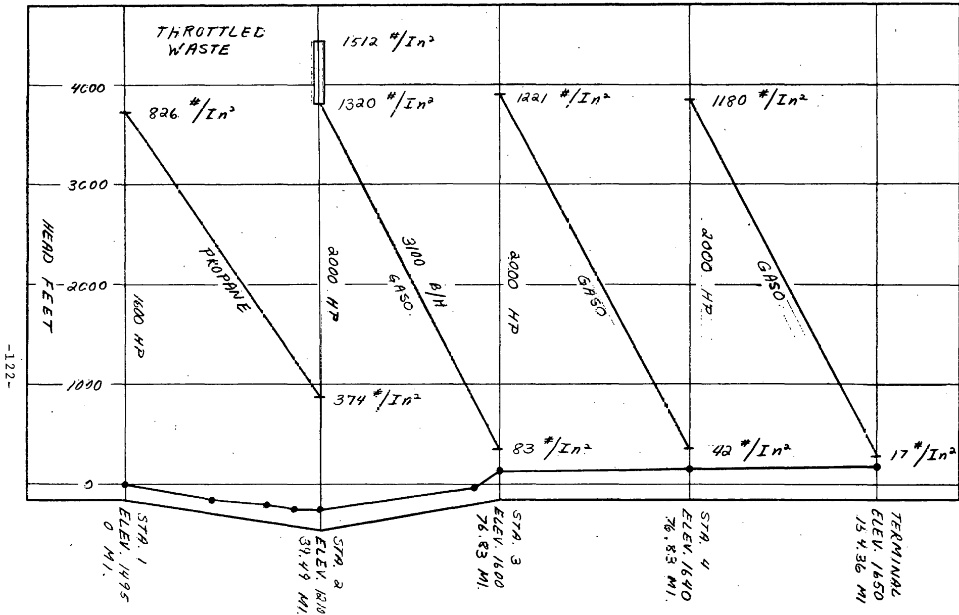
FIGURE 4.3.6.1.2-13 - HYDRAULIC GRADIENT, EIGHT PUMPS, ONE SEGMENT PROPANE, THREE SEGMENTS GASOLINE
