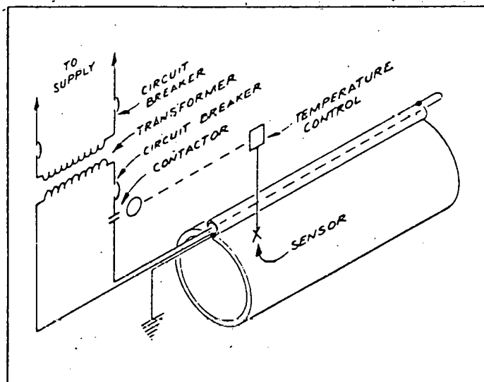
Figure 8.1-2 Details of SECT power circuit.
