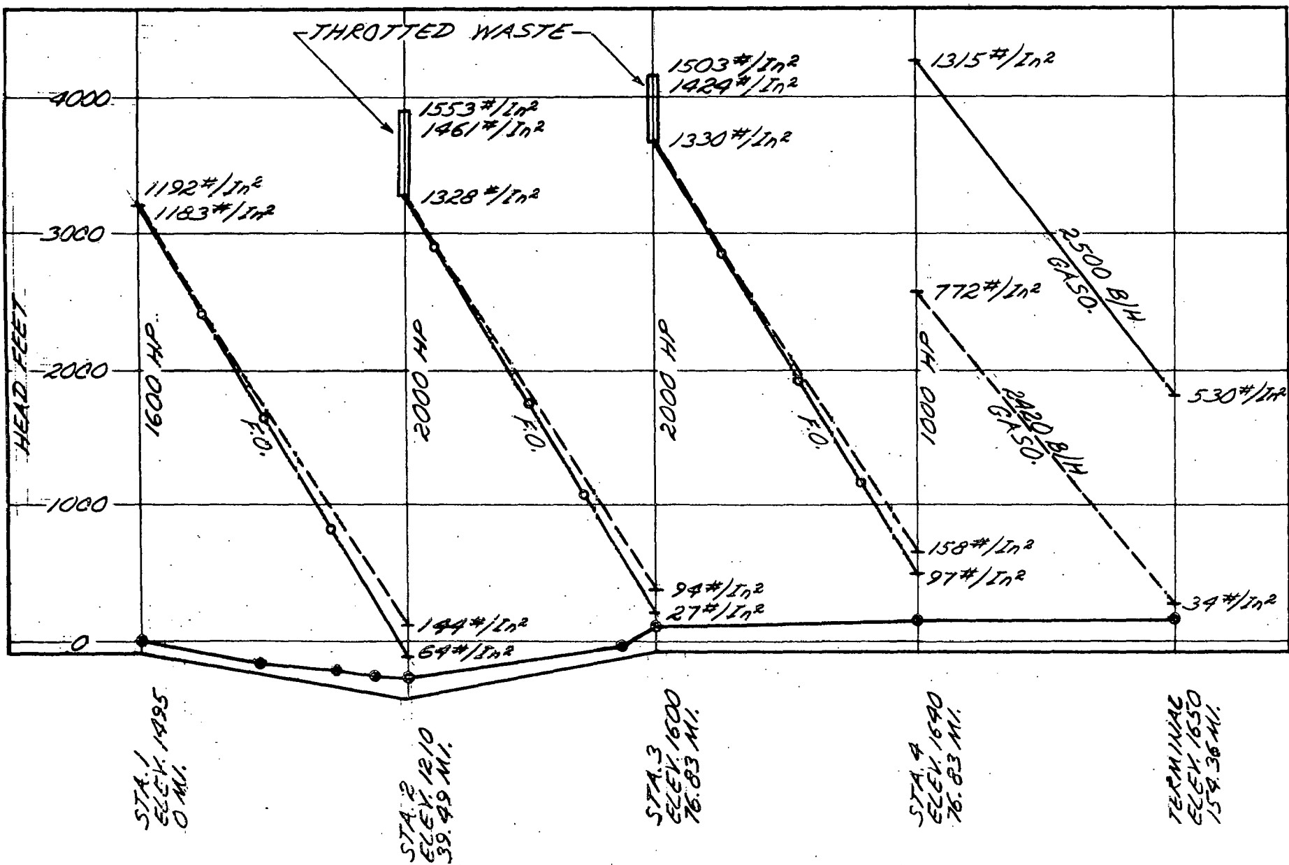
FIGURE 4.3.6.1.2-11 - HYDRAULIC GRADIENT, SEVEN/EIGHT PUMPS, THREE SEGMENTS FUEL OIL, ONE SEGMENT GASOLINE
