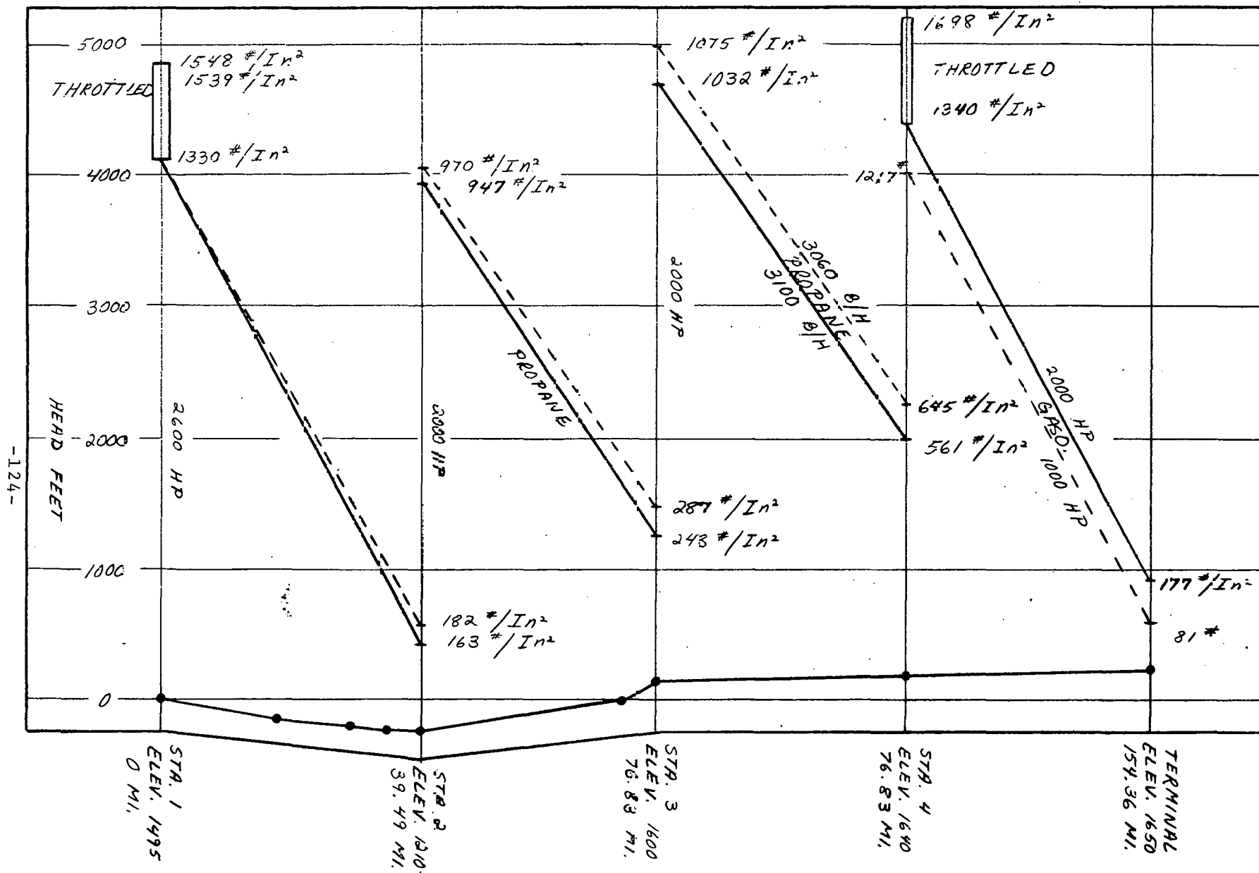
FIGURE 4.3.6.1.2-15 - HYDRAULIC GRADIENT, SEVEN PUMPS, TWO INITIAL SEGMENTS PROPANE, TWO SEGMENTS GASOLINE
