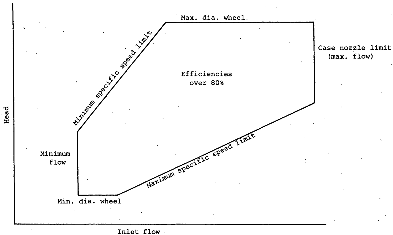
Fig. 7.3-2 - Centrifugal compressor case characteristics
