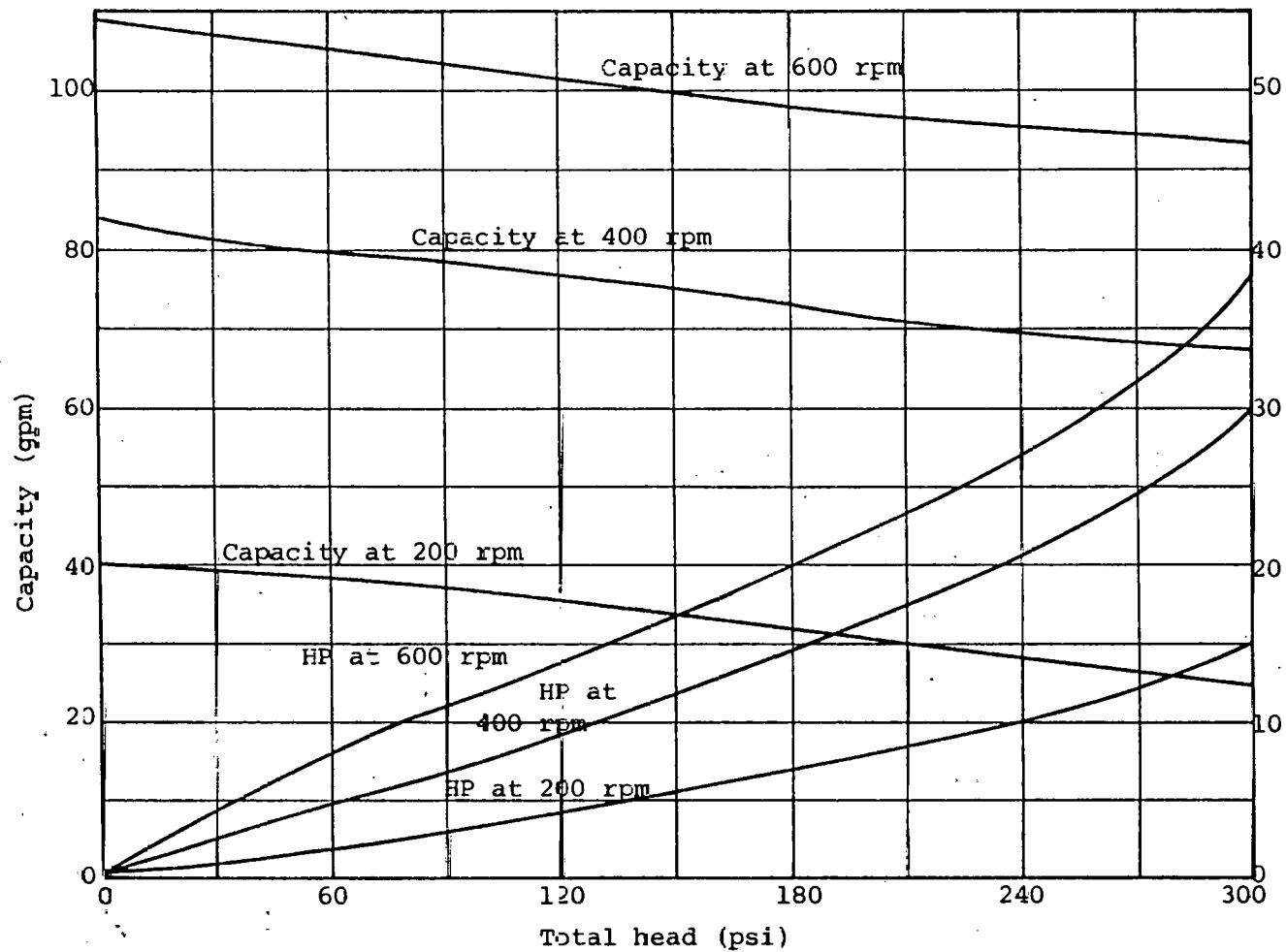
Fig. 7.1.2-1 - Capacity and horsepower characteristics of a typical rotary pump
