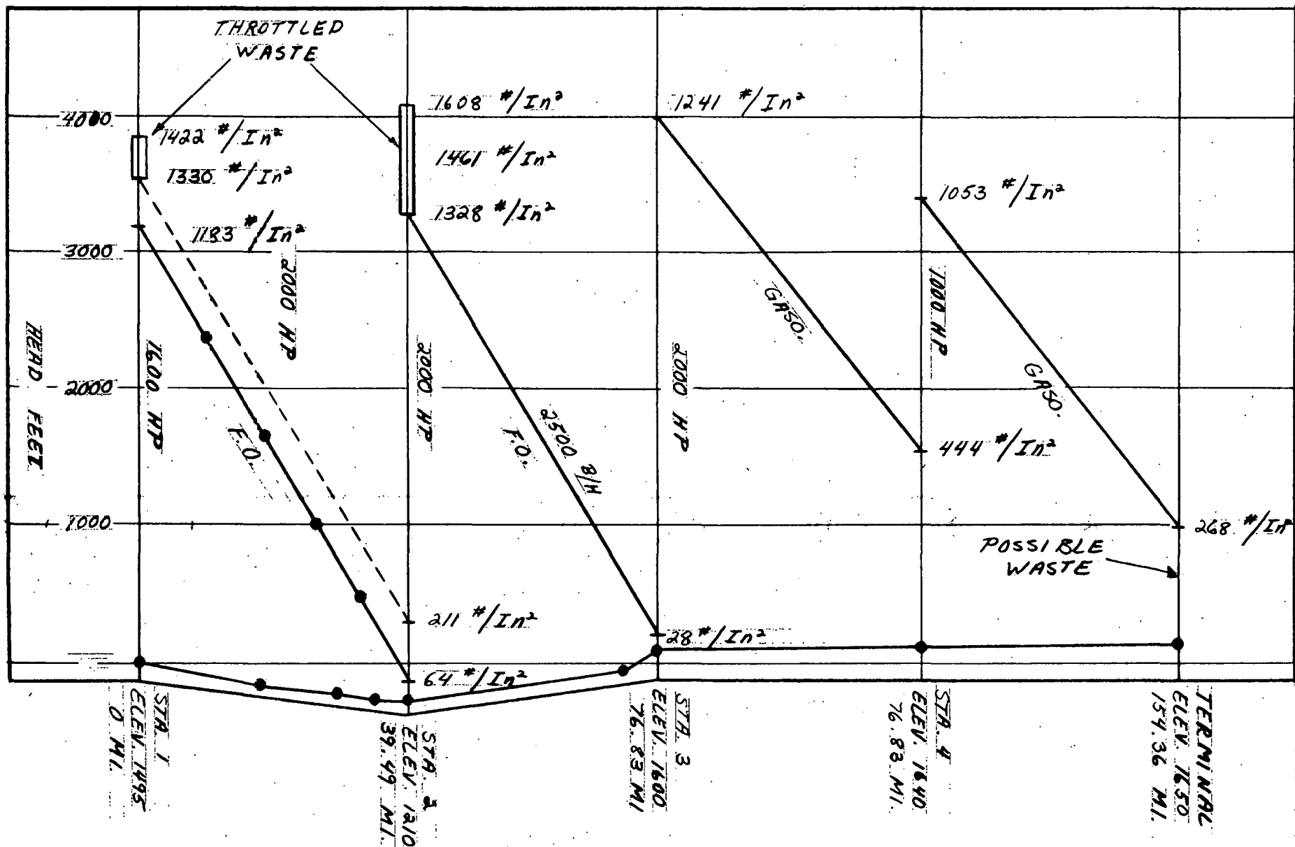
FIGURE 4.3.6.1.2-10 - HYDRAULIC GRADIENT, SEVEN PUMPS, TWO SEGMENTS FUEL OIL, TWO SEGMENTS GASOLINE
