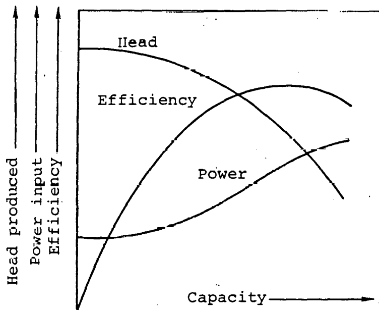
Fig. 7.1.1-1 - Typical characteristic curves at constant rpm
