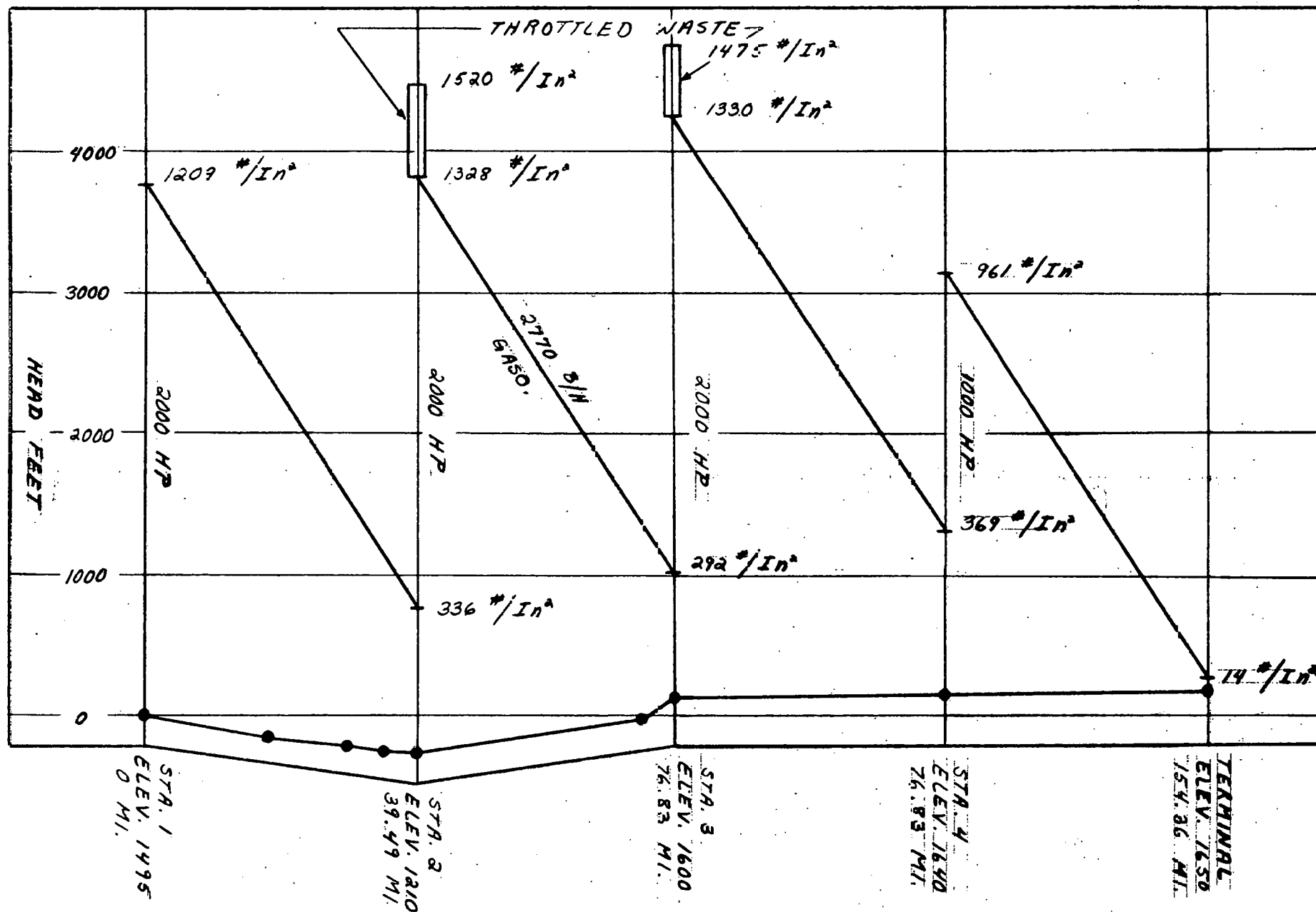
FIGURE 4.3.6.1.2-7 - HYDRAULIC GRADIENT, SEVEN PUMPS ALL GASOLINE
