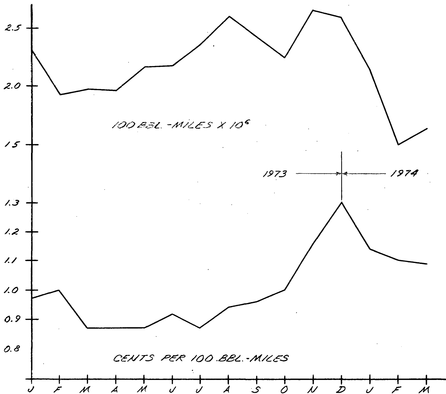
FIGURE 4.3.6.1.2-20 - UNIT ENERGY COST AND TOTAL THROUGHPUT
