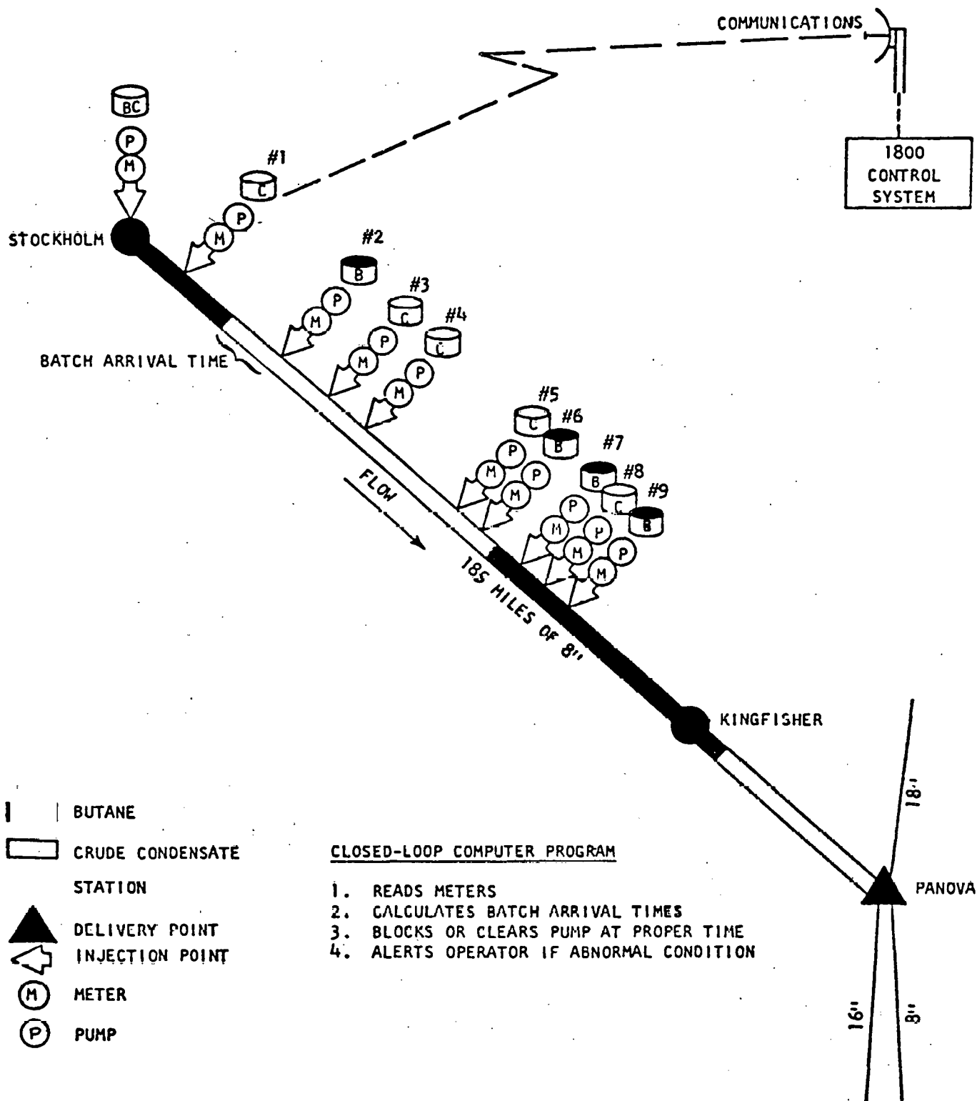
Figure 9.1-4 ARCO Western Oklahoma crude condensate line block-clear computer control program
