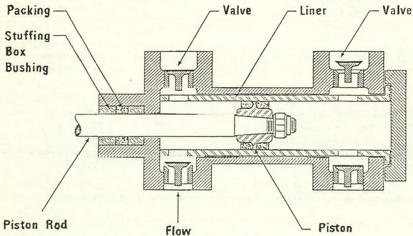
Fig. 7.2-1 - Piston pump - fluid end
