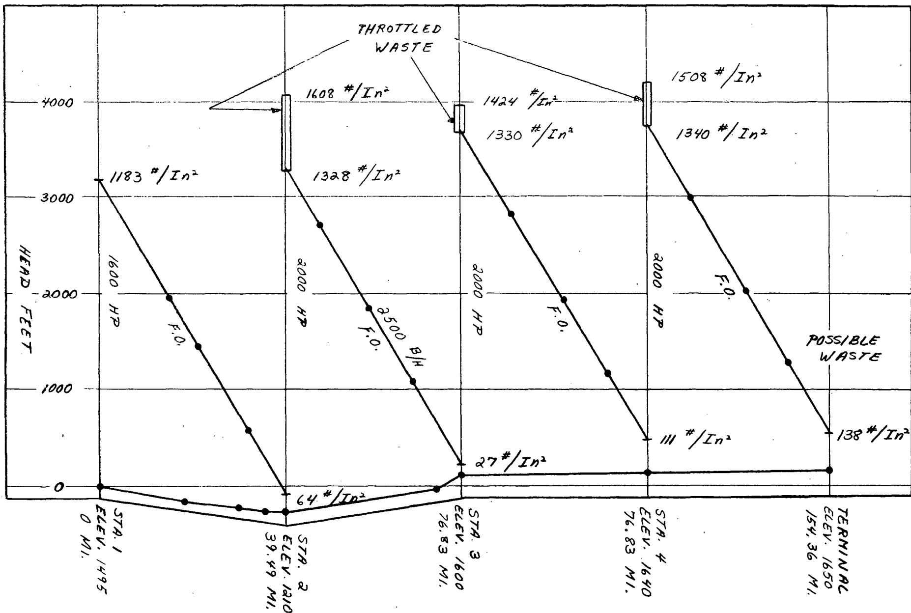
FIGURE 4.3.6.1.2-12 - HYDRAULIC GRADIENT, EIGHT PUMPS ALL FUEL OIL
