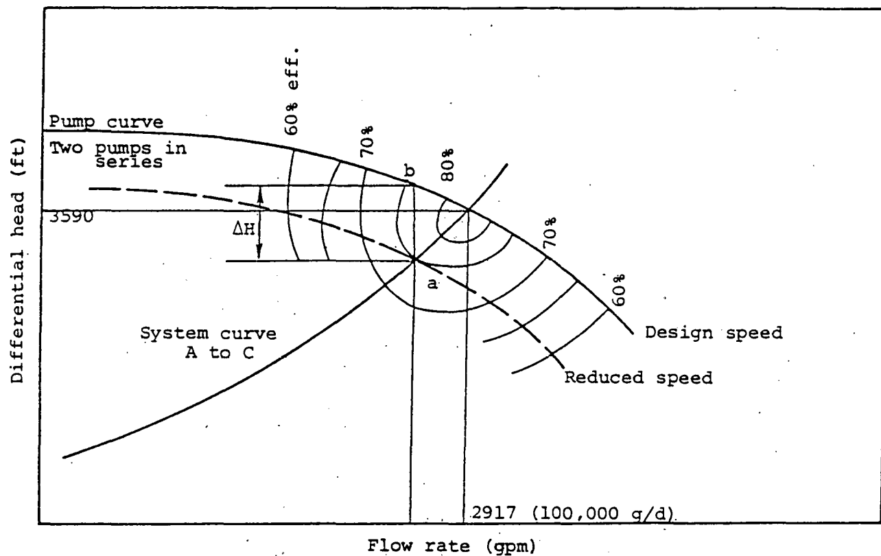
Fig. 7.1.1-6 - Head-capacity curves at design speed and reduced speed - two pumps in series
