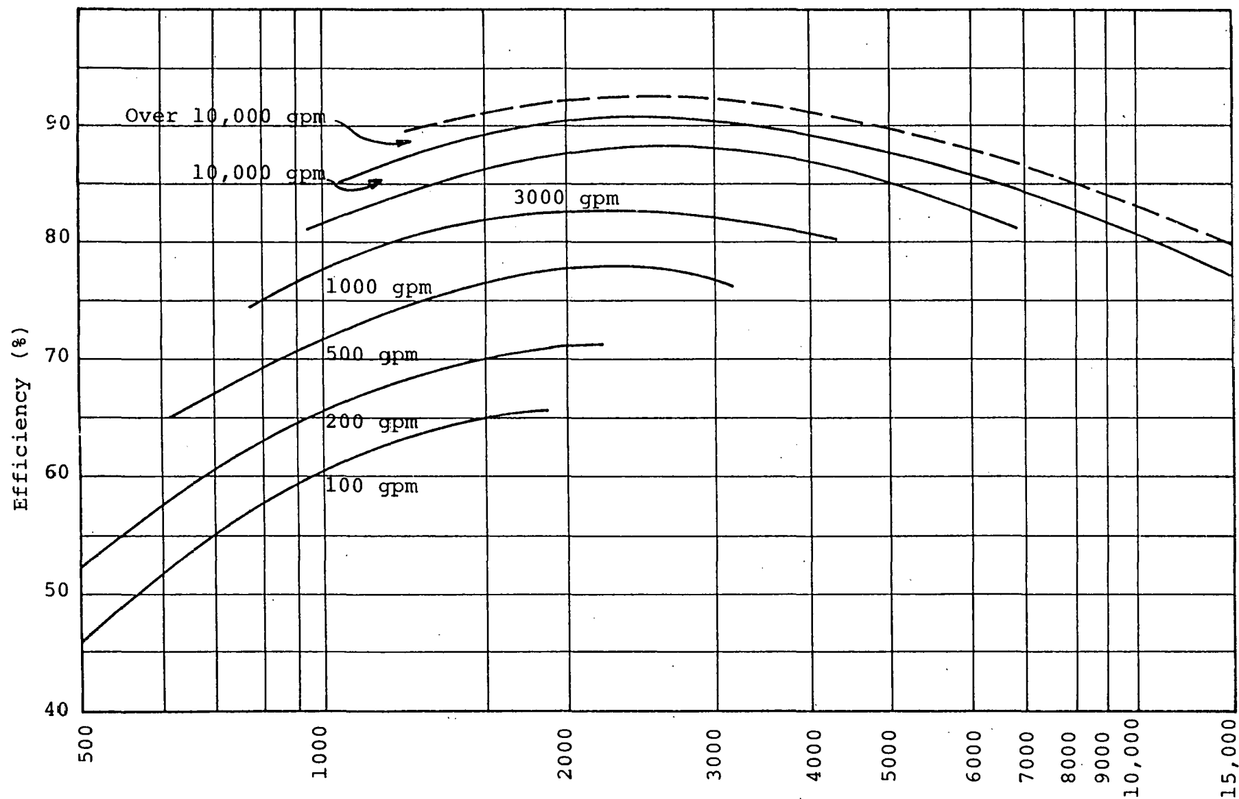
Fig. 7.1.1-2 - Efficiencies of single-stage pumps
