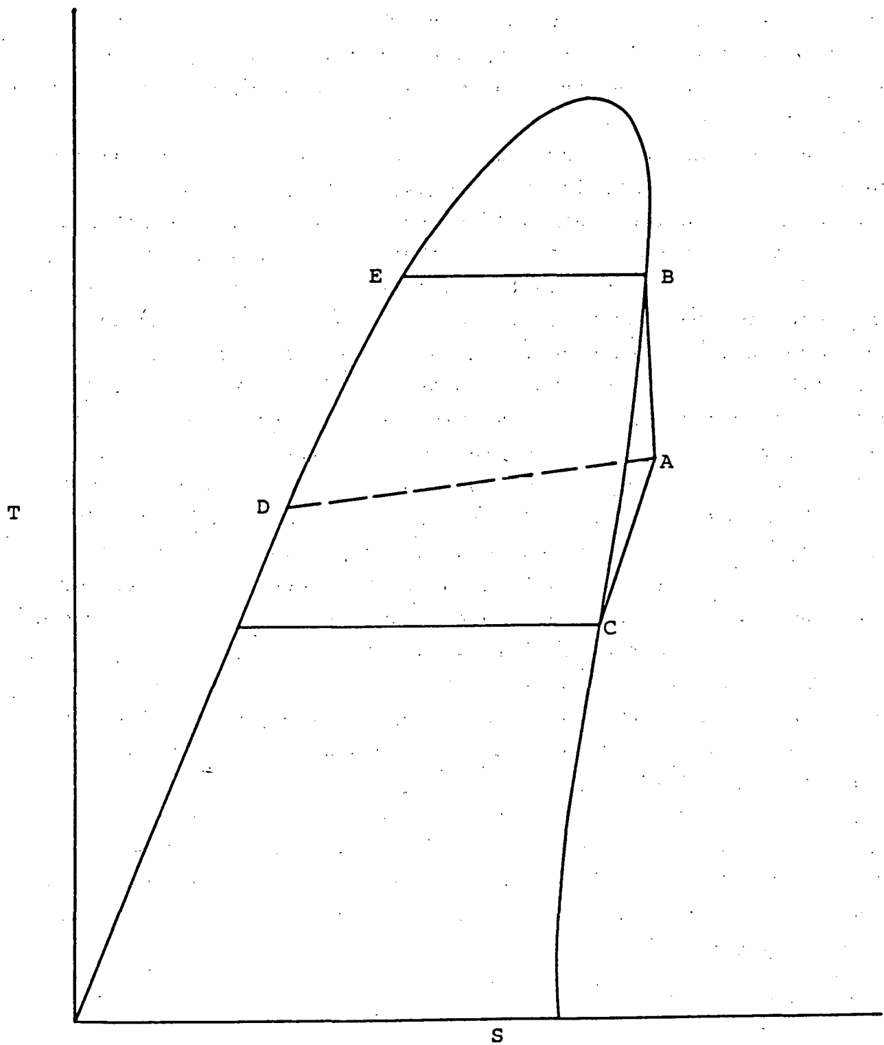
Fig. 4.1.2.2-3 Typical saturation line for organic fluid
