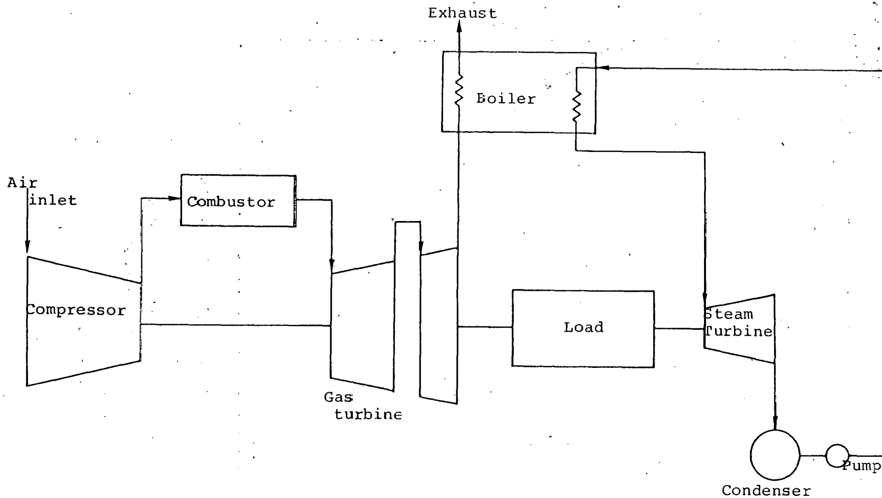
Fig. 4.1.1.2-1 Simple cycle gas turbine/Rankine cycle combined power plant
