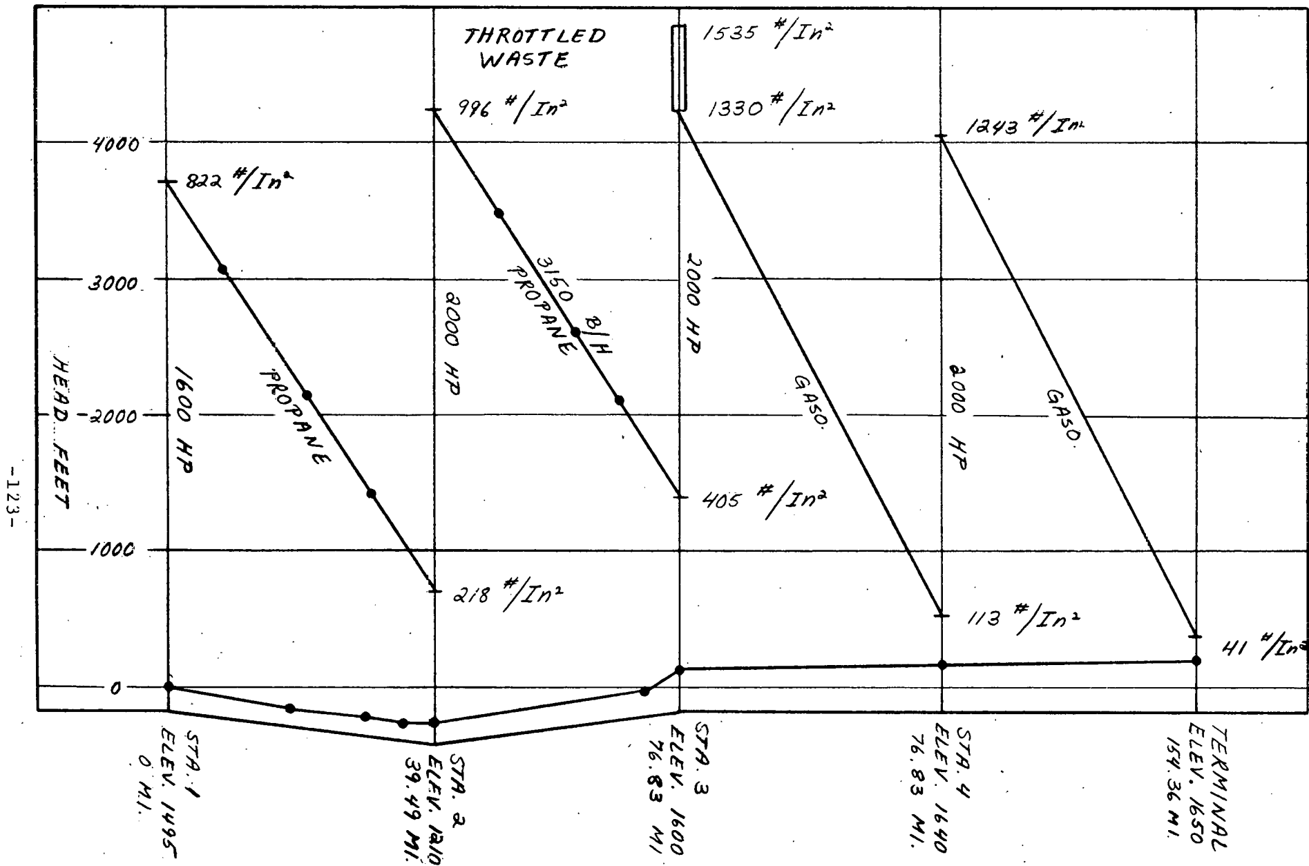
FIGURE 4.3.6.1.2-14 - HYDRAULIC GRADIENT, EIGHT PUMPS, TWO INITIAL SEGMENTS PROPANE, TWO SEGMENTS GASOLINE
