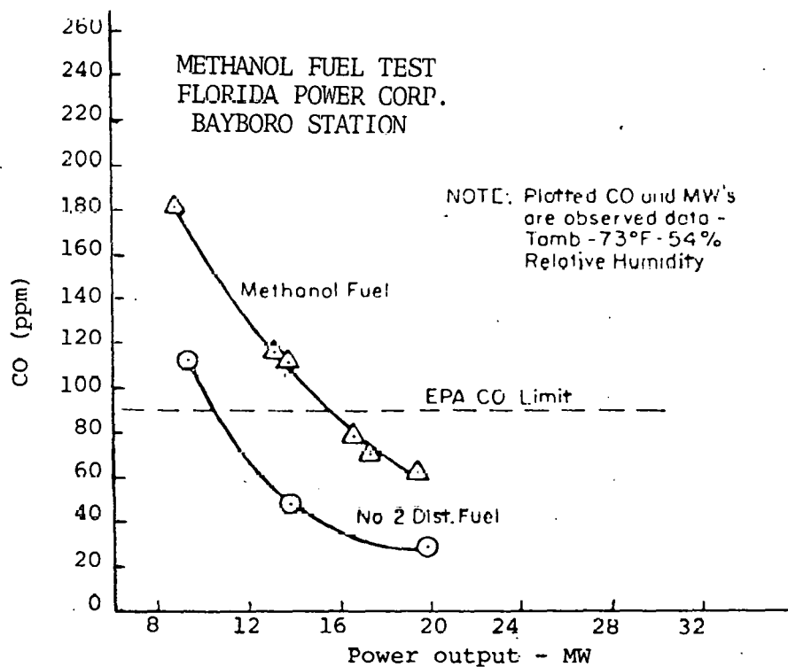
Fig. 5.3.2-2 - CO Emission - Gas Turbine Test with Methanol Fuel
