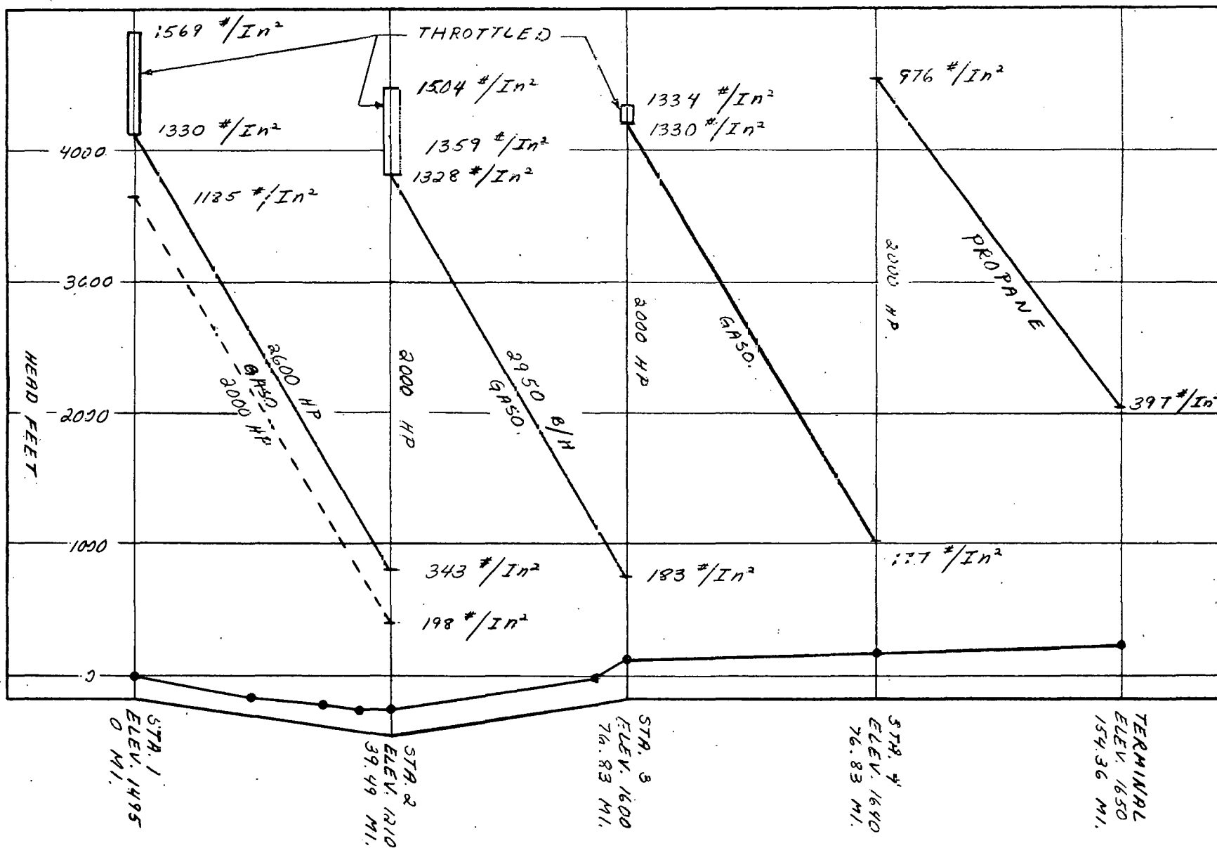
FIGURE 4.3.6.1.2-17 - HYDRAULIC GRADIENT, EIGHT/NINE PUMPS, THREE INITIAL SEGMENTS GASOLINE, LAST SEGMENT PROPANE
