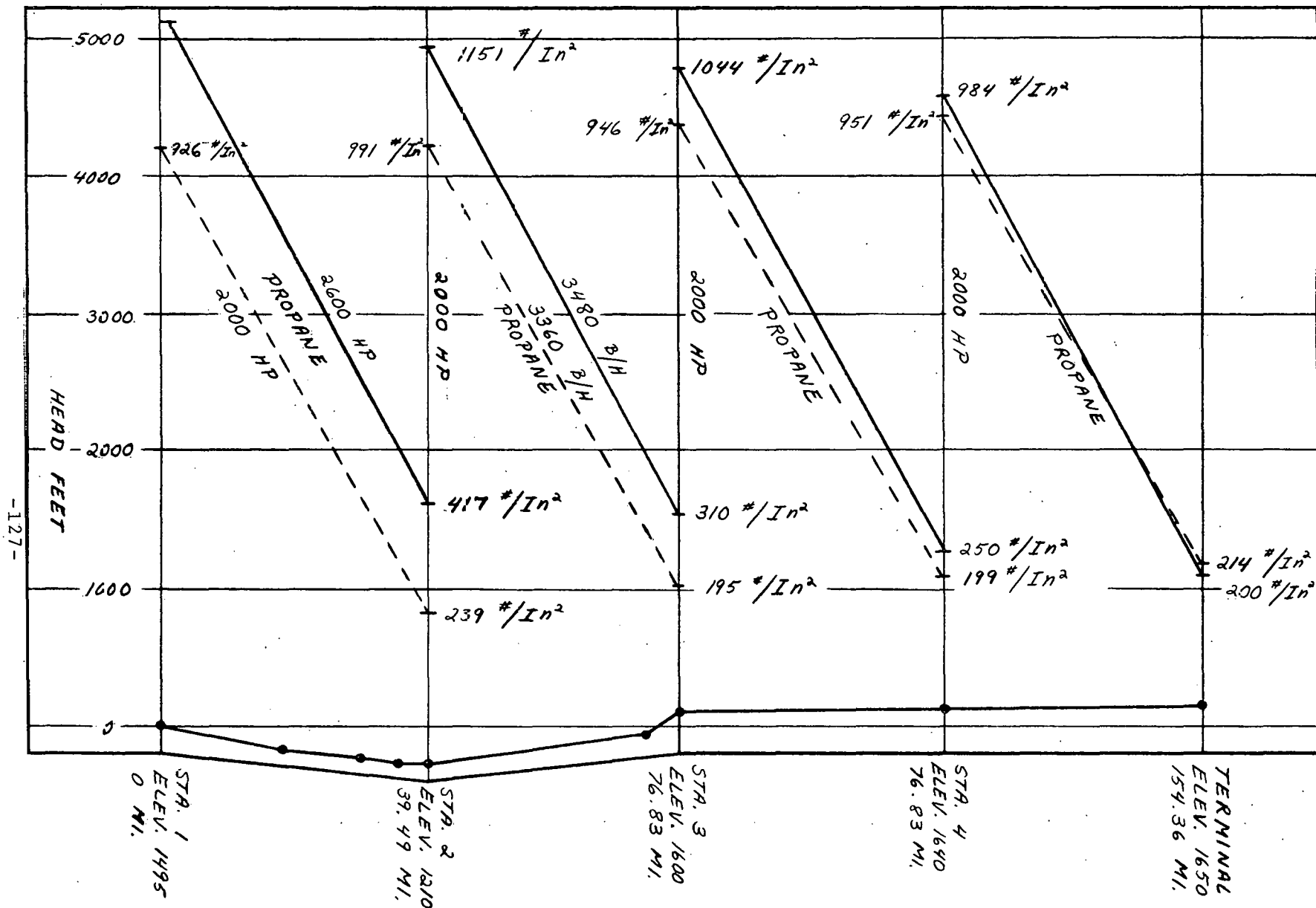
FIGURE 4.3.6.1.2-18 - HYDRAULIC GRADIENT, EIGHT/NINE PUMPS, ALL PROPANE
