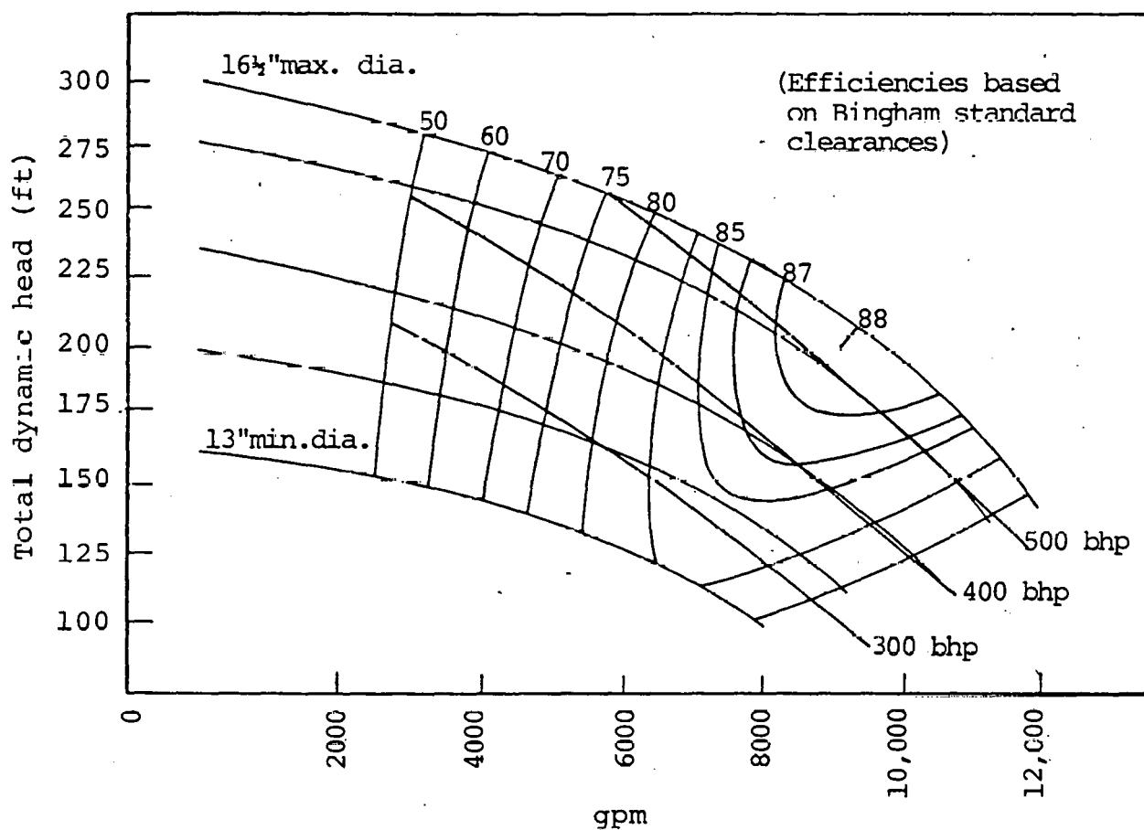
Fig. 7.1.1-3 - Efficiency curves for small commercial pipeline pump
