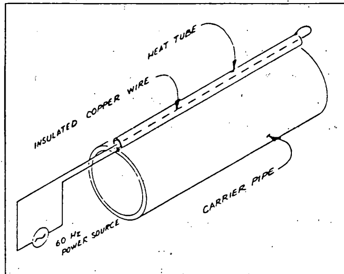
Figure 8.1-1 Basic skin effect tracing circuit.
