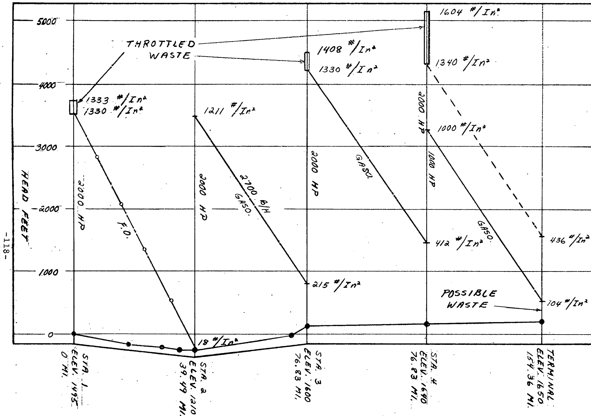
FIGURE 4.3.6.1:2-9 - HYDRAULIC GRADIENT, SEVEN/EIGHT PUMPS, ONE SEGMENT FUEL OIL, THREE SEGMENTS GASOLINE
