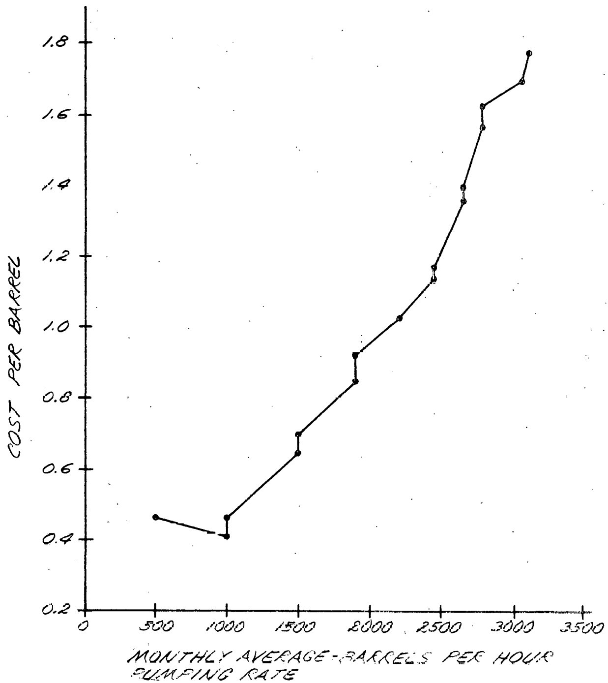
FIGURE 4.3.6.1.2-19 - POWER COST VS. THROUGHPUT
