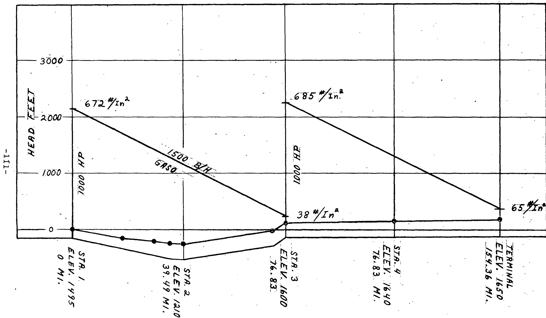
FIGURE 4.3.6.1.2-2 - HYDRAULIC GRADIENT, TWO PUMPS, ALL GASOLINE
