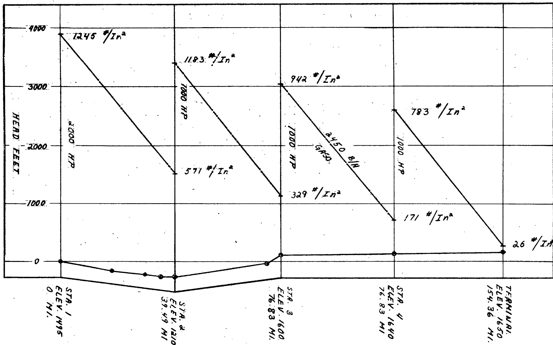
FIGURE 4.3.6.1.2-5 - HYDRAULIC GRADIENT, FIVE PUMPS, ALL GASOLINE
