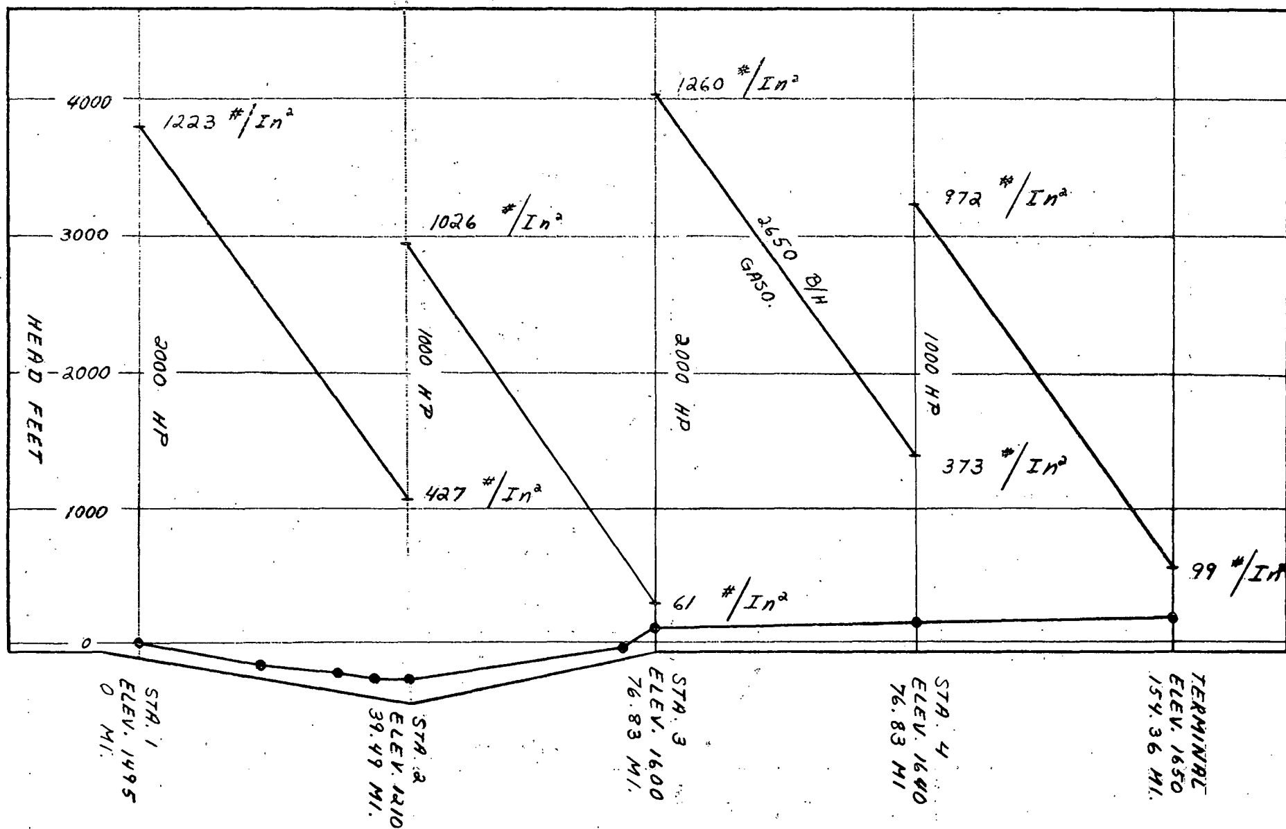
FIGURE 4.3.6.1.2-6 - HYDRAULIC GRADIENT, SIX PUMPS, ALL GASOLINE
