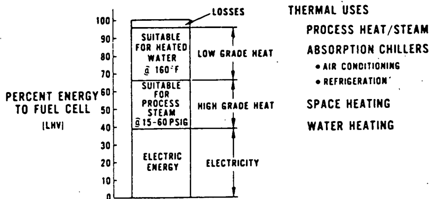
Fig. 4.3.2-4 - Waste heat recovery potential
