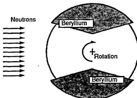
Figure 2. Schematic drawing of a T_0 chopper.
