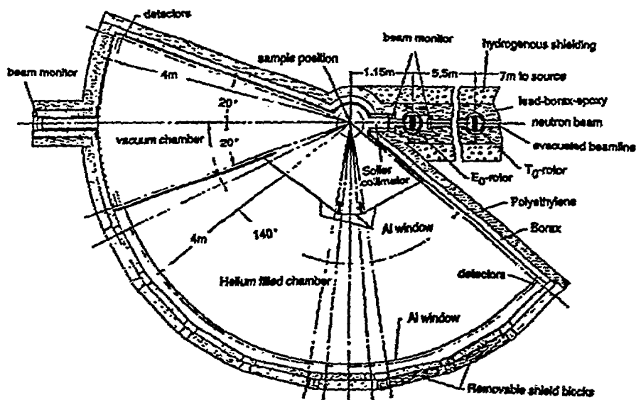
Figure 5. The High Resolution Medium Energy Chopper Spectrometer.
