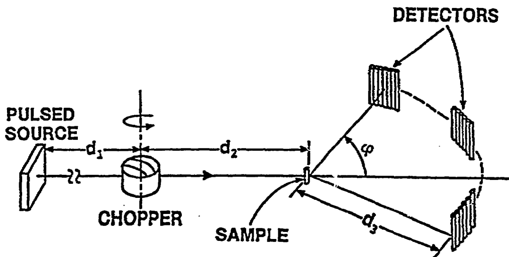
Figure 1. Schematic diagram of a pulsed source chopper spectrometer.
