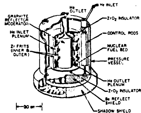
Fig. 6. Fluidized Bed Reactor
