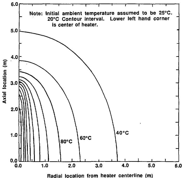
Figure 5. Temperature contours calculated for time of 13 weeks after start of thermal loading (after Montan, 1986).
