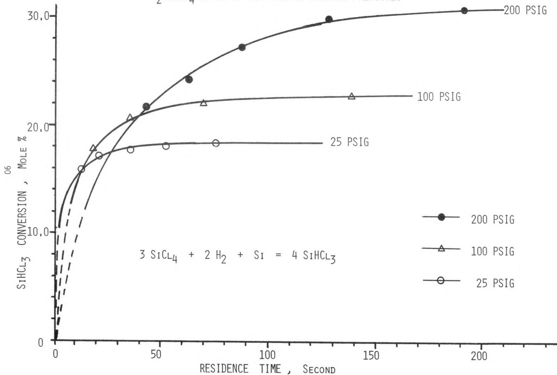
FIGURE XIII HYDROCHLORINATION OF \text{SiCl}_4 AND M.G. SILICON AT 500^\circ\text{C} , \text{H}_2/\text{SiCl}_4 RATIO OF 2.0 AND AT VARIOUS PRESSURES
