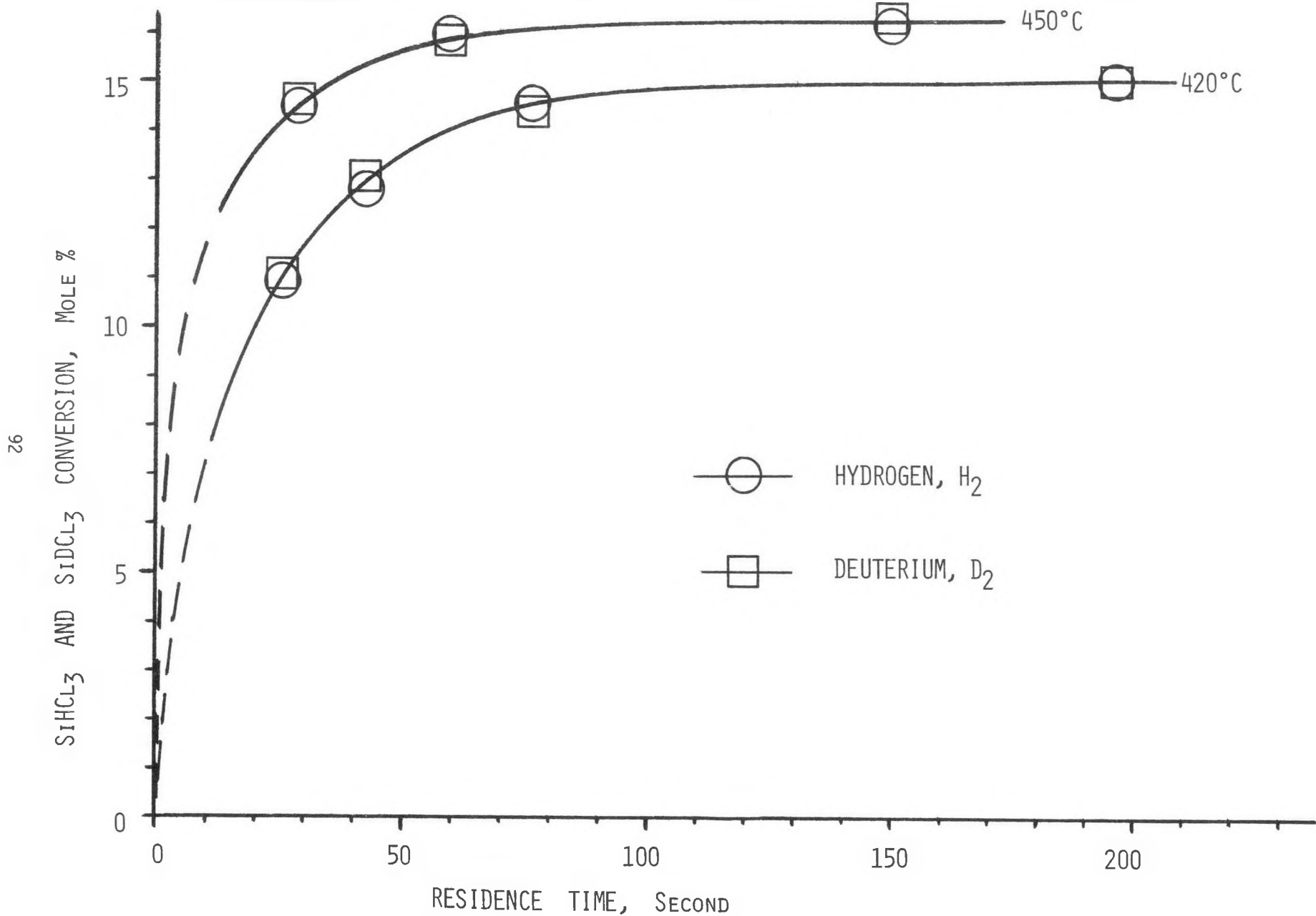
FIGURE XV PLOT OF % \text{SiHCl}_3 AND % \text{SiDCl}_3 CONVERSION VERSUS RESIDENCE TIME
