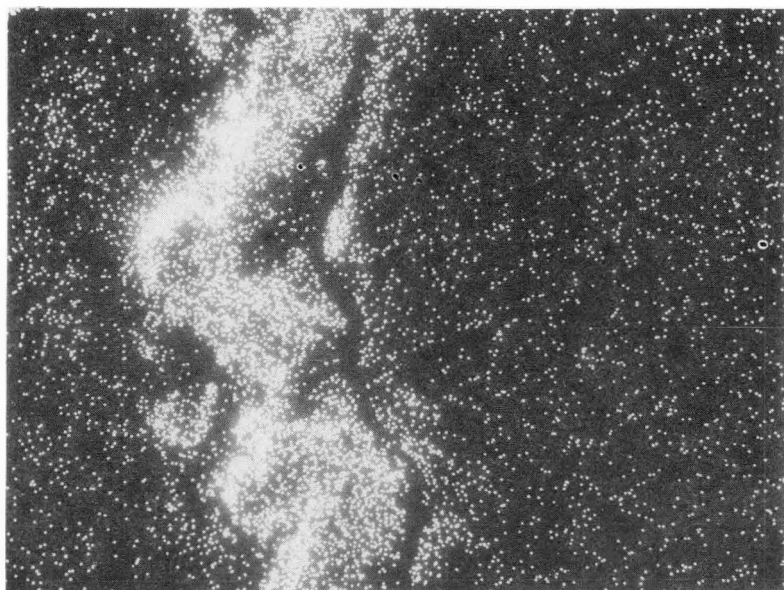
Silicon X-ray Distribution Photo 8 40000
