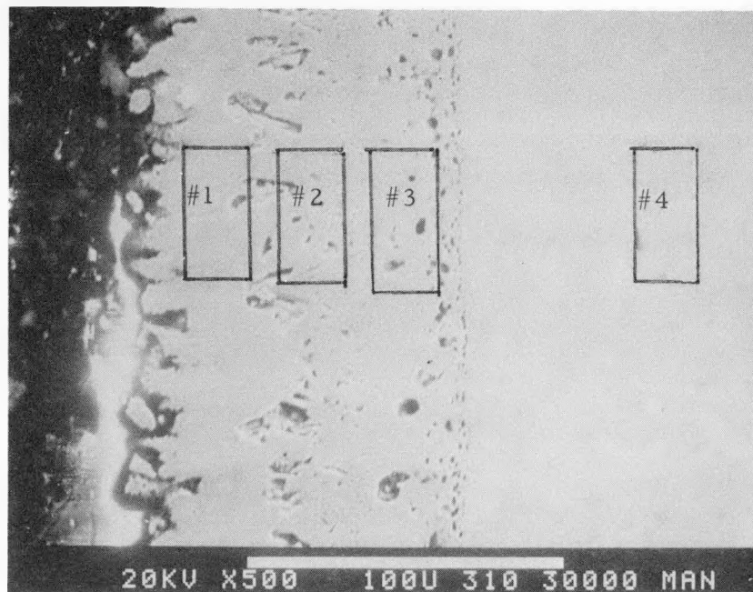
FIGURE XVIII SCANNING ELECTRON MICROGRAPH AND X-RAY DISTRIBUTION MAPS OF THE CORROSION TEST SAMPLE ON NICKEL
