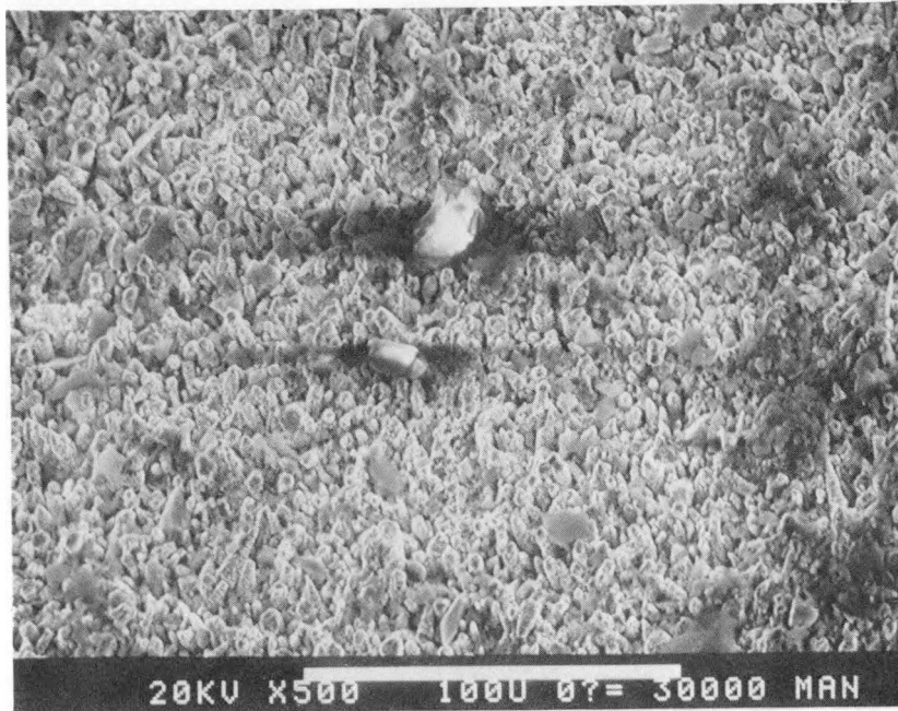
FIGURE XVI CORROSION TEST ON PURE NICKEL: 87 HOURS AT 500°C, 300 PSIG AND H_2/SiCl_4 RATIO OF 2.0
