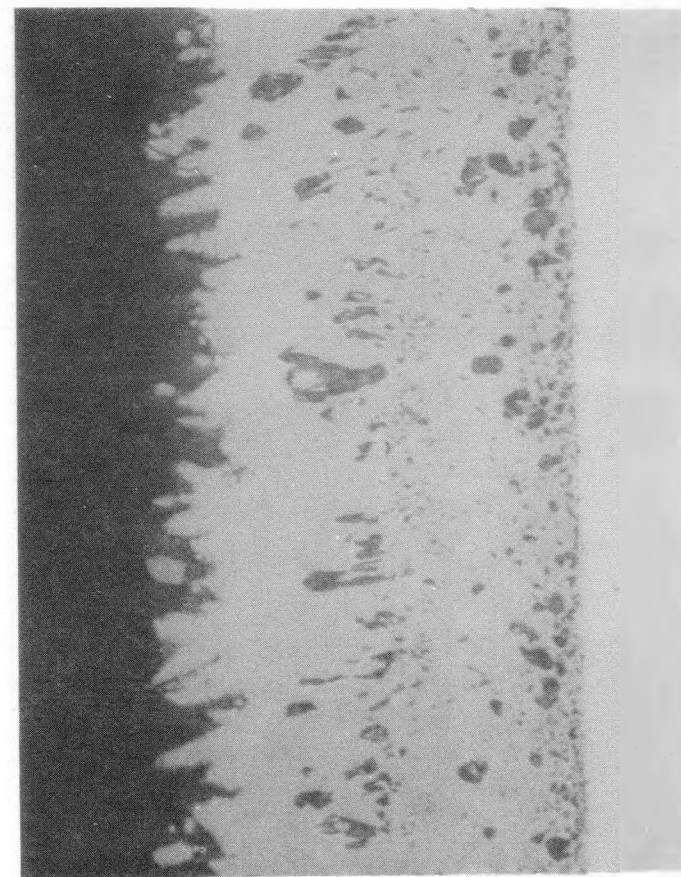
#3 Silicon on Nickel 500 X
