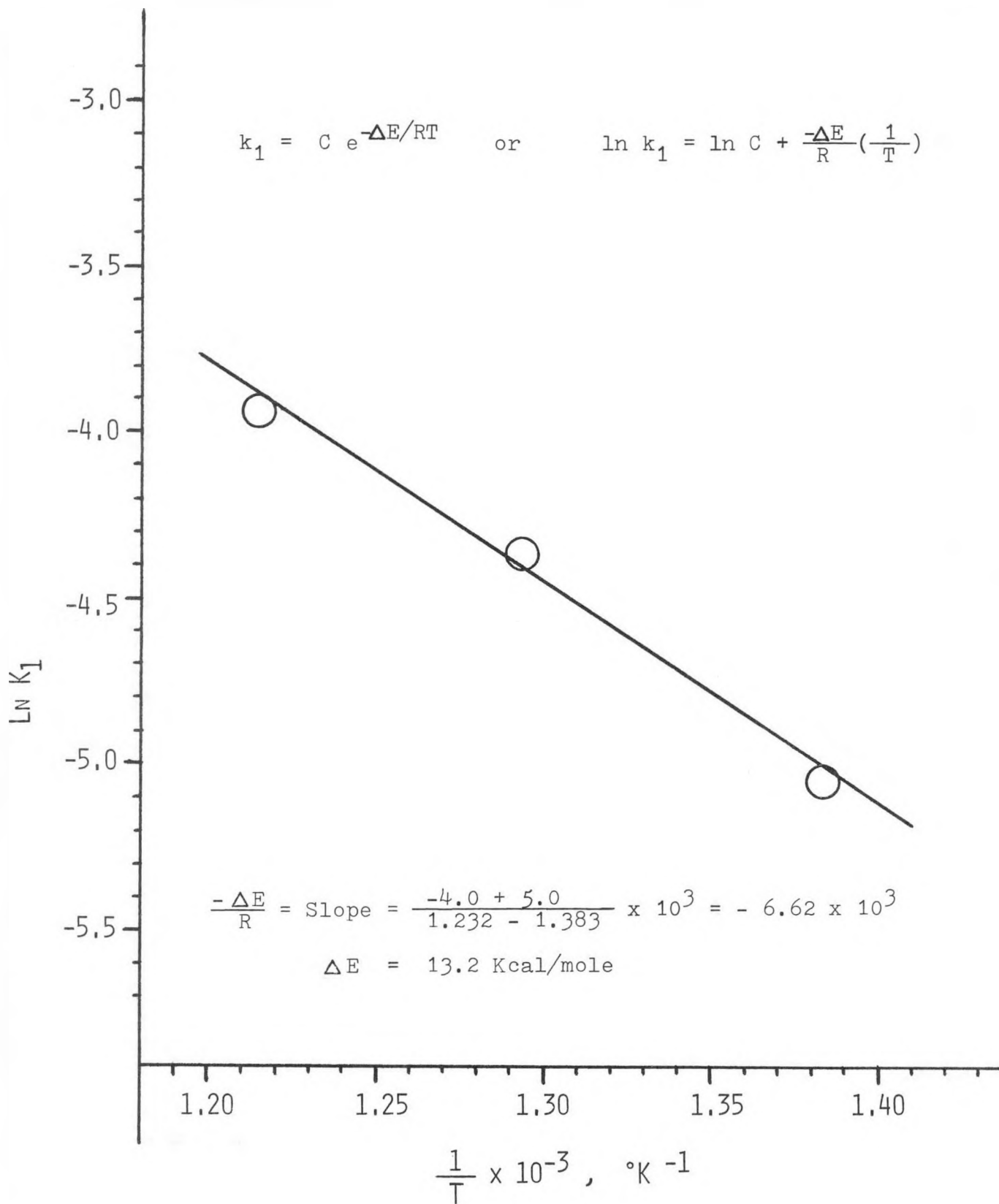
FIGURE XII PLOT OF THE ARRHENIUS EQUATION
