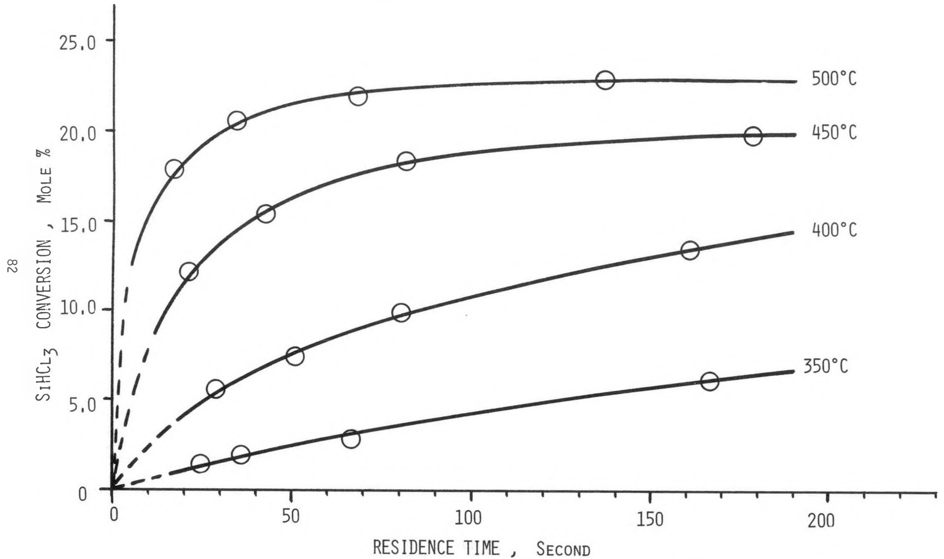
FIGURE V THE EFFECT OF TEMPERATURE ON THE HYDROCHLORINATION OF \text{SiCl}_4 AND M.G. SILICON AT 100 PSIG AND \text{H}_2/\text{SiCl}_4 MOLAR RATIO OF 2.0
