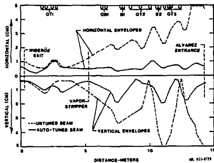
Fig. 5: Beam transmission envelopes through the MEBT both before and after a test of the auto-tuning program for 94\text{Nb}^{3+70+} .
