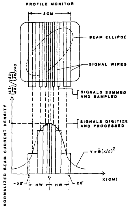
Fig. 3: Derivation of profile measurements from the raw data generated when beam is intercepted by multi-wire monitors.
