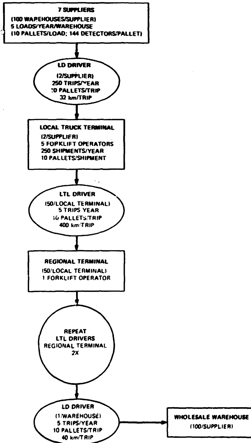
Fig. 3. Flow chart for the transport of 5 million smoke detectors from the supplier to a wholesale warehouse.
