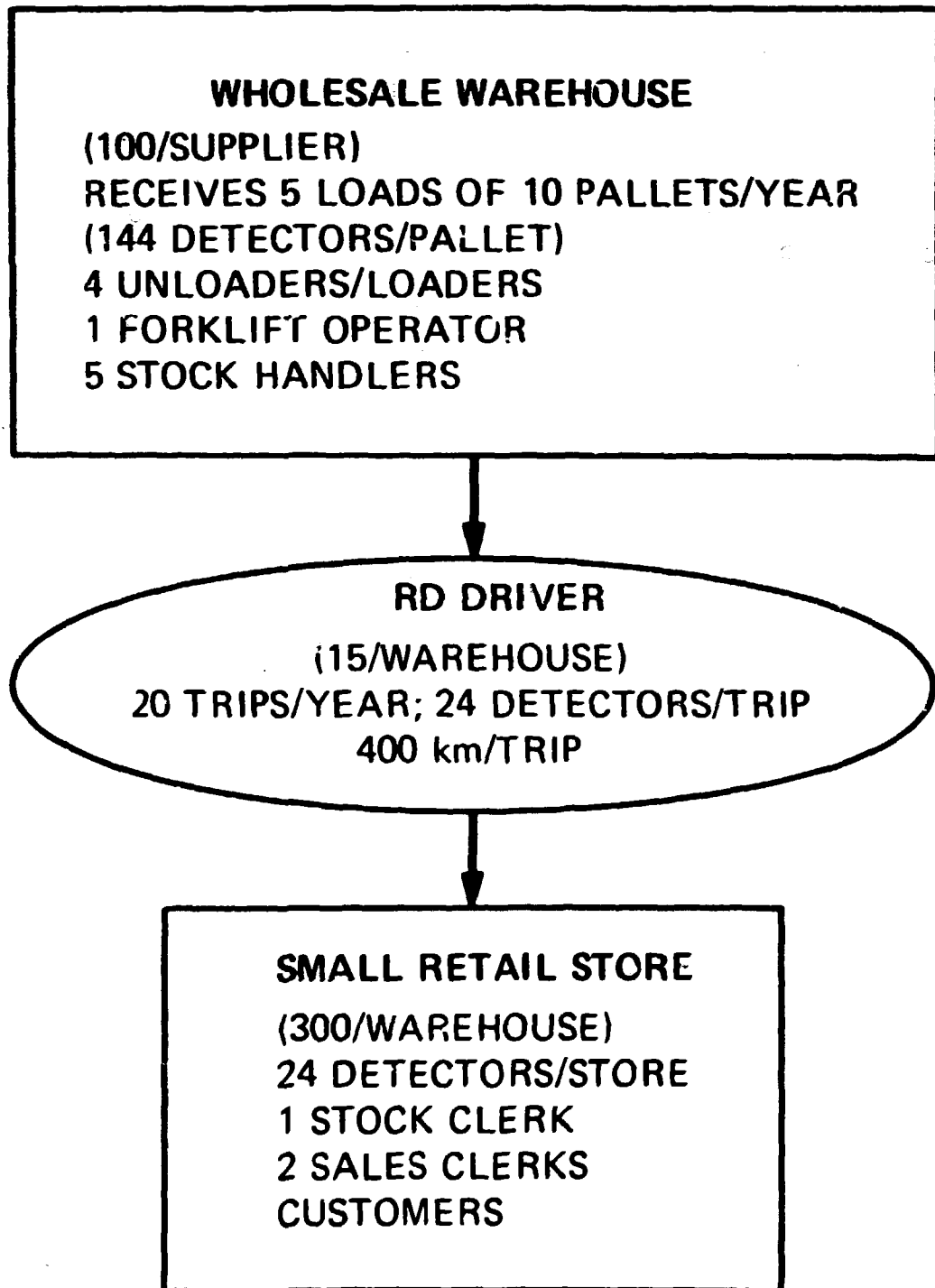
Fig. 5. Flow chart for the distribution of smoke detectors from a wholesale warehouse to small retail stores.
