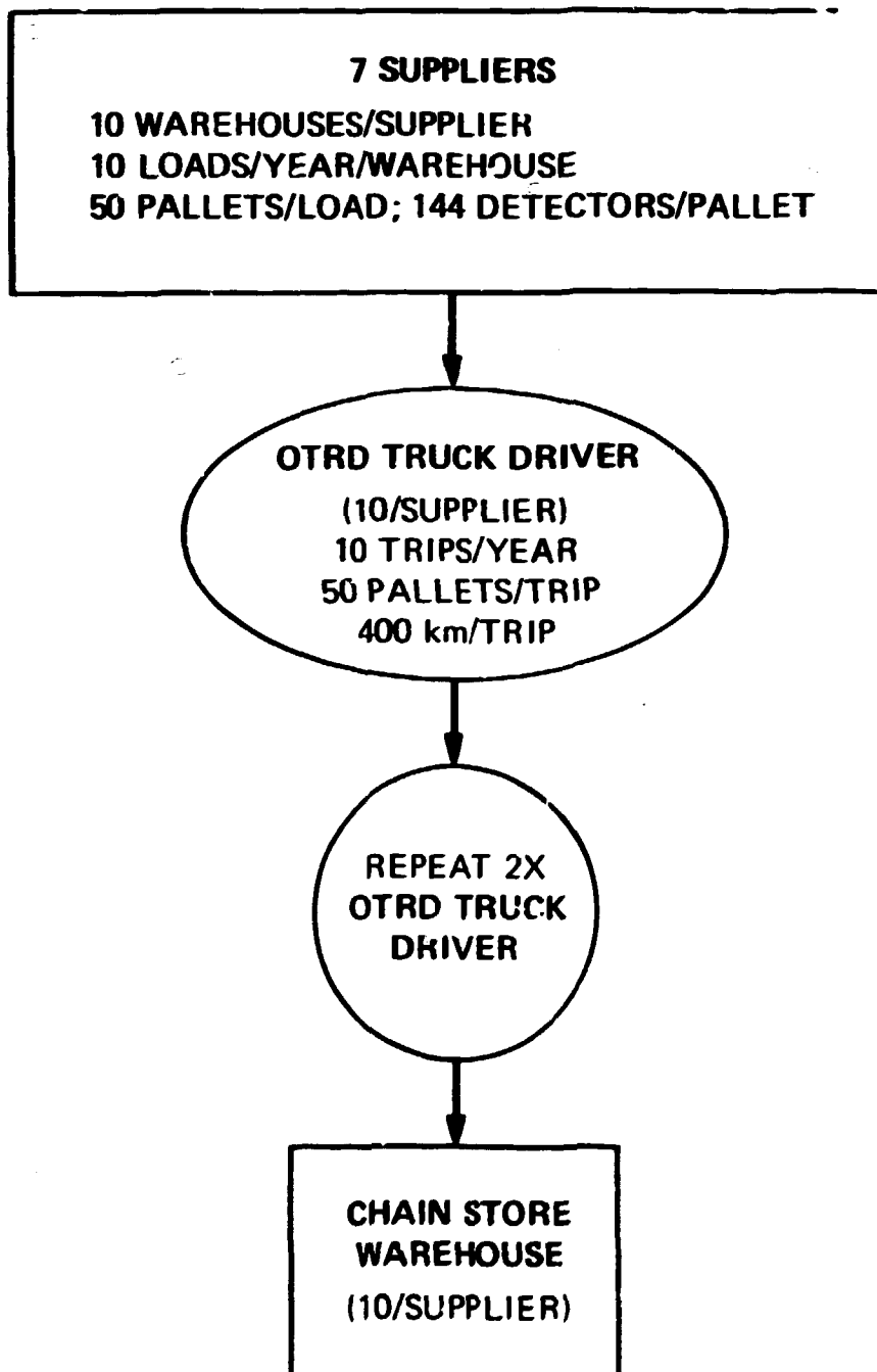
Fig. 2. Flow chart for the transport of 5 million smoke detectors from the supplier to a chain store warehouse.
