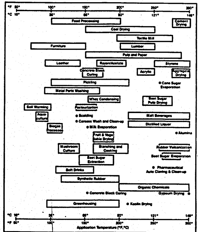
Fig. 11. Application temperature range for some industrial processes and agricultural applications (Anderson and Lund, 1979).
