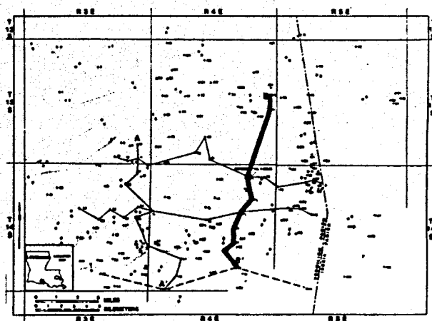
Fig. 4. Location of cross section B-B1 (UTA).
