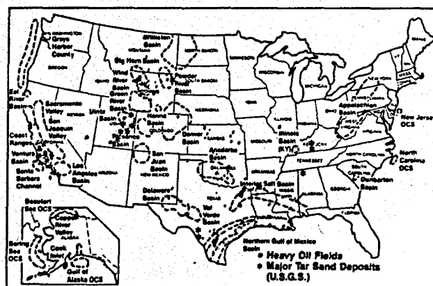
Fig. 1. Index map of geopressure locations with heavy oil and tar sands (Modified after Strongin, 1981; Meyer U.S.G.S., 1989)
