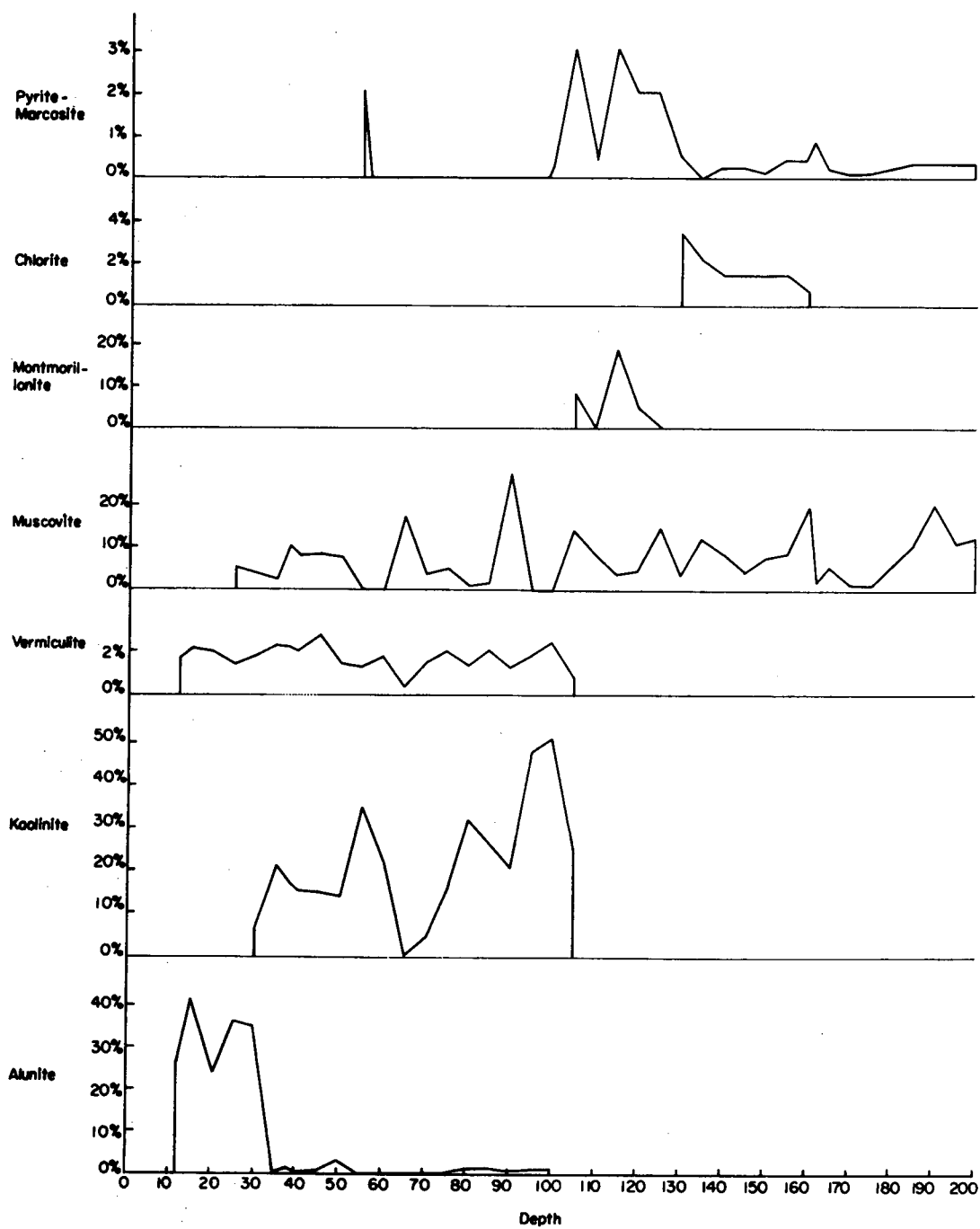
Figure 5. Major Alteration Mineralogy (MODECALC) versus Depth.
