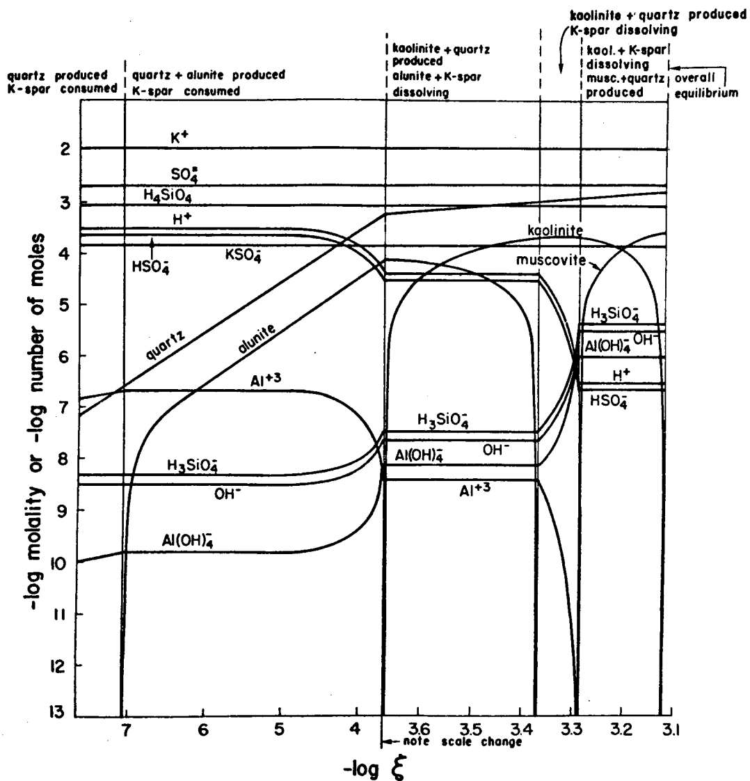
Figure 9. Reaction path for the dissolution of microcline at 100^\circ\text{C} and initial solution pH = 3.6 (Dedolph and Parry, 1976).
