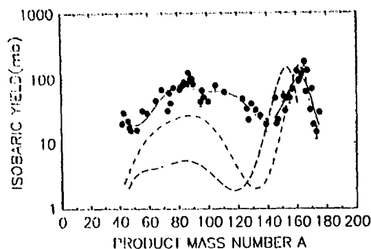
Figure 1. Isobaric yield distributions for the fragmentation of ^{163}\text{Ho} by (a) 12 MeV/nucleon ^{32}\text{S} , solid points, solid line (b) 17 MeV/nucleon ^{16}\text{O} , short dashed line (c) 442 MeV ^{12}\text{C} , long dashed line.
