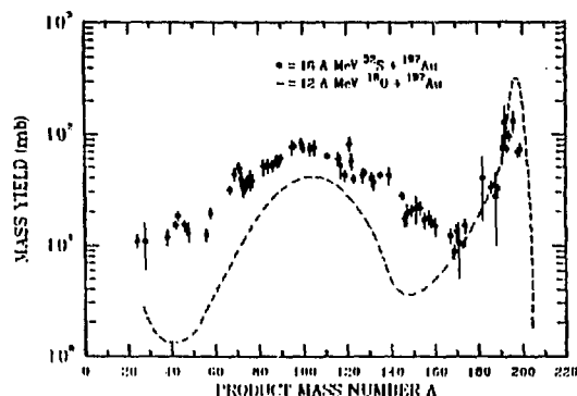
Figure 2. Comparison of isobaric yield distributions for the fragmentation of ^{197}\text{Au} by (a) 12 MeV/nucleon ^{16}\text{O} , dashed line and (b) 16 MeV/nucleon ^{32}\text{S} .
