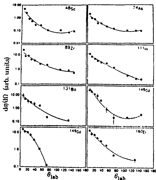
Figure 3. Laboratory frame angular distributions for representative fragments from the reaction of 16 MeV/nucleon ^{32}\text{S} with ^{164}\text{Ho} .
