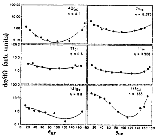
Figure 6. Moving frame angular distributions for representative fragments from the interaction of 16 MeV/nucleon 32 S with 163 Ho.
