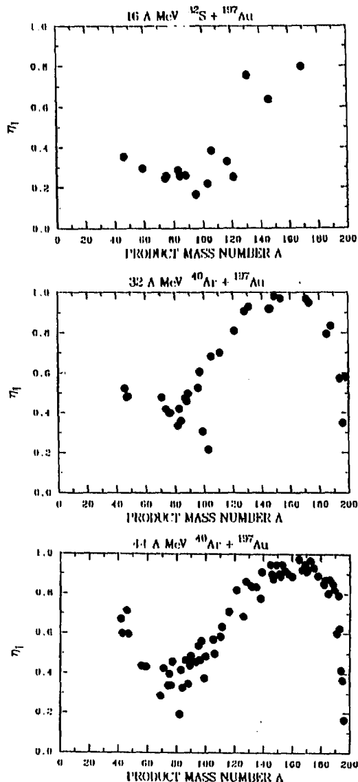
Figure 5. Values of \eta_1 as a function of product mass number for all the reactions involving Au targets.
