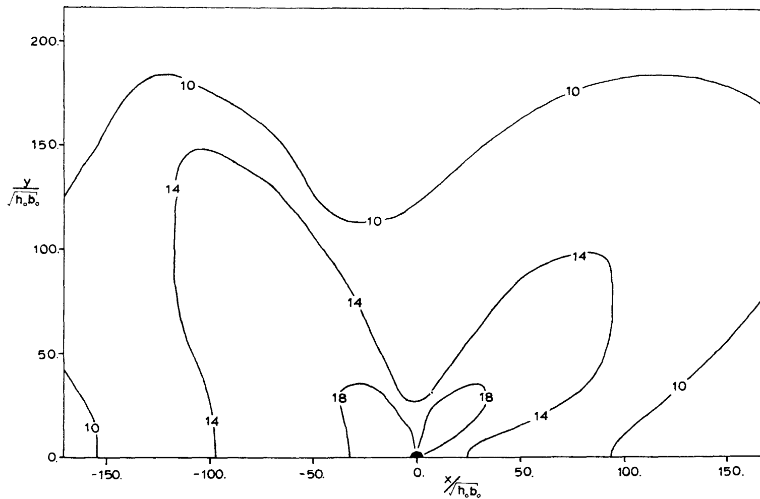
Figure A.2.1 Plan View. Run #10
