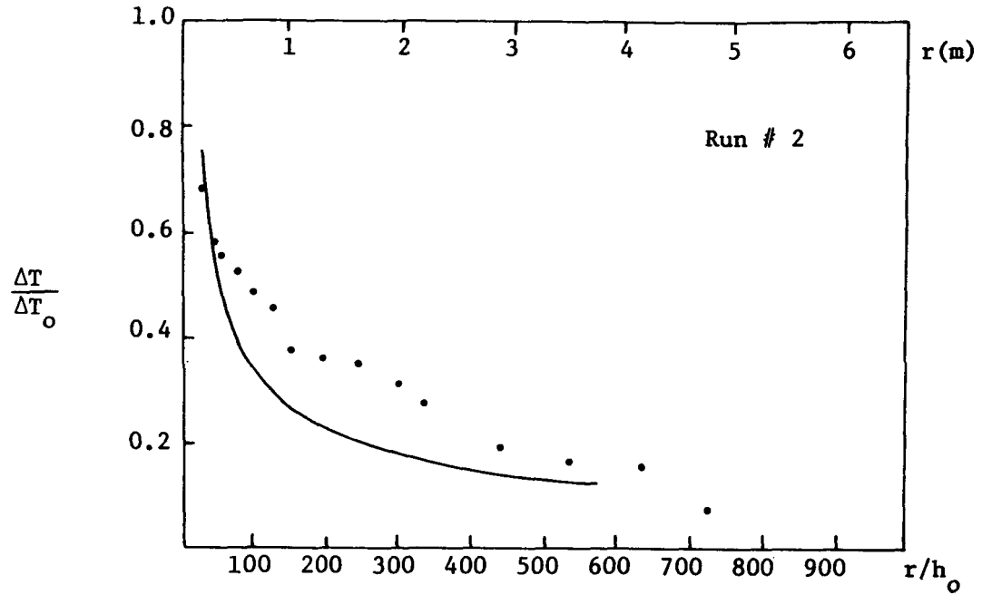
Figure 7.11a Temperature vs. Distance, Experimental Comparison to Model
