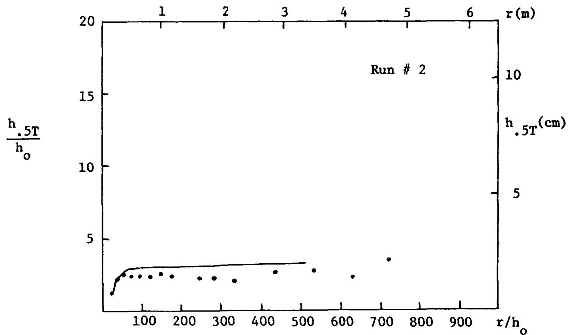
Figure 7.11b Half-Temperature Depth vs. Distance, Experimental Comparison to Model
