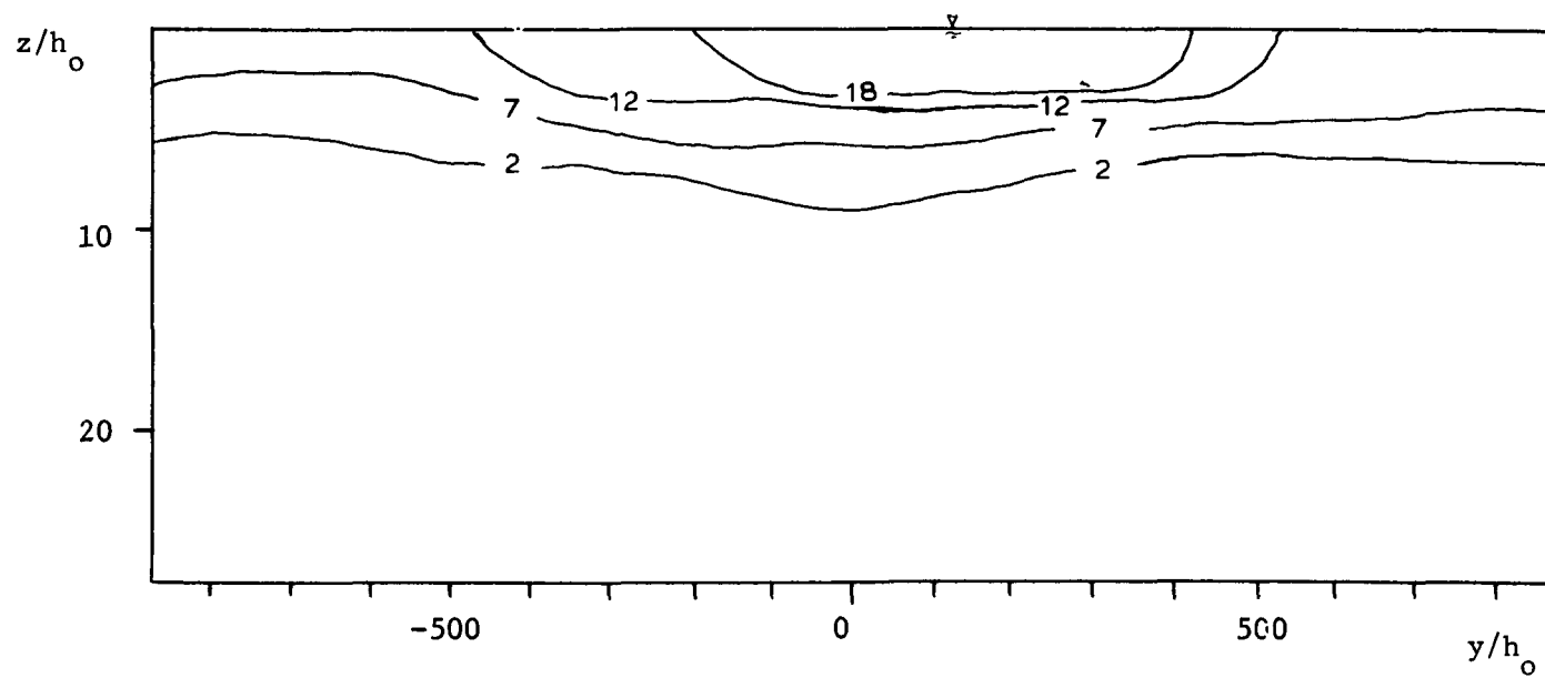
Figure A.3.27 Lateral Transect B-B at x = -4\text{m} , Run #32.
