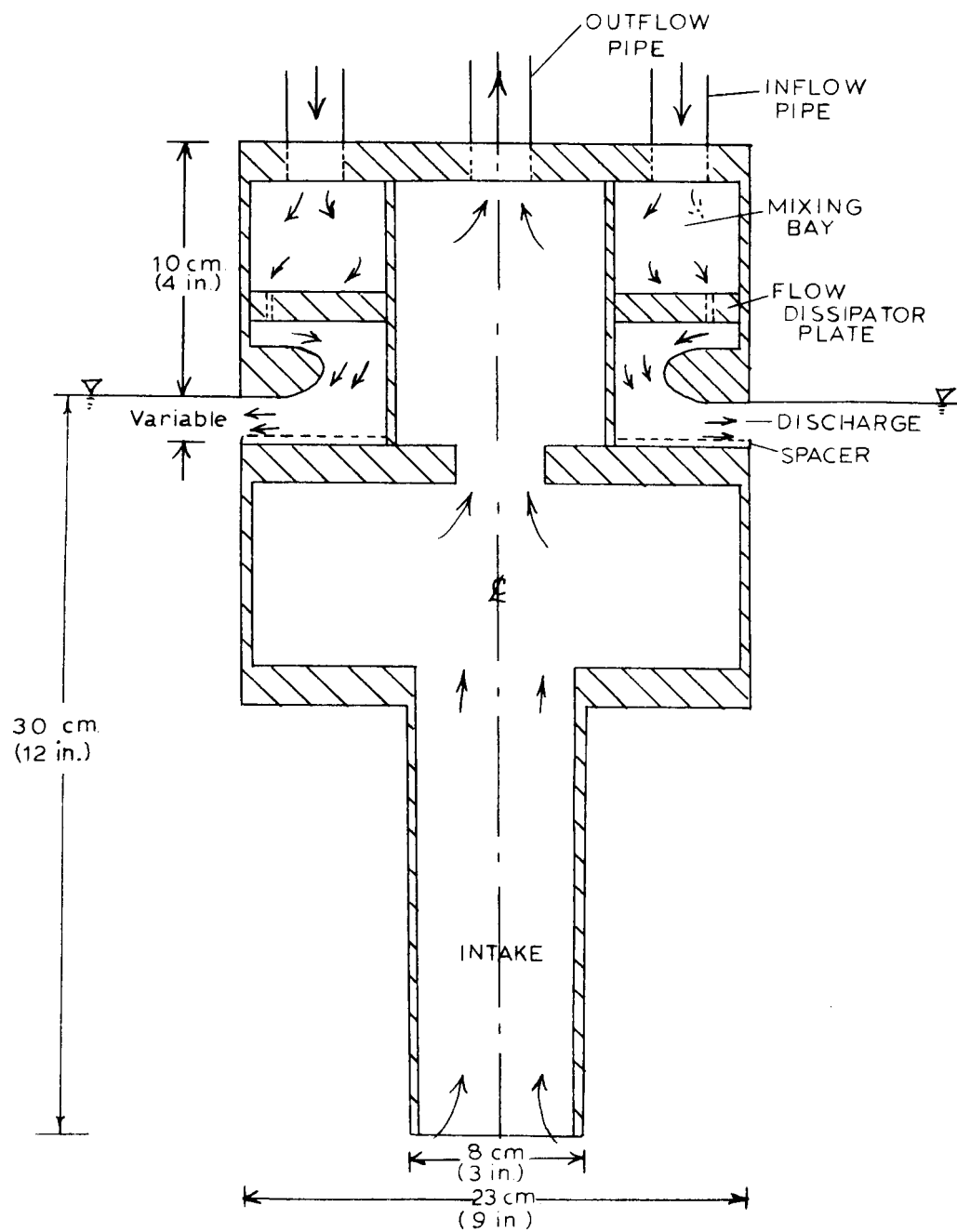
Figure 3.1 Schematic Diagram of the Plexiglass Model
