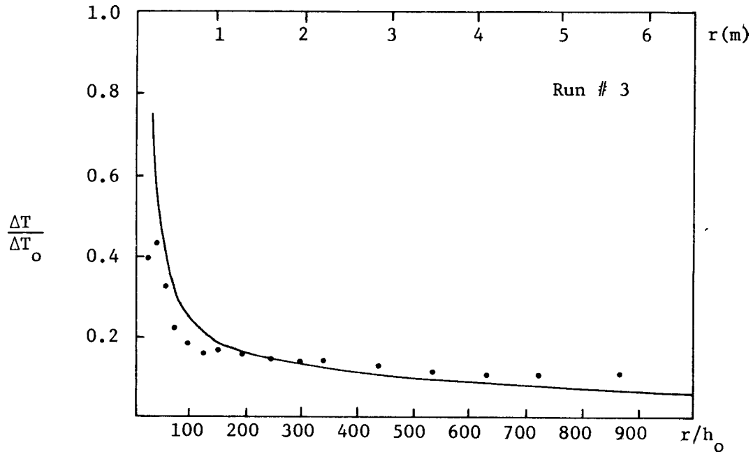
Figure 7.12a Temperature vs. Distance, Experimental Comparison to Model
