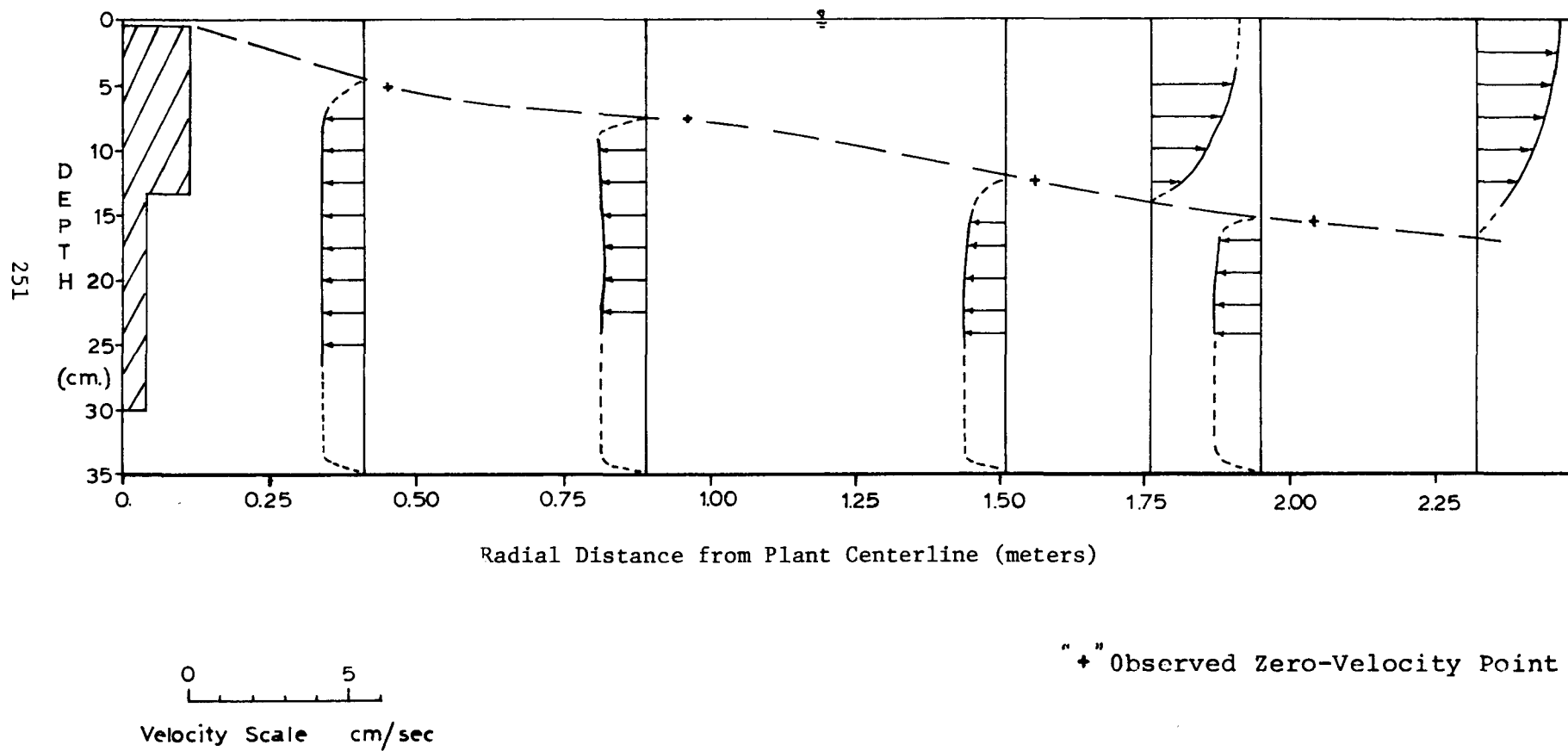
Figure B.3 Photographic Velocity Measurements, Exp #56
