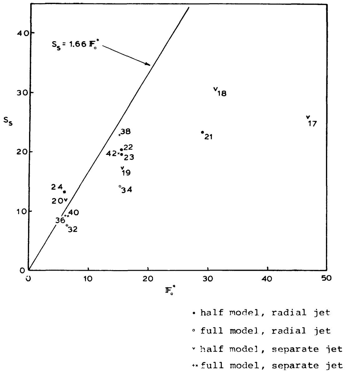
Figure 6.4 Stable Downstream Dilution vs. Quarter Module "Port" Discharge Froude Number, Ambient Current Experiments
