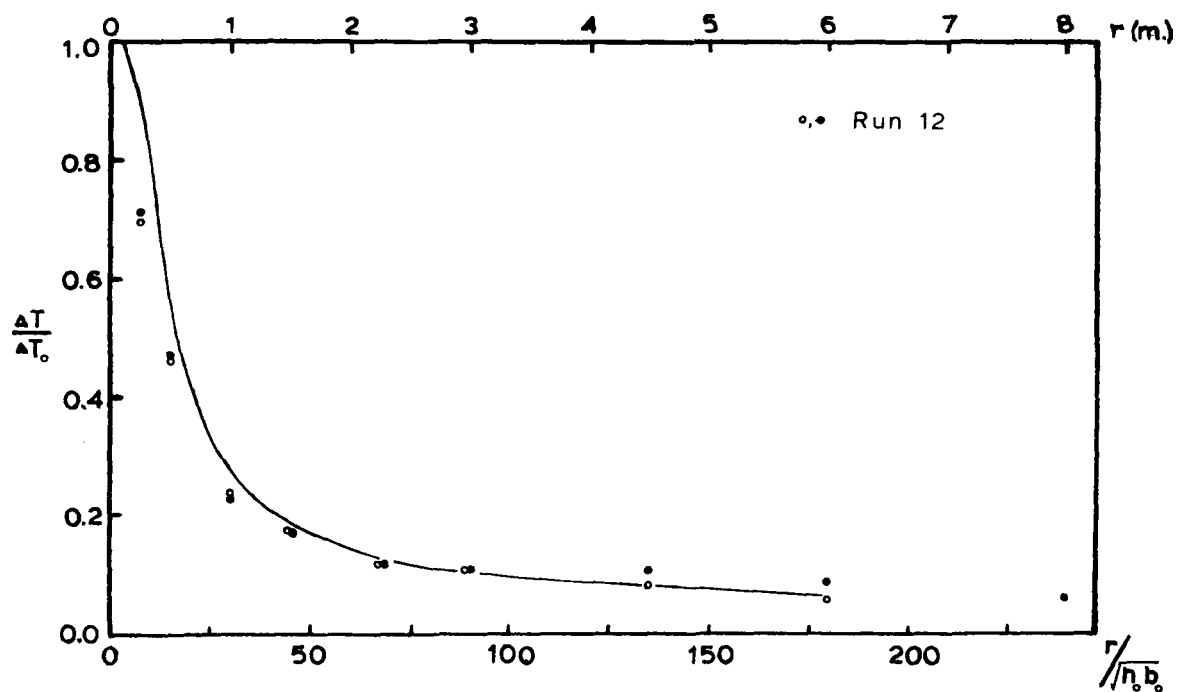
Figure 8.11a Temperature vs. Distance, Experimental Comparison to Model
