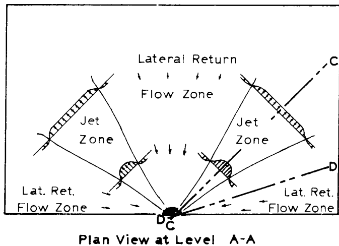
Figure 5.1 Flow Zones for Separate Jet Configuration
