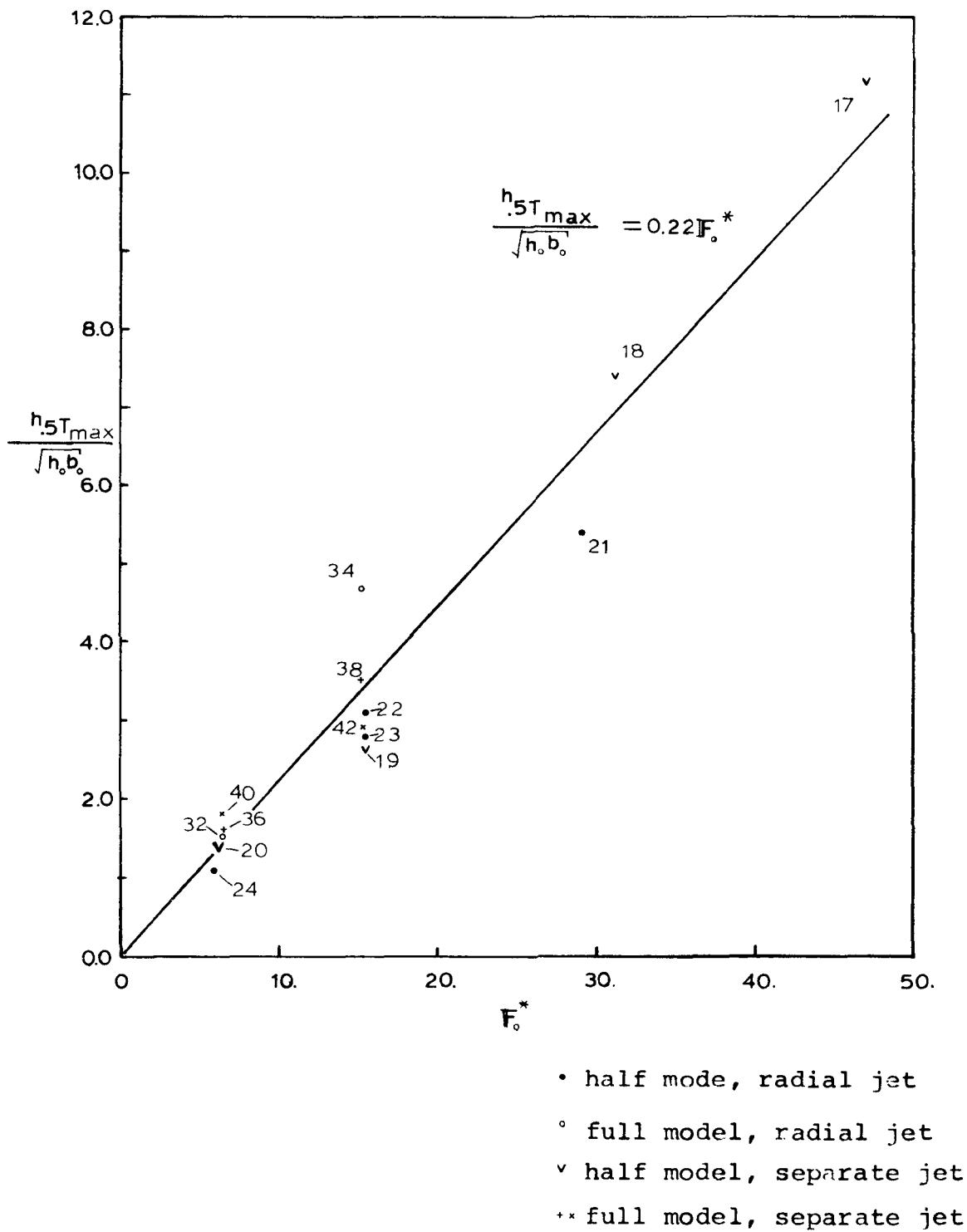
Figure 6.5 Maximum Half Temperature Depth vs. Quarter Module "Port" Discharge Froude Number; Ambient Current Experiments
