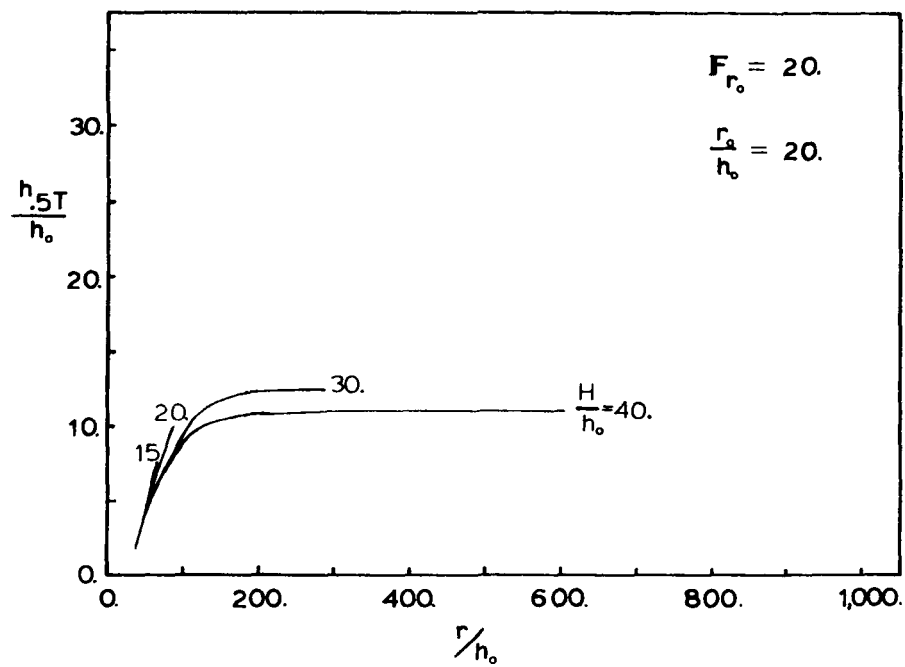
Figure 7.4b Half Temperature Depth vs. Distance, Varying H/h_o .
