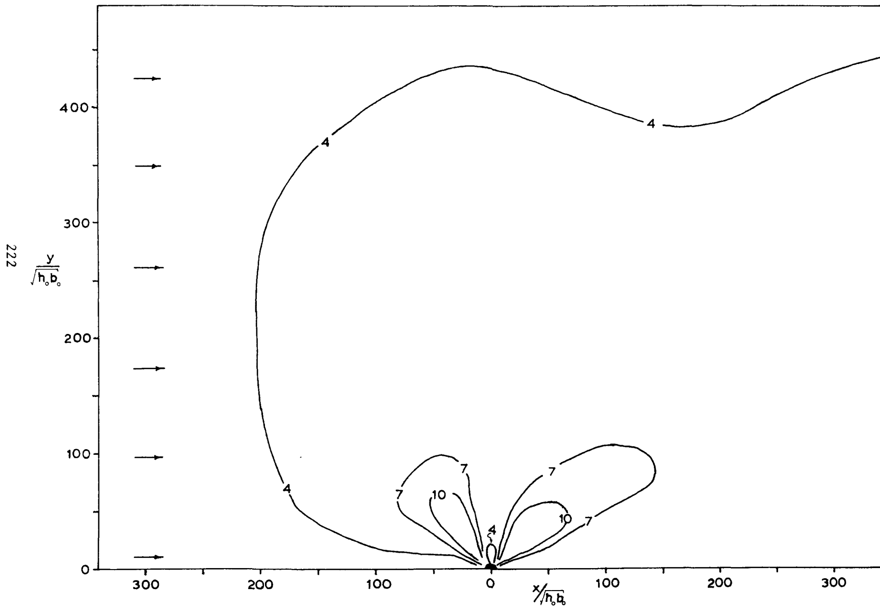
Figure A.3.4 Plan View. Run #18, Separate Jet Discharge
