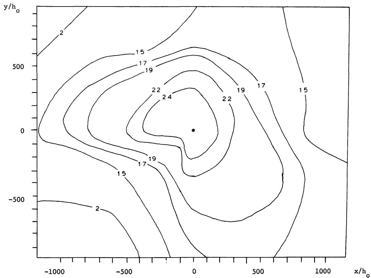
Figure A.3.25 Surface Plan, Rur #32, Radial Jet Discharge.
