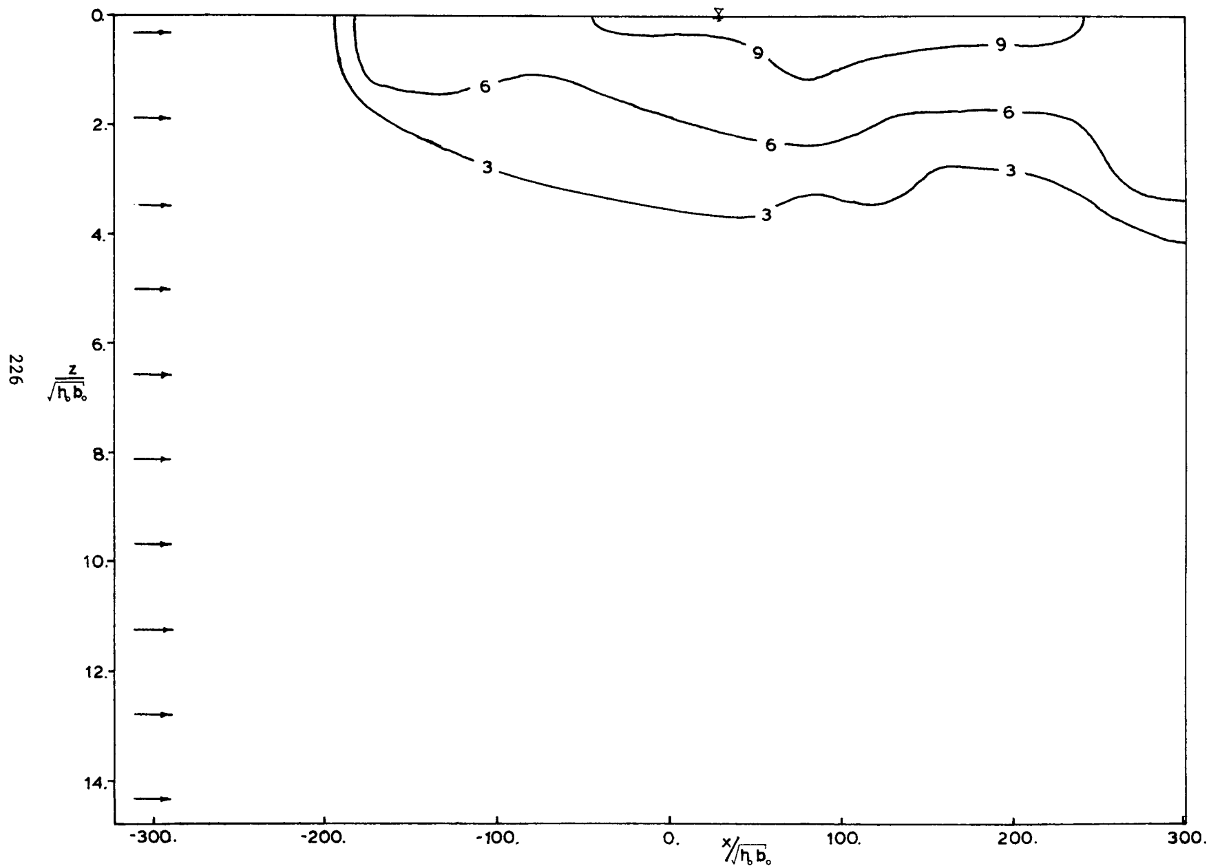
Figure A.3.8 Longitudinal Transect A-A at y = 2.25\text{m} , Run #19.
