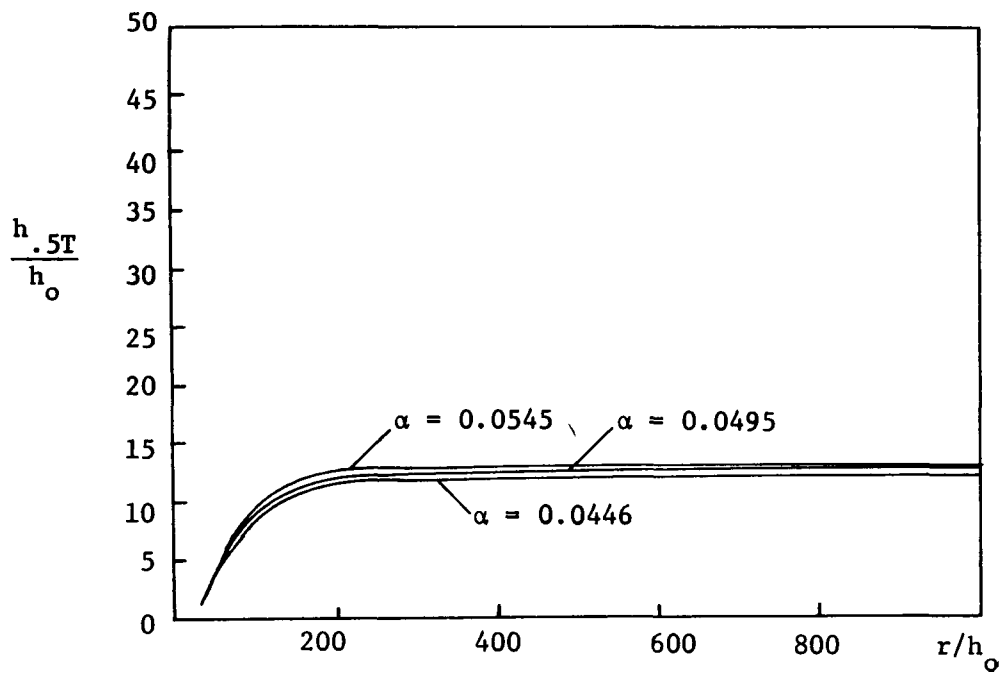
Figure 7.5b Half-Temperature Depth vs. Distance, Varying \alpha
