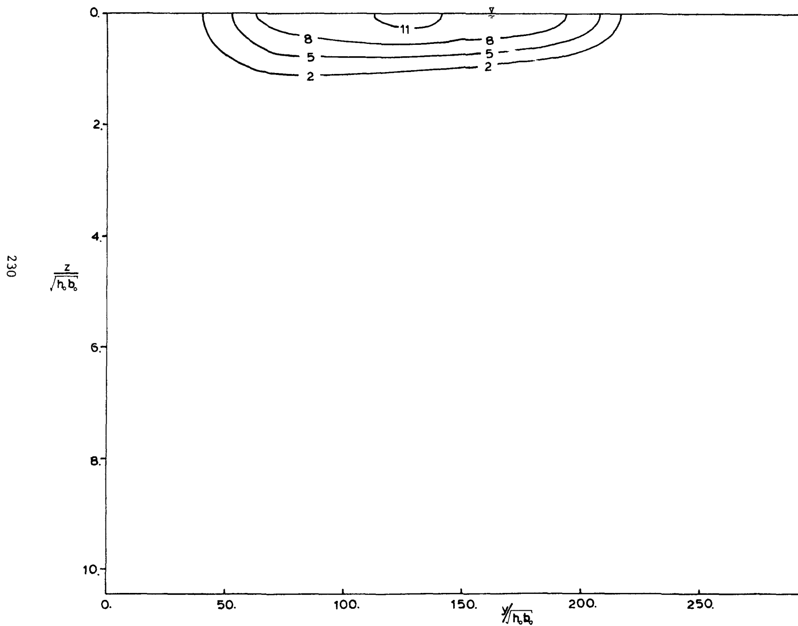
Figure A.3.12 Lateral Transect B-B at x = -5.5\text{m} , Run #20.
