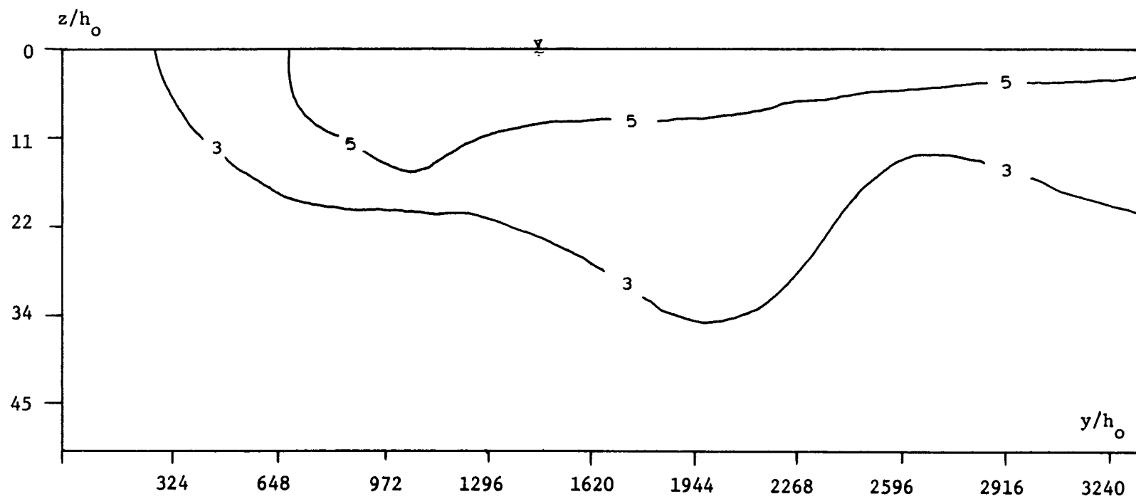
Figure A.3.15 Lateral Transect E-B at x = -4.0\text{m} , Run #21.
