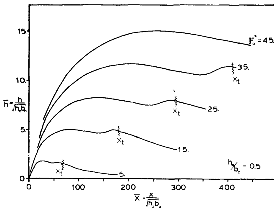
Figure 8.4b Jet Depth vs. Distance, Varying F_o^*
