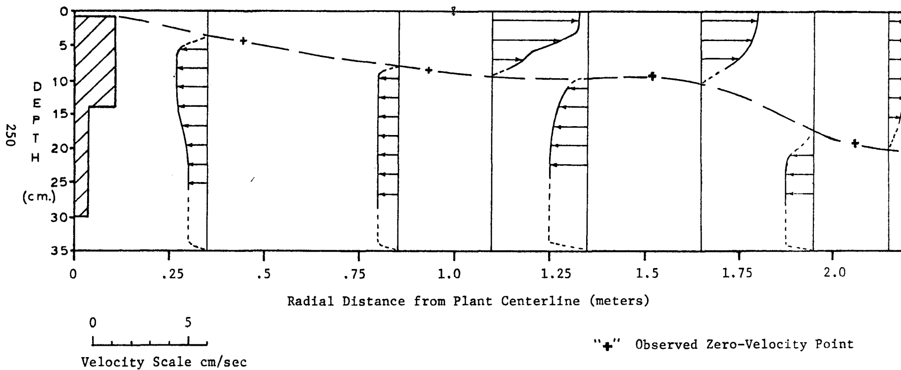
Figure B.2 Photographic Velocity Measurement Exp #51
