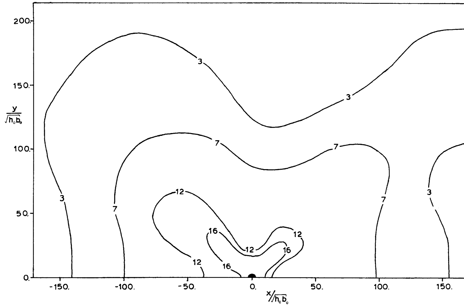
Figure A.2.7 Plan View. Run #12.
