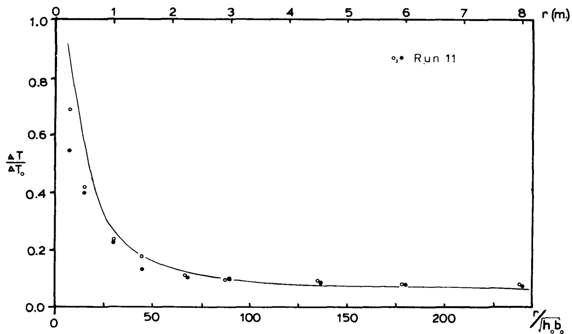
Figure 8.10a Temperature vs. Distance, Experimental Comparison to Model
