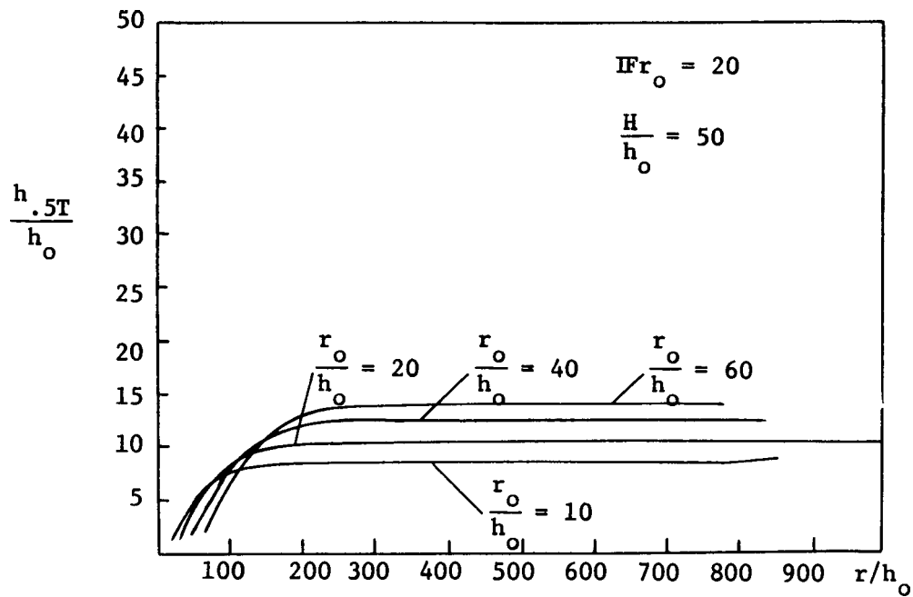
Figure 7.3b Half-Temperature Depth vs. Distance, Varying r_o/h_o
