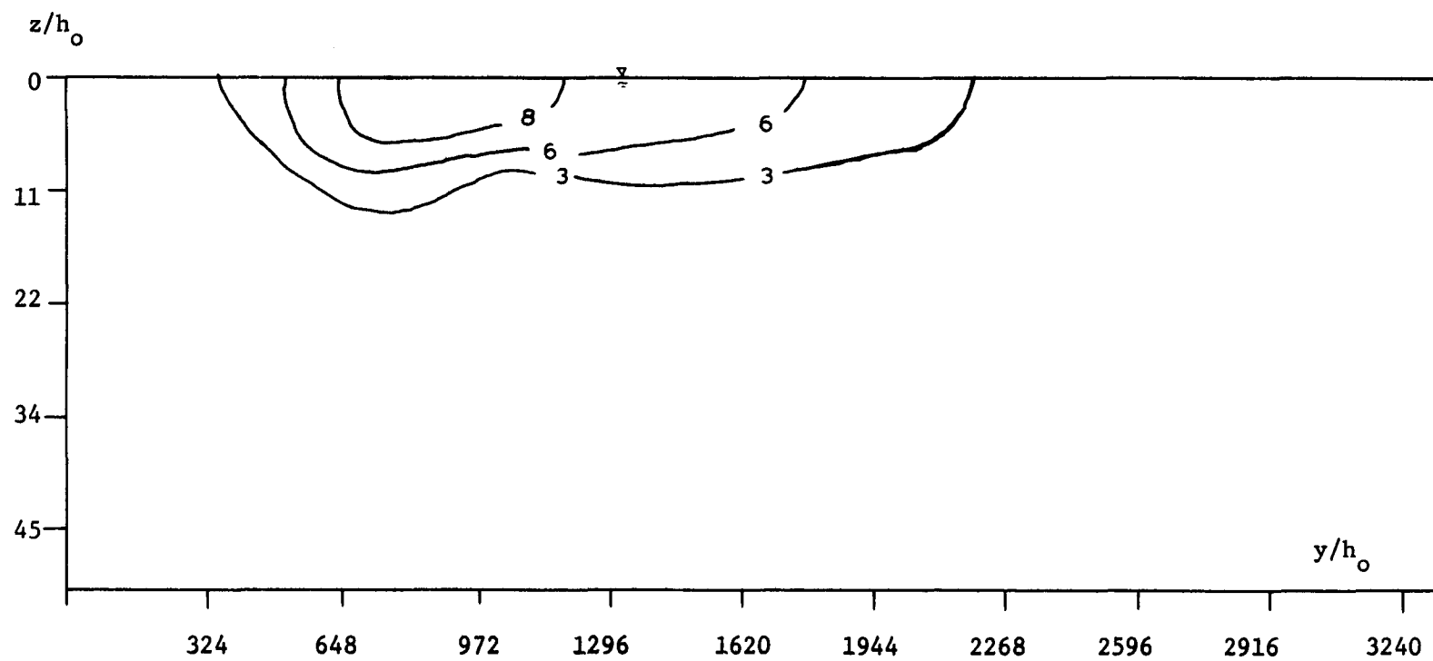
Figure A.3.21 Lateral Transect B-B at x = -4\text{m} , Run #23.
