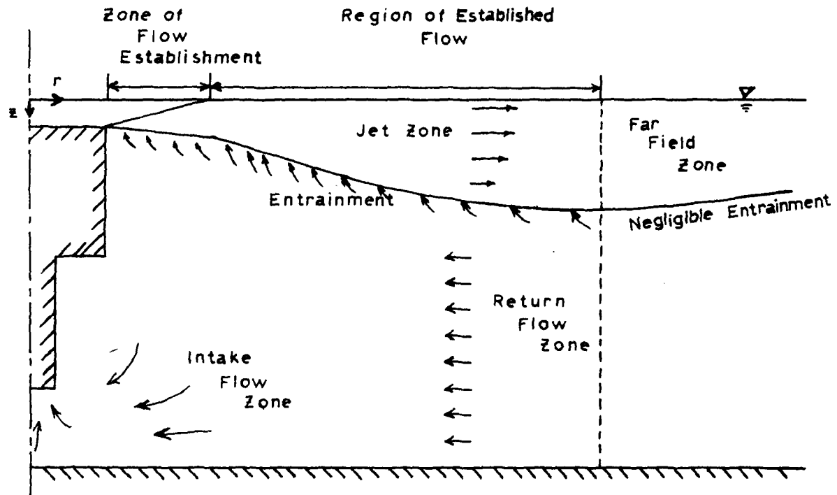
Figure 7.1 Schematic Diagram of the Induced External Flow Field.
