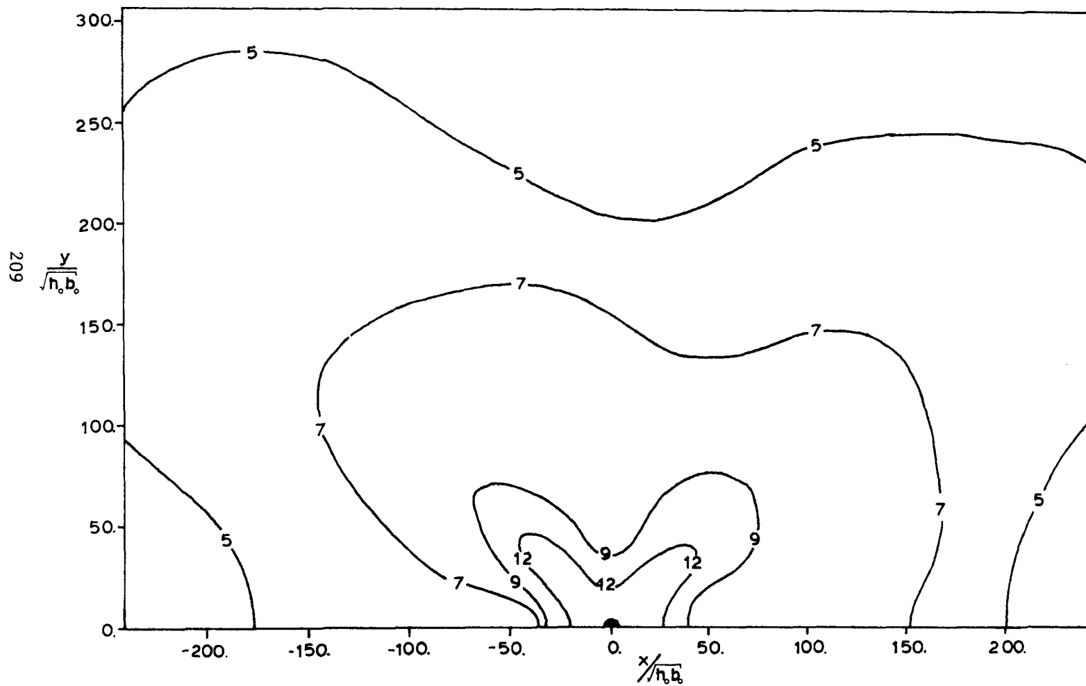
Figure A.2.10 Plan View. Run #13.
