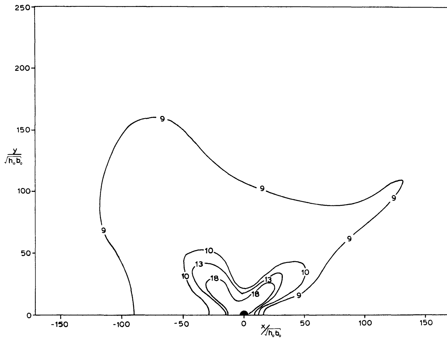
Figure A.2.4 Plan View. Run #11.
