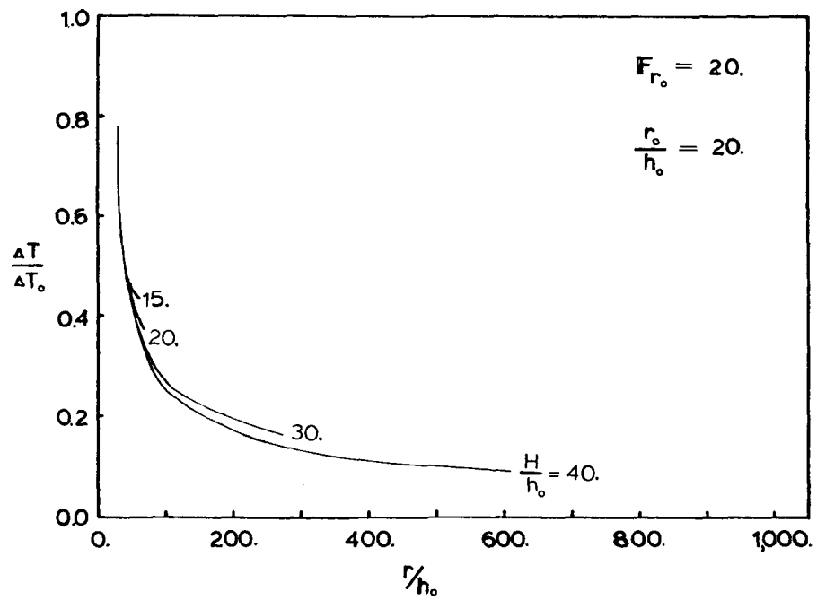
Figure 7.4a Temperature vs. Distance, Varying H/h_o .
