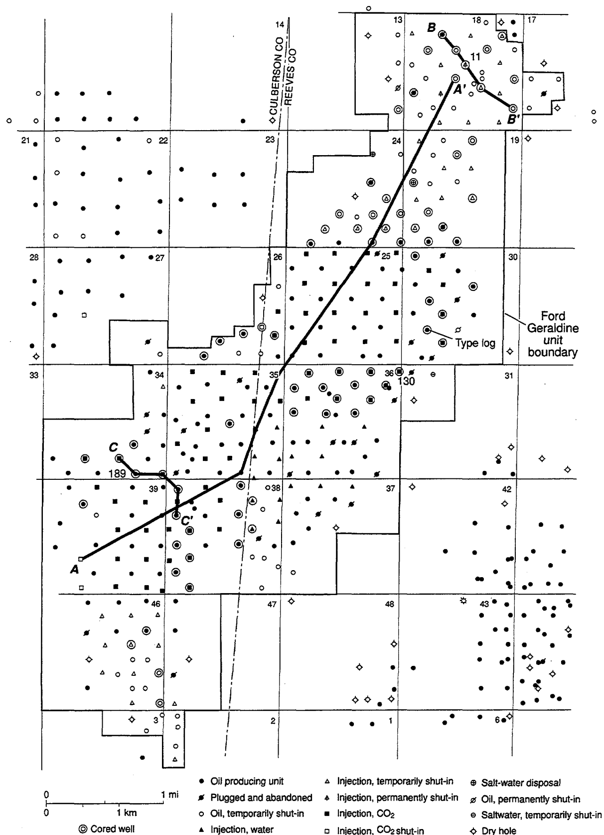
Figure 2. Status of wells in the Ford Geraldine unit and distribution of core control. Type log is shown in figure 5, cross section A-A' in figure 20, cross section B-B' in figure 26, and C-C' in figure 27. Core descriptions of the three wells identified by number (11, 130, and 189) are shown in figure 28.
