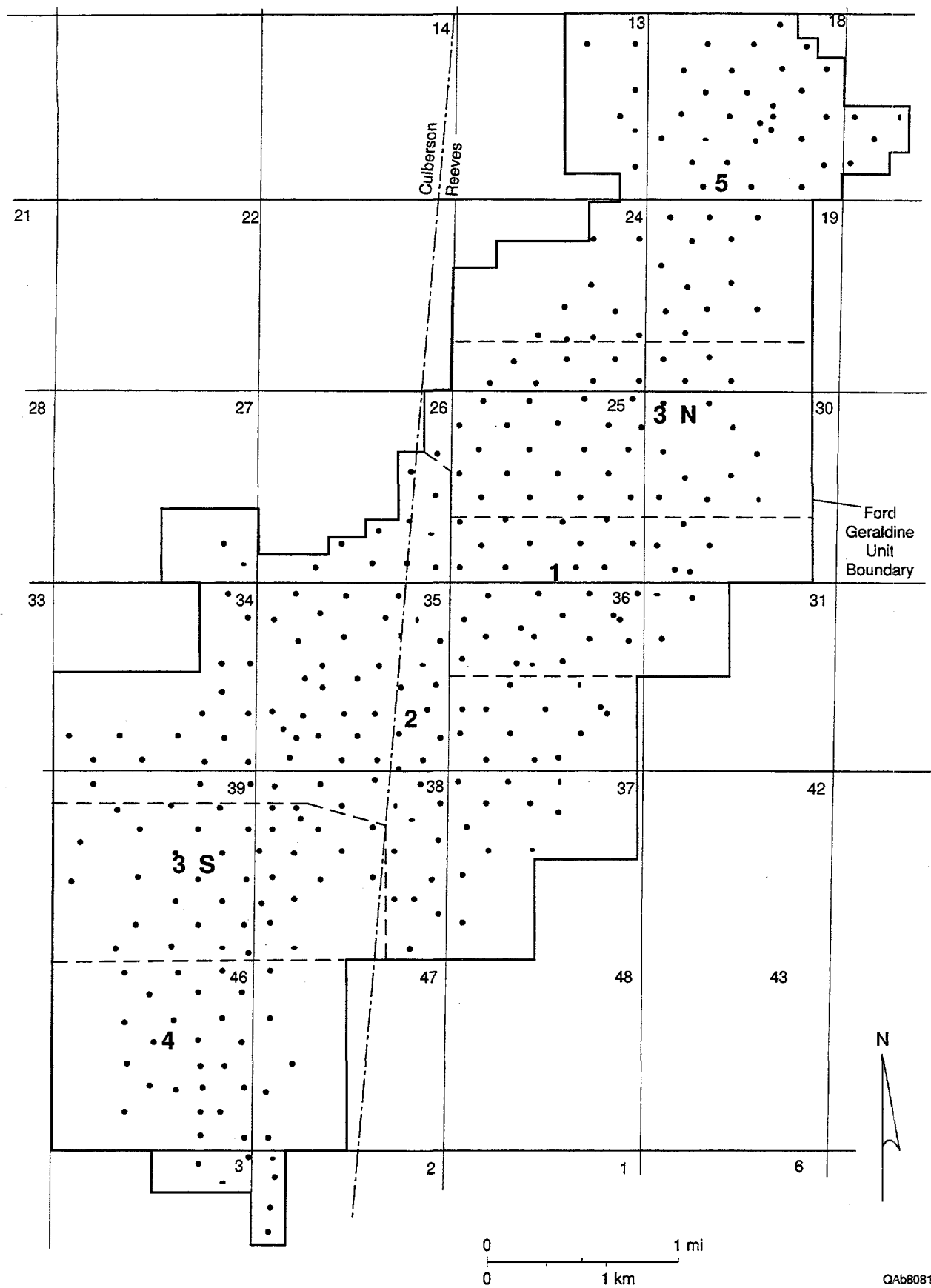
Figure 4. Waterflooding of the Ford Geraldine unit took place in five stages, in the areas shown.
