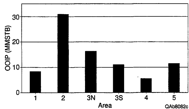
Figure 48. Original oil in place (OOIP) in waterflood areas 1 through 5. Areas are shown in figure 4.
