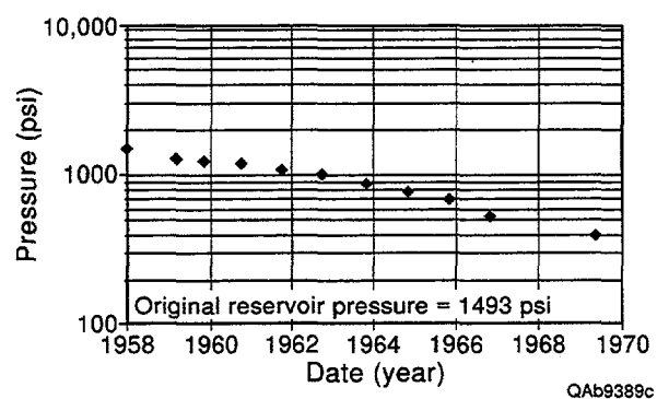
Figure 36. Plot of average reservoir pressure through time for Geraldine Ford field during the period of primary recovery.
