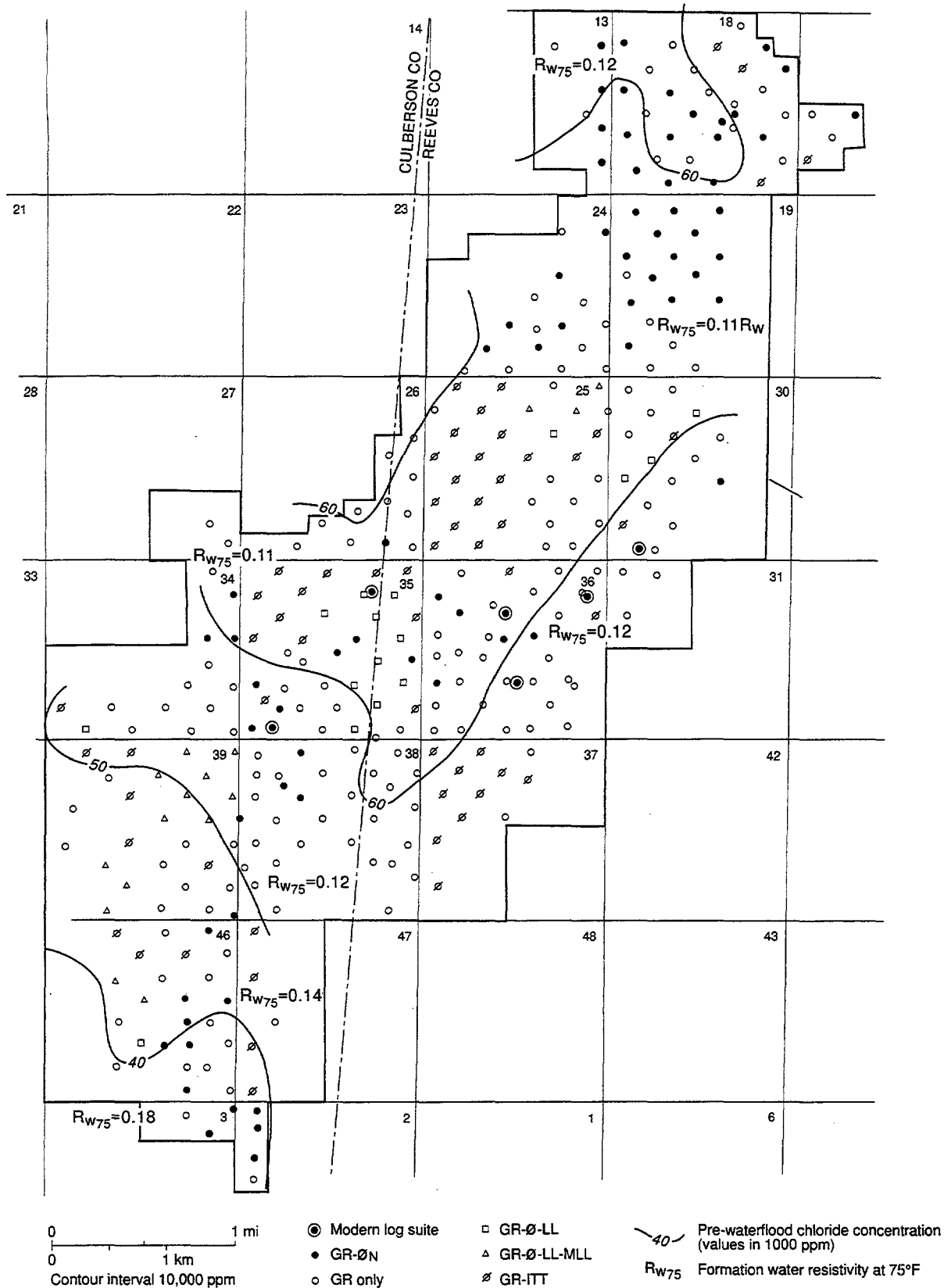
Figure 6. Distribution of geophysical log suites available in Ford Geraldine unit. Map also shows prewaterflood water-salinity distribution and formation-water resistivities ( R_w ) at 75°F for the Ford Geraldine unit. Water-salinity distribution from Ruggiero, 1985.
