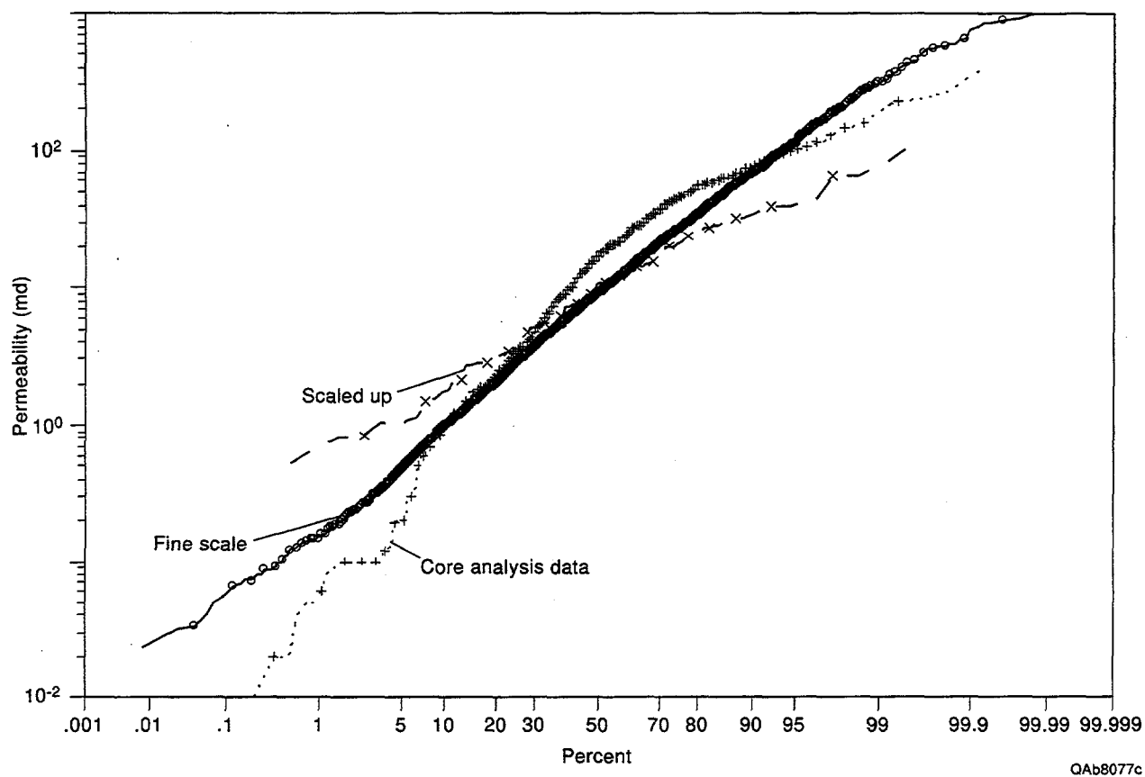
Figure 47. Cumulative distribution functions of permeability from (1) fine-scale permeability distribution, (2) scaled-up permeability distribution, and (3) permeability data from core analyses.
