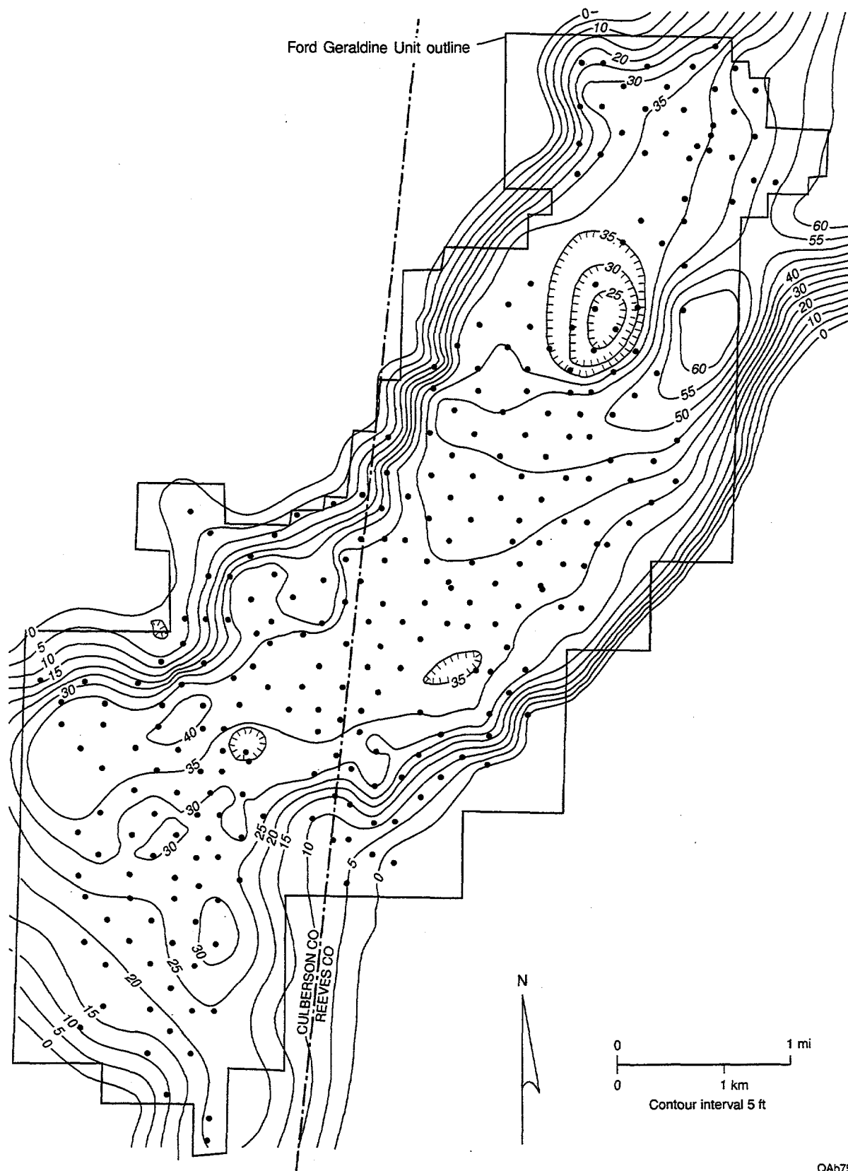
Figure 17. Map of thickness of the total Ramsey sandstone interval, from the top of the Ford siltstone to the base of the Trap siltstone, which is equivalent to gross pay thickness. Average Ramsey sandstone (gross-pay) thickness is 31.3 ft, with a standard deviation of 11.8 ft.
