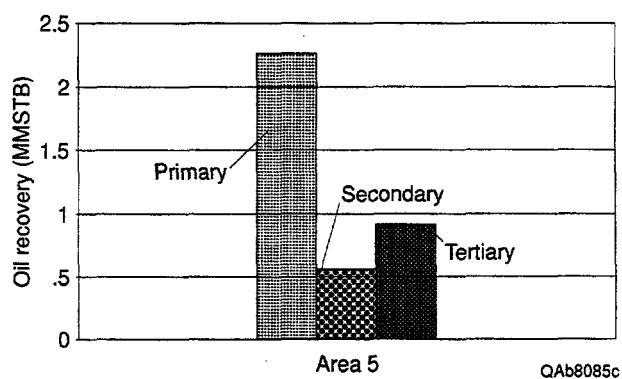
Figure 51. Primary and secondary recovery and project tertiary recovery for area 5.
