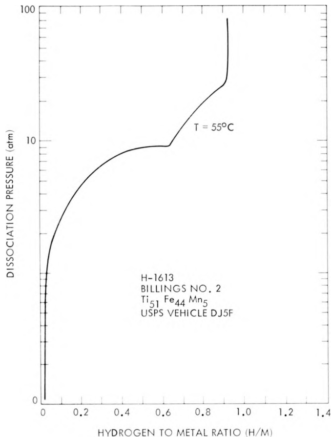
Figure 3. Hydride Dissociation Pressure Equilibrium Curve (reproduced from Hydrogen Fueled Vehicle-Hydride Storage System , Project 6120, final report to the U. S. Postal Service, by V. Anderson, Billings Energy Corp., July 31, 1978)
