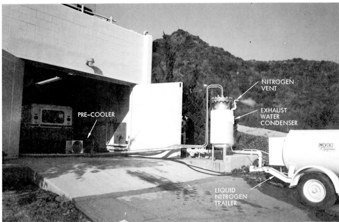
Figure 2. Exhaust Cooling System for Hydrogen USPS Jeep Tests
