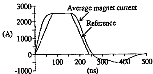
Figure 3. Simulation result for the circuit in Figure 2.
