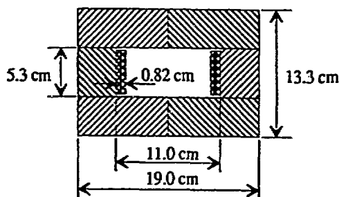
Figure 1. Cross section of the PAR kicker/bumper magnet
