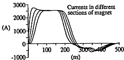
Figure 4. Simulation result for the circuit in Figure 2.
