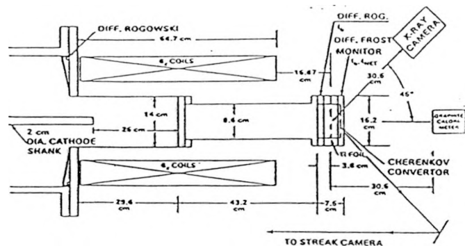
Fig. 3: Schematic diagram of the immersed foilless diode with associated diagnostics.
