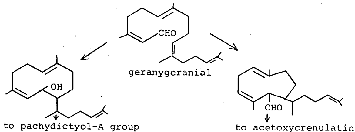
Two possible cyclizations of geranylgeranial
