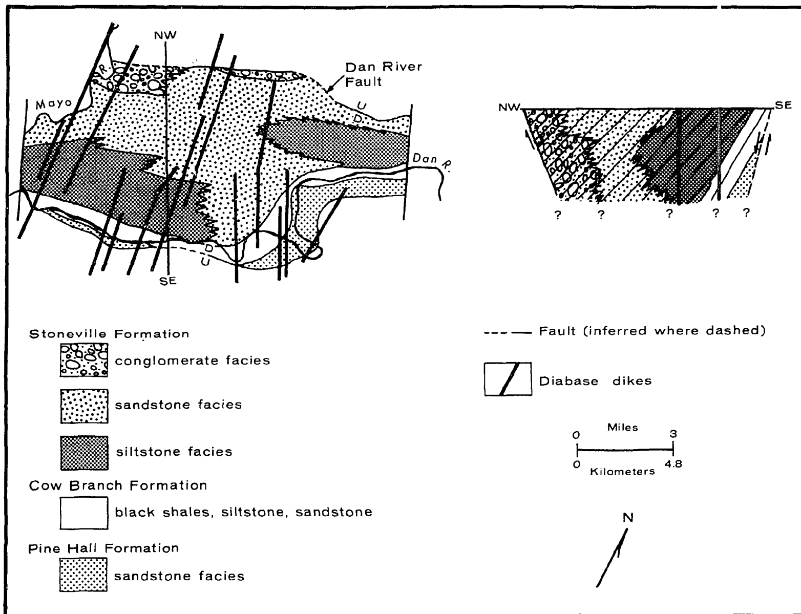
FIGURE 4-2. GEOLOGIC MAP AND CROSS SECTION OF DAN RIVER BASIN, IN NORTH-CENTRAL NORTH CAROLINA, ILLUSTRATING GEOLOGIC COMPLEXITY AND HIGHLY VARIABLE LITHOLOGY (MODIFIED FROM THAYER, 1970)
