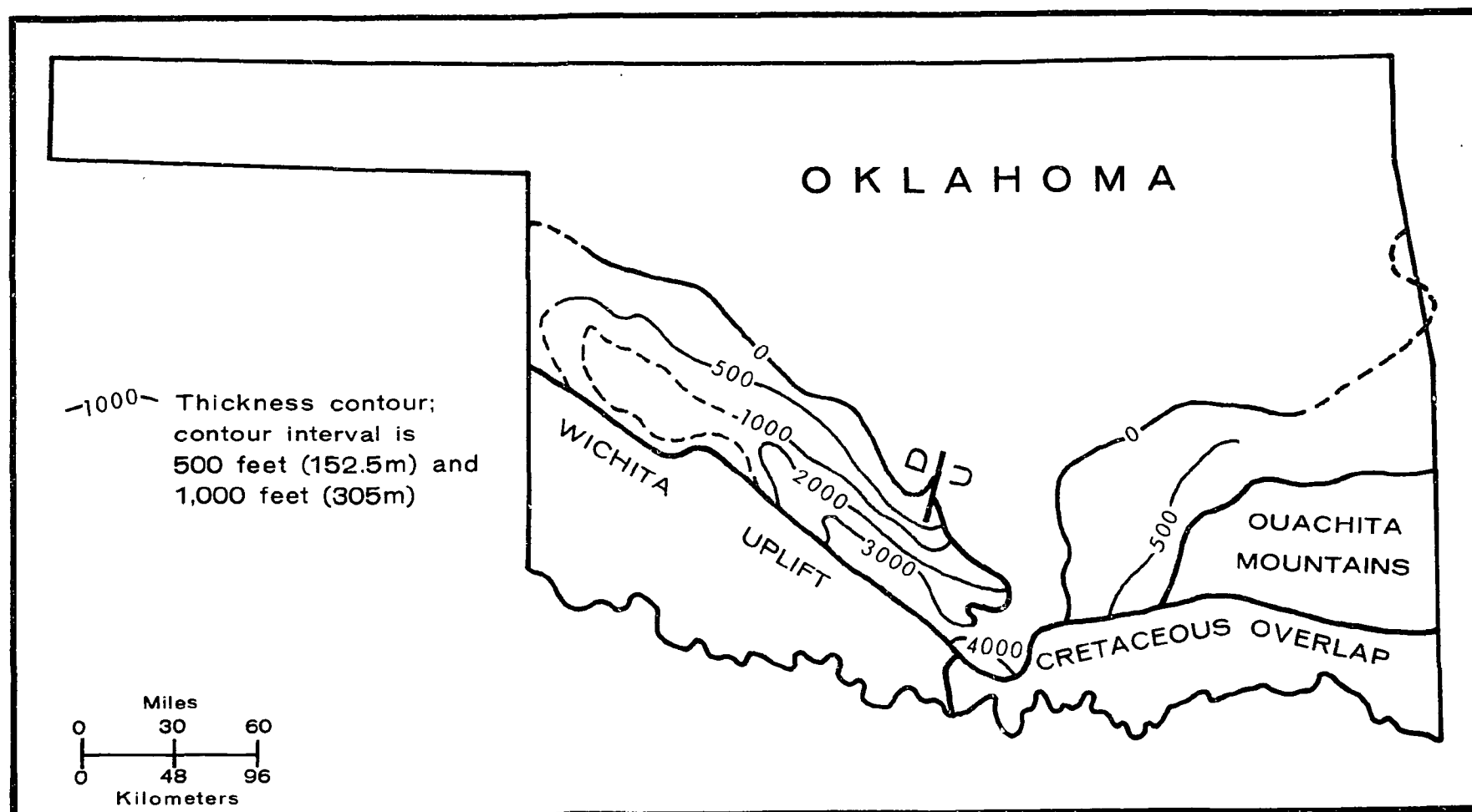
FIGURE 6-12. MAP OF OKLAHOMA, SHOWING THICKNESS OF COMBINED SEQUENCE OF DELAWARE CREEK AND GODDARD SHALES (MODIFIED FROM HUFFMAN, 1959)
