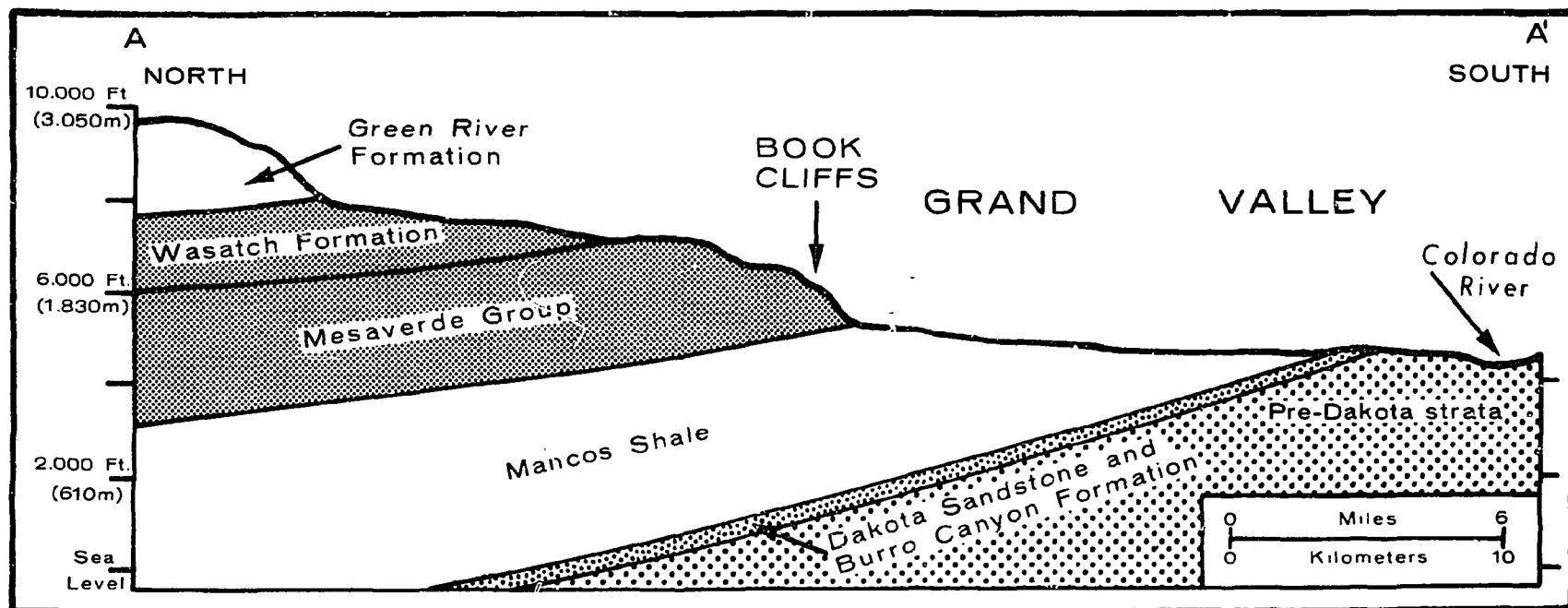
FIGURE 8-2. CROSS SECTION A-A', SHOWING MANCOS SHALE ON SOUTHERN FLANKS OF UINTA AND PICEANCE BASINS IN VICINITY OF UTAH-COLORADO STATE LINE (MODIFIED FROM CASHION, 1973)
