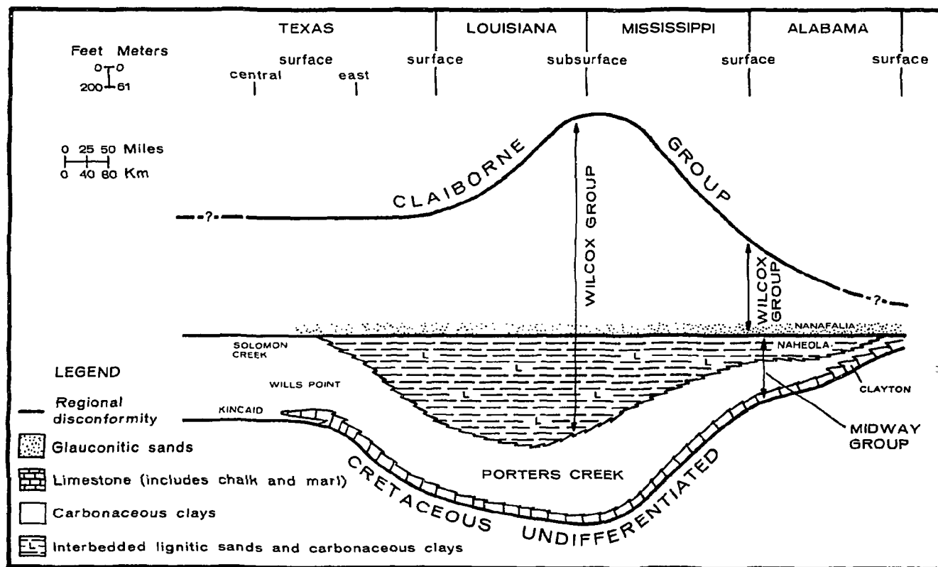
FIGURE 5-3. DIAGRAM OF GENERALIZED STRATIGRAPHIC RELATIONSHIPS BETWEEN PORTERS CREEK CLAY AND OTHER FORMATIONS IN THE MIDWAY AND WILCOX GROUPS OF THE GULF COAST (MODIFIED FROM MURRAY, 1961)
