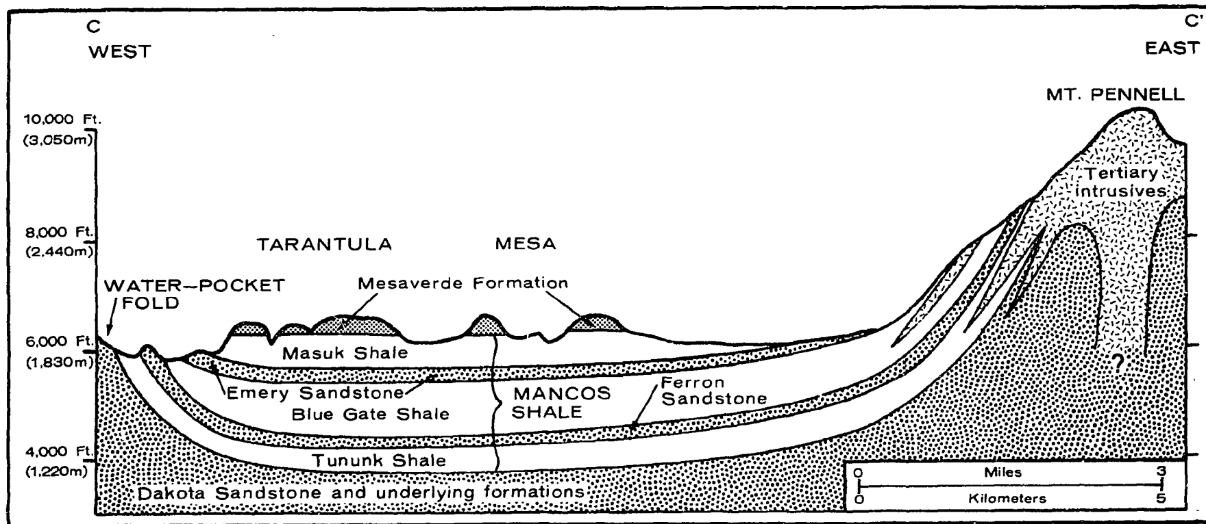
FIGURE 8-4. CROSS SECTION C-C', SHOWING MANCOS SHALE IN HENRY BASIN, WAYNE AND GARFIELD COUNTIES, UTAH (MODIFIED FROM DOELLING AND GRAHAM, 1972b)
