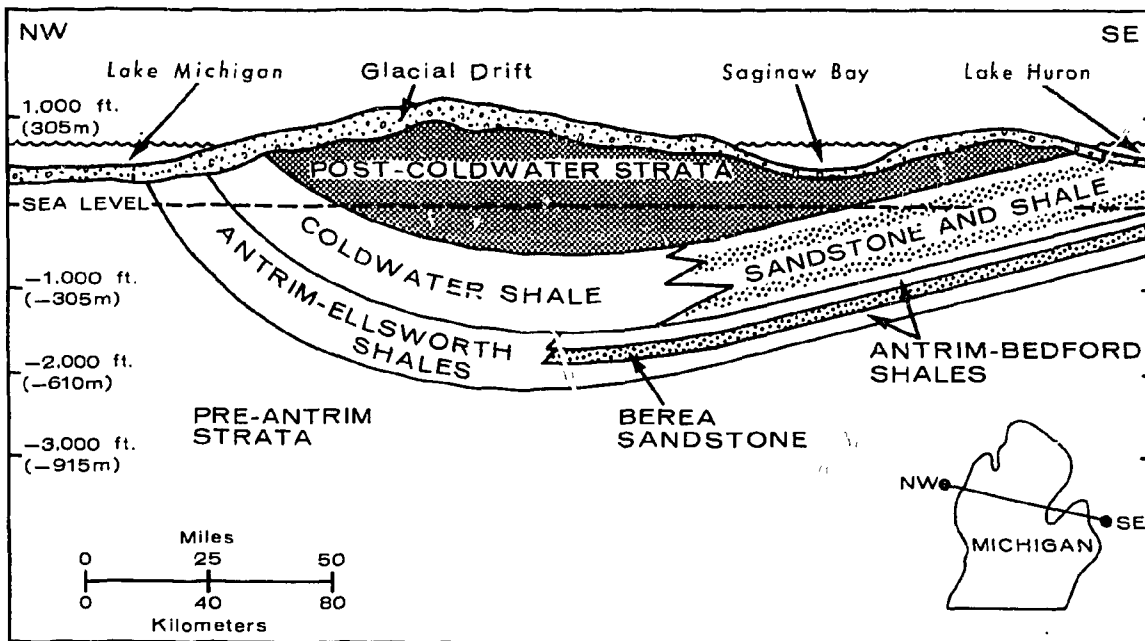
FIGURE 3-19. GENERALIZED NORTHWEST-SOUTHEAST CROSS SECTION SHOWING STRATIGRAPHIC AND LITHOLOGIC RELATIONSHIPS BETWEEN COLDWATER AND ANTRIM-ELLSWORTH SHALE SEQUENCES IN NORTH-CENTRAL PART OF MICHIGAN BASIN (MODIFIED FROM LOMENICK ET AL., 1983)
