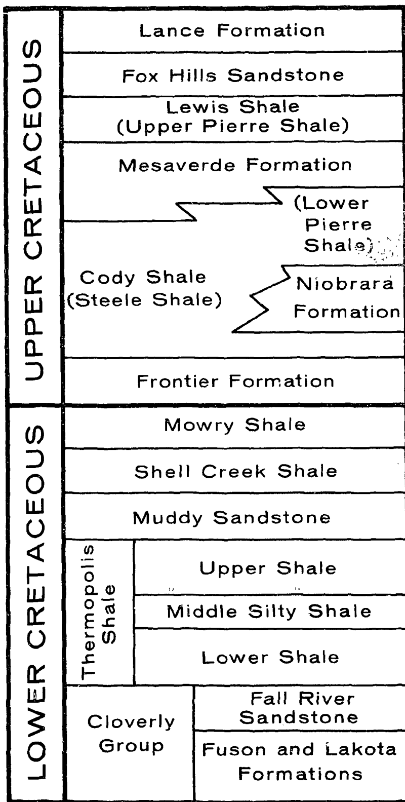
FIGURE 7-4. CHART SHOWING GENERALIZED STRATIGRAPHIC NOMENCLATURE FOR CRETACEOUS STRATA IN WYOMING BASINS AND NEARBY AREAS OF ROCKY MOUNTAINS (MODIFIED AFTER MCGOOKEY ET AL., 1972). VERTICAL DIMENSIONS ARE UNRELATED TO THICKNESS OF FORMATIONS
