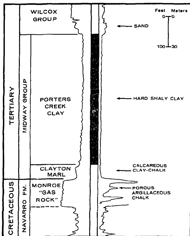
FIGURE 5-4. DIAGRAM SHOWING CHARACTERISTIC ELECTRIC-LOG RESPONSE OF PORTERS CREEK CLAY AS DOMINANT UNIT WITHIN MIDWAY GROUP OF GULF COAST (MODIFIED FROM WANG, 1952)
