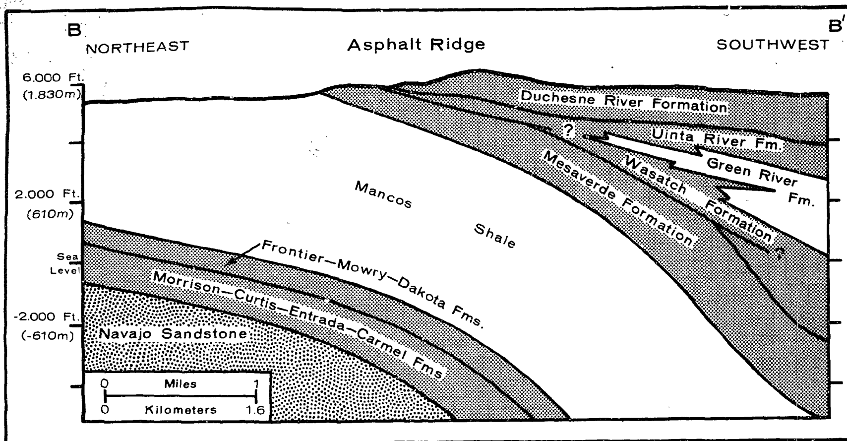
FIGURE 8-3. CROSS SECTION B-B', SHOWING MANOS SHALE AT ASPHALT RIDGE NEAR VERNAL, UTAH, ON NORTHEASTERN SIDE OF UINTA BASIN (MODIFIED FROM COVINGTON, 1963)
