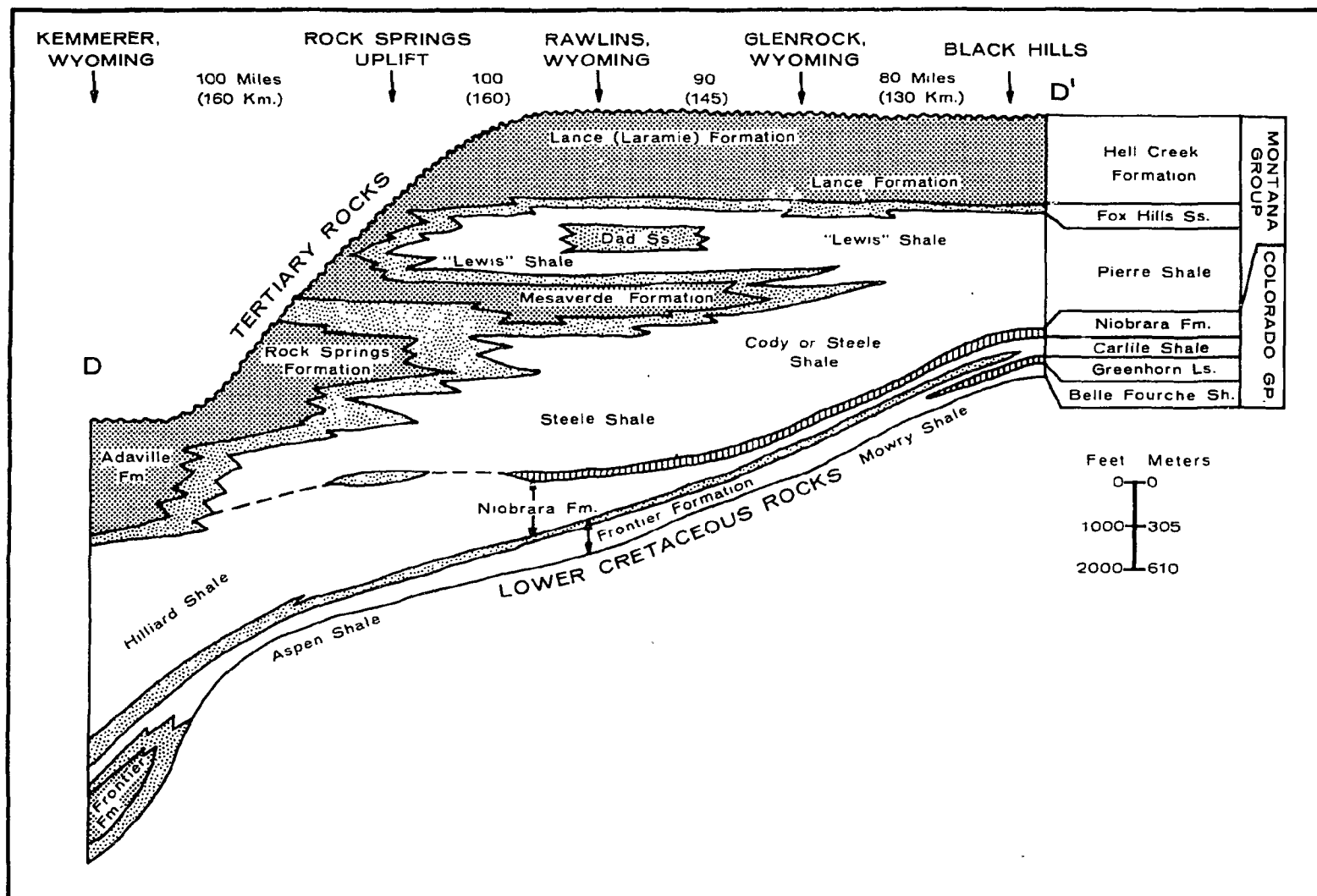
FIGURE 6-24. GENERALIZED STRATIGRAPHIC CROSS SECTION D-D', SHOWING UPPER CRETACEOUS SHALES AND ASSOCIATED STRATA IN NORTHERN GREAT PLAINS AND ROCKY MOUNTAINS (MODIFIED FROM WEIMER, 1960; MCGOOKEY ET AL., 1972). SEE FIGURE 6-22 FOR LOCATION MAP AND EXPLANATION
