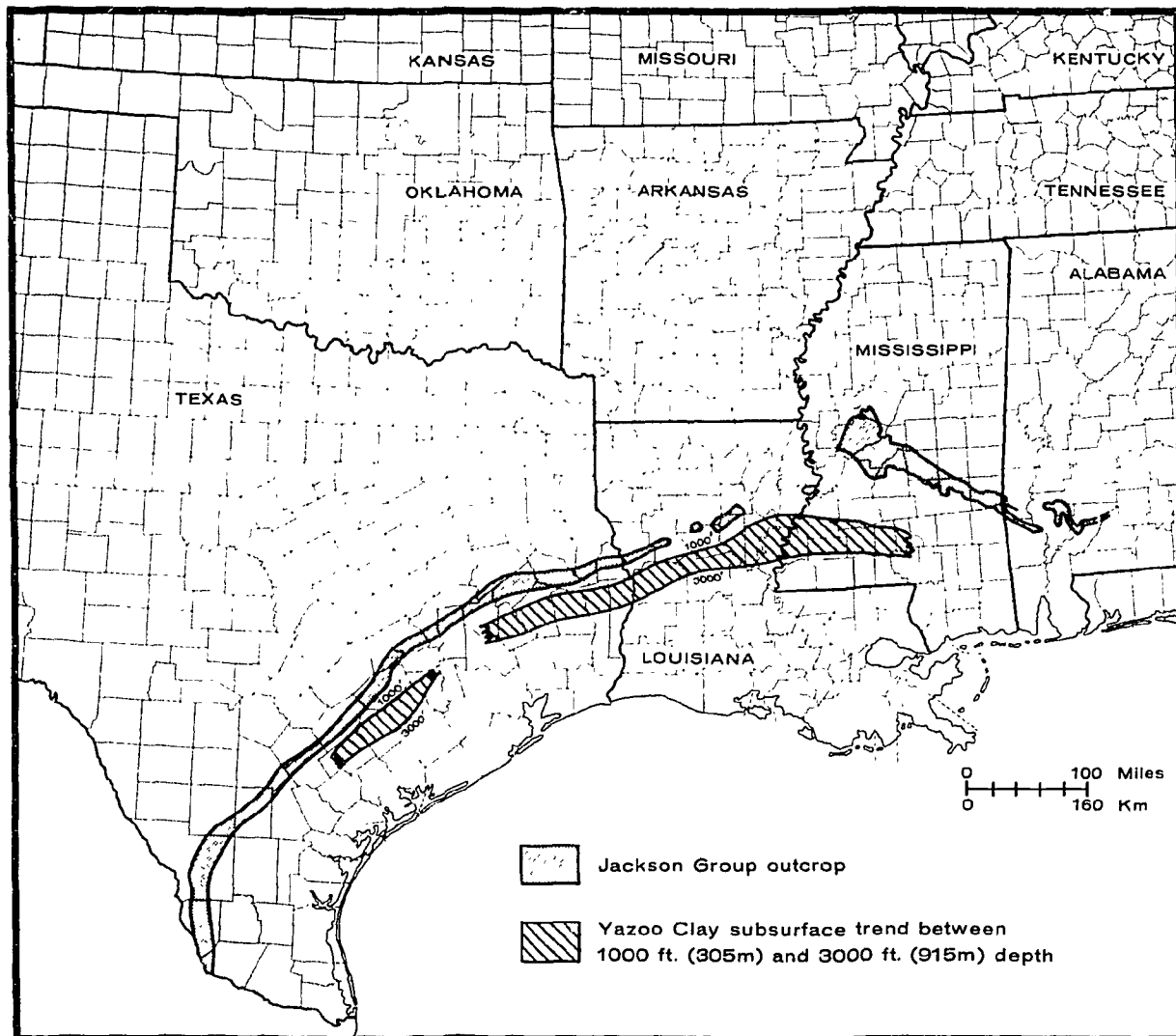
FIGURE 5-11. MAP SHOWING OUTCROP OF JACKSON GROUP AND DISTRIBUTION OF YAZOO CLAY WITHIN THE MODERATE DEPTH RANGE
