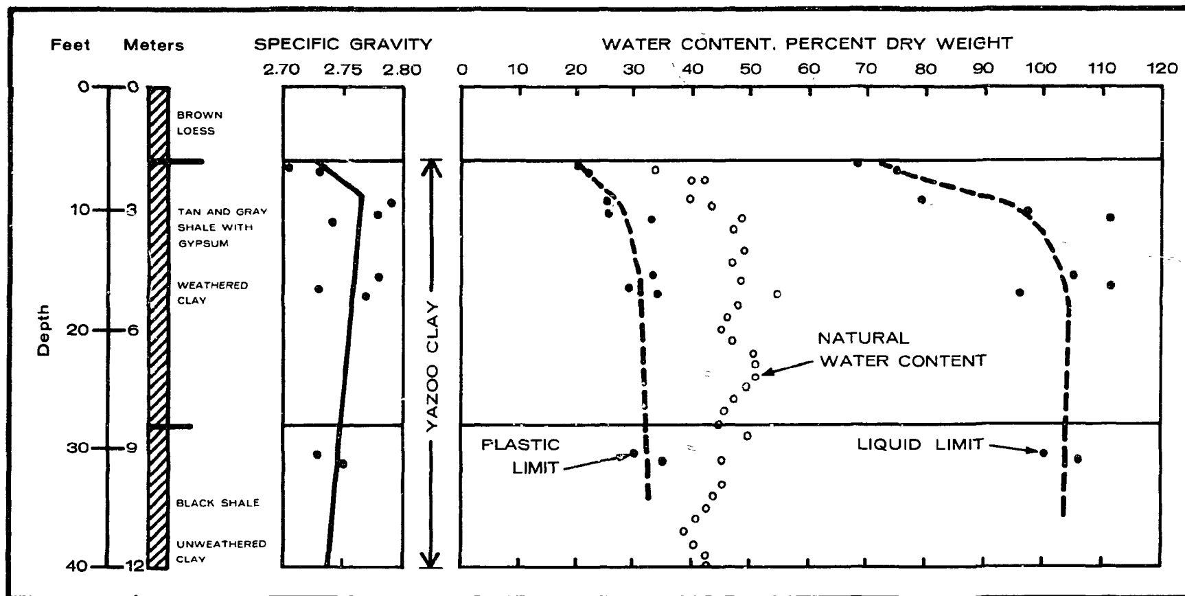
FIGURE 5-12. PLOTS OF SOME PHYSICAL CHARACTERISTICS OF YAZOO CLAY AS MEASURED IN CORE SAMPLE FROM CLINTON, MISSISSIPPI (MODIFIED FROM JOHNSON, 1978)
