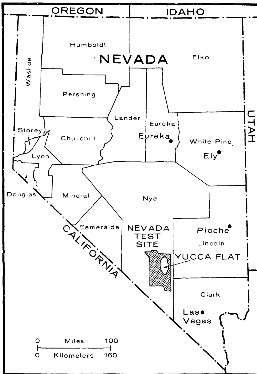
FIGURE 9-1. MAP SHOWING COUNTIES AND SEVERAL CITIES IN NEVADA AND LOCATION OF NEVADA TEST SITE IN SOUTHERN NYE COUNTY
