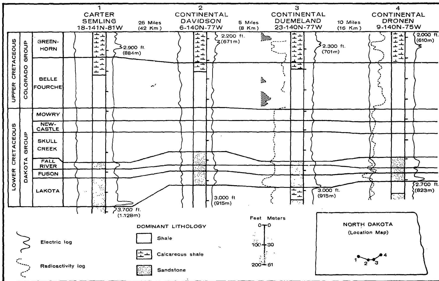
FIGURE 6-33. CORRELATION OF CRETACEOUS SHALES IN SKULL CREEK, NEWCASTLE, MOWRY, AND BELLE FOURCHE FORMATIONS OF SOUTH-CENTRAL NORTH DAKOTA (MODIFIED FROM HANSEN, 1955)
