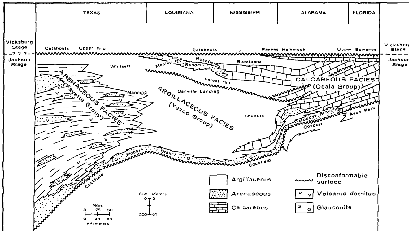
FIGURE 5-9. DIAGRAM SHOWING STRATIGRAPHIC RELATIONSHIPS OF YAZOO CLAY AND OTHER JACKSON AND VICKSBURG UNITS (MODIFIED FROM MURRAY, 1961)
