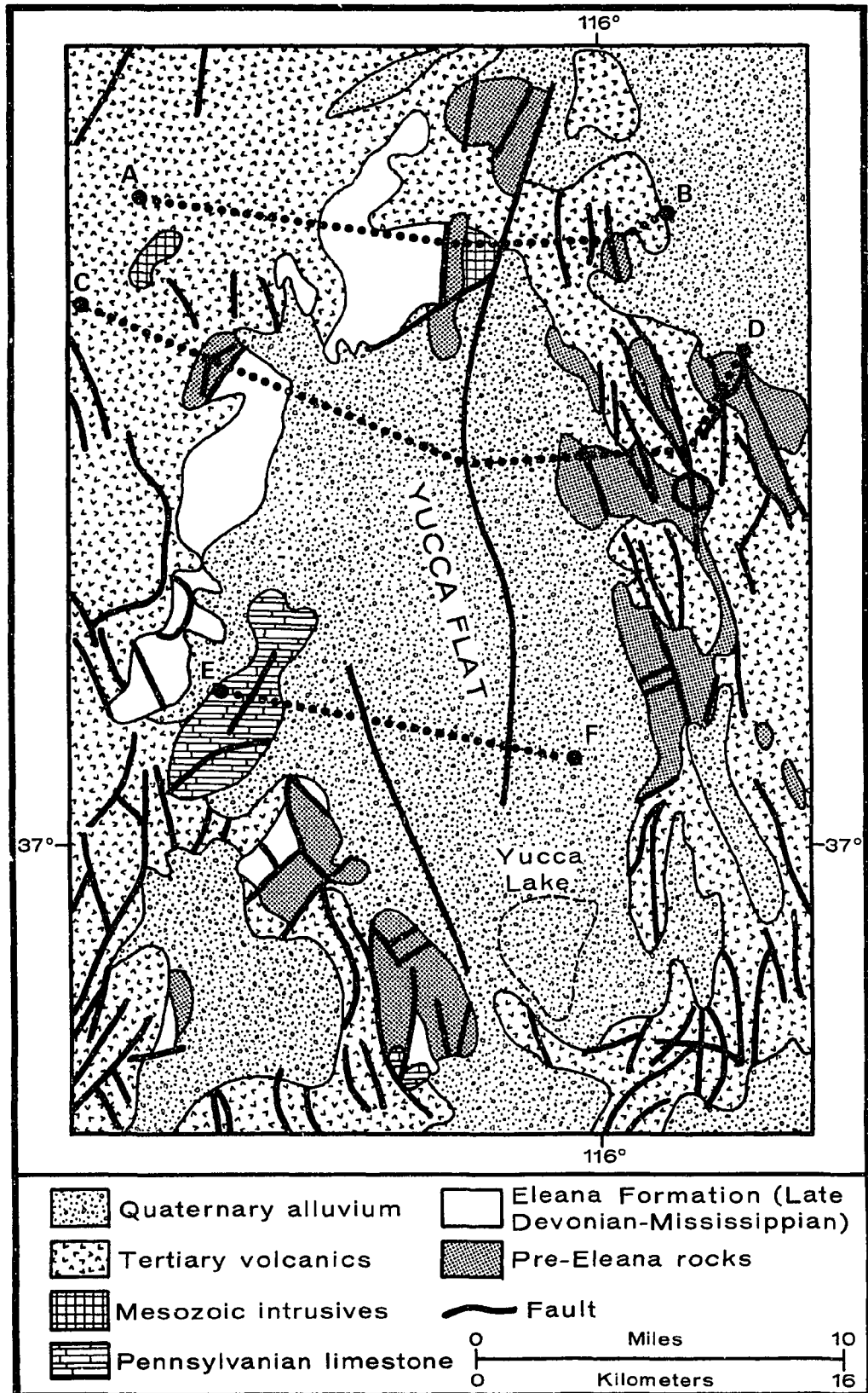
FIGURE 9-5. GENERALIZED GEOLOGIC MAP OF YUCCA FLAT AREA OF NEVADA TEST SITE, NYE COUNTY, NEVADA (MODIFIED FROM CORNWALL, 1972). CROSS SECTIONS A-B, C-D, AND E-F ARE SHOWN IN NEXT FIGURE
