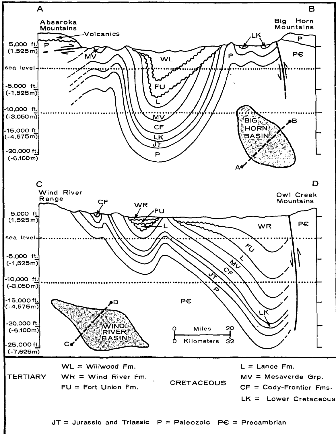
FIGURE 7-5. DIAGRAMMATIC CROSS SECTIONS THROUGH BIG HORN BASIN (SECTION A-B) AND WIND RIVER BASIN (SECTION C-D) OF WYOMING (MODIFIED FROM STAUFFER, 1971)
