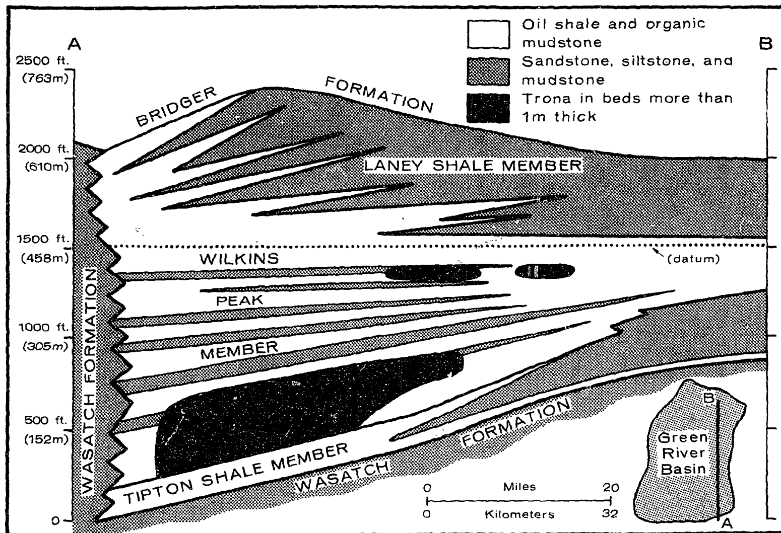
FIGURE 7-6. STRATIGRAPHIC CROSS SECTION OF GREEN RIVER FORMATION IN GREEN RIVER BASIN OF SOUTHWESTERN WYOMING (MODIFIED FROM NETHERLAND, SEWELL AND ASSOCIATES, 1975b)
