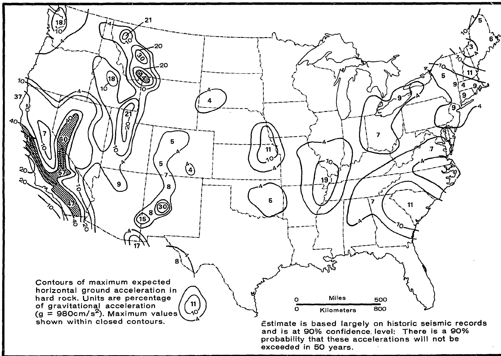
FIGURE 1-3b. MAP OF UNITED STATES SHOWING SEISMIC HAZARD BASED UPON SEISMIC-RISK ZONATION (a) AND PROBABILITY OF GROUND SHAKING (b) (MODIFIED FROM ALGERMISSSEN AND PERKINS, 1976)
