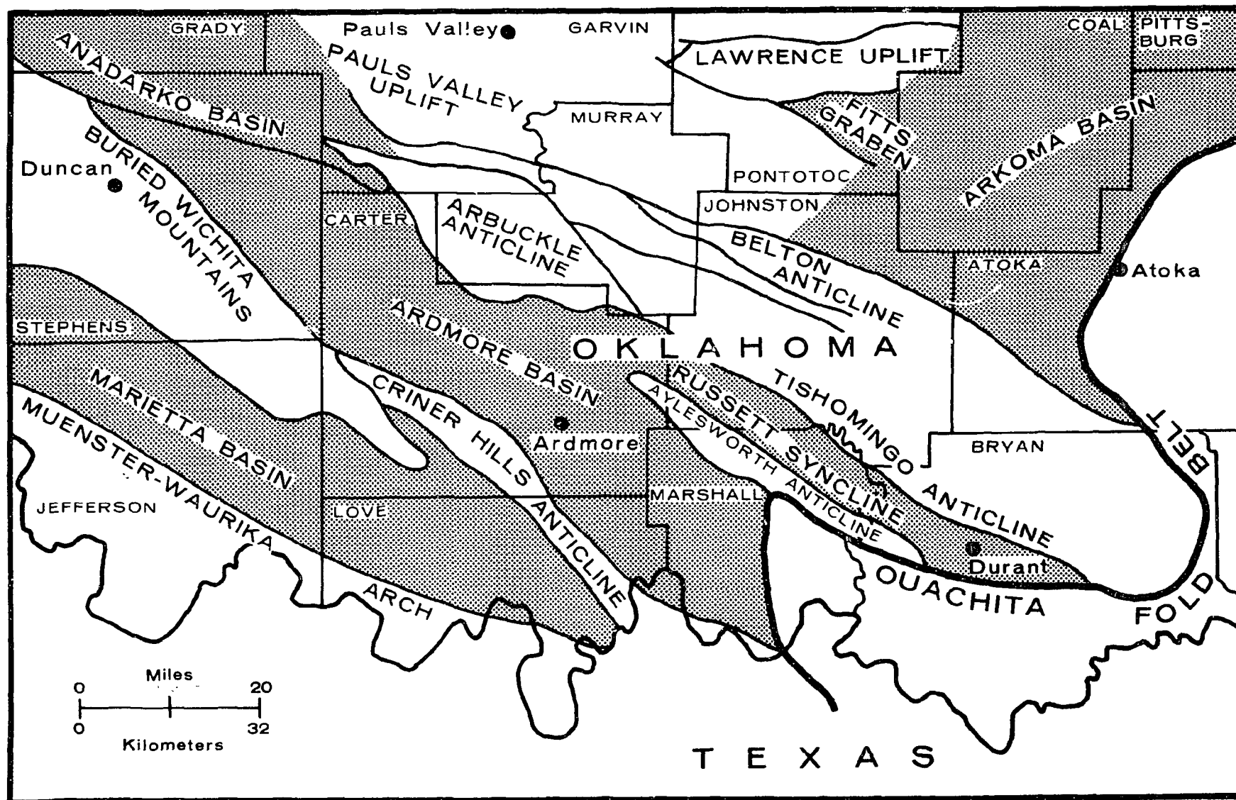
FIGURE 6-8. MAP OF SOUTHERN OKLAHOMA FOLDED BELT, SHOWING STRUCTURAL PROVINCES (MODIFIED FROM HICKS, 1971); STIPPLING INDICATES PRINCIPAL BASINS AND SYNCLINES
