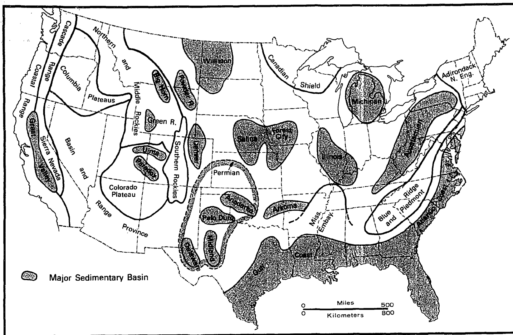
FIGURE 2-2. MAP OF UNITED STATES SHOWING LOCATIONS AND EXTENT OF PRINCIPAL AND SELECTED SMALLER SEDIMENTARY BASINS
