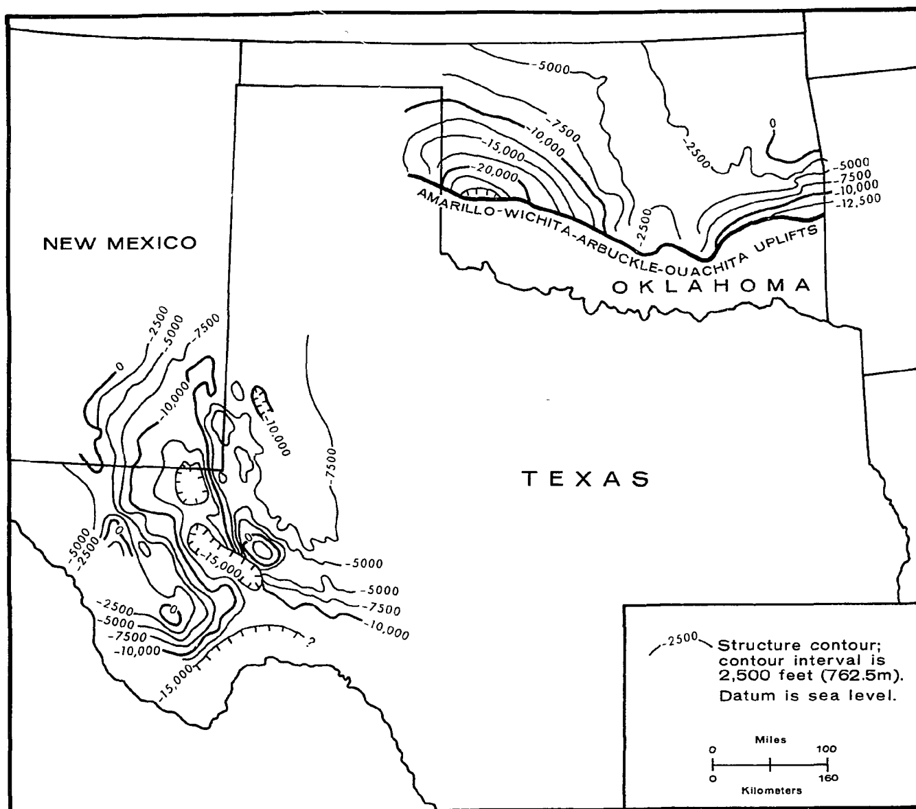
FIGURE 6-7. STRUCTURE MAP ON BASE OF WOODFORD (CHATTANOOGA) SHALE IN OKLAHOMA, WEST TEXAS, AND SOUTHEASTERN NEW MEXICO. CONTOURS PARTIALLY RESTORED WHERE WOODFORD HAS BEEN ERODED (MODIFIED FROM SALISBURY, 1968; AMSDEN, 1975, 1980)
