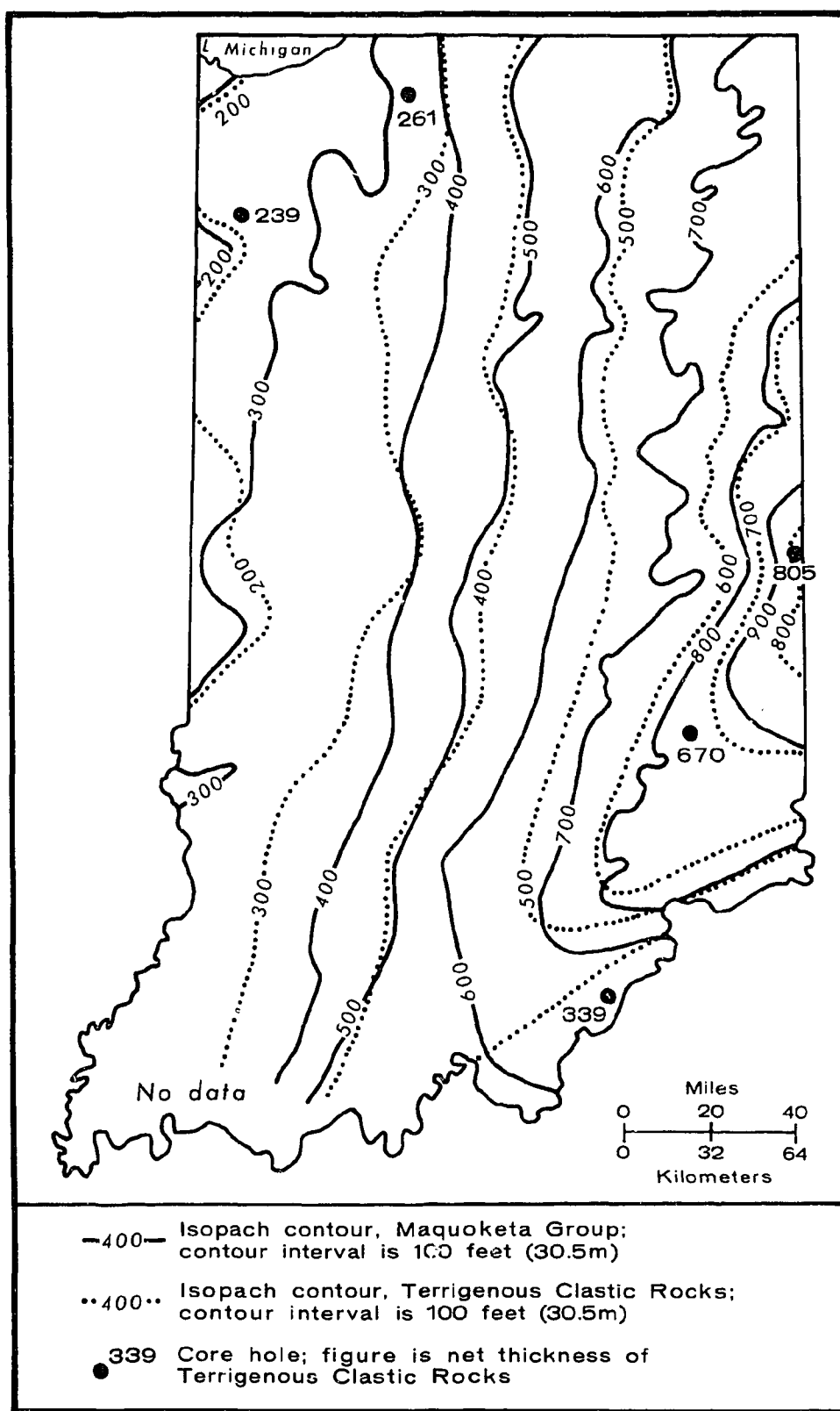
FIGURE 3-4. MAP SHOWING THICKNESS OF ENTIRE MAQUOKETA GROUP IN INDIANA, AND APPROXIMATE NET THICKNESS OF TERRIGENOUS CLASTIC ROCKS (MODIFIED FROM GRAY, 1972)
