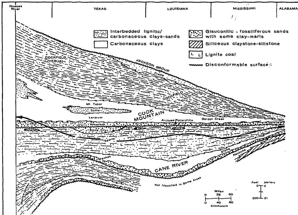
FIGURE 5-6. DIAGRAM OF GENERALIZED STRATIGRAPHIC RELATIONSHIPS BETWEEN CANE RIVER AND COOK MOUNTAIN FORMATIONS AND OTHER CLAIBORNE GROUP UNITS OF GULF COAST (MODIFIED FROM MURRAY, 1961)
