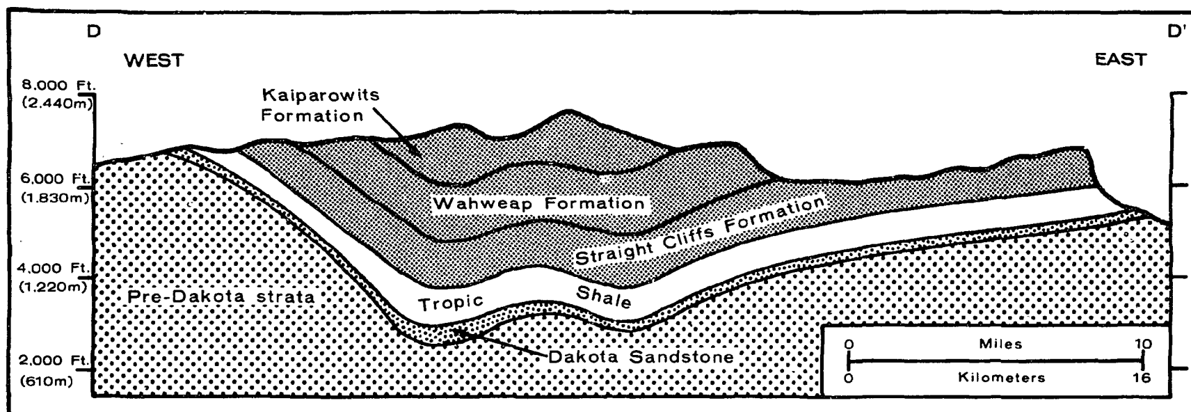
FIGURE 8-5. CROSS SECTION D-D' THROUGH KAIPAROWITS BASIN, KANE AND GARFIELD COUNTIES, UTAH, SHOWING RELATION OF TROPIC SHALE (EQUIVALENT TO LOWER PART OF MANCOS SHALE) TO ADJACENT SANDSTONES (MODIFIED FROM DOELLING AND GRAHAM, 1972b)
