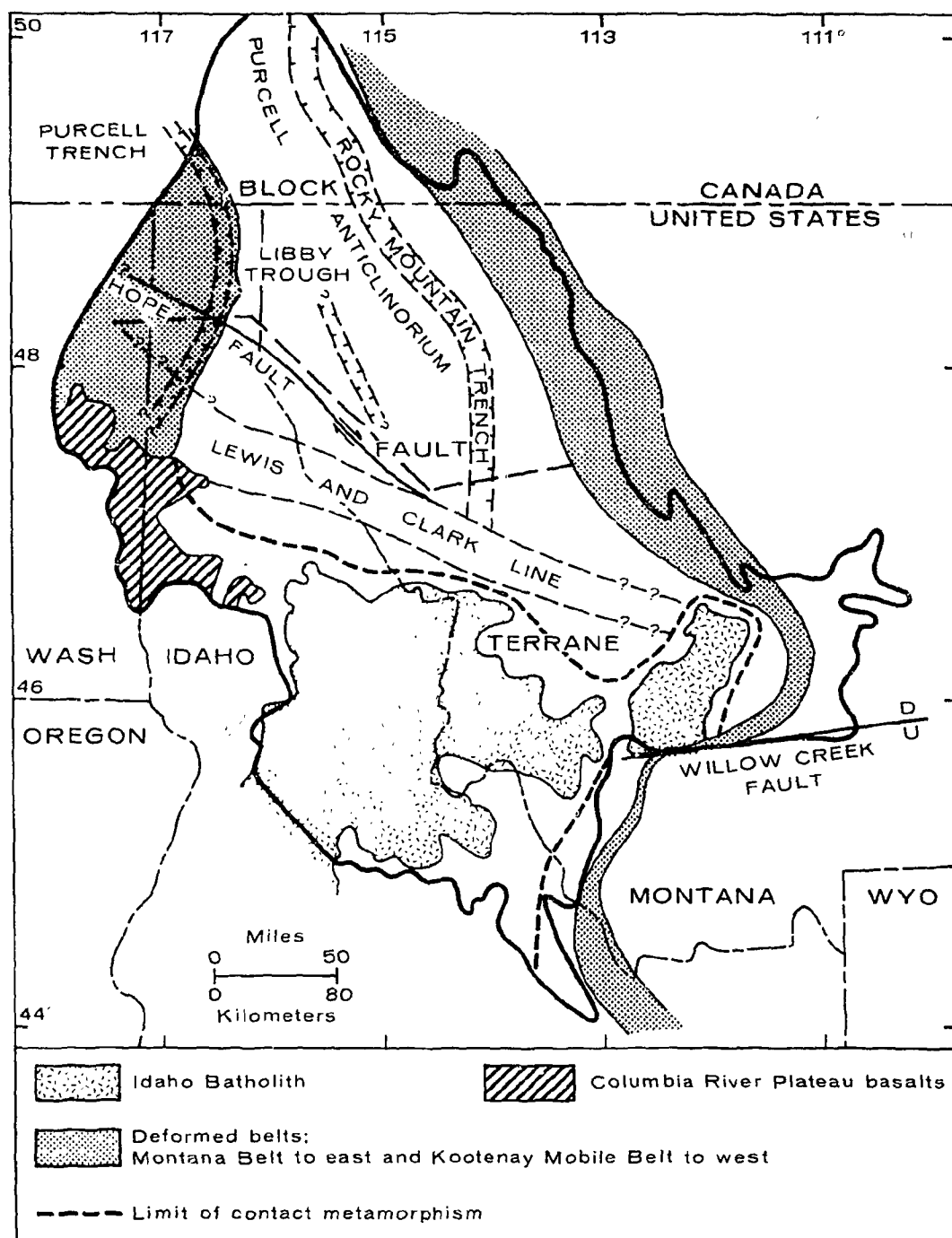
FIGURE 12-2. MAP SHOWING OUTCROP BELT AND REGIONAL TECTONIC SETTING OF THE BELT SERIES IN MONTANA, IDAHO, AND ADJACENT AREAS (MODIFIED FROM HARRISON, 1972)
