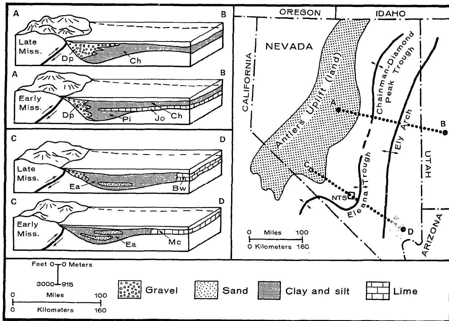
FIGURE 9-2. PALEOTECTONIC MAP AND BLOCK DIAGRAMS, SHOWING MISSISSIPPIAN SEDIMENTARY UNITS FORMED IN GREAT BASIN AREA (MODIFIED FROM LARSON AND LANGENHEIM, 1979). ABBREVIATIONS: DP, DIAMOND PEAK FORMATION; Ch, CHAINMAN FORMATIONS; Pi, PILOT SHALE; Jo, JOANA LIMESTONE; Ea, ELEANA FORMATION; Bw, BATTLESHIP WASH FORMATION; Mc, MONTE CRISTO FORMATION
