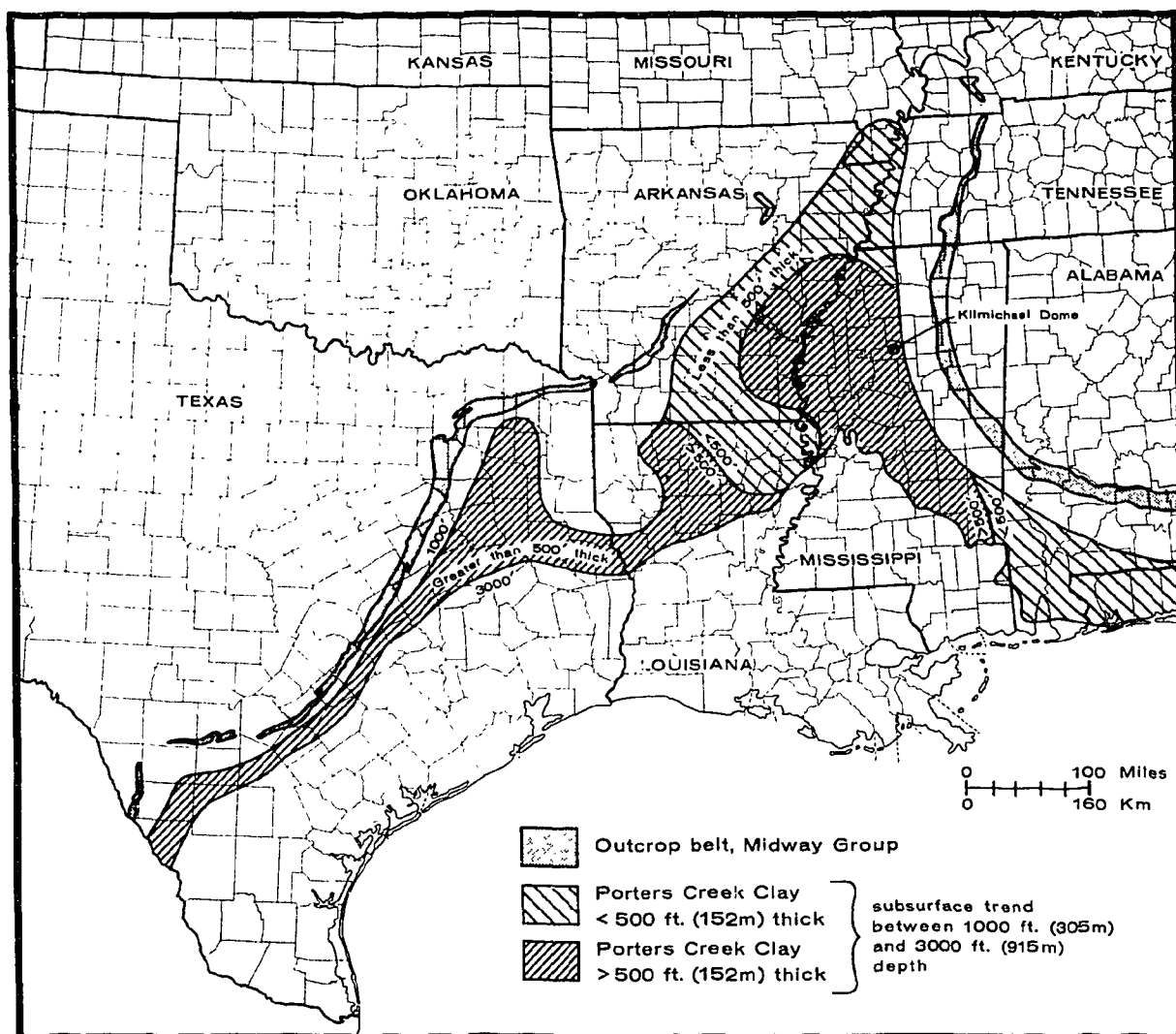
FIGURE 5-5. MAP SHOWING OUTCROP BELT OF MIDWAY GROUP, AND DISTRIBUTION AND THICKNESS OF PORTERS CREEK CLAY WITHIN THE MODERATE DEPTH RANGE
