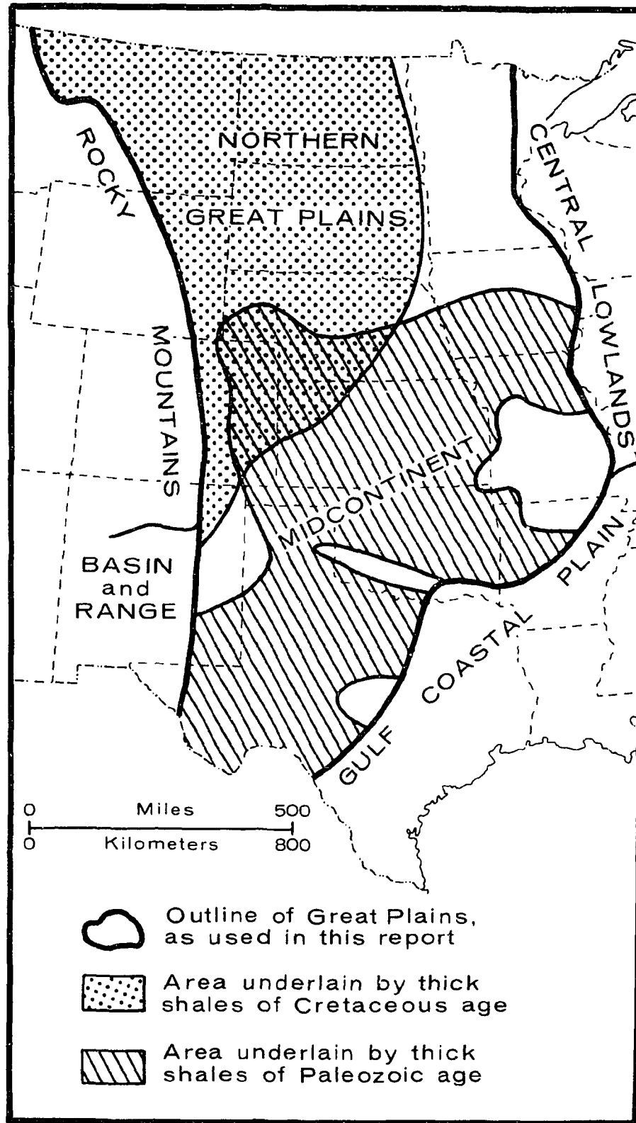
FIGURE 6-1. MAP OF WEST-CENTRAL UNITED STATES, SHOWING OUTLINE OF GREAT PLAINS AND AREAS UNDERLAIN BY THICK SHALES OF PALEOZOIC AND CRETACEOUS AGE
