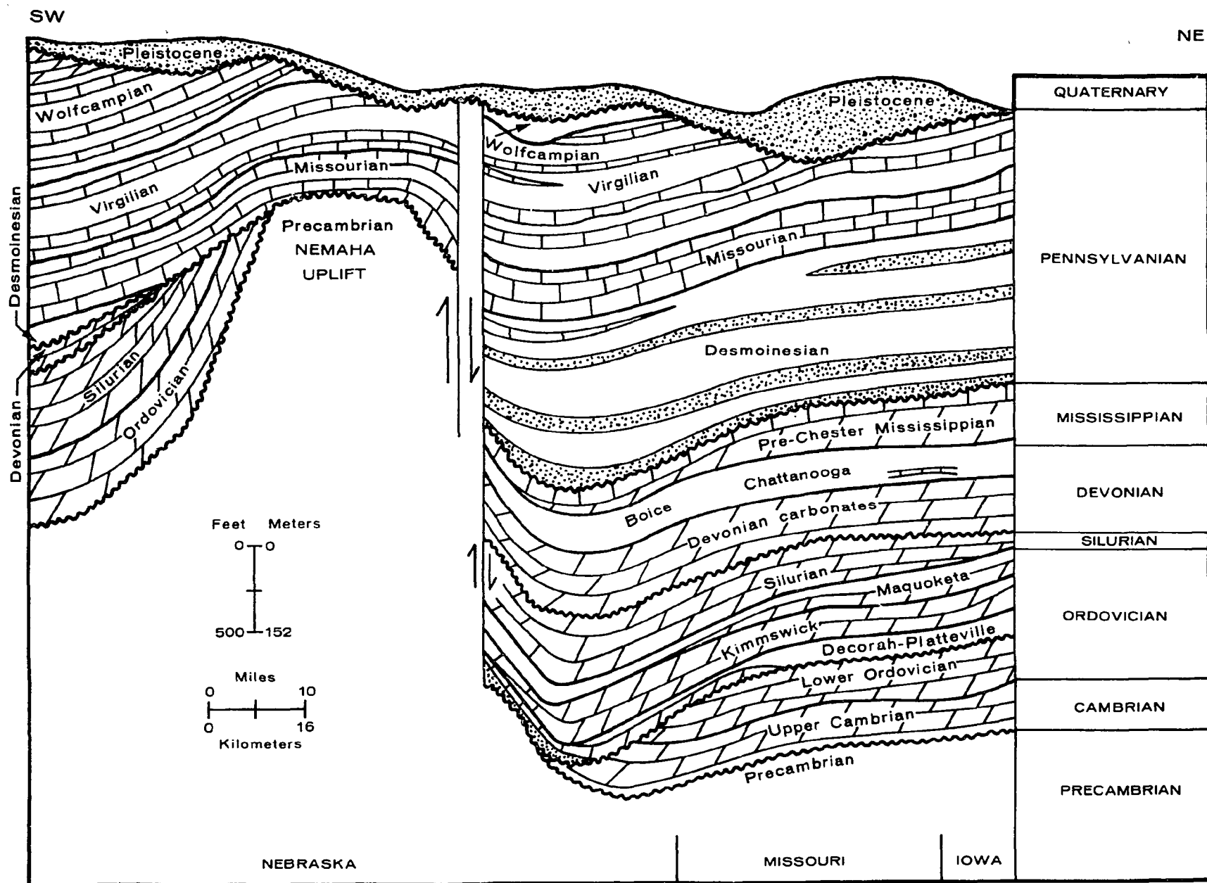
FIGURE 6-10. DIAGRAMMATIC SOUTHWEST-NORTHEAST LITHOLOGIC CROSS SECTION FROM SALINA BASIN THROUGH NEMAHA UPLIFT AND FOREST CITY BASIN (MODIFIED FROM CARLSON, 1971)
