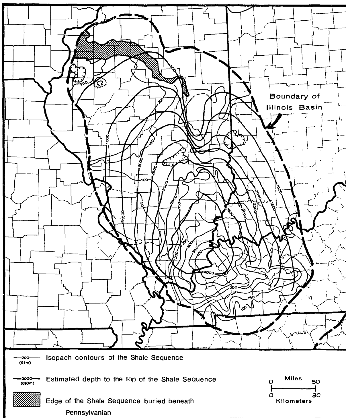
FIGURE 3-16. MAP OF ILLINOIS BASIN, SHOWING THICKNESS OF AND DEPTH TO DEVONIAN-MISSISSIPPIAN NEW ALBANY SHALE (MODIFIED FROM LOMENICK ET AL., 1983). THICKNESS DATA (NARROW CONTOUR LINES) AND DEPTH DATA (WIDE CONTOUR LINES) ARE GIVEN IN FEET. DIAGONAL LINES IN NORTH SHOW AREA WHERE ERODED EDGE OF NEW ALBANY SHALE IS BURIED BENEATH PENNSYLVANIAN STRATA
