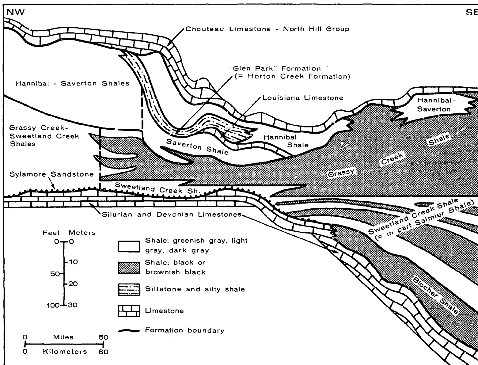
FIGURE 3-14. GENERALIZED NORTHWEST-SOUTHEAST CROSS SECTION THROUGH THE ILLINOIS PORTION OF THE ILLINOIS BASIN, SHOWING STRATIGRAPHIC RELATIONSHIPS BETWEEN SUBDIVISIONS OF NEW ALBANY SHALE AND ADJACENT STRATA (MODIFIED FROM REINHOLD, 1978; CLUFF ET AL., 1981)
