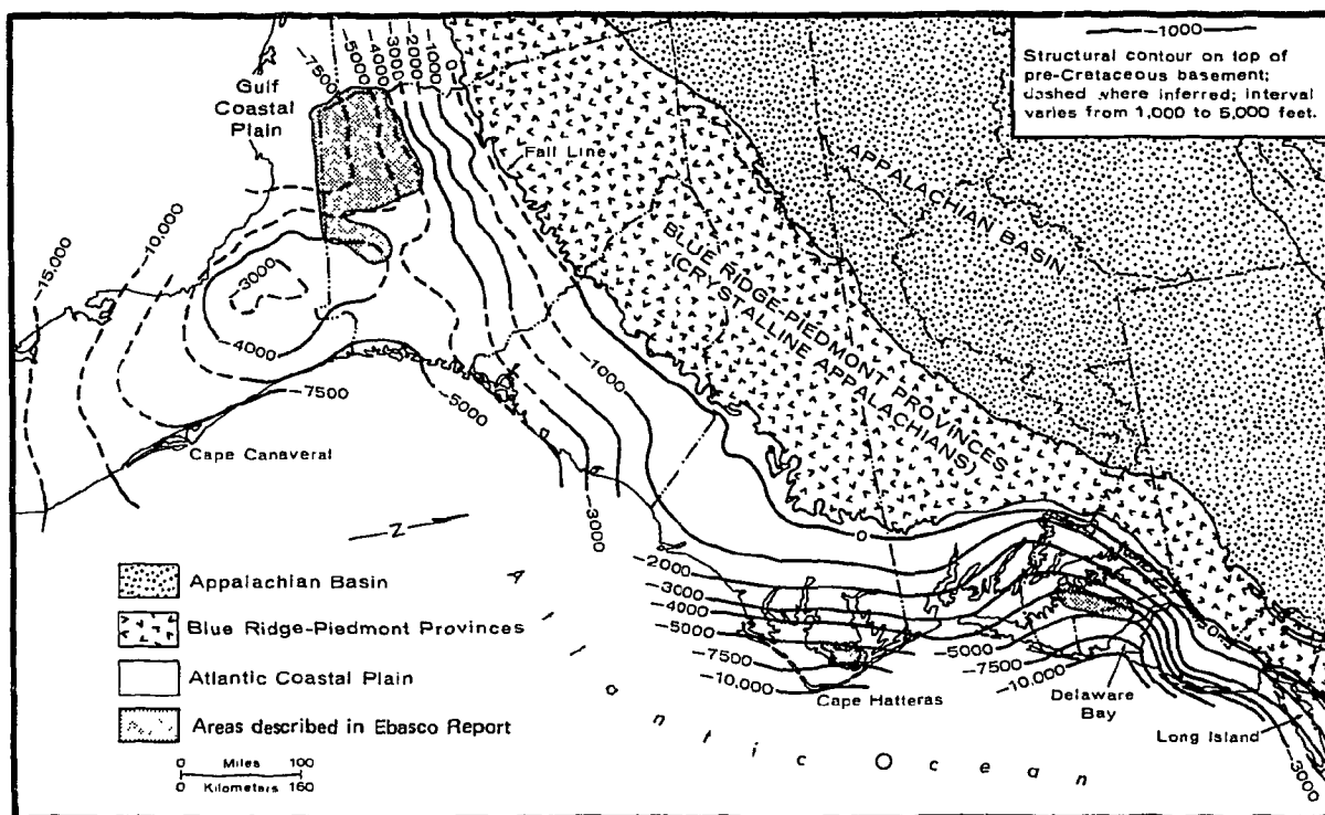
FIGURE 4-4. STRUCTURE-CONTOUR MAP OF BASEMENT BENEATH ATLANTIC COASTAL PLAIN FROM NEW YORK TO FLORIDA. ALSO SHOWN ARE POSITIONS OF FALL LINE, ADJACENT GEOLOGIC PROVINCES, AND LOCATION OF AREAS AS STUDIED BY EBASCO SERVICES, INC. (MODIFIED FROM MAHER, 1971; EBASCO SERVICES, INC., 1980)
