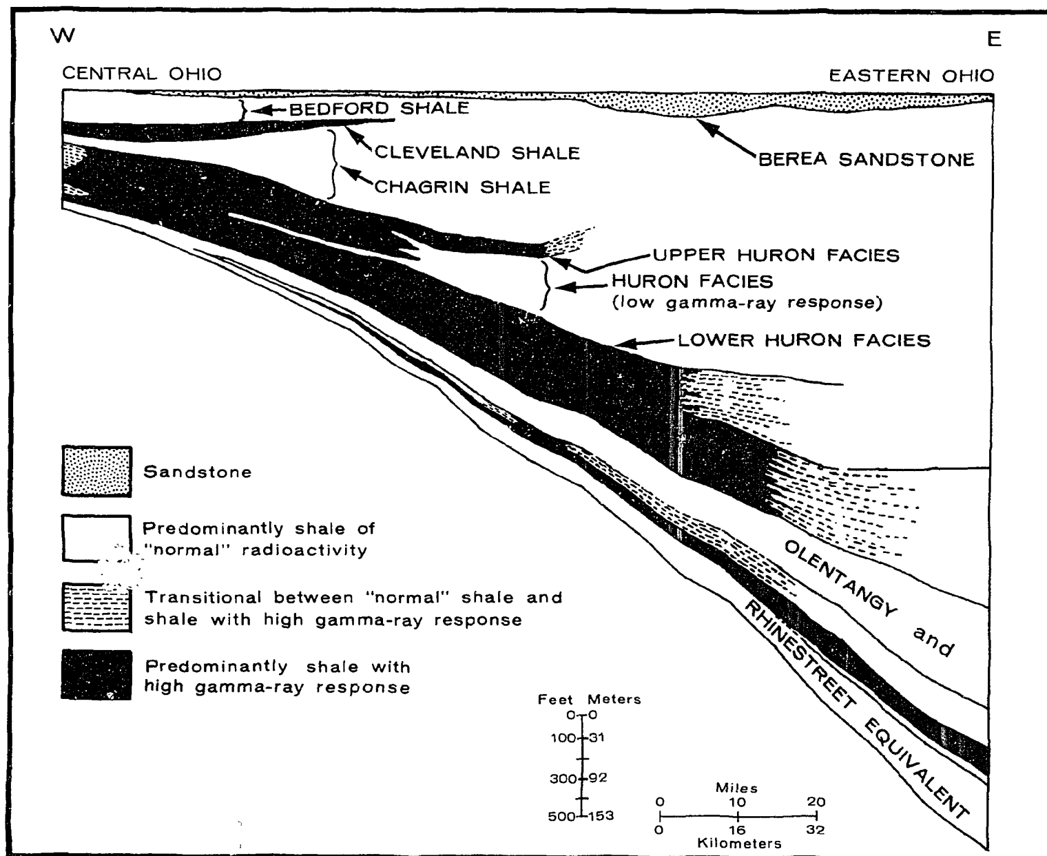
FIGURE 3-24. WEST-EAST STRATIGRAPHIC CROSS SECTION SHOWING RELATIONSHIP BETWEEN SHALES WITH HIGH GAMMA-RAY RESPONSES ("RADIOACTIVE" FACIES) AND OTHER LITHOLOGIES OF UPPER DEVONIAN-LOWER MISSISSIPPIAN IN EASTERN OHIO (MODIFIED FROM MAJCHSZAK, 1978)
