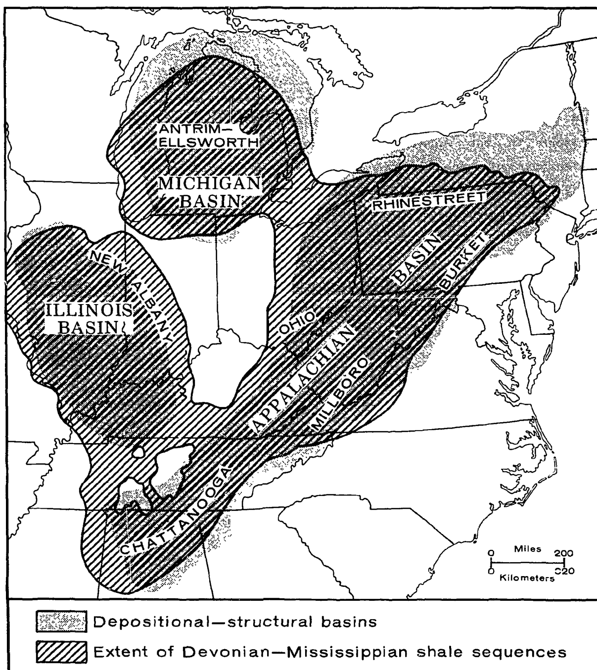
FIGURE 3-11. MAP SHOWING LOCATION OF APPALACHIAN, ILLINOIS, AND MICHIGAN BASINS; PRESENT EXTENT OF DEVONIAN-MISSISSIPPIAN SHALE SEQUENCE; AND REGIONAL POSITION OF SEVERAL WELL-KNOWN SHALE FORMATION NAMES (MODIFIED IN PART FROM PROVO ET AL., 1978)
