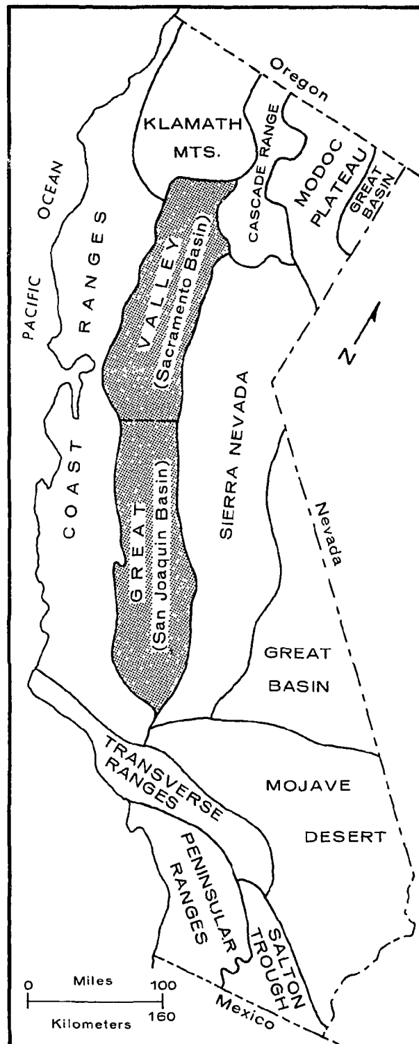
FIGURE 10-1. MAP SHOWING LOCATION OF GREAT VALLEY (SAN JOAQUIN AND SACRAMENTO BASINS) AND OTHER GEOLOGIC PROVINCES OF CALIFORNIA
