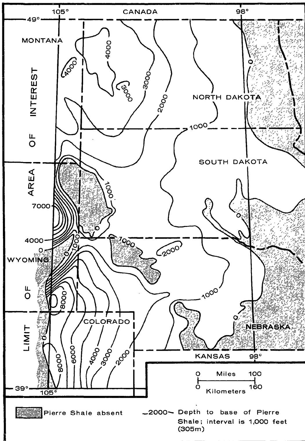
FIGURE 6-30. MAP SHOWING DEPTH FROM SURFACE TO BASE OF PIERRE SHALE IN NORTHERN GREAT PLAINS (MODIFIED FROM SHURR, 1977)
