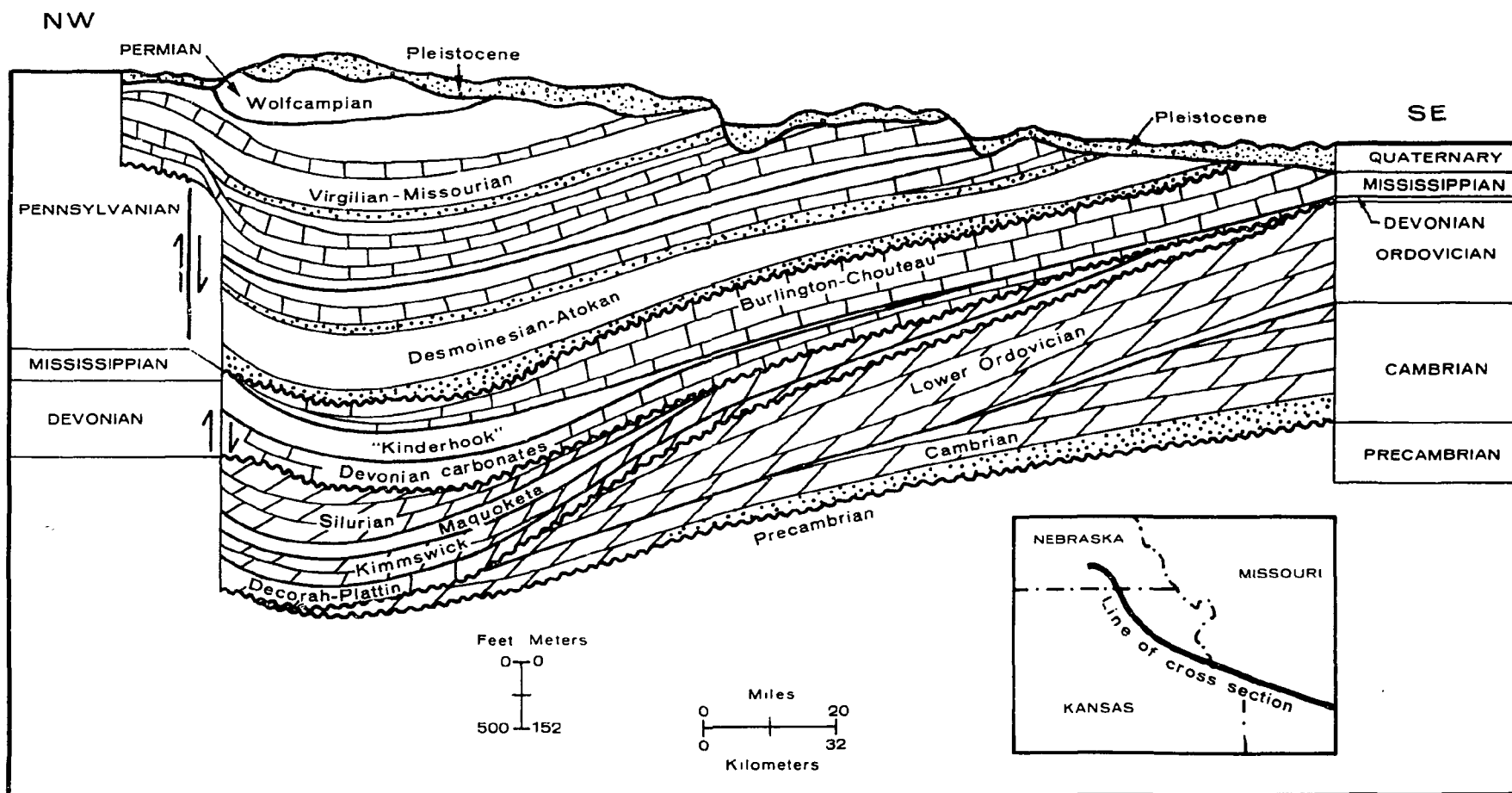
FIGURE 6-9. DIAGRAMMATIC NORTHWEST-SOUTHEAST LITHOLOGIC CROSS SECTION OF FOREST CITY BASIN (MODIFIED FROM WELLS, 1971)
