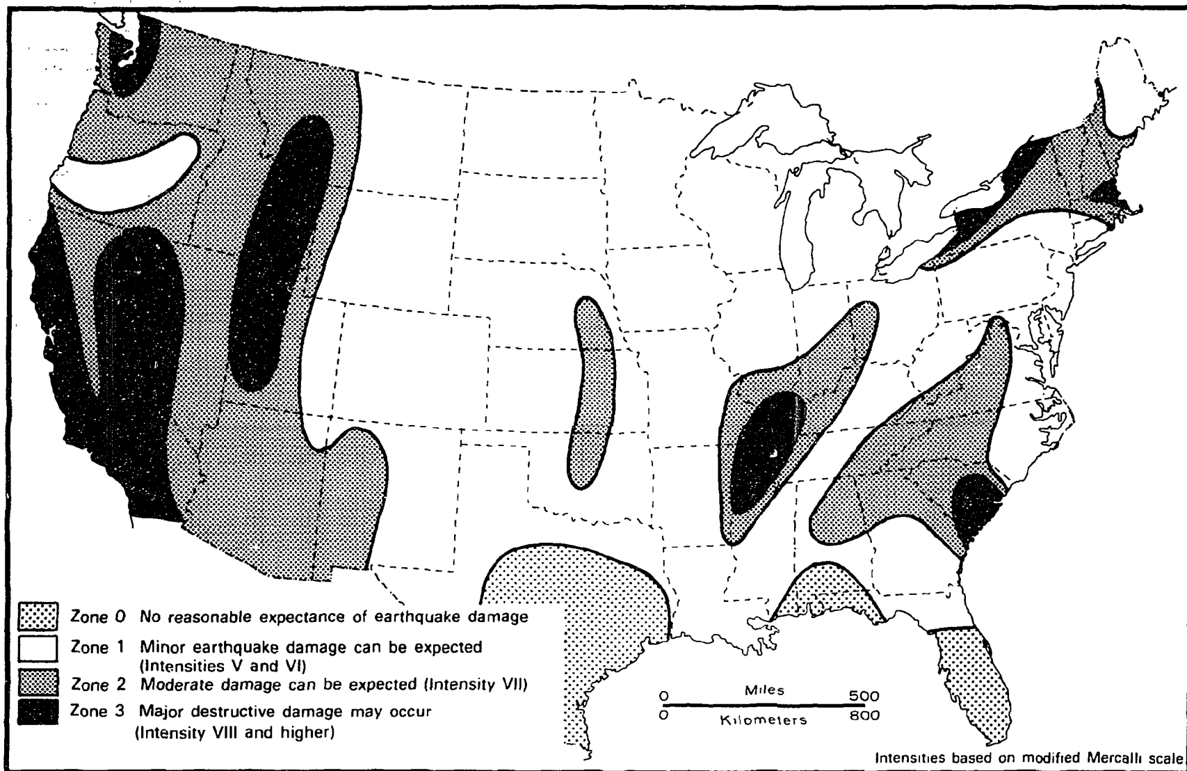
FIGURE 1-3a. MAP OF UNITED STATES SHOWING SEISMIC HAZARD BASED UPON SEISMIC-RISK ZONATION (a) AND PROBABILITY OF GROUND SHAKING (b) (MODIFIED FROM ALGERMISSEN, 1969; ALGERMISSEN AND PERKINS, 1976)
