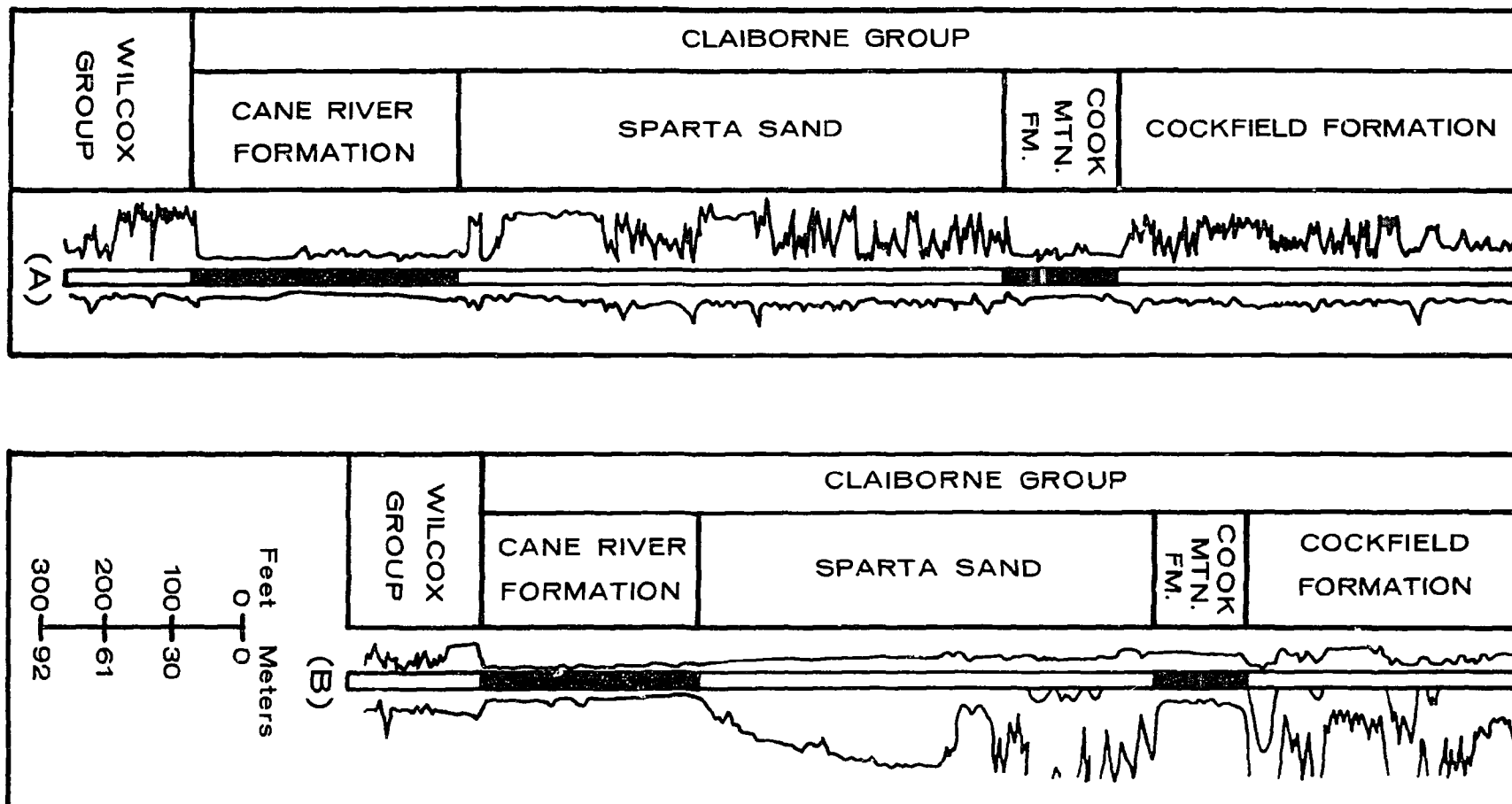
FIGURE 5-8. DIAGRAM SHOWING ELECTRIC-LOG RESPONSES FOR CANE RIVER AND COOK MOUNTAIN FORMATIONS IN COMPARISON TO OTHER CLAIBORNE GROUP UNITS (MODIFIED FROM ROLLO, 1960)
