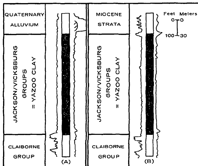
FIGURE 5-10. DIAGRAM SHOWING TYPICAL ELECTRIC-LOG RESPONSE OF JACKSON AND VICKSBURG GROUPS (= YAZOO CLAY) WHERE OVERLAIN BY ALLUVIUM (A) AND BY MIOCENE STRATA (B). (MODIFIED FROM ROLLO, 1960)
