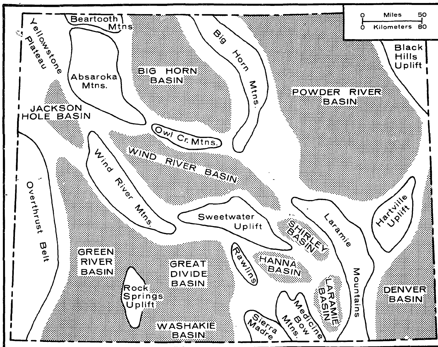
FIGURE 7-1. MAP OF WYOMING SHOWING MAJOR BASINS AND UPLIFTS IN CENTRAL PART OF ROCKY MOUNTAIN PROVINCE (MODIFIED FROM GLASS ET AL., 1975)
