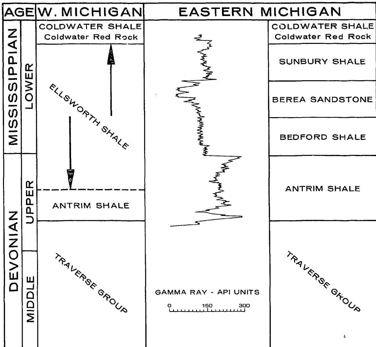
FIGURE 3-17. CHART SHOWING STRATIGRAPHIC RELATIONSHIP WITHIN DEVONIAN-MISSISSIPPIAN SHALE SEQUENCE BETWEEN EASTERN AND WESTERN PARTS OF MICHIGAN BASIN. ALSO SHOWN IS GAMMA-RAY BOREHOLE-LOG RESPONSE FOR SHALE SEQUENCE IN SANILAC COUNTY IN EASTERN MICHIGAN (MODIFIED FROM ELLS, 1979)
