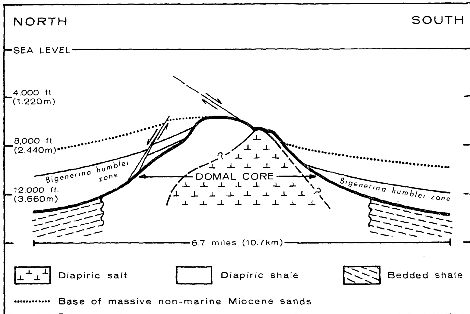
FIGURE 5-14. NORTH-SOUTH STRUCTURAL CROSS SECTION THROUGH VALENTINE SALT DOME, LA FOURCHE PARISH, LOUISIANA, SHOWING RELATIONSHIP OF DIAPIRIC SHALE MASS TO SALT CORE AND SURROUNDING NORMAL-BEDDED STRATA (MODIFIED FROM ATWATER AND FORMAN, 1959)
