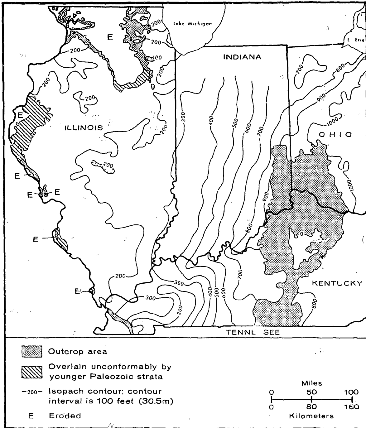
FIGURE 3-3. MAP SHOWING THICKNESS OF MAQUOKETA GROUP IN ILLINOIS BASIN (MODIFIED FROM BOND ET AL., 1971; WILLMAN ET AL., 1975)
