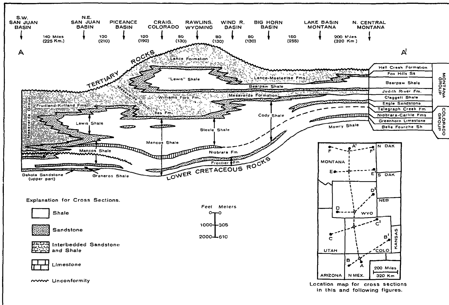
FIGURE 6-22. GENERALIZED STRATIGRAPHIC CROSS SECTION A-A', SHOWING UPPER CRETACEOUS SHALES AND ASSOCIATED STRATA IN NORTHERN GREAT PLAINS, ROCKY MOUNTAINS, AND COLORADO PLATEAU (MODIFIED FROM WEIMER, 1960; MCGOOKEY ET AL., 1972). SEE FOLLOWING FIGURES FOR OTHER CROSS SECTIONS
