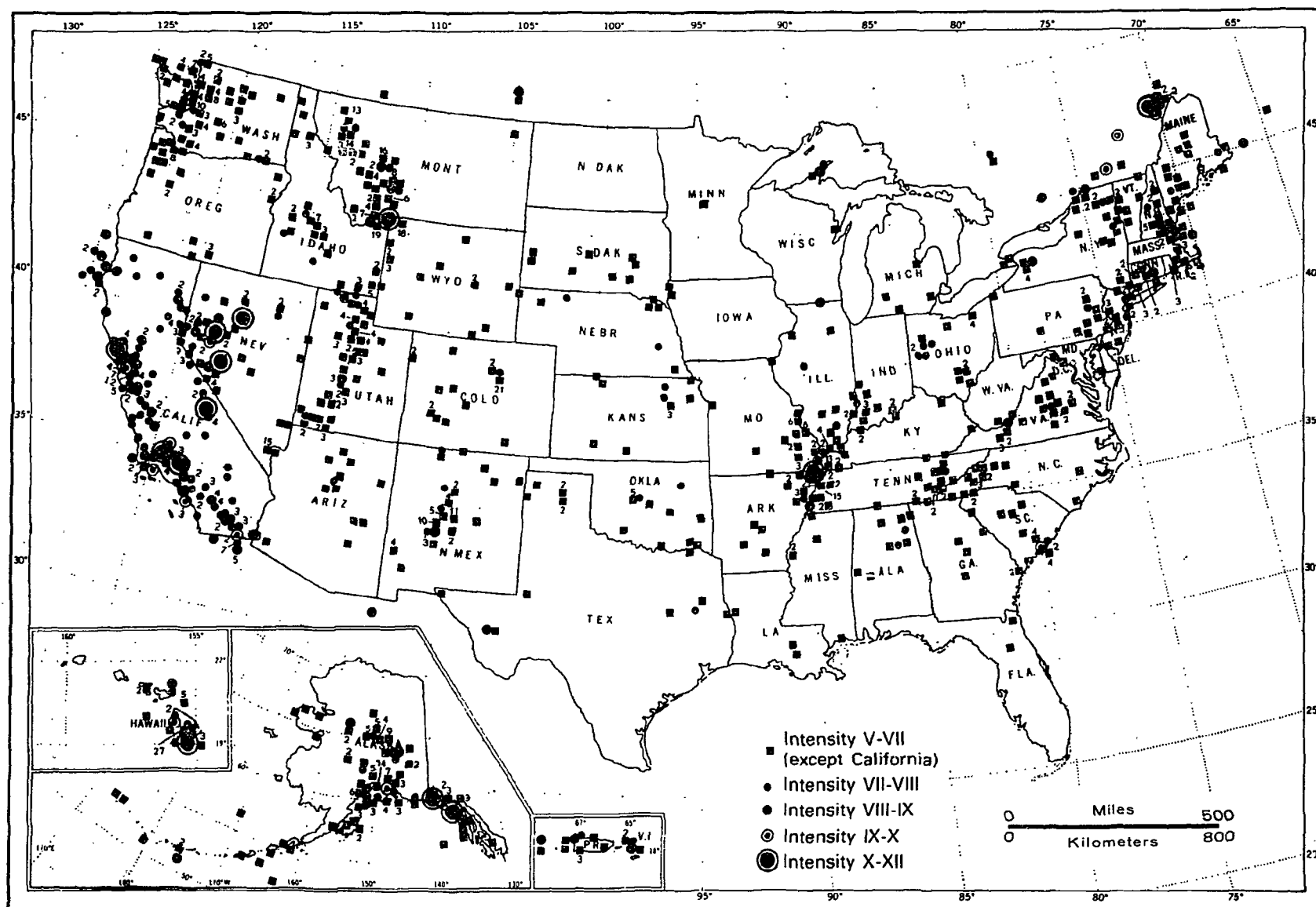
FIGURE 1-2. MAP OF UNITED STATES SHOWING LOCATIONS AND INTENSITY OF HISTORICALLY RECORDED EARTHQUAKES THROUGH 1970 (MODIFIED FROM COFFMAN AND VON HAKE, 1973)
