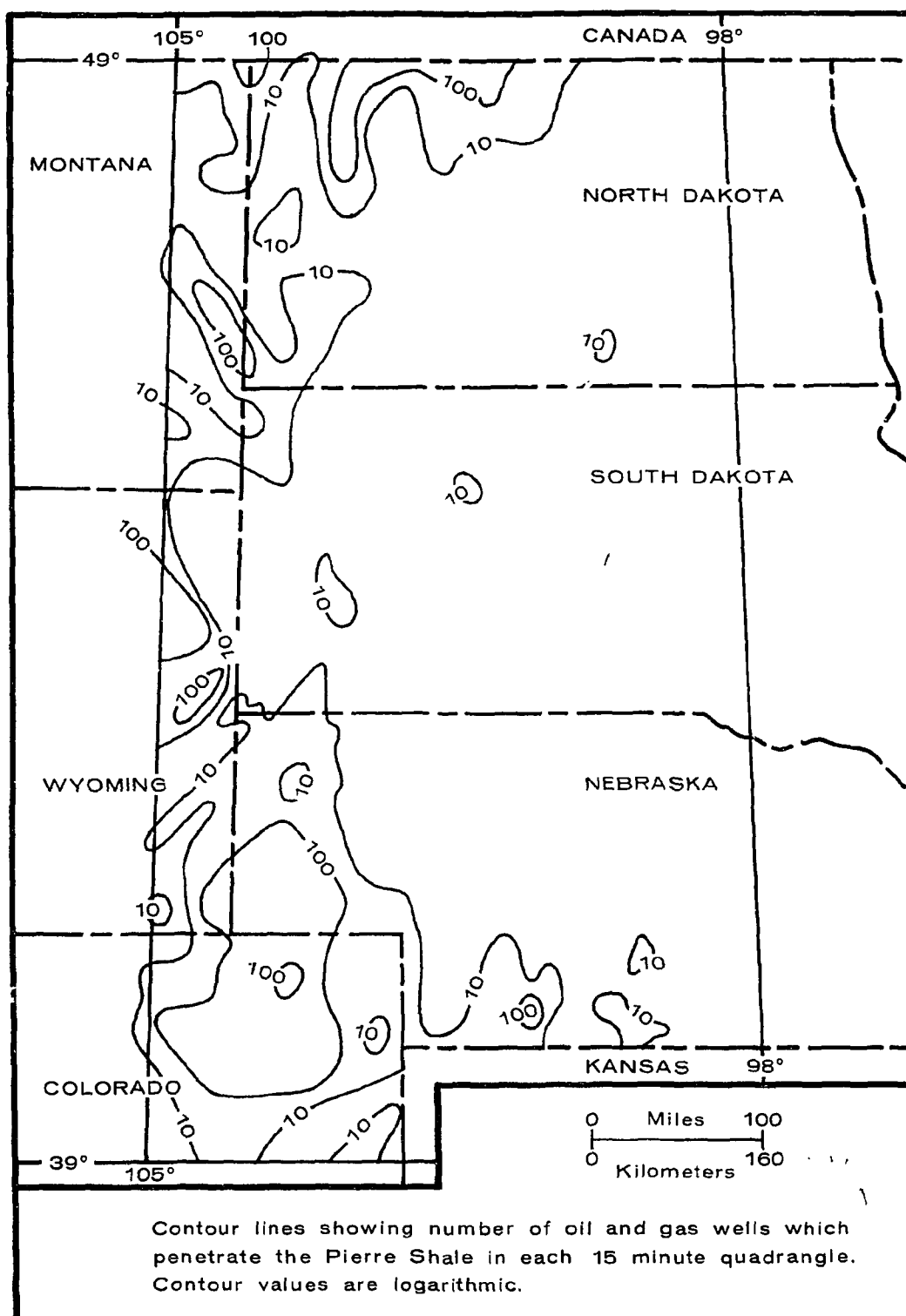
FIGURE 6-32. MAP SHOWING NUMBER OF OIL AND GAS WELLS THAT PENETRATE PIERRE SHALE IN NORTHERN GREAT PLAINS (MODIFIED FROM SHURR, 1977). BASED ON RECORDS OF 33,000 WELLS
