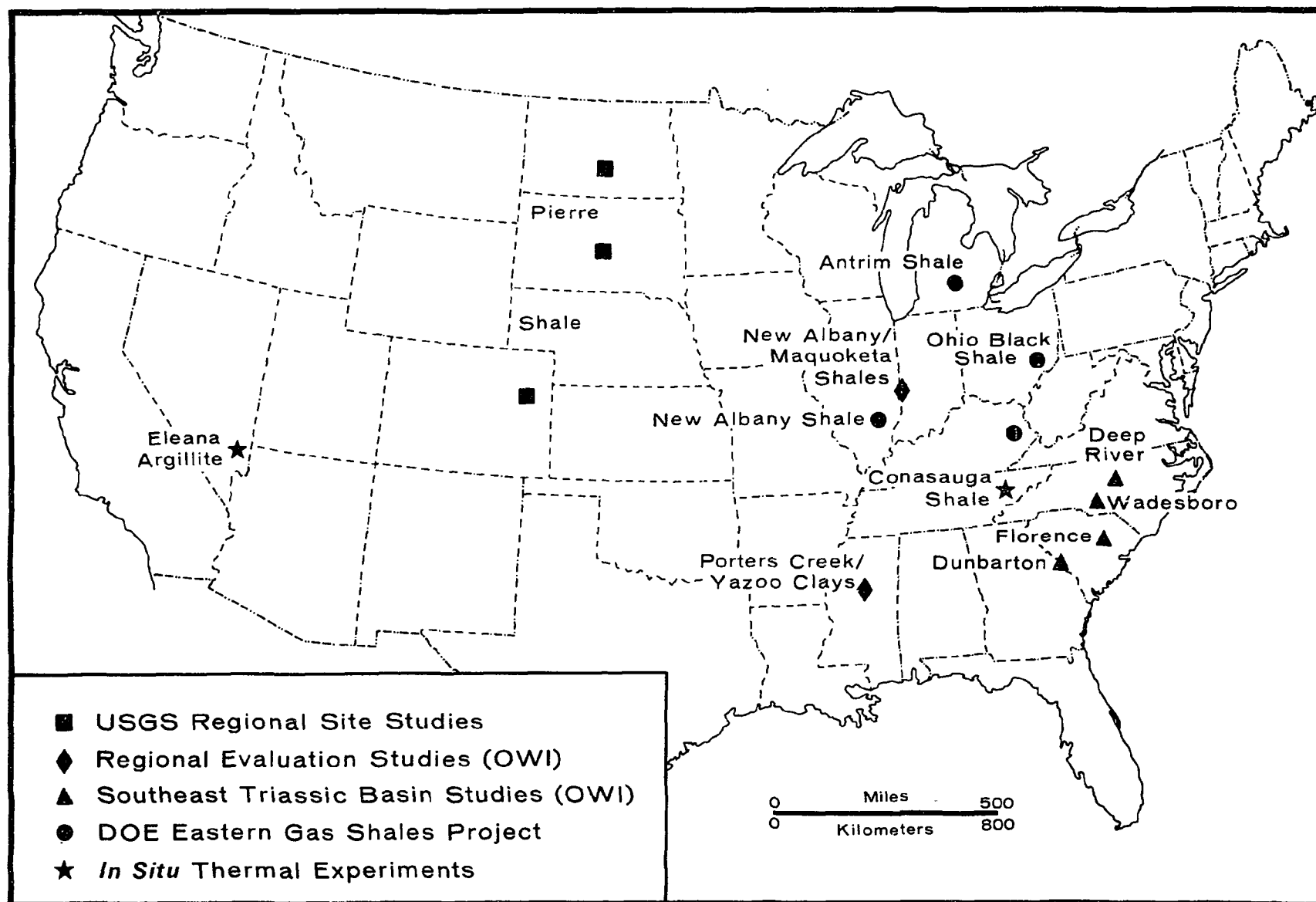
FIGURE 1-1. MAP OF UNITED STATES SHOWING LOCATIONS OF PREVIOUS FIELD AND SUBSURFACE STUDIES AND IN SITU THERMAL EXPERIMENTS CONDUCTED ON ARGILLACEOUS STRATA
