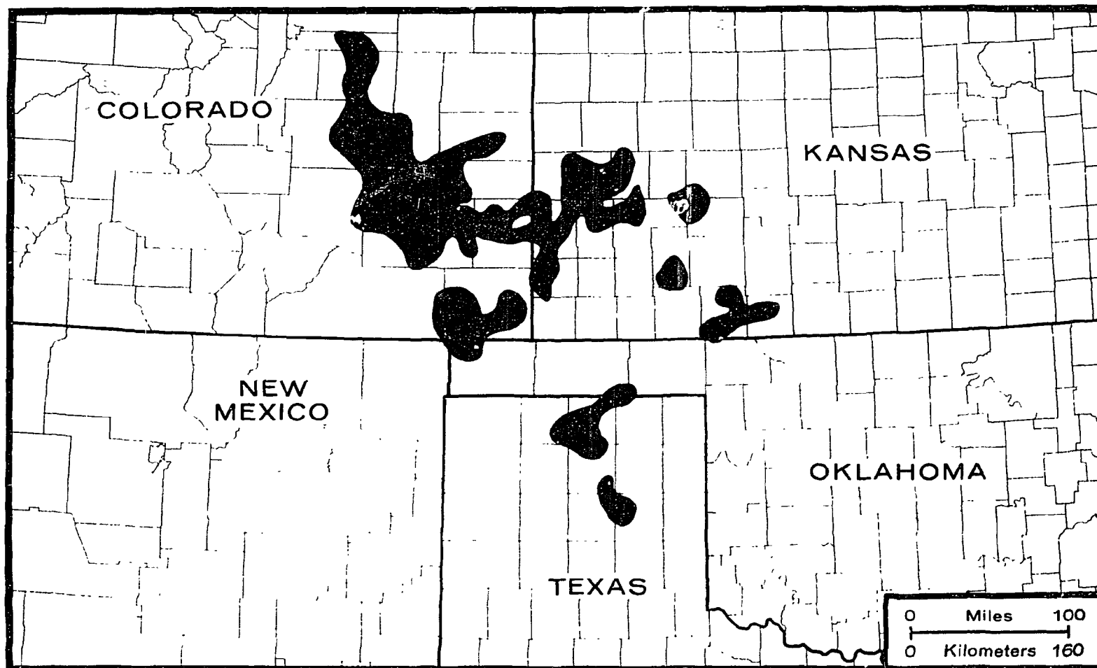
FIGURE 6-20. MAP OF CENTRAL AND SOUTHERN MIDCONTINENT REGION, SHOWING DISTRIBUTION OF ARGILLACEOUS FACIES, IN A RATIO OF AT LEAST 4:1, OF GUADALUPIAN ROCKS MORE THAN 75 M THICK (MODIFIED FROM MCKEE ET AL., 1967b)
