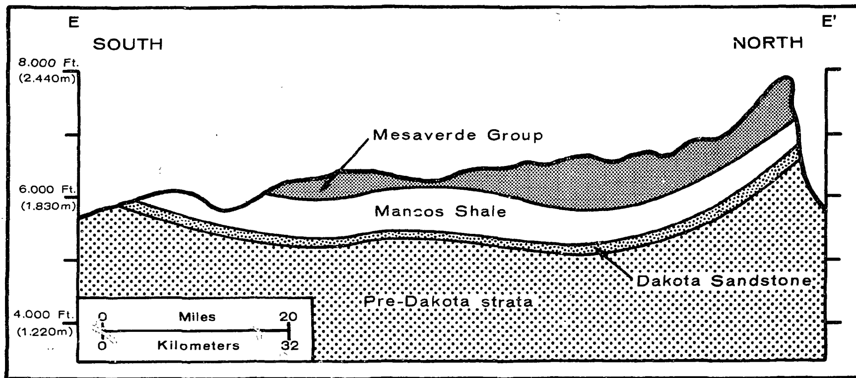
FIGURE 8-6. CROSS SECTION E-E', SHOWING MANCOS SHALE IN BLACK MESA BASIN OF NORTHEASTERN ARIZONA (MODIFIED FROM PIERCE ET AL., 1970)
