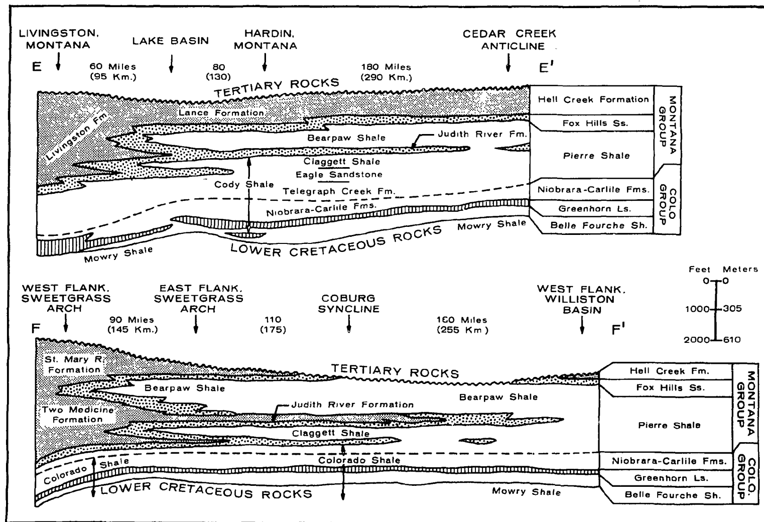
FIGURE 6-25. GENERALIZED STRATIGRAPHIC CROSS SECTIONS E-E' AND F-F', SHOWING UPPER CRETACEOUS SHALES AND ASSOCIATED STRATA IN NORTHERN GREAT PLAINS AND ROCKY MOUNTAINS (MODIFIED FROM WEIMER, 1960; MCGOOKEY ET AL., 1972). SEE FIGURE 6-22 FOR LOCATION MAP AND EXPLANATION
