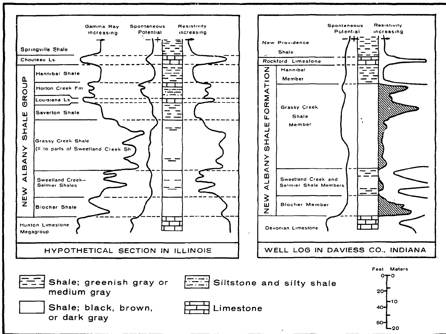
FIGURE 3-15. DIAGRAM SHOWING BOREHOLE-LOG RESPONSES OF STRATIGRAPHIC DIVISIONS OF NEW ALBANY SHALE GROUP IN ILLINOIS AND NEW ALBANY SHALE FORMATION IN INDIANA (MODIFIED FROM BASSETT AND HASENMUELELR, 1977; REINBOLD, 1978; CLUFF ET AL., 1981)
