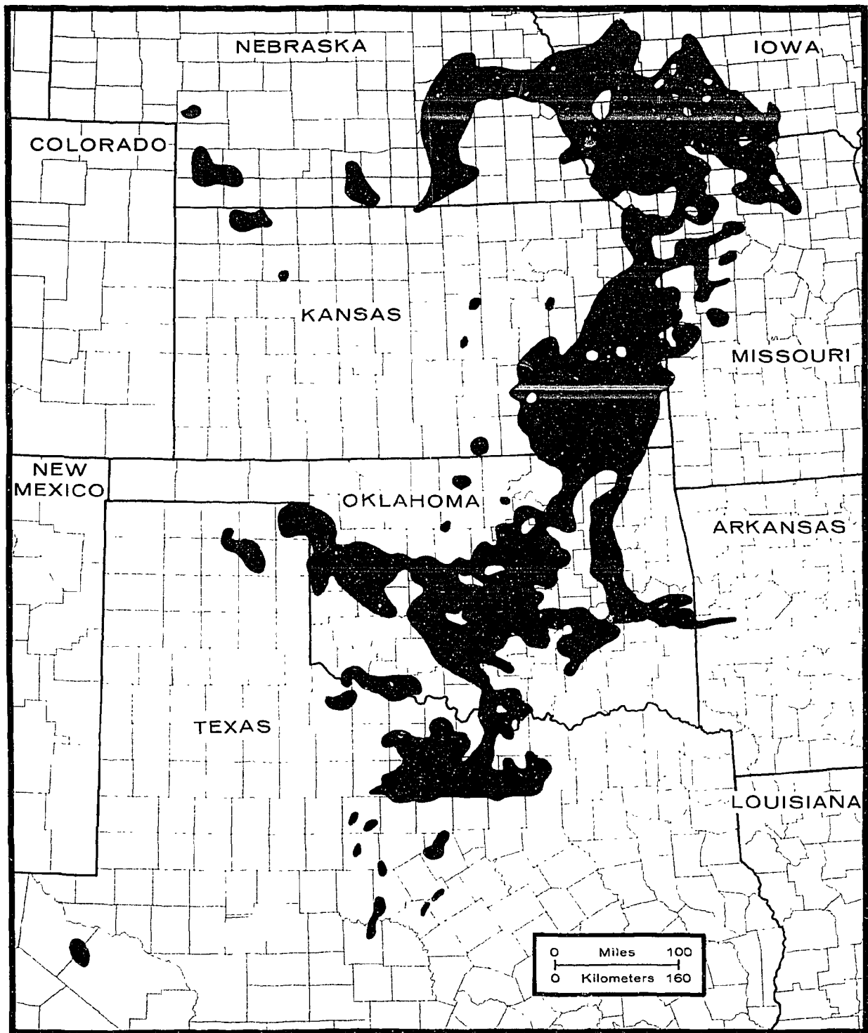
FIGURE 6-15. MAP OF CENTRAL AND SOUTHERN MIDCONTINENT REGION, SHOWING DISTRIBUTION OF ARGILLACEOUS FACIES, IN A RATIO OF AT LEAST 4:1, OF DESMOINESIAN ROCKS MORE THAN 75 M THICK (MODIFIED FROM MCKEE AND CROSBY, 1975)
