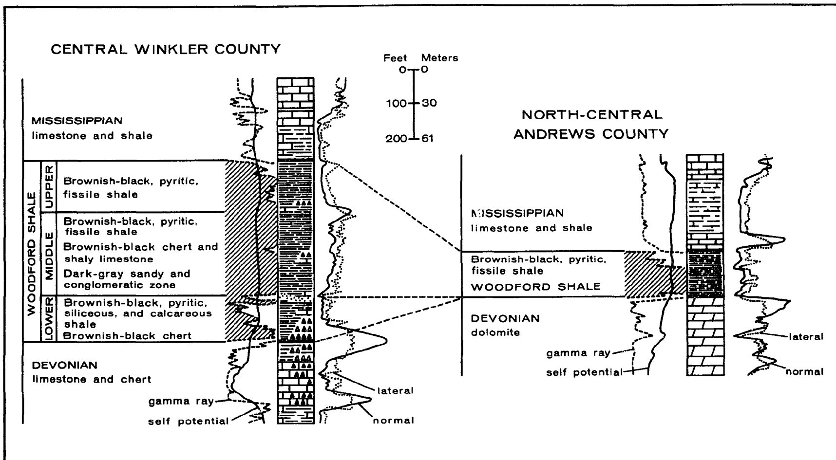
FIGURE 6-6. LOG SECTION SHOWING LITHOLOGY AND CHANGE IN THICKNESS OF WOODFORD SHALE FROM WINKLER COUNTY NORTHEASTWARD TO ADJOINING ANDREWS COUNTY, WEST TEXAS (MODIFIED FROM ELLISON, 1950)
