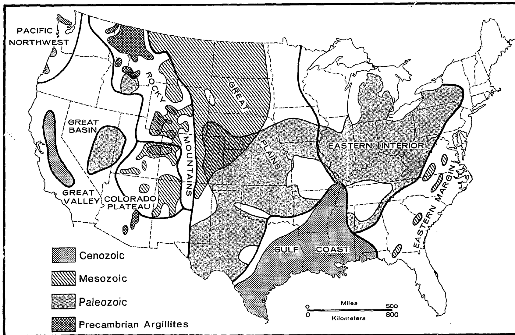
FIGURE 2-1. MAP OF UNITED STATES SHOWING DISTRIBUTION OF PRINCIPAL SHALES BY GENERAL GEOLOGIC AGE, AND REGIONS UNDER WHICH EACH SHALE UNIT IS DISCUSSED IN THIS REPORT
