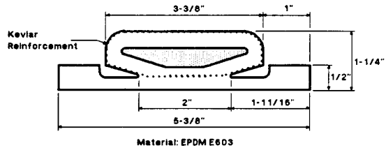
(a) "Old" Design
