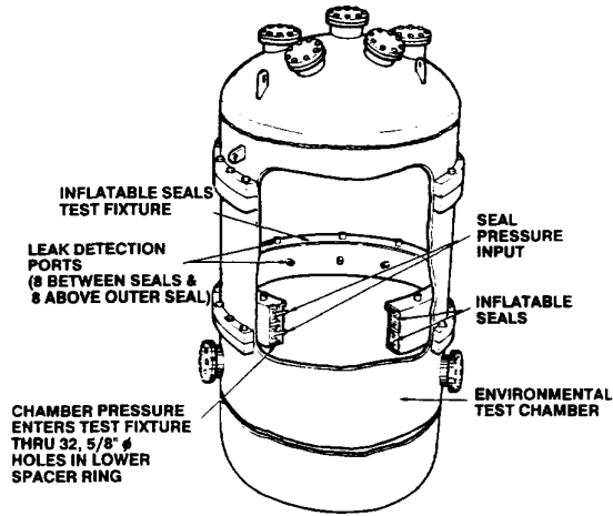
Figure 3. Inflatable Seals Test Fixture Inside Test Chamber
