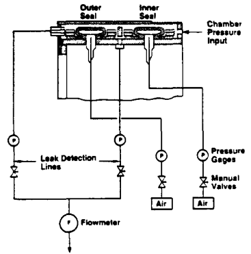
Figure 4. Schematic of Test Setup
