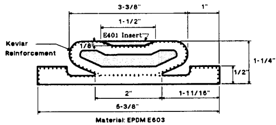
(b) "New" Design
