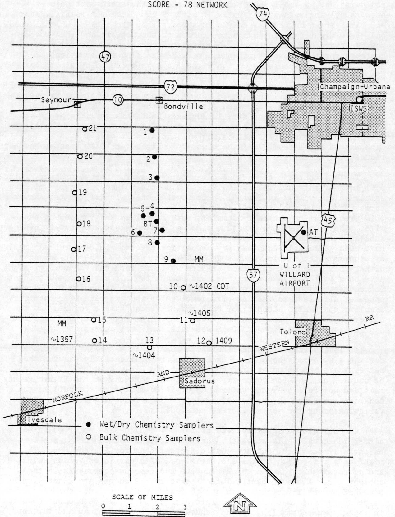
Figure 2. The time of ending of the rainfall for the 1 July 1978 single shower.
