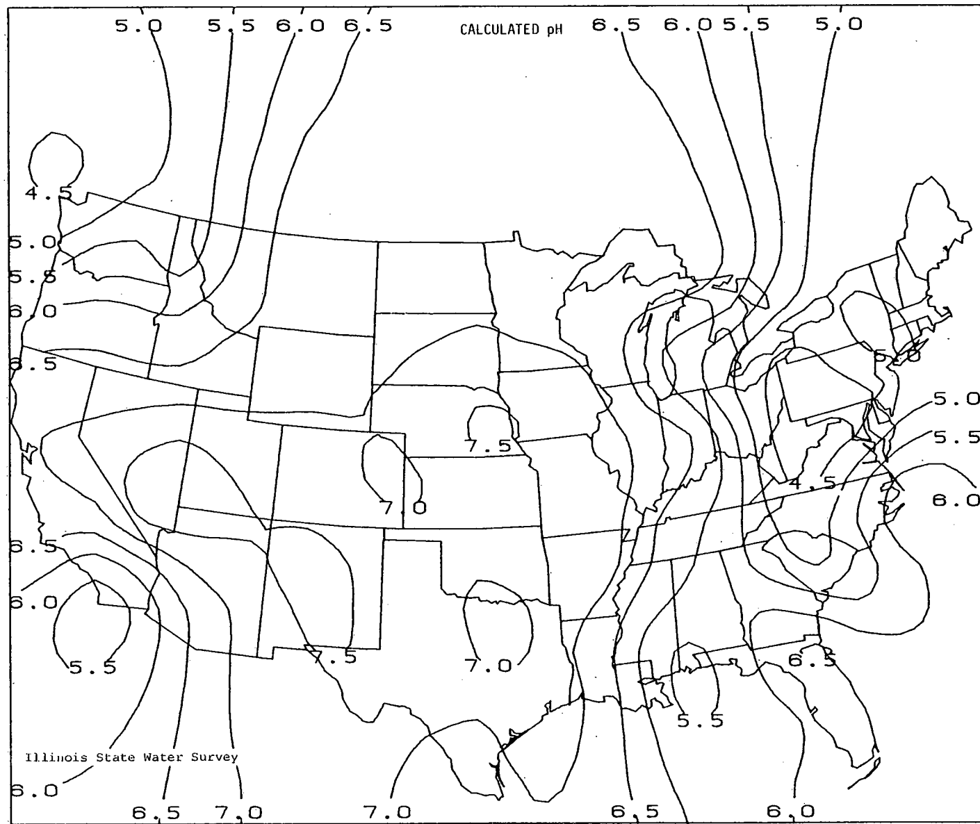
Figure 12. pH values calculated for the 1955-56 Junge data using Eqs. 11 and 5.
