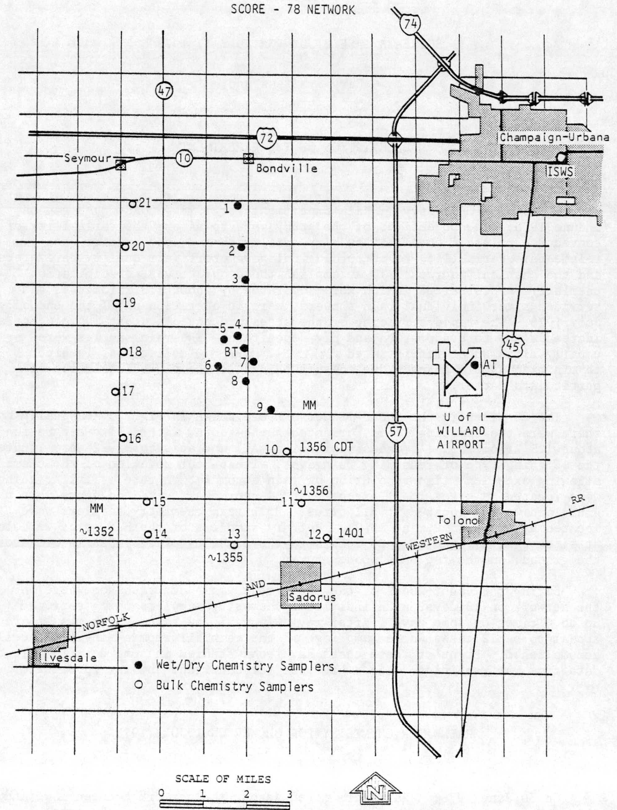
Figure 1. The SCORE-78 network showing the time of beginning of rainfall on 1 July 1978.
