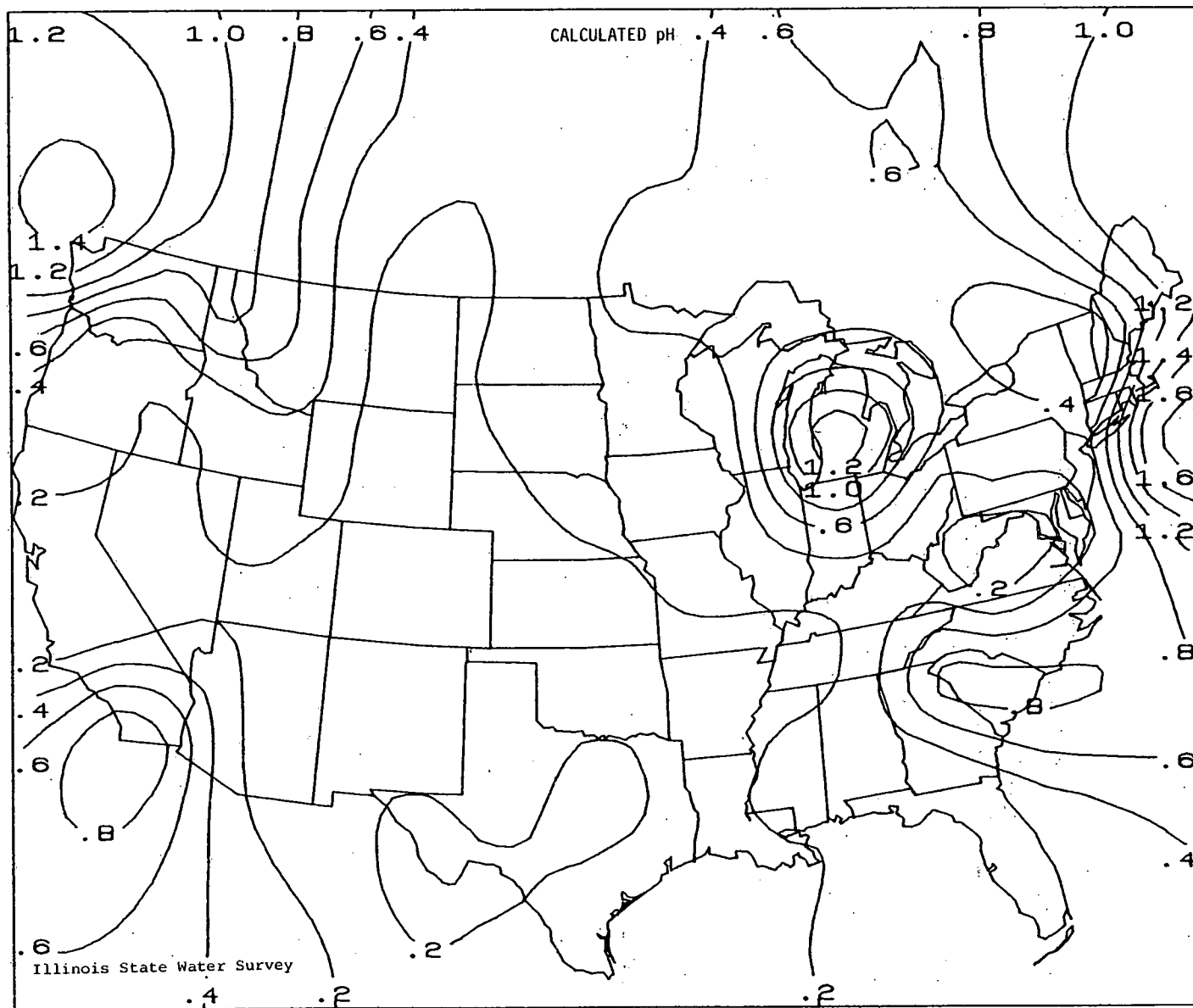
Figure 16. Difference between the pH calculated with twice the (Ca^{++}/Mg^{++}) ratios in Table I and the pH calculated with one half the ratios.
