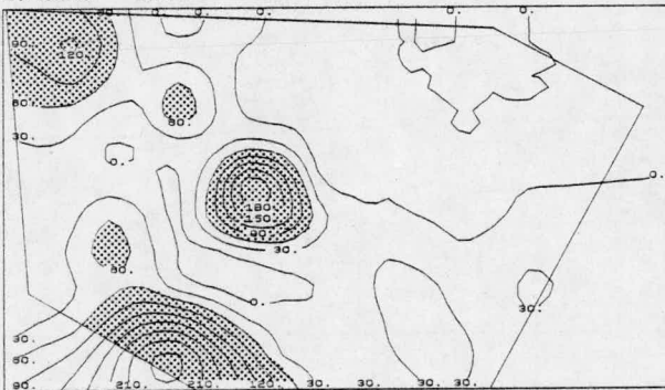
INSOLUBLE Fe DEPOSITION, \text{ng cm}^{-2} LOADING = 0.74
