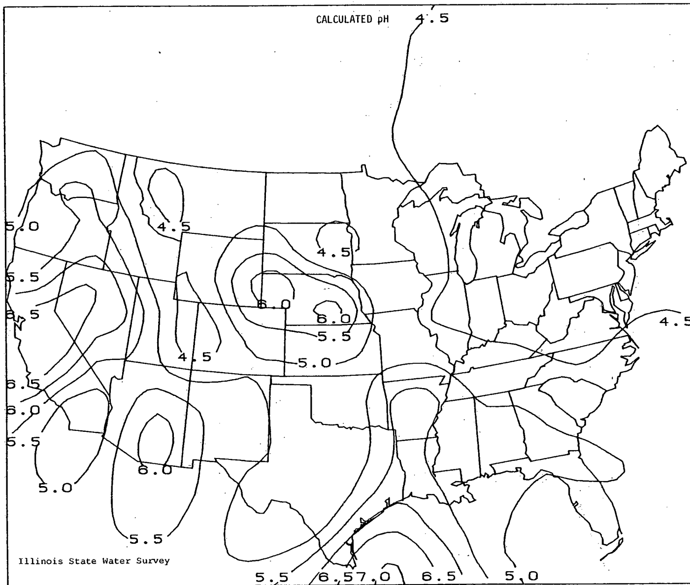
Figure 18. pH values calculated for the 1955-56 Junge data, using Eqs. 1 and 5 and \text{Ca}^{++} concentrations equal to 1/6 those reported by Junge.
