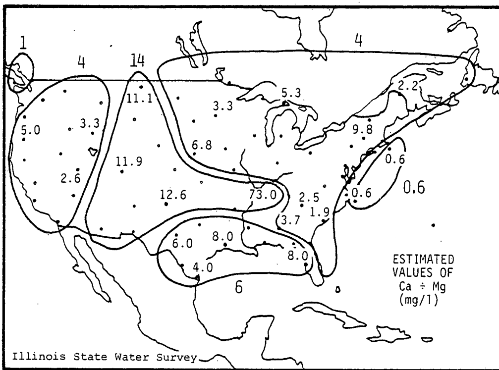
Figure 2. Ratios of Ca^{++} to Mg^{++} for the United States.
