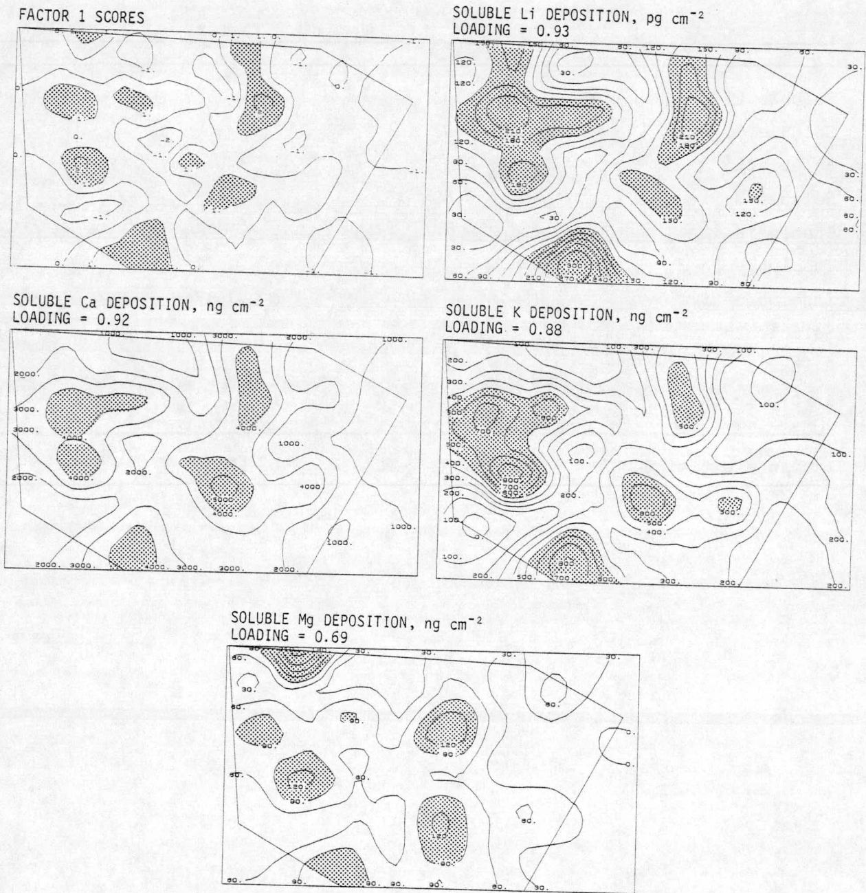
Figure 2. Factor 1 scores and deposition patterns of associated chemical constituents, 13 August 1975.
