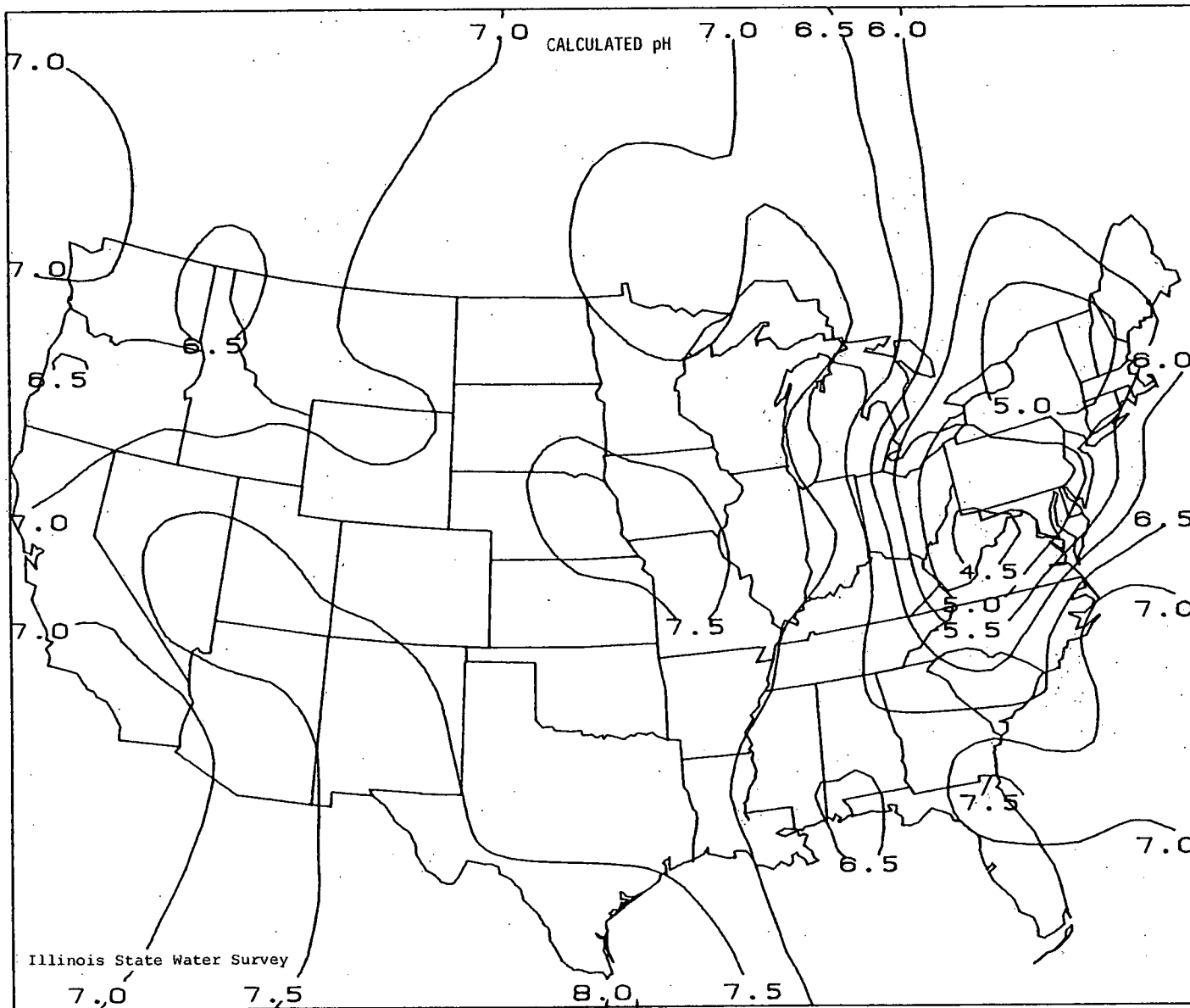
Figure 14. pH values calculated for the 1955-56 Junge data, using Eqs. 1 and 5 and one half the (Ca^{++}/Mg^{++}) ratio values listed in Table I.
