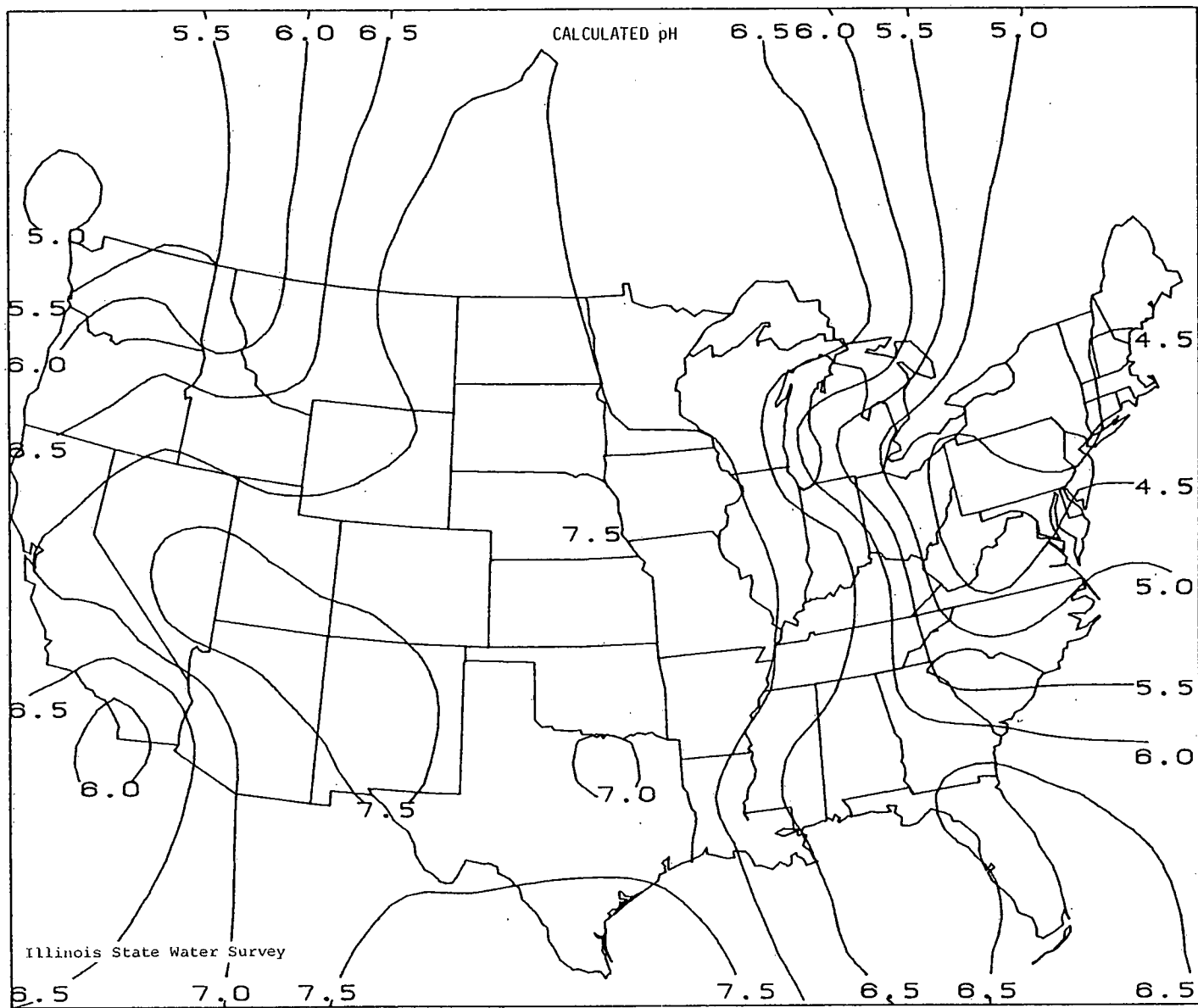
Figure 17. pH values calculated for the 1955-56 Junge data, using Eqs. 1 and 5 and a ratio of \text{Ca}^{++} / \text{Mg}^{++} = 6 at all the Junge sites.
