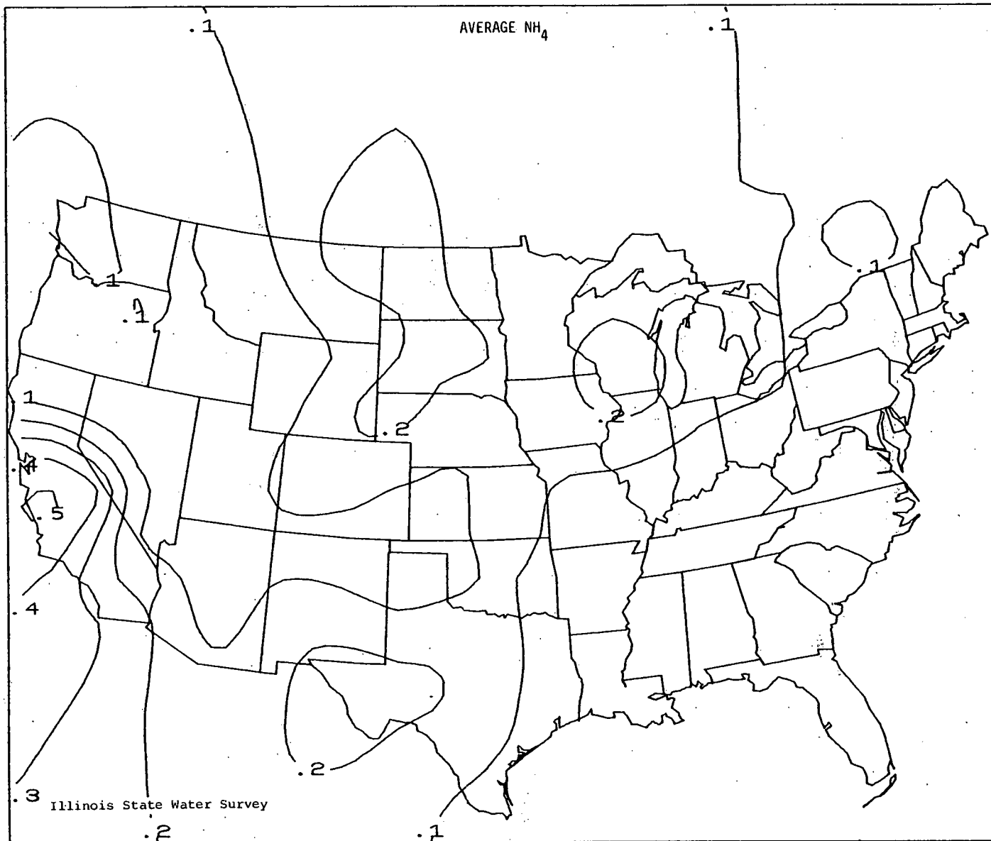
Figure 9. Precipitation-weighted ammonium concentrations (Mg/l) for the 1955-56 Junge data.
