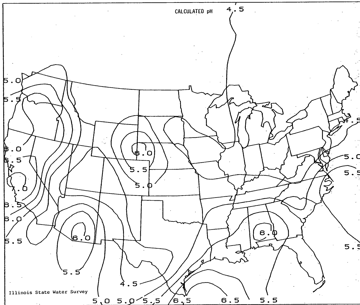
Figure 19. pH values calculated for the 1955-56 Junge data, using Eqs. 1 and 5 and (Ca^{++}) = 0.2 \text{ mg/l} at all the Junge sites.
