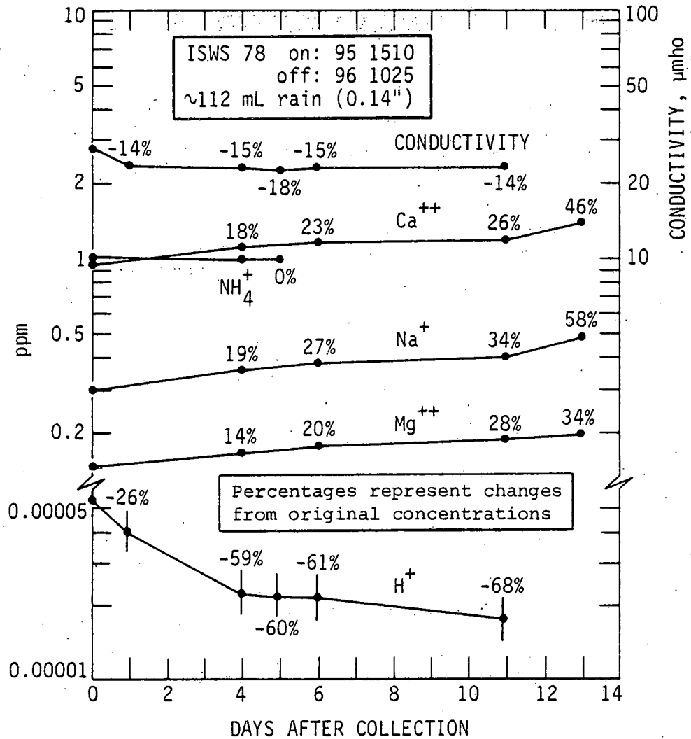
Figure 3. Ionic concentration changes of rain sampled with a HASL wet-dry collector. Exposure time was 19 hours, 15 minutes. The sample was unfiltered and stored in the original collection vessel at 25°C.
