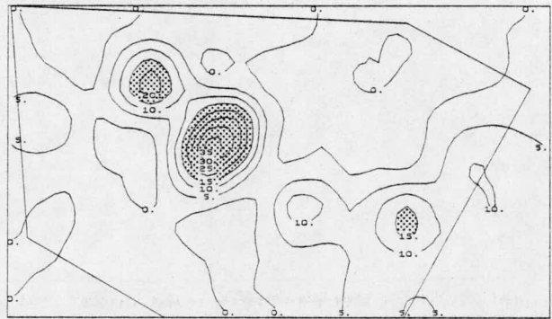
INSOLUBLE K DEPOSITION, \text{ng cm}^{-2} LOADING = 0.78
