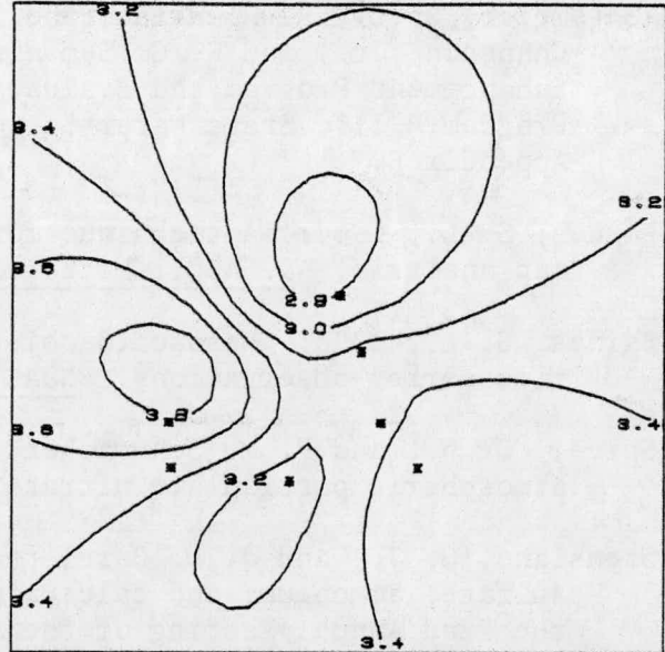
SCORE - GROUP 182 VALUE: NO3 (PPM)
