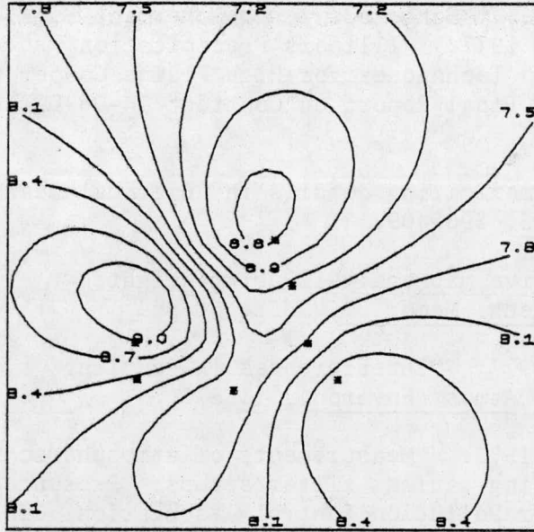
SCORE - GROUP 182 VALUE: SO4 (PPM)
