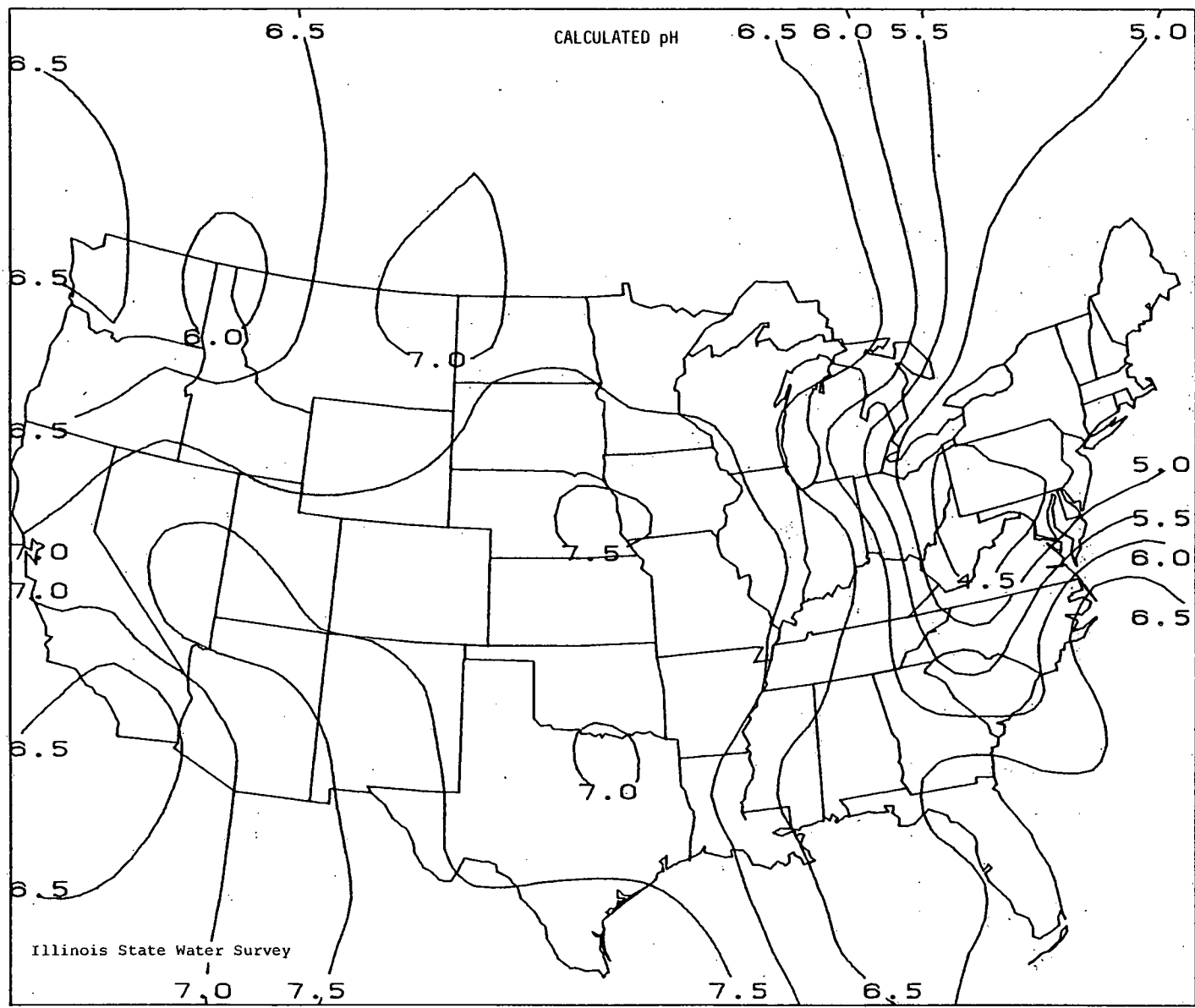
Figure 11. pH values calculated for the 1955-56 Junge data using Eqs. 12 and 5.
