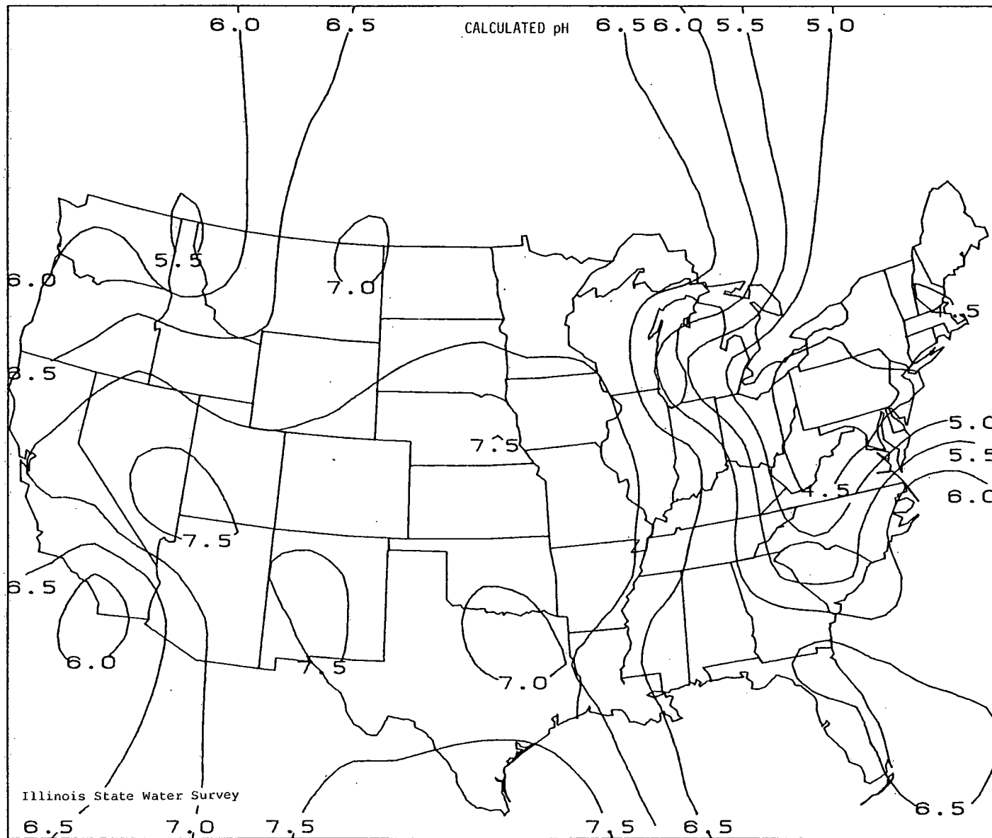
Figure 15. pH values calculated for the 1955-56 Junge data, using Eqs. 1 and 5 and twice the (Ca^{++}/Mg^{++}) ratio values listed in Table 1.
