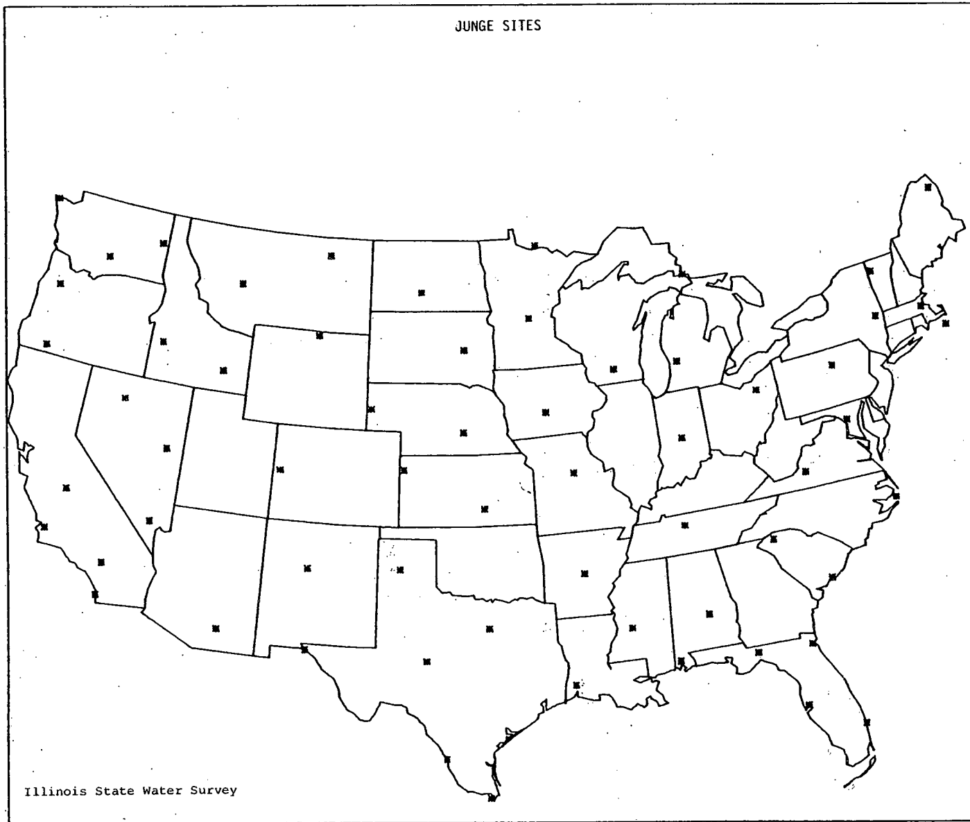
Figure 7. Location of the 1955-56 Junge sites.
