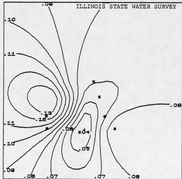
SCORE - GROUP 182 VALUE: MG (PPM)
