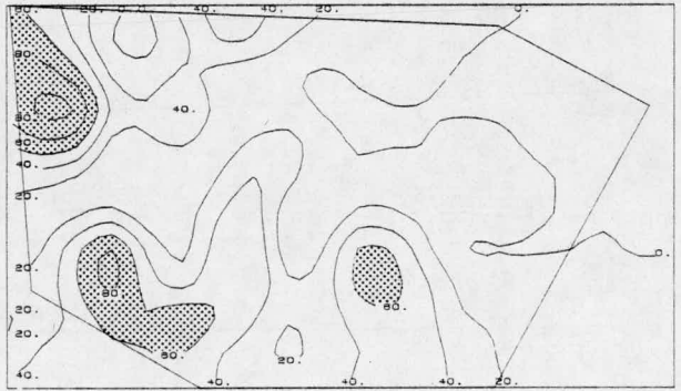
INSOLUBLE Li DEPOSITION, \text{pg cm}^{-2} LOADING = 0.67
