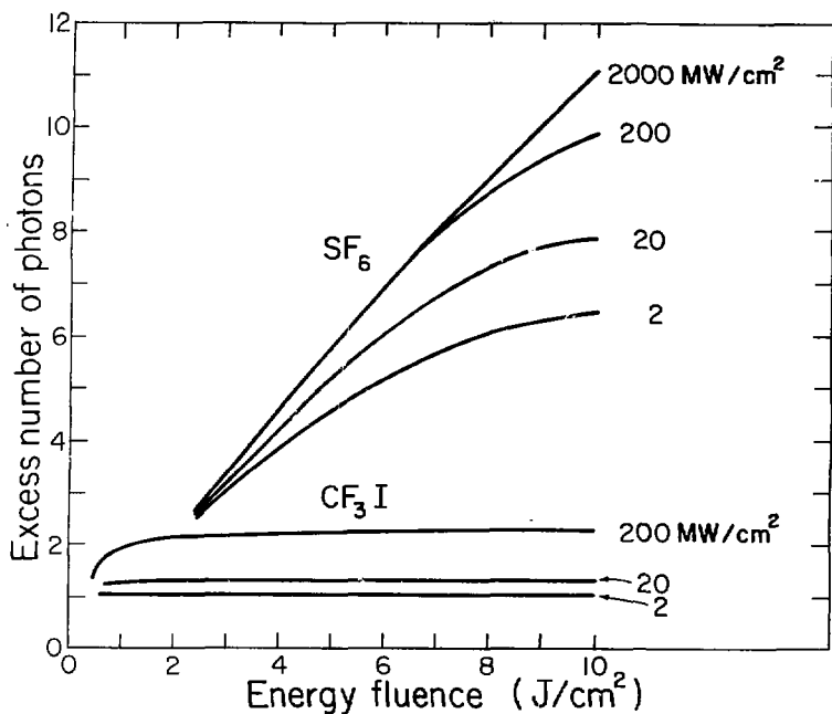
Fig. 5. Excess energy with which \text{CF}_3\text{I} and \text{SF}_6 dissociate for several peak laser intensities and energy fluences below 10 \text{ J}/\text{cm}^2 .
