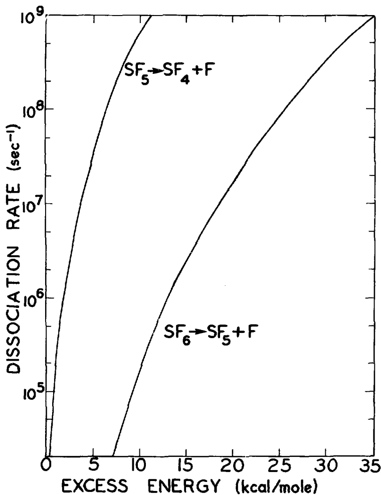
Fig. A1. RRKM calculated rate constant using a dissociation energy of 93 kcal/mole for \text{SF}_6 \rightarrow \text{SF}_5 + \text{F} and a dissociation energy of 51 kcal/mole for \text{SF}_5 \rightarrow \text{SF}_4 + \text{F} .
