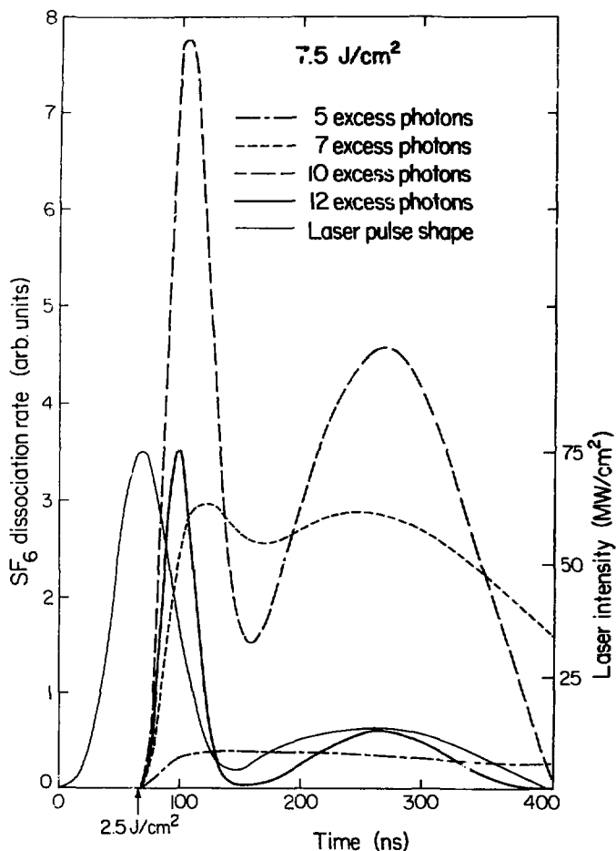
Fig. 7. Excess energies with which \text{SF}_6 dissociates versus time. The \text{CO}_2 TEA laser pulse used in this model calculation is shown by the light solid curve with the intensity scale shown on the right.
