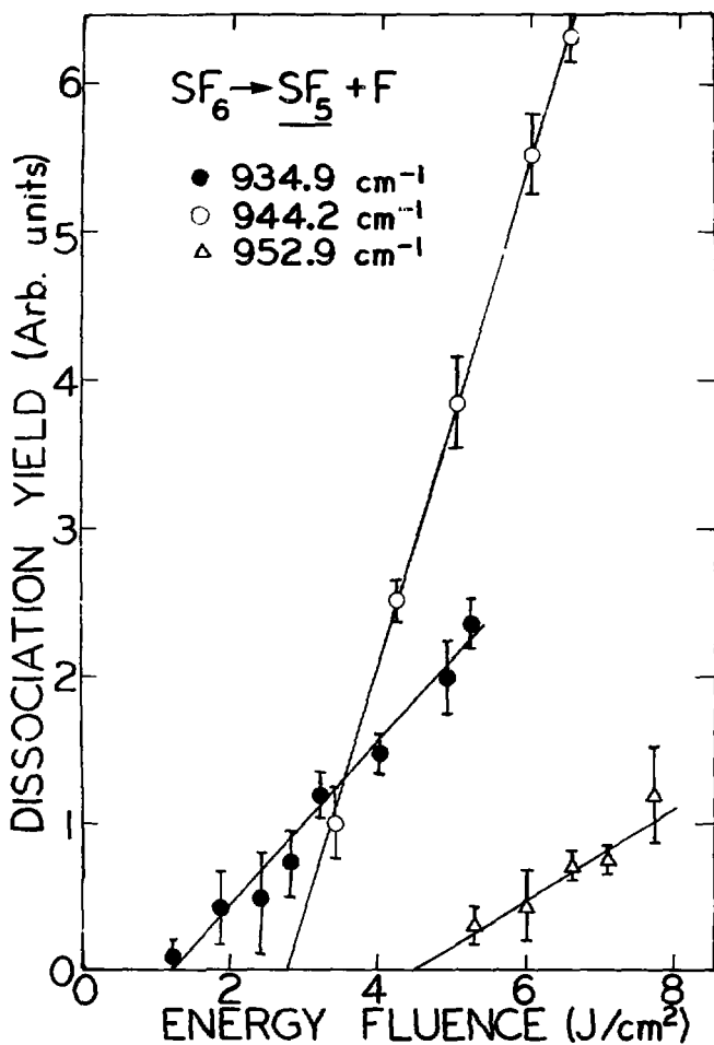
Fig. 7. Energy fluence dependence of \text{SF}_6 MPD at three \text{CO}_2 laser frequencies.
