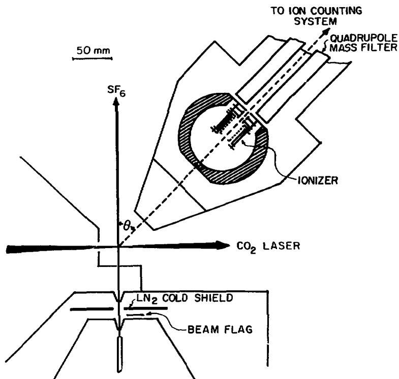
Fig. 1. Diagram of the molecular beam apparatus used for the study of \text{SF}_6 multiphoton dissociation.
