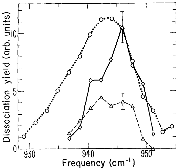
Fig. 9. Frequency spectrum of \text{SF}_6 absorption with a weak \text{CO}_2 laser pulse. Detection was achieved by dissociation with a 10 \text{ J/cm}^2 laser pulse at 1060 \text{ cm}^{-1} .
