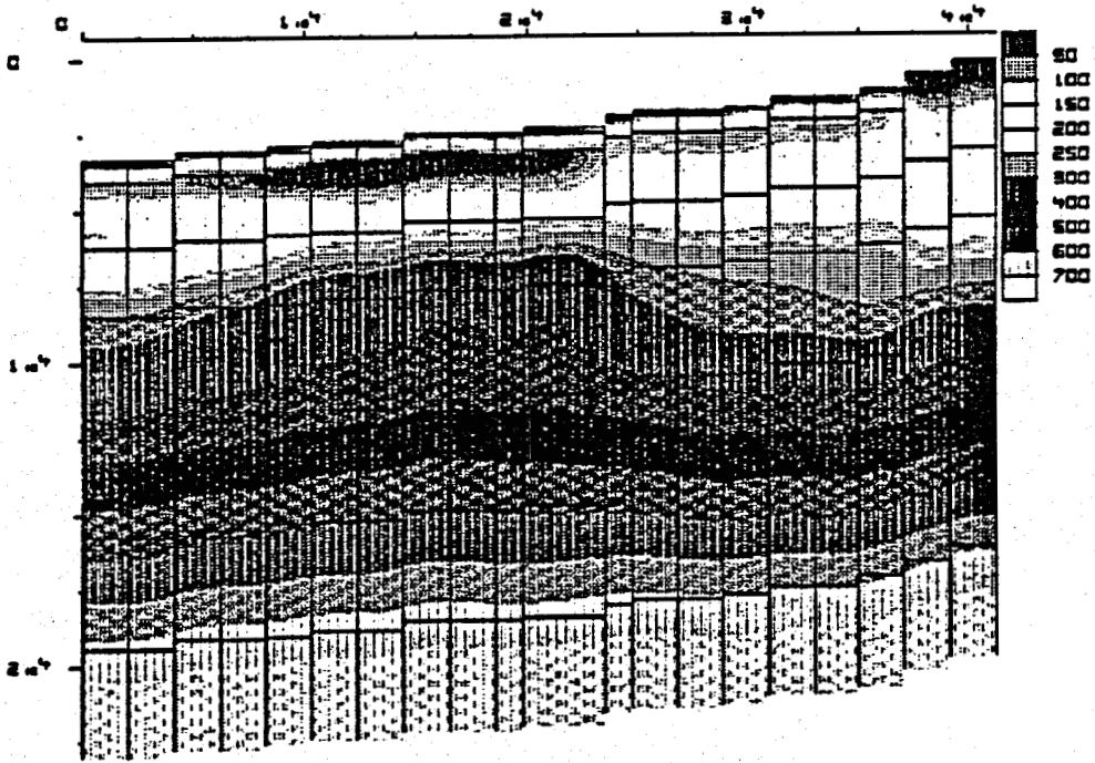
Figure 9 Model temperatures ( ^{\circ}\text{F} ) after 50,000 years for 0.05 mD in mountain massif.
