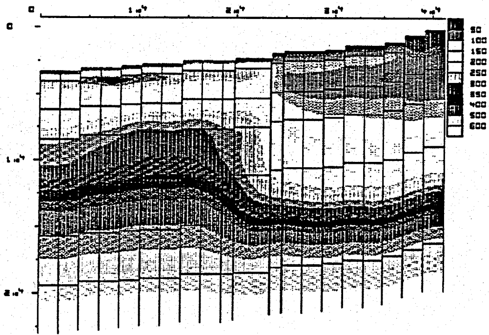
Figure 8 Model temperatures ( ^{\circ} F) after 30,000 years for 0.5 mD in mountain massif.
