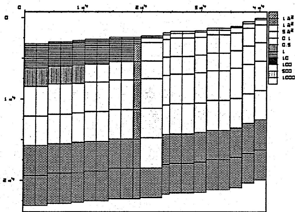
Figure 7 Vertical permeability (mD) used in the simulation study, note 0.5 mD in mountain massif.
