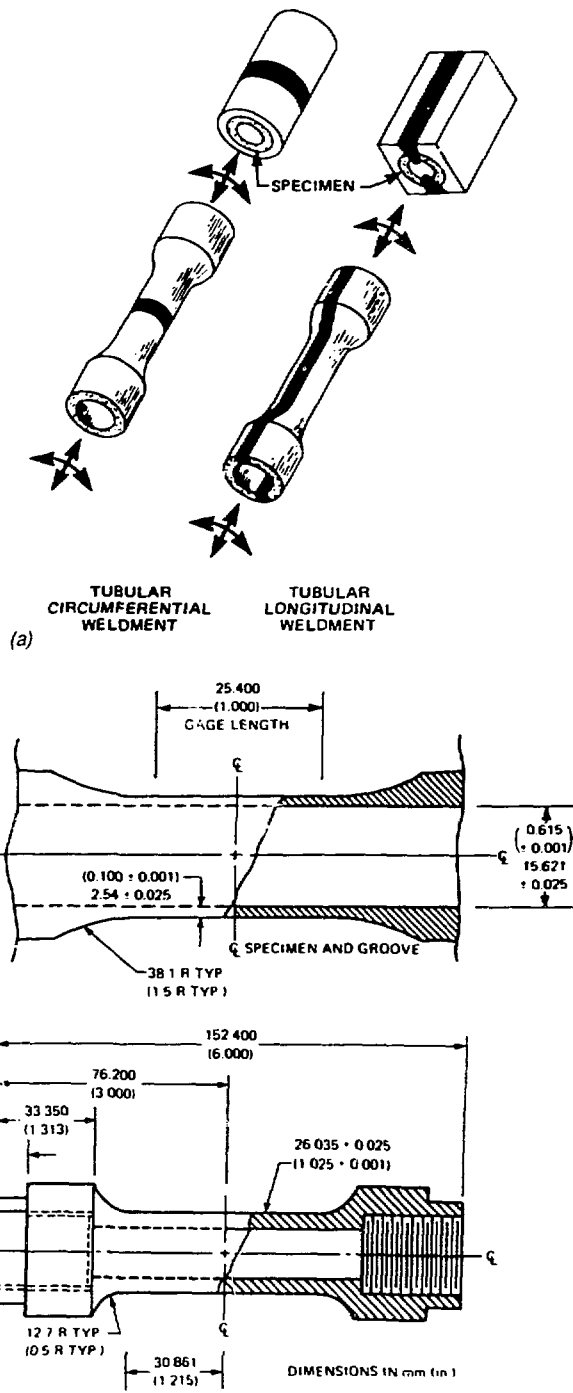
Fig. 2. Weld locations and specimen details. (a) Method of obtaining tubular specimens with welds. (b) Dimensions of creep-rupture specimen.
