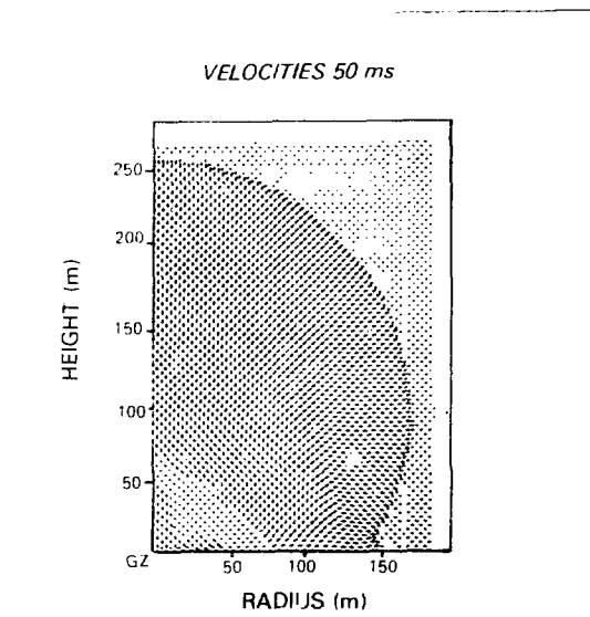
Figure 3. BADGER at 50 ms. The reverse flow is established. Note the counter-clockwise flow in the region within 50 m of GZ. Note in the pressure plot (upper right) that the pressure at GZ has risen, creating a negative gradient. This is an indication of the real transients in the flow.
