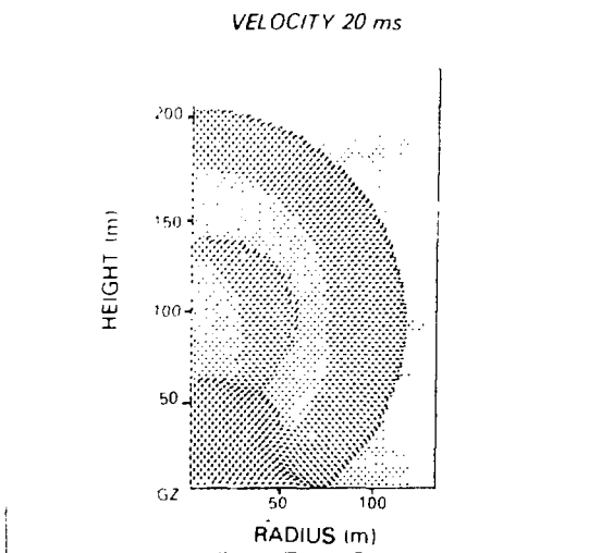
Figure 1. Flow field calculated for Epsht-Knothole BADGER (23 kt at 91 m) at 20 ms. The flow is characterized by the direct shock that has reached a radius of 120 m, the reflected shock that has reached 60-m altitude on the vertical axis, and their intersection, which is particularly prominent at about 75-m radius in the pressure plot. The expanding, spherical disturbance with a radius of about 40 m and centered on the burst point is real and can be seen in one-dimensional calculations.
