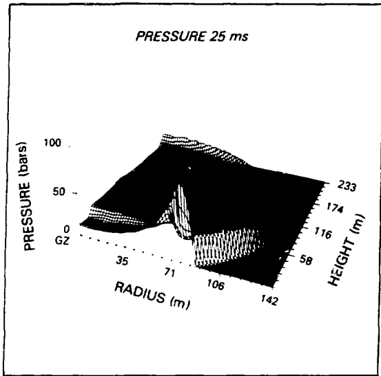
Figure 2. Badger at 25 ms. A rarefaction at ground zero (GZ) has lowered the pressure and created a strong positive pressure gradient at about 20-m altitude. The downward accelerations generated by this gradient are the source of the reverse vortex. Note the reflected shock in the acceleration plot, having reached 110-m altitude on axis.
