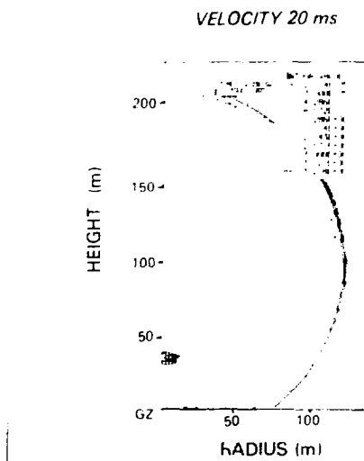
Figure 1. Flow field calculated for Epsht-Knothole BADGER (23 kt at 91 m) at 20 ms. The flow is characterized by the direct shock that has reached a radius of 120 m, the reflected shock that has reached 60-m altitude on the vertical axis, and their intersection, which is particularly prominent at about 75-m radius in the pressure plot. The expanding, spherical disturbance with a radius of about 40 m and centered on the burst point is real and can be seen in one-dimensional calculations.
