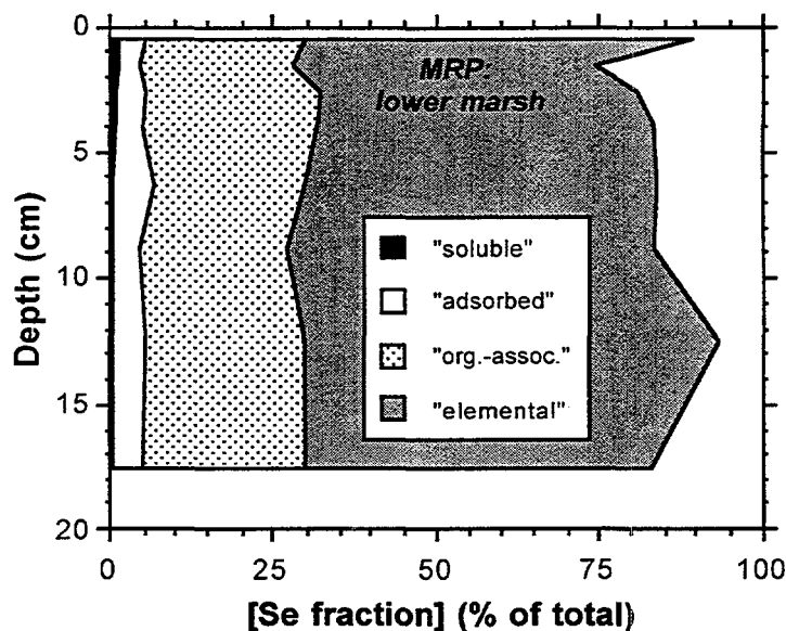
Figure 2.22 Se fractionation in lower marsh sediments from site MRP. The difference between total Se and the 4 fractions shown is "residual Se."
