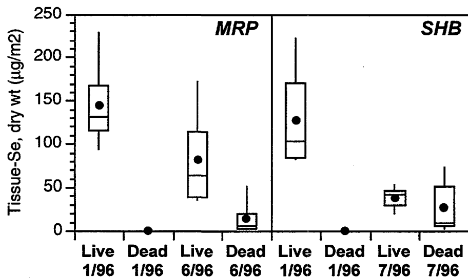
Figure 5.10 Tissue-Se mass in Scirpus californicus at sites MRP and SHB, normalized to marsh area.
