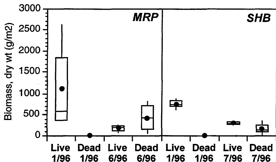
Figure 5.4 Biomass of Scirpus robustus at sites MRP and SHB.
