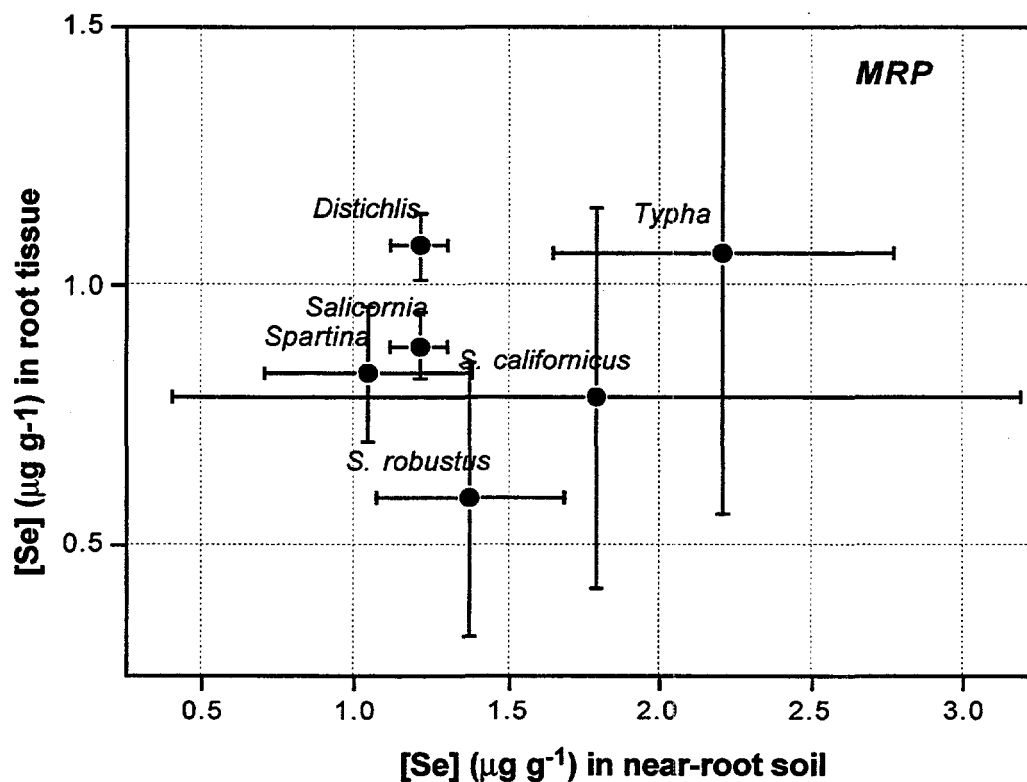
Figure 5.17 Se concentrations in roots of marsh plants at site MRP, vs. Se concentrations in near-root soil.
