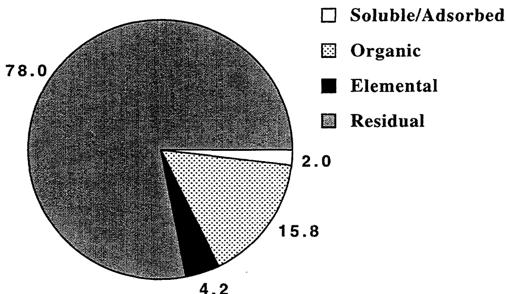
Figure 3.4 Speciation of Se on representative suspended sediment collected off the Martinez pier.
