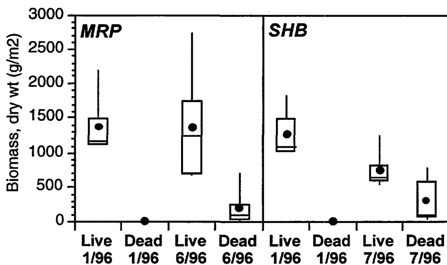
Figure 5.3 Biomass of Scirpus californicus at sites MRP and SHB.
