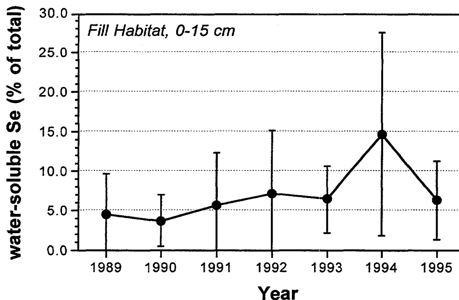
Figure 2.2.8. Water-soluble Se concentrations in the top 15 cm of Fill habitat soil, shown as percentage of total Se.
