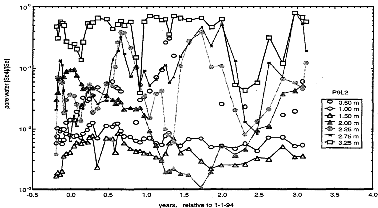
Figure 2.1.8. Time series for pore water [\text{Se(IV)}]:[\text{total Se}] ratios at various depths within site P9L.
