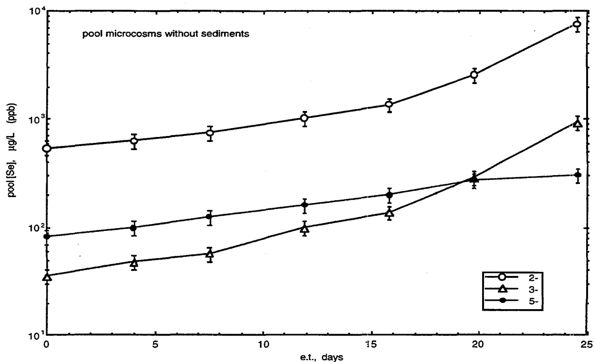
Figure 3.3.4a. Selenium concentrations in pool waters without sediments.
