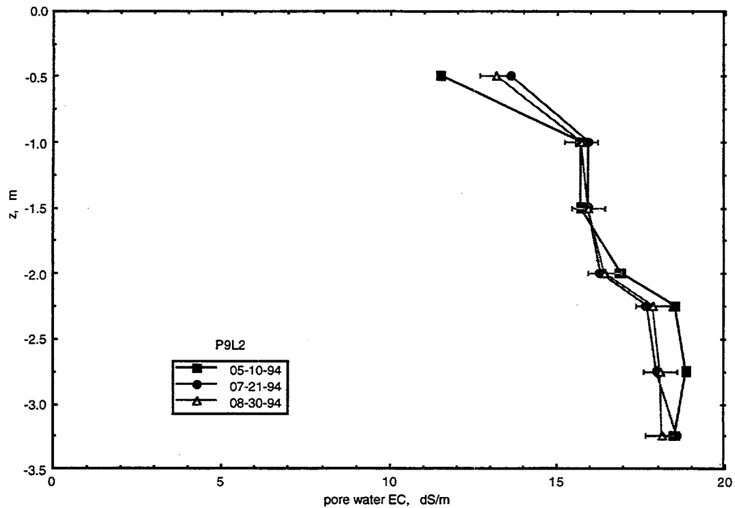
Figure 2.1.10a. Pore water EC profiles at site P9L2, during spring 1994 through summer 1994.
