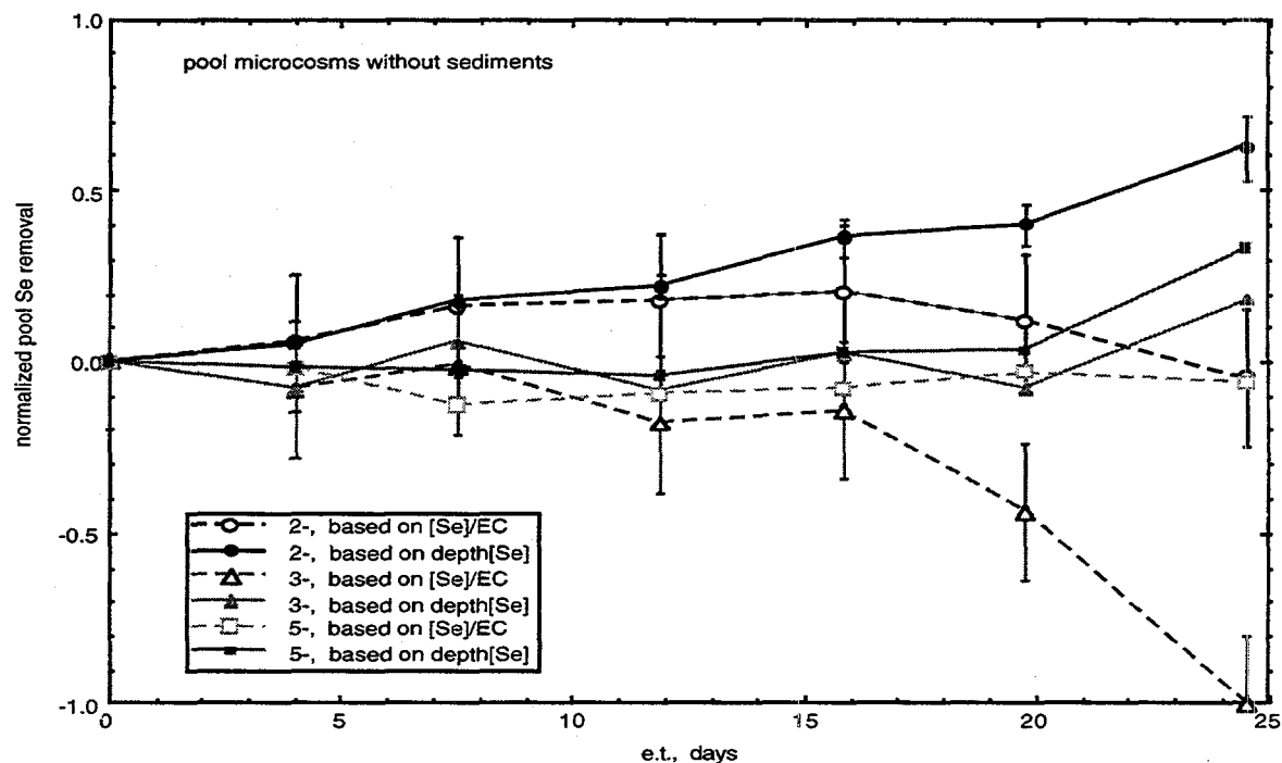
Figure 3.3.8a. Fraction of the initial pool water Se removed from solution during ponding without sediments. Calculations based on direct depth-concentration data and on Se/EC ratios are compared.
