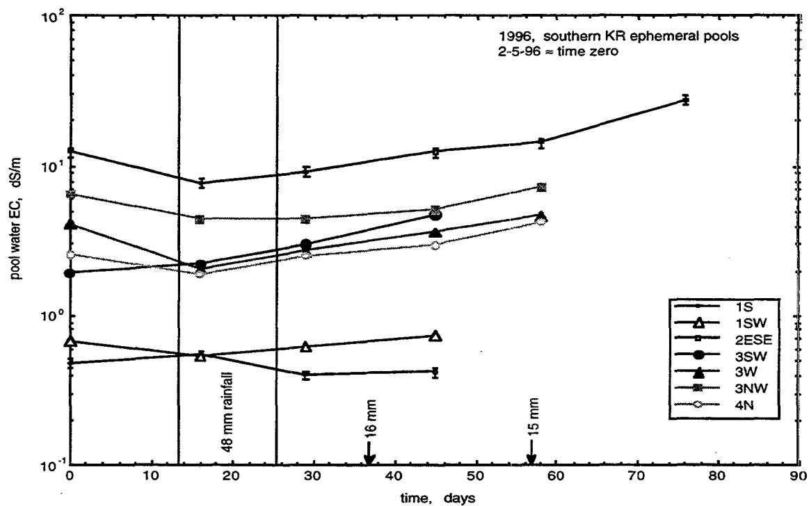
Figure 3.1.4c Time trends in 1996 ephemeral pool water salinities (southern KR pools).
