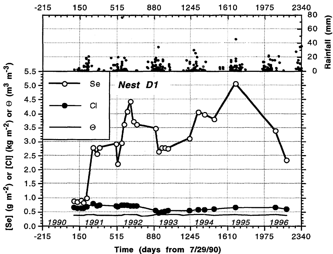
Figure 4.7. Mass of Se and Cl, and volumetric moisture content over the depth of 0.4 m to 1.00 m in treatment D, based on data from soil water samplers and neutron probe measurements at nest D1.
