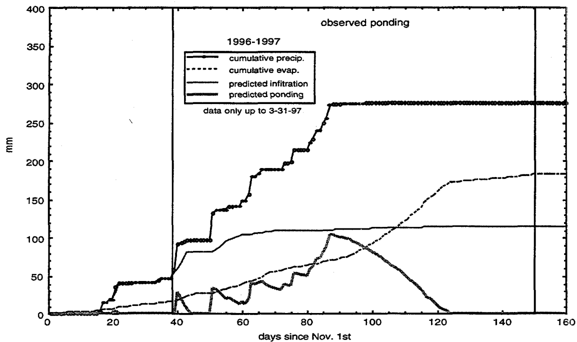
Figure 3.2.2h. Predicted versus observed duration of main ephemeral pools at Kesterson Reservoir during the 1996-97 wet season.
