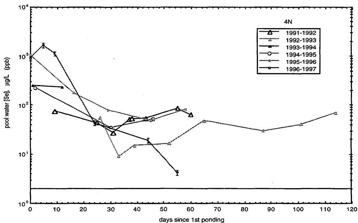
Figure 3.1.3b. Comparison of yearly trends in pool water Se concentrations at cattail site 4N. The horizontal line at 2 µg/L indicates the wetland surface water quality goal.
