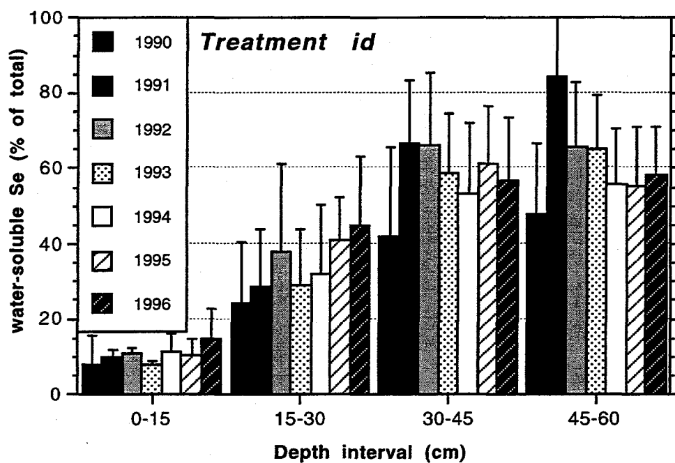
Figure 4.14. Mean water-soluble Se, as percentage of total, in 15-cm intervals of the top 60 cm of the soil profile along the N-S transect of treatment ID. Error bars represent one standard deviation from the arithmetic mean.
