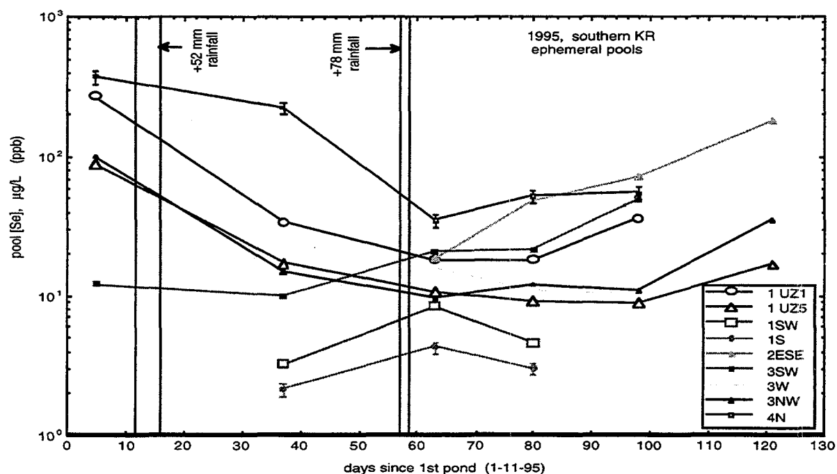
Figure 3.1.2a. Time trends in ephemeral pool Se concentrations. 1994-1995 wet season, southern pools.
