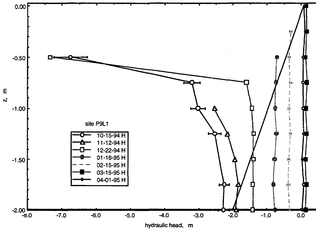
Figure 2.1.15a. Hydraulic head profiles at site P9L during the 1994-1995 wetting cycle. The gravitational head datum is at the soil surface. The diagonal line separates negative (matric) and positive pressure head values.
