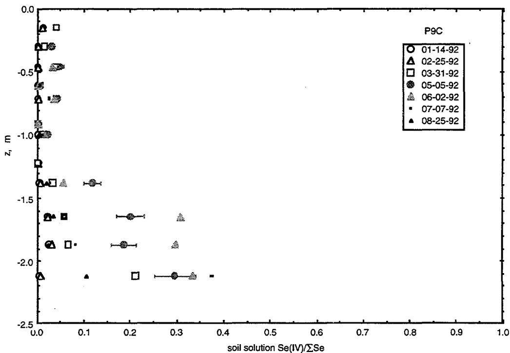
Figure 2.1.9a. Depth profiles of [Se(IV)]:[total\ dissolved\ Se] at site P9C during 1992. Flooding occurred on 2-12-92 at this site.
