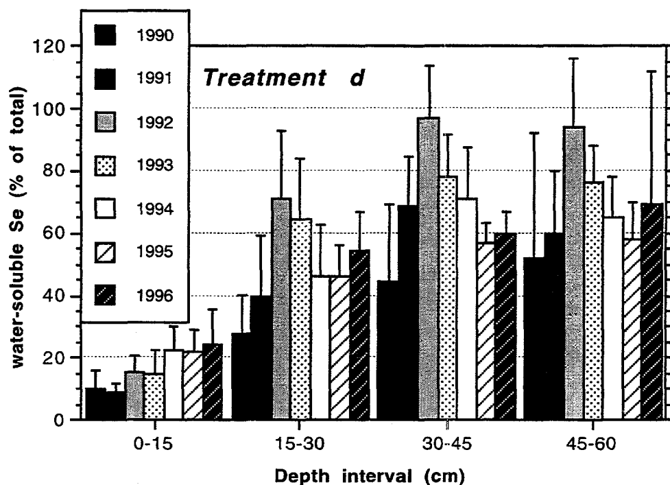
Figure 4.15. Mean water-soluble Se, as percentage of total, in 15-cm intervals of the top 60 cm of the soil profile along the N-S transect of treatment D. Error bars represent one standard deviation from the arithmetic mean.
