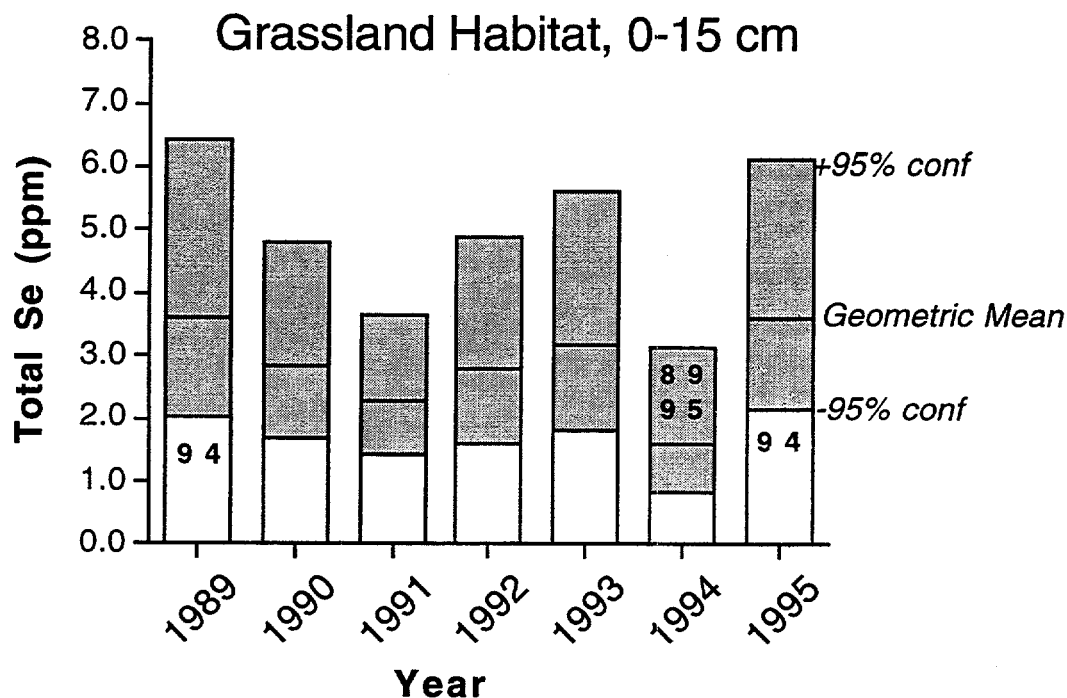
Figure 2.2.4. Total Se concentrations in the top 15 cm of soil in the Grassland habitat. Years which were significantly different at the 95% confidence interval shown for each year.
