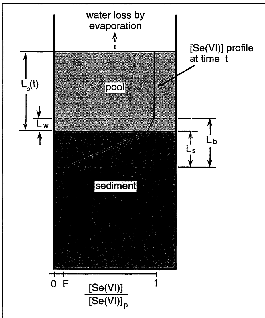
Figure 3.3.1. Conceptual model for estimating Se(VI) transport from pool waters into sediments. L_p(t) is the pool depth at time t ; L_w is the pool boundary layer thickness; L_s is the sediment boundary layer thickness; L_b is the composite boundary region thickness.
