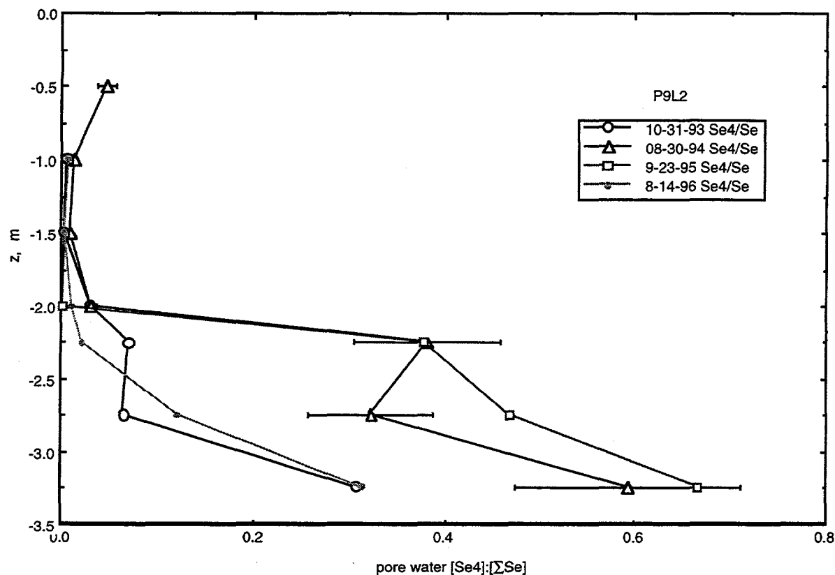
Figure 2.1.3b. Late summer- early fall depth profiles of pore water [Se(IV)]:[total Se] ratios, 1993 - 1996.
