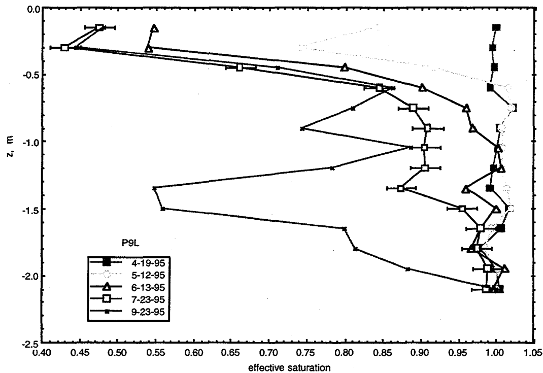
Figure 2.1.13b. Depth profiles of effective water saturation during the 1995 drying cycle at site P9L.
