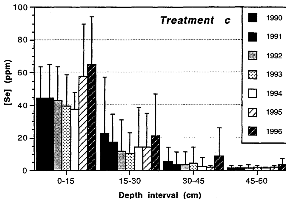
Figure 4.12. Mean total Se concentrations in 15-cm intervals of the top 60 cm of the soil profile along the N-S transect of treatment C. Error bars represent one standard deviation from the arithmetic mean.
