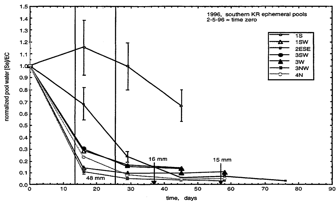
Figure 3.1.5c. Trends in ratios of pools Se to EC, normalized to values in initial samples. 1996, southern KR pools.
