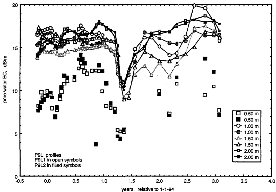
Figure 2.1.12a. Time series of pore water EC from the 0.50 m to 2.00 m depths at sites P9L1 and P9L2.
