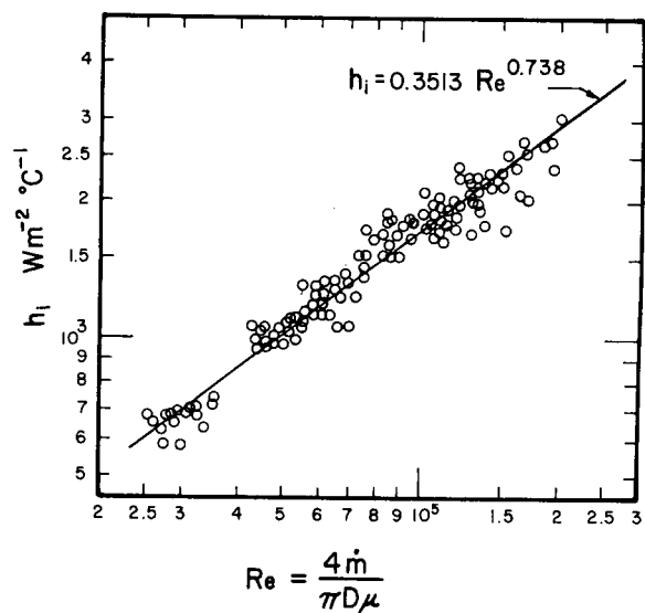
Fig.4 Inside heat transfer film coefficient for heating isobutane at 4.14 MPa Vs Reynolds number for data Set A away from the pseudocritical temperature
