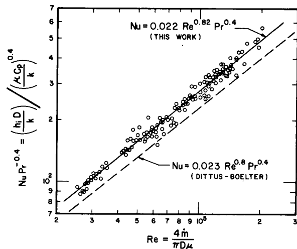
Fig.5 Dimensionless plot of data on heating isobutane at 4.14 MPa vs Reynolds number for data Set A away from the pseudocritical temperature
