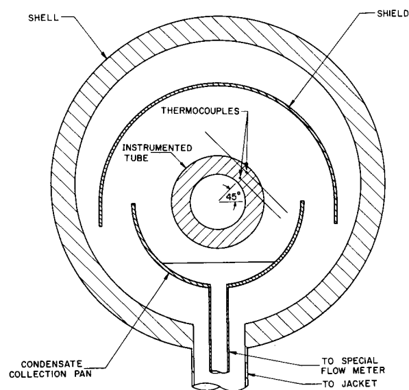
Fig.3 Heater cross section showing tube, condensate tray, drip shield and outer shell
