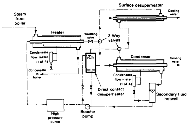
Fig.1 Binary fluid experiment, schematic flow diagram
