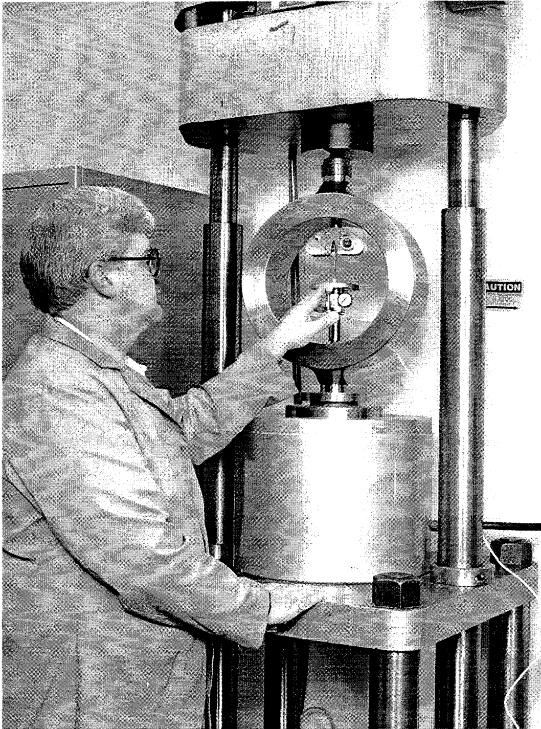
Proving Ring Calibration
