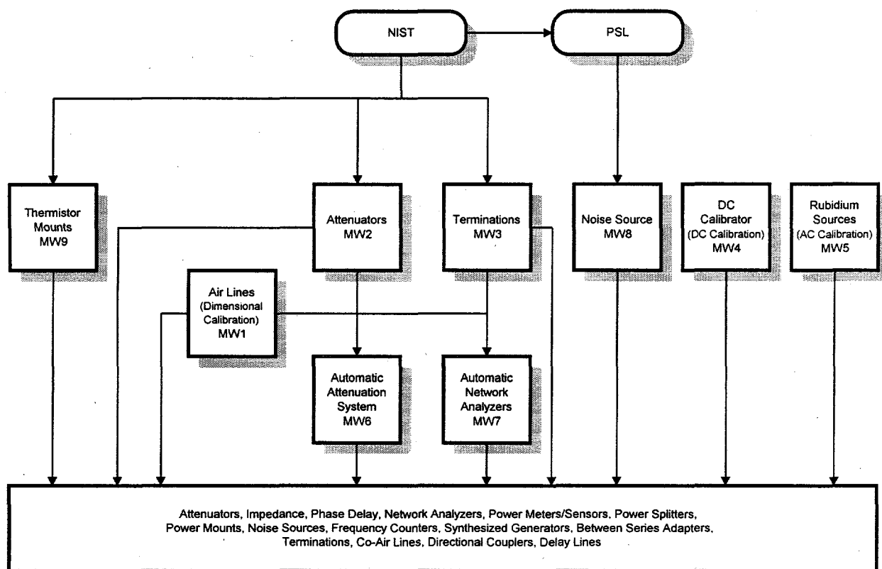
Figure 6C: Radio Frequency and Microwave Traceability
