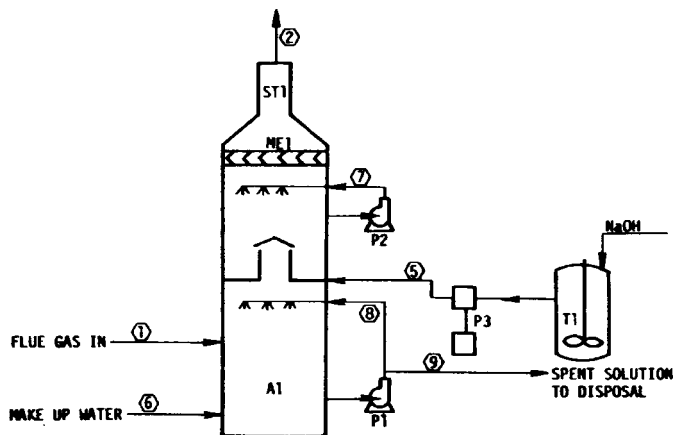
Figure 14-35. Sun Production Company, Oildale, California; Fellows, California.
