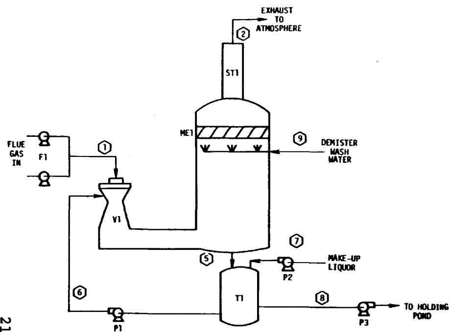
Figure 14-29. Northern Ohio Sugar Co., Freemont, Ohio.
