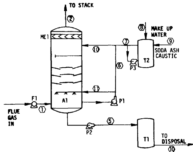
Figure 14-17. Getty Oil Company. Bakersfield, California FMC Environmental Eqmnt.
