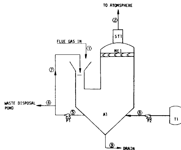
Figure 14-25. Mobil Oil Company, Buttonwillow, California.
