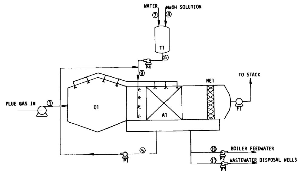
Figure 14-37. Texaco, Inc., San Ardo, California. Ceilcote
