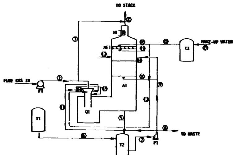
Figure 14-38. Texasgulf, Granger, Wyoming.
