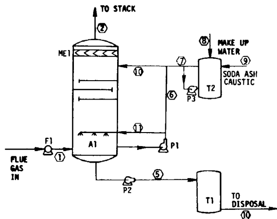
Figure 14-18. Getty Oil Company, Bakersfield, California. In-House Design
