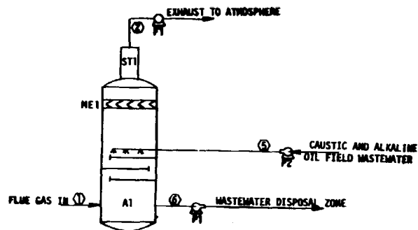
Figure 14-26. Mobil Oil Corp., San Ardo, California.
