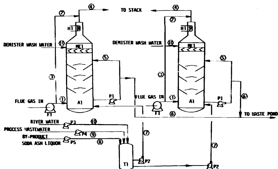
Figure 14-11. FMC (Soda Ash Plant), Green River, Wyoming.
