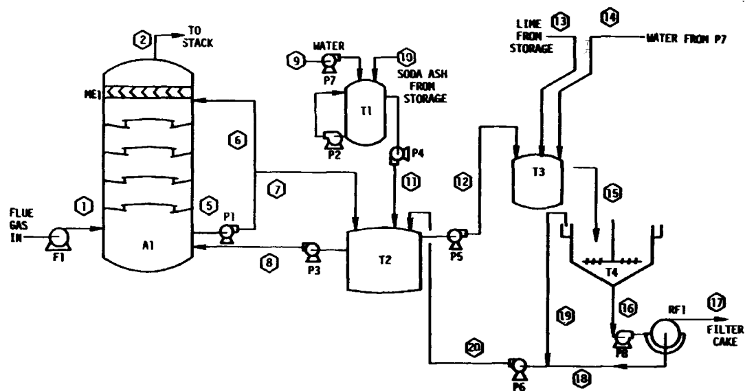
Figure 14-32. Santa Fe Energy Corp., Bakersfield, California.
