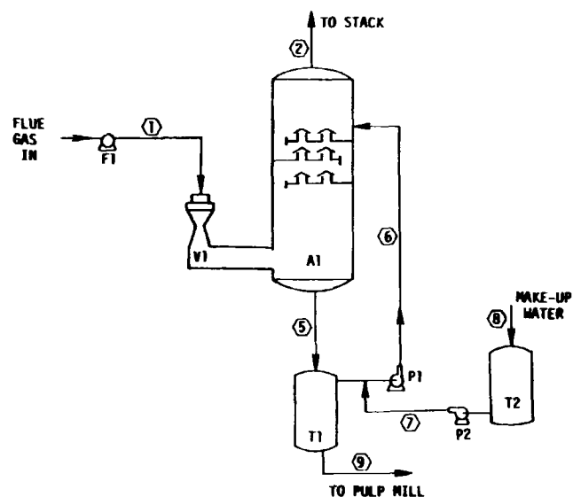
Figure 14-23. Mead Paperboard Co. Stevenson, Alabama .
